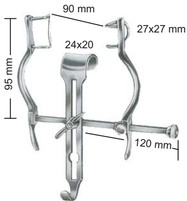
Baby-Balfour Retractor complete 0015-0628-000
