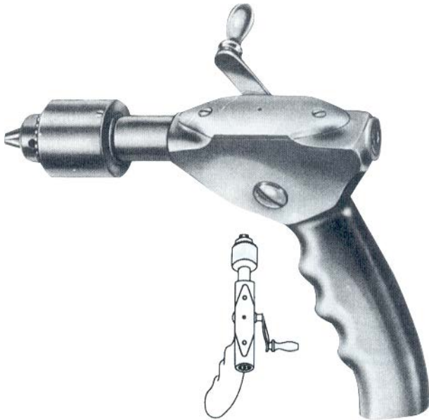
Ralk 0022-0334-000 accomodating up to 6.35mmØ
