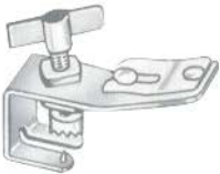
0023-0045-001 Fixation base, for skull mounting, holding 1 flexible arm
