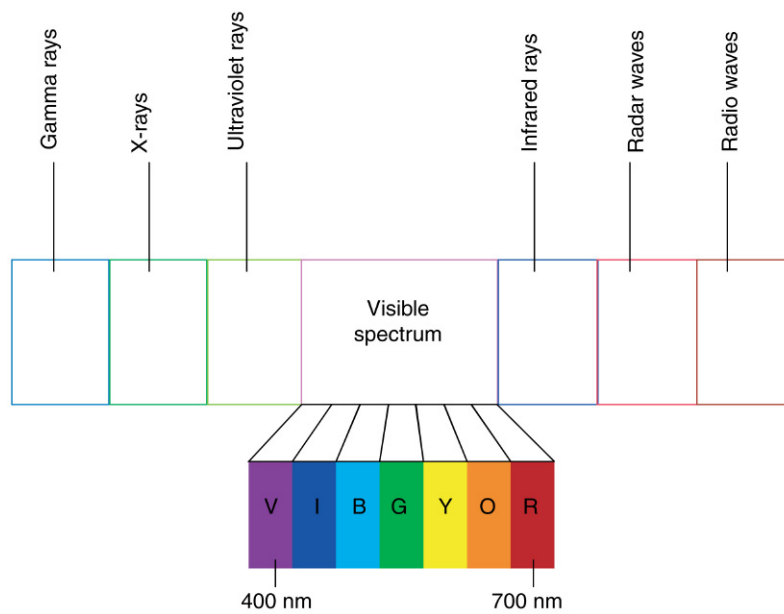
Figure 73.1. Electromagnetic spectrum.
