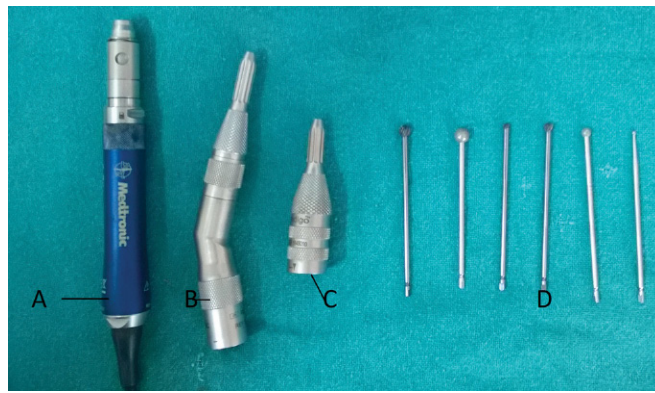
Mastoid drill. (A) Motor. (B) Curved hand piece. (C) Straight hand piece. (D) Different types of burs.
