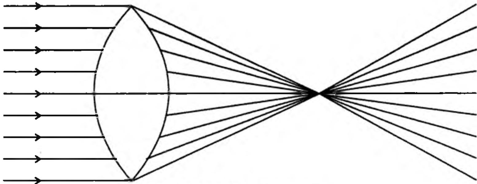
Fig. 32.17 Spherical aberration.
