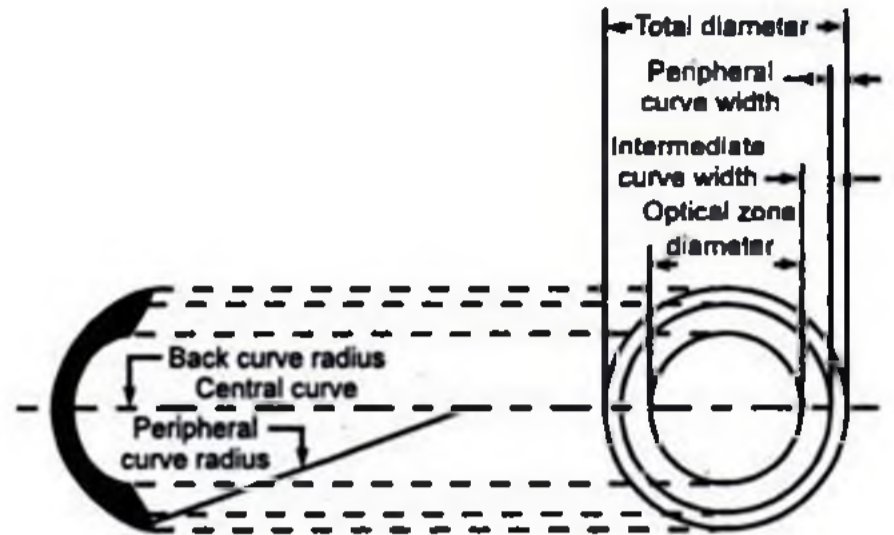
Fig. 32.33 Different measurements of hard contact lens.
