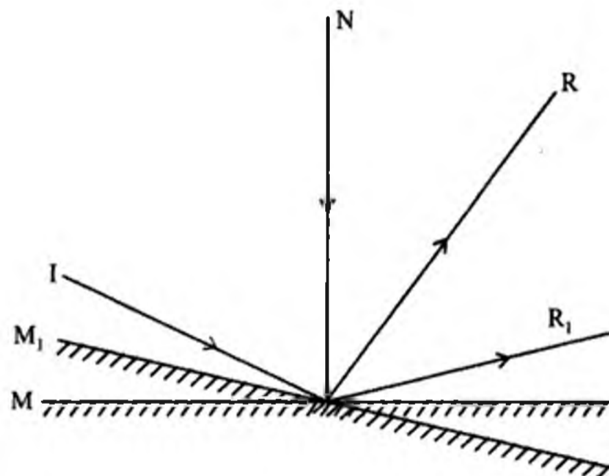
Fig. 32.2 Rotation of a plane mirror M: IN , the normal; the incident ray: R , the reflected ray; and M_1 , the mirror tilted.
