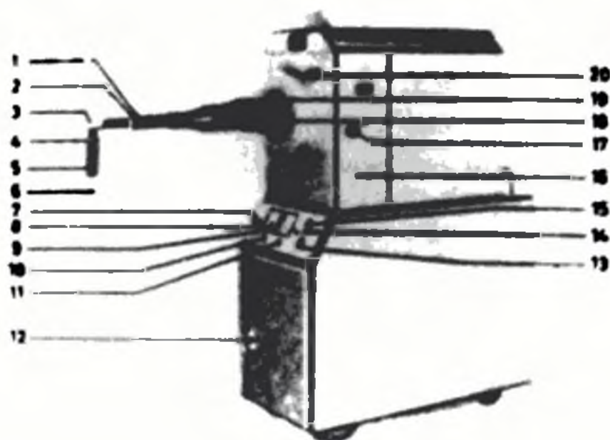
Fig. 51.40 Carl-Zeiss light coagulation apparatus: 1, Filter disc; 2, Image field diaphragm; 3, Mirror; 4, Release knob; 5, Handle; 6, Cable; 7, Cable connection; 8, Ammeter; 9, Voltmeter; 10, Switch-OFF; 11, Switch-ON; 12, Protective switch; 13, Multi-stage switch for normal load; 14, Selector switch; 15, Multi-stage switch for overload; 16, Door; 17, Door-handle; 18, Optical beam director; 19, Lever for iris diaphragm; 20, Locking lever (Meyer-Schwickerath).
