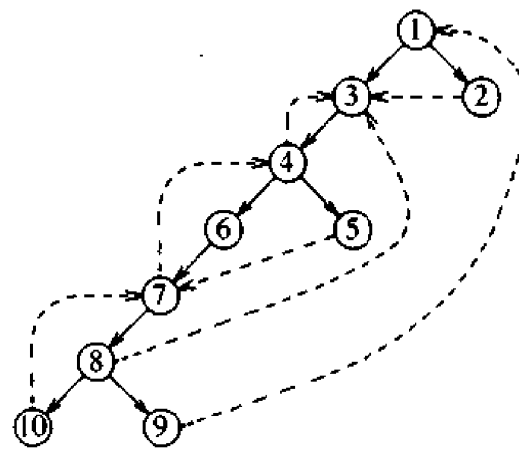
Fig. 10.46. Depth-first presentation
