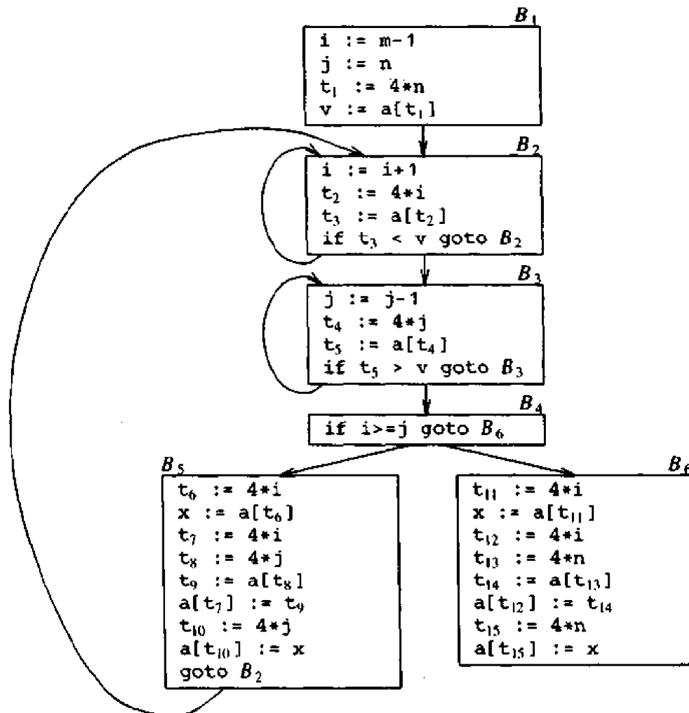
Fig. 10.5. Flow graph.
