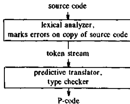
Fig. 12.2. Pascal-P compiler.
