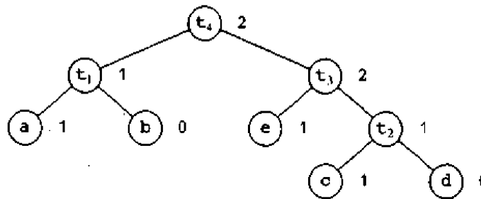
Fig. 9.24. Labeled tree.
