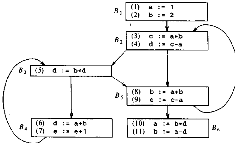
Fig. 10.74. Flow graph.
