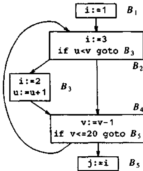
Fig. 10.37. Illustrating condition (2).
