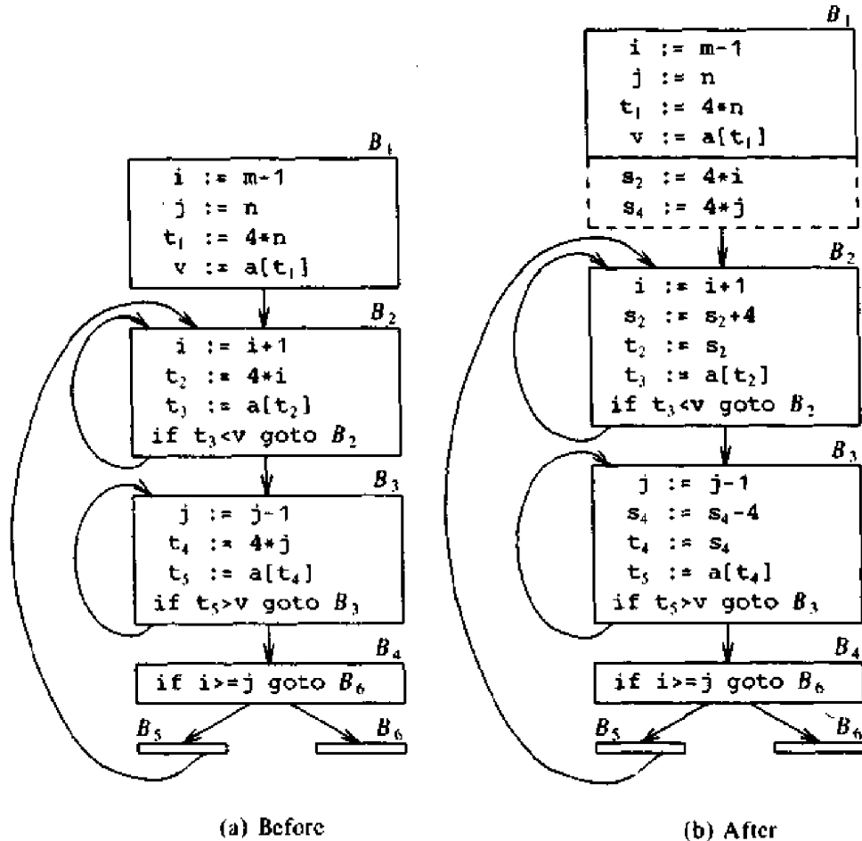
Fig. 10.39. Strength reduction.
