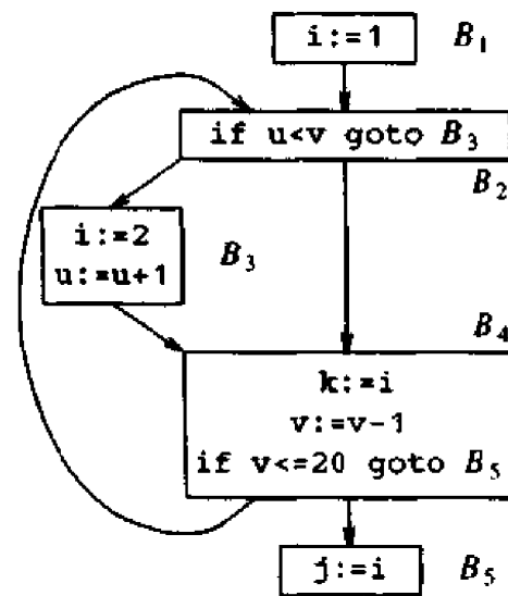
Fig. 10.38. Illustrating condition (3).
