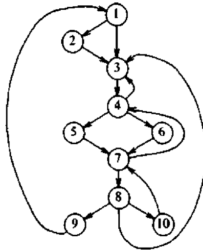
Fig. 10.13. Flow graph.
