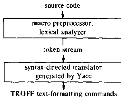
Fig. 12.1. EQN implementation.
