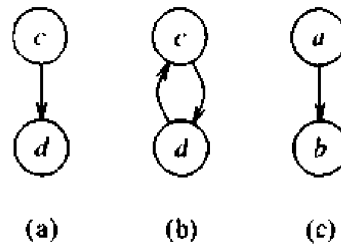
Fig. 10.51. Some regions.
