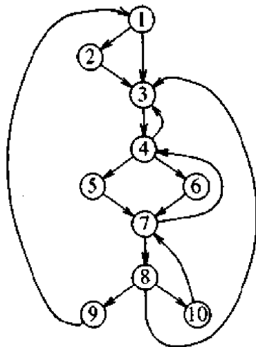
Fig. 10.45. Flow graph
