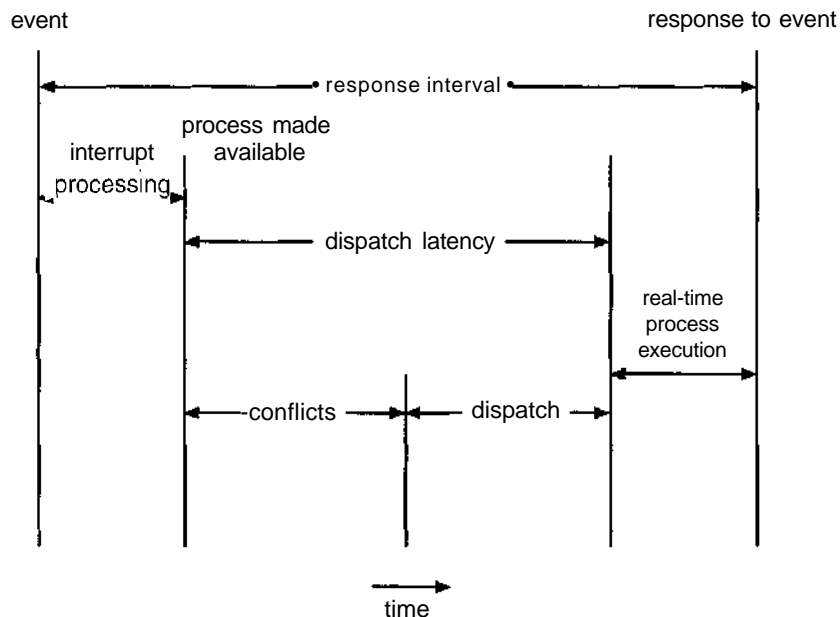
Figure 19.5 Dispatch latency.
