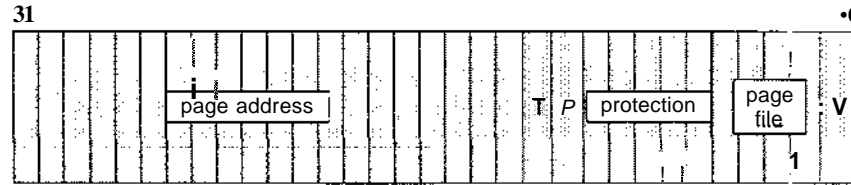
Figure 22.5 Page-file page-table entry. The valid bit is zero.
