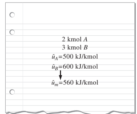
FIGURE 13-12 The intensive properties of a mixture are determined by weighted averaging.
