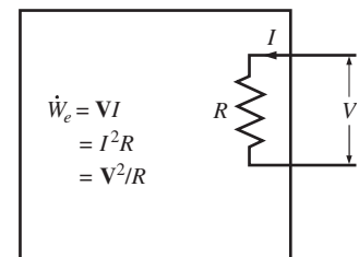
FIGURE 2–24 Electrical power in terms of resistance R , current I , and potential difference \mathbf{V} .
