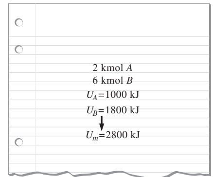
FIGURE 13-11 The extensive properties of a mixture are determined by simply adding the properties of the components.
