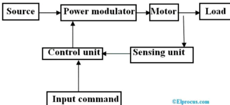
Fig.8.1.2 Electrical Drives And Their Block Diagram
