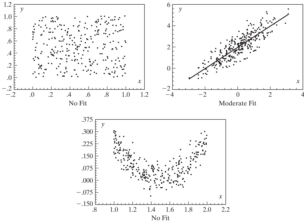
FIGURE 3.3 Sample Data.
