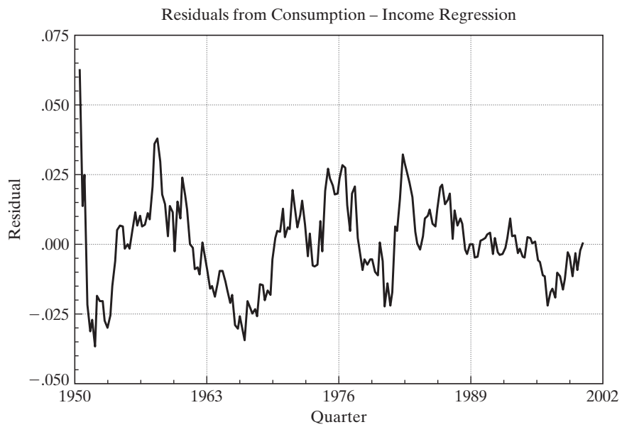
FIGURE 20.17 Regression Residuals.
