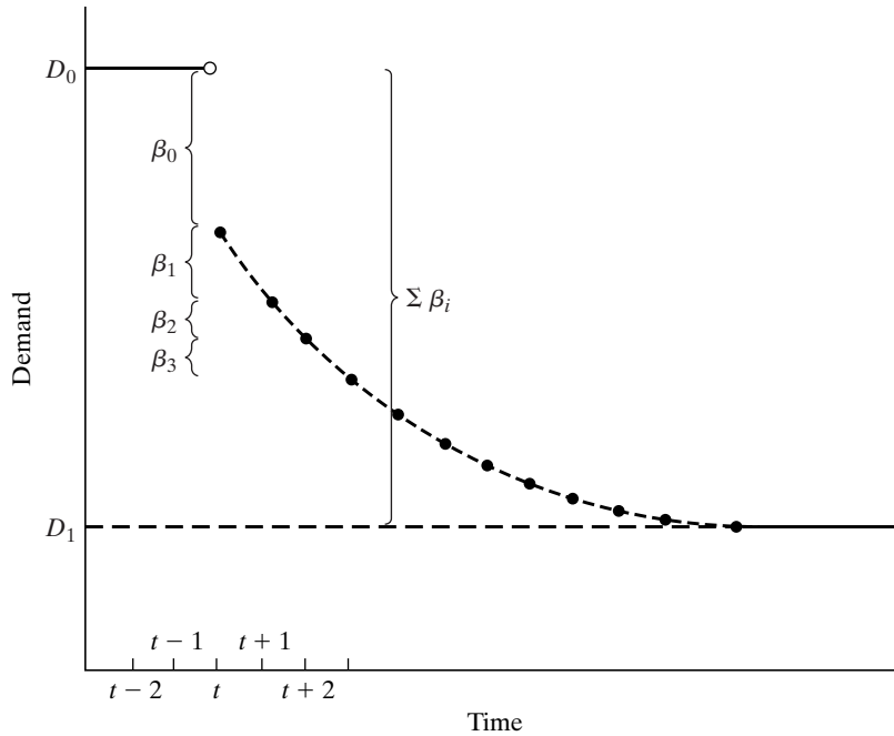
FIGURE 19.1 Lagged Adjustment.
