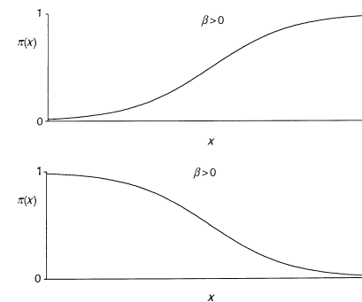
Figure 3.2. Logistic regression functions.
