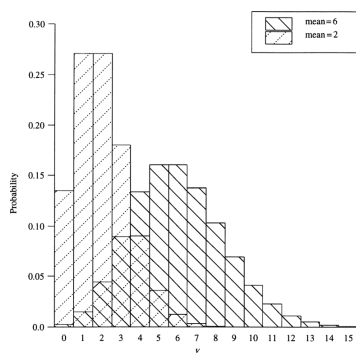
Figure 3.3. Poisson distributions having means 2 and 6.
