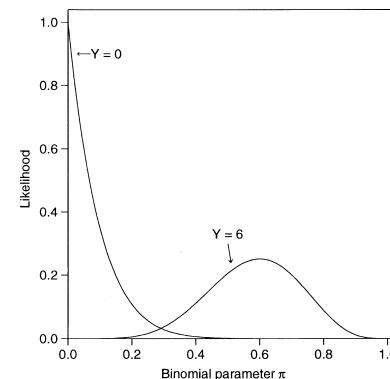
Figure 1.1. Binomial likelihood functions for y = 0 successes and for y = 6 successes in n = 10 trials.
