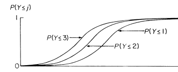
Figure 6.2. Depiction of cumulative probabilities in proportional odds model.
