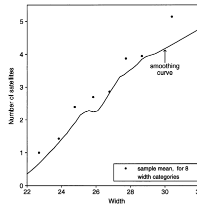
Figure 3.5. Smoothings of horseshoe crab counts.
