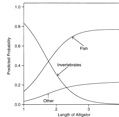
Figure 6.1. Estimated probabilities for primary food choice.
