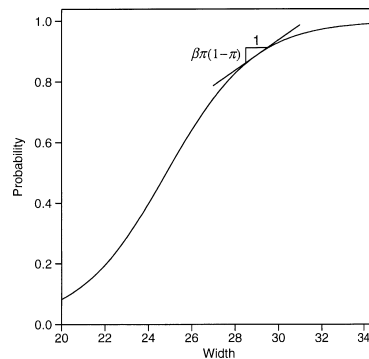
Figure 4.1. Linear approximation to logistic regression curve.
