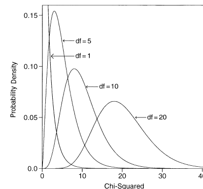
Figure 2.2. Examples of chi-squared distributions.
