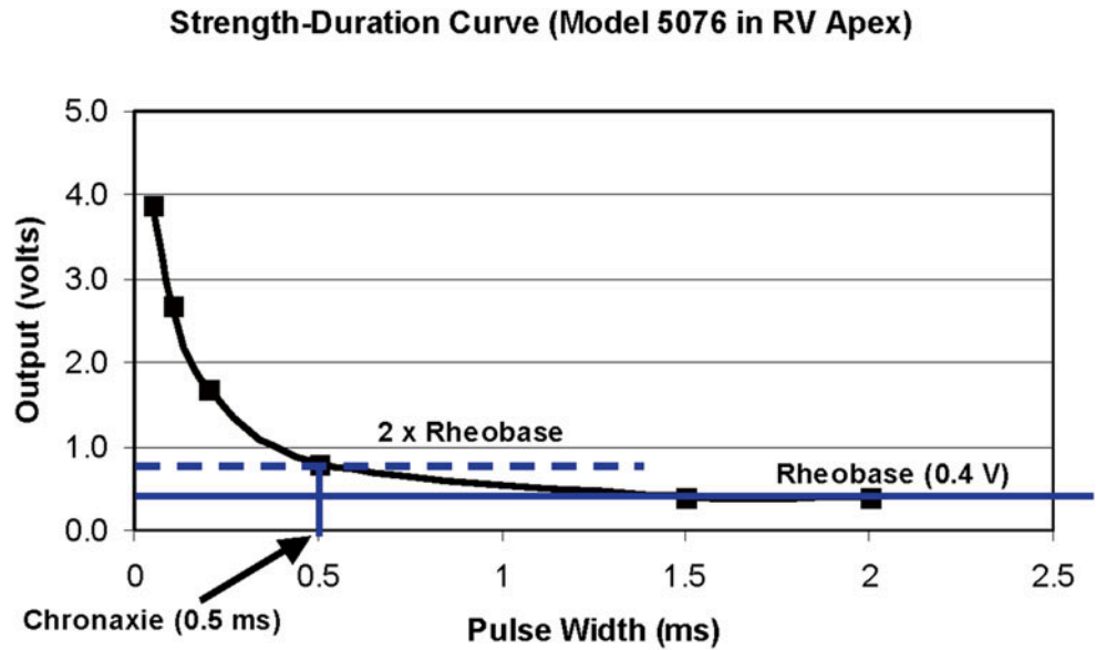
Fig. 30.6 A typical strength-duration curve for cardiac pacing. This particular curve was obtained using a Medtronic model 5076 bipolar pacing lead positioned in the right ventricular (RV) apex of a canine. In this plot, chronaxie and rheobase were 0.5 ms and 0.4 V, respectively
