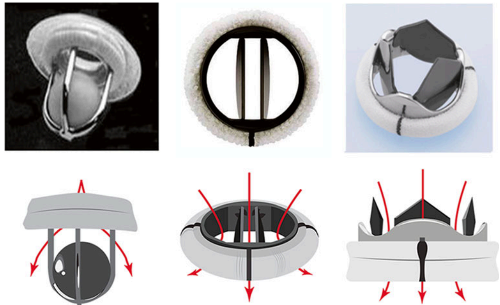
Fig. 27.2 Comparison of different mechanical valves with their flow characteristics. The evolution of the valve from the Starr-Edwards ball (left), the current standard bi-leaflet (center; St. Jude Medical, St. Paul, MN, USA), and a novel trileaflet design (right, Triflow Medical Inc.) currently in development. Below each valve is a stylized representation of the flow patterns reflecting the improvement in valve design
