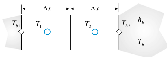
Fig. 13.23 One-dimensional domain used for Exercise 3
