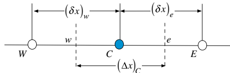
Fig. 8.6 Interpolation of properties at element faces
