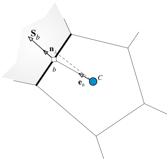
Fig. 12.20 Wall boundary condition for the convection flux
