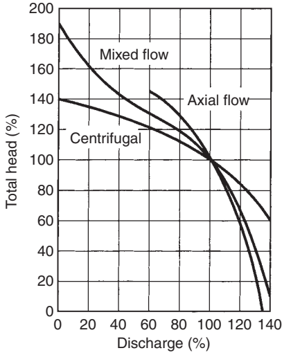
(a) Discharge-head
