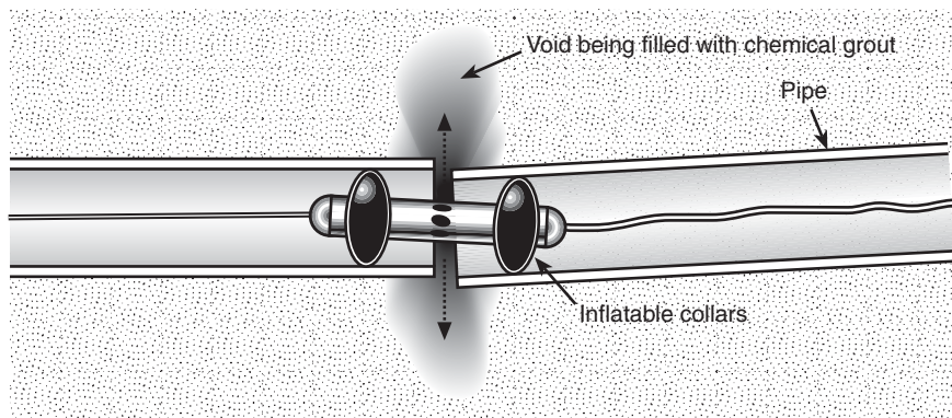
Fig. 18.2 Chemical grouting
