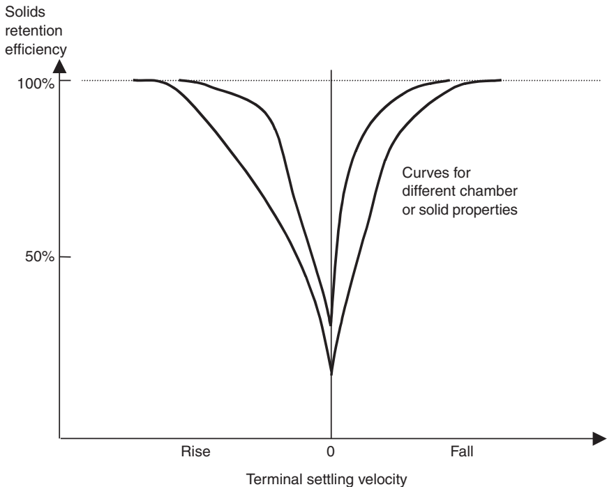
Fig. 12.13 Plots of CSO solids separating efficiency (conceptual)
