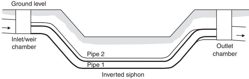
Fig. 9.12 Inverted siphon for wastewater, vertical section (schematic)
