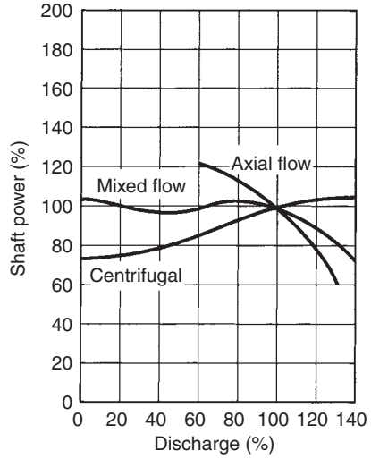
(b) Discharge-power
