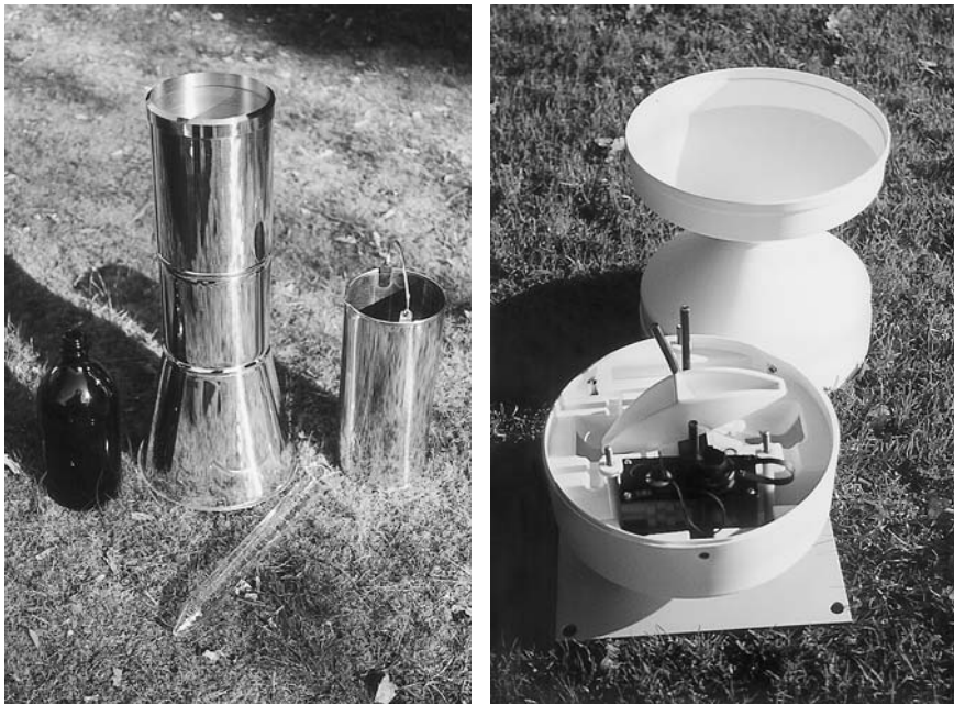
Fig. 5.1 Rain gauges: (a) standard; (b) tipping bucket (courtesy of Hydrokit, Poole)
