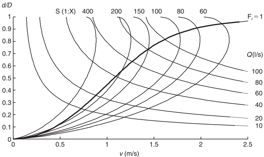
Fig. 8.9 Butler-Pinkerton chart ( D 300 mm, k_s 0.6 mm)
