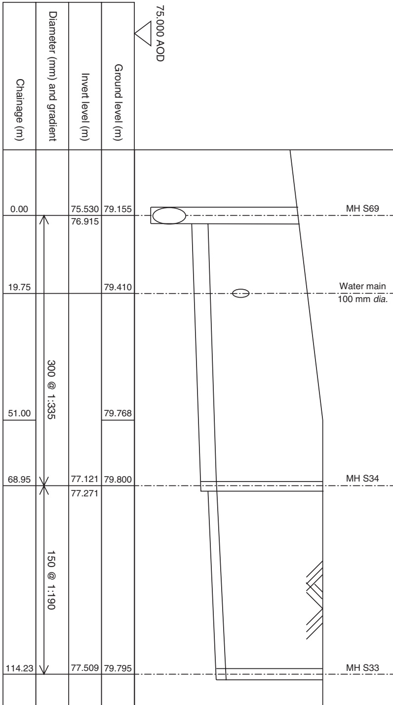
Fig. 7.3 Longitudinal profile of a sewer
