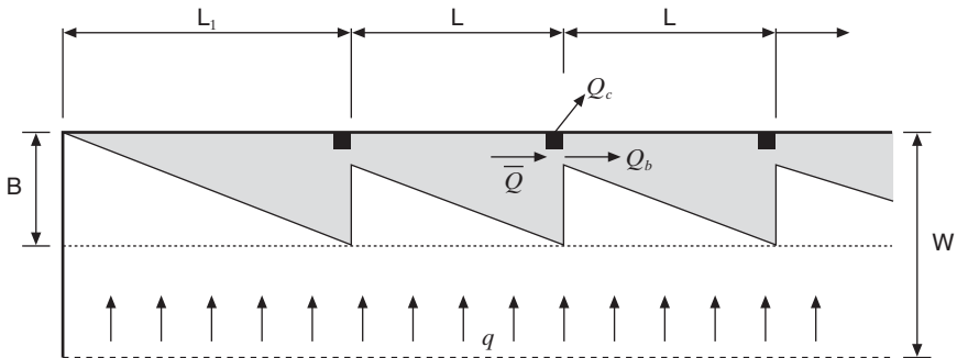
Fig. 9.16 Spacing of initial and intermediate gullies
