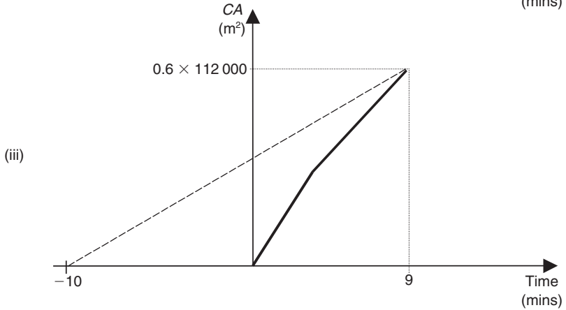
Fig. 11.5 Time-area diagrams
