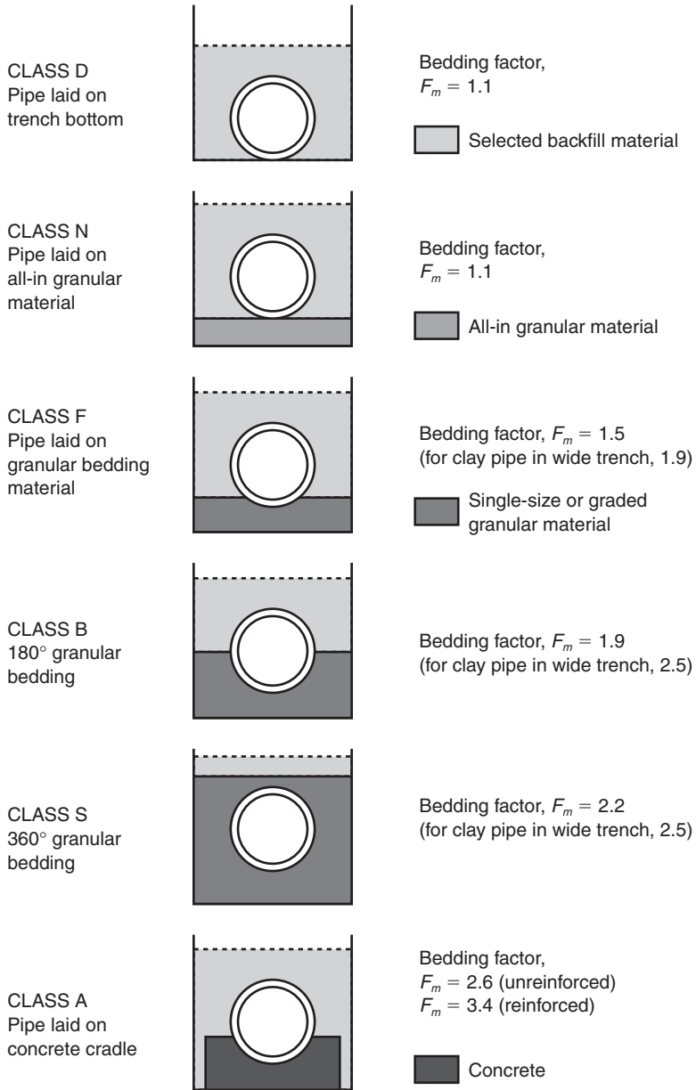
Fig. 15.4 Bedding classes and bedding factors
