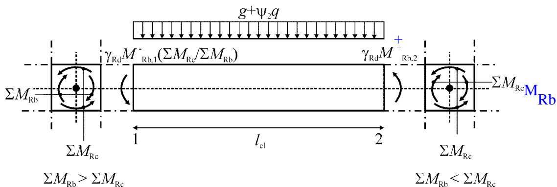
Figure 5.1: Capacity design values of shear forces on beams
