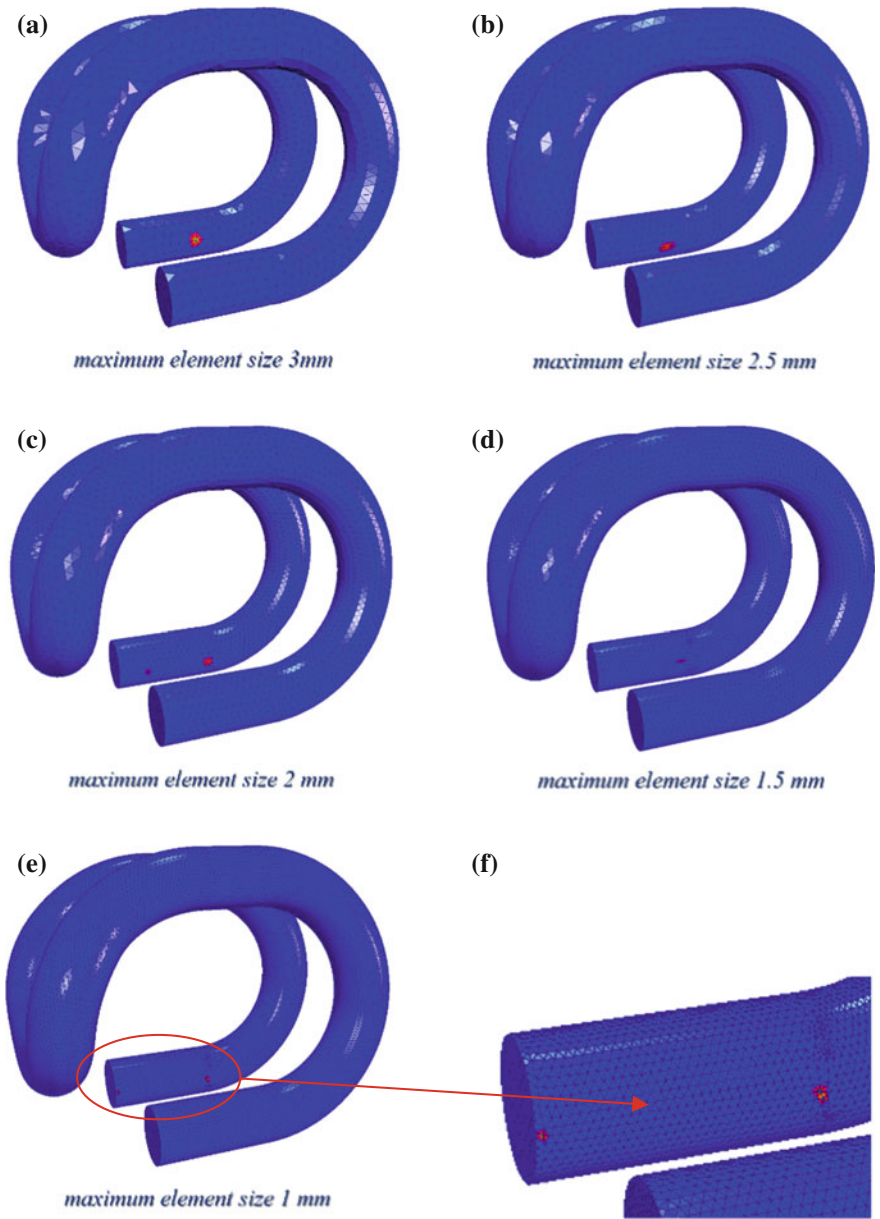
Fig. 8.13 Normal contact stress on the contact surface of spring clips for different element size
