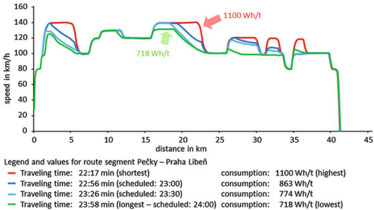
Fig. 2.10 Graph showing effect of different driving behaviours on energy consumption and travel time of a train between Pečky and Praha Libeň ( source Ceske Drah)
