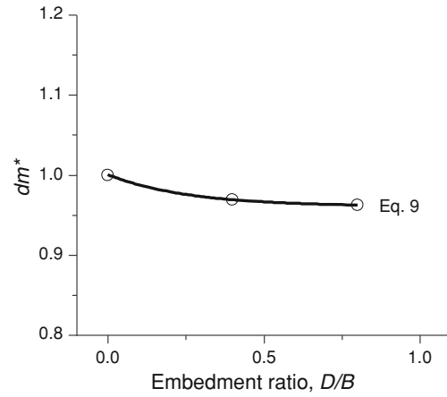
Fig. 7 Decrease in normalised moment load capacity with embedment
