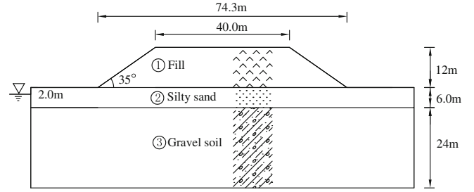
Fig. 2 Engineering geology cross section of embankment slope
