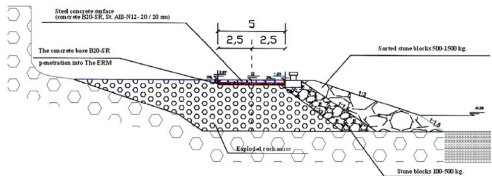
Fig. 7 Profile of the strengthening of the sea coast near town of Primorsko with embankment of exploded rocks
