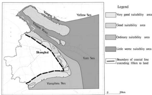
Fig. 3 Sketch map showing the suitability of pile foundation projects
