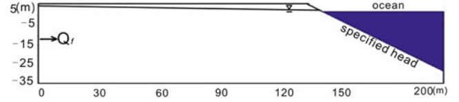
Fig. 2 Model domain and boundary conditions
