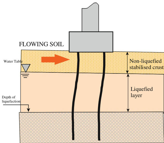
Fig. 9 Failure mechanism based on lateral spreading
