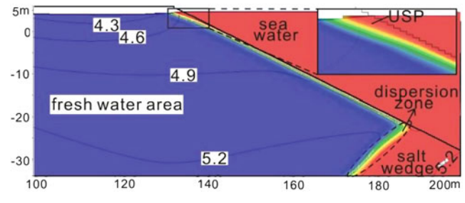
Fig. 4 Salt concentration (colored area) and head equivalent (contours) at high tide
