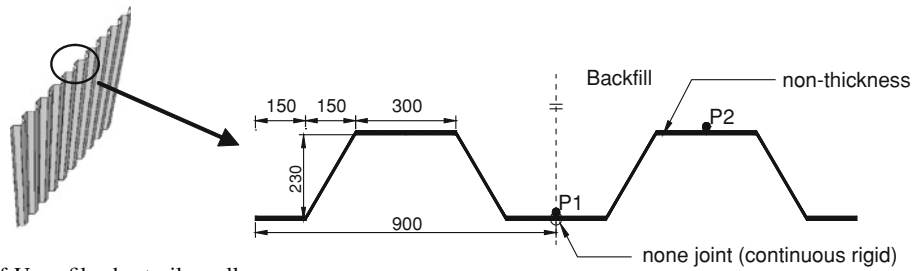
Fig. 5 Dimensions of U-profile sheet pile wall
