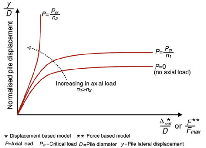
Fig. 16 Plot of normalised pile head displacement and normalised force/ground displacement
