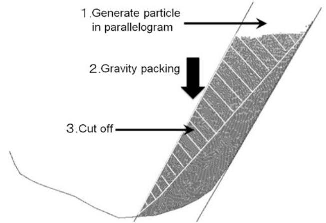
Fig. 2 Calculation process for constructing Landslide body and appearance of gravity packing
