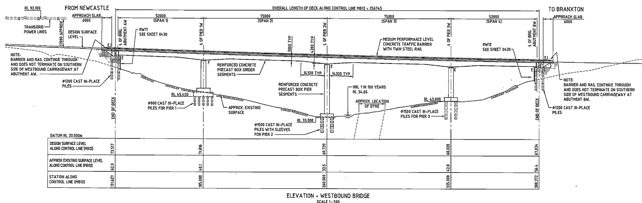
Fig. 2 BW010 cross section view
