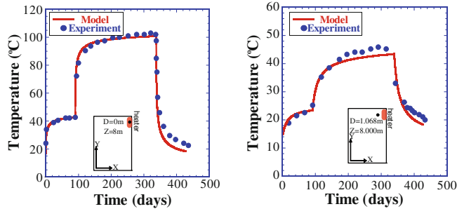
Fig. 4 Change of temperature at different position
