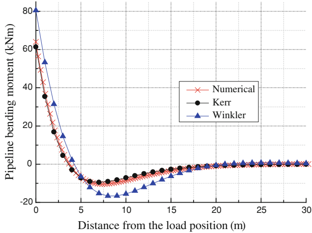
Fig. 7 Pipeline moment under concentrated load
