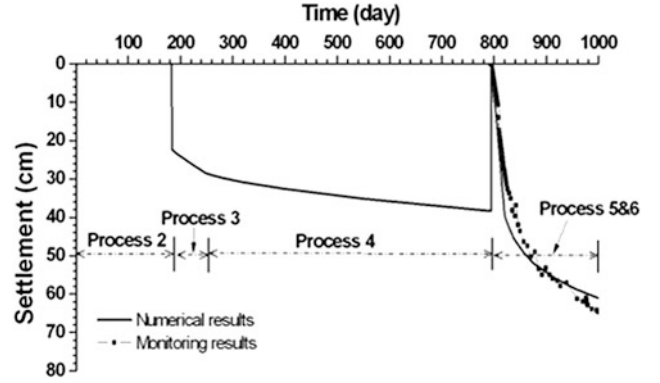
Fig. 2 Temporal changing curves of the surface settlement
