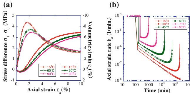
Fig. 1 Theoretical prediction of host rock by the proposed model a triaxial compression test b triaxial creep test
