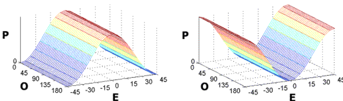
Polarization signatures of a large conducting sphere. P = Power, O = Orientation (degrees), E = Ellipticity (degrees)
