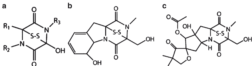
Fig. 8.1 Structures of epithiodioxopiperazines. (a) Core epithiodioxopiperazine (ETP) moiety; (b) sirodesmin PL; (c) gliotoxin
