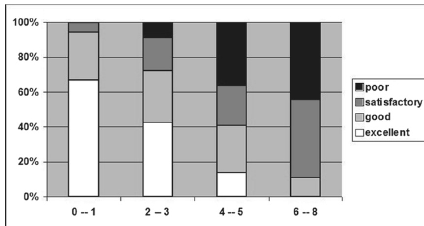
Fig. 1 Responder rate
