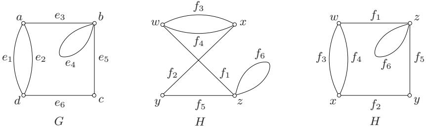
Fig. 1.6. Isomorphic graphs
