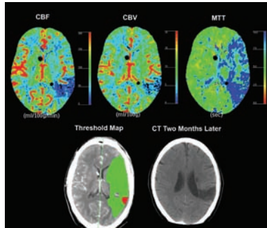
Fig. 9.6 Deconvolution method
