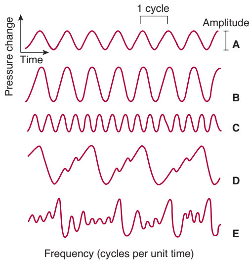
FIGURE 13-8 Characteristics of sound waves. A is the record of a pure tone. B has a greater amplitude and is louder than A . C has the same amplitude as A but a greater frequency, and its pitch is higher. D is a complex wave form that is regularly repeated. Such patterns are perceived as musical sounds, whereas waves like that shown in E , which have no regular pattern, are perceived as noise.
