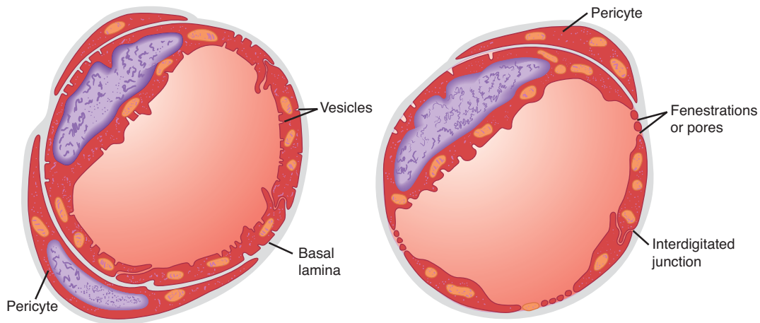
FIGURE 32-19 Cross-sections of capillaries. Left: Type of capillary found in muscle. Right: Fenestrated type of capillary. (Reproduced with permission from Fawcett DW: Bloom and Fawcett, Textbook of Histology , 11th ed. Saunders, 1986.)
