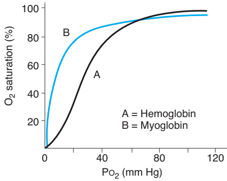
FIGURE 36-5 Dissociation curve of hemoglobin and myoglobin. The myoglobin binding curve (B) lacks the sigmoidal shape of the hemoglobin binding curve (A) because of the single O 2 binding site in each molecule. Myoglobin also has greater affinity for O 2 than hemoglobin (curve shifted left) and thus can store O 2 in muscle.
