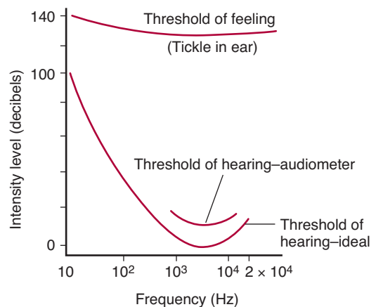
FIGURE 13-9 Human audibility curve. The middle curve is that obtained by audiometry under the usual conditions. The lower curve is that obtained under ideal conditions. At about 140 decibels (top curve), sounds are felt as well as heard.
