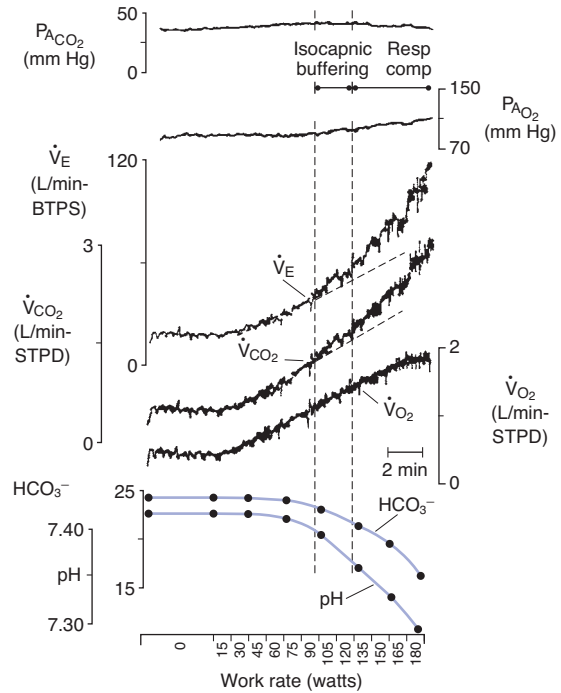
FIGURE 37–15 Physiologic responses to work rate during exercise. Changes in alveolar \text{PCO}_2 , alveolar \text{PO}_2 , ventilation ( \dot{V}_E ), \text{CO}_2 production ( \dot{V}_{\text{CO}_2} ), \text{O}_2 consumption ( \dot{V}_{\text{O}_2} ), arterial \text{HCO}_3^- , and arterial pH with graded increases in work by an adult male on a bicycle ergometer. Resp comp, respiratory compensation. See text for details. (Reproduced with permission from Wasserman K, Whipp BJ, Casaburi R: Respiratory control during exercise. In: Handbook of Physiology , Section 3, The Respiratory System . Vol II, part 2. Fishman AP [editor]. American Physiological Society, 1986.)
