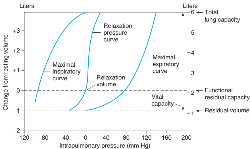
FIGURE 35-10 Intrapulmonary pressure and volume relationship, the relaxation pressure curve. The middle curve is the relaxation pressure curve of the total respiratory system; that is, the static pressure curve of values obtained when the lungs are inflated or deflated by various amounts and the intrapulmonary pressure (elastic recoil pressure) is measured with the airway closed. The relaxation volume is the point where the recoil of the chest and the recoil of the lungs balance. The slope of the curve is the compliance of the lungs and chest wall. The maximal inspiratory and expiratory curves are the airway pressures that can be developed during maximal inspiratory and expiratory efforts.
