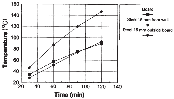
Fig. 10.5 Temperatures of protection board and steel plate in compartment adjacent to fire; 150 \times 10 mm protection on each side of wall; plate thickness 22 mm
