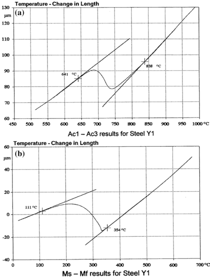
Fig. 7.2 Dilation curves of as-forged steel after cooling to -196^{\circ}\text{C} . a A_{c1} - A_{c3} ; b M_s - M_f (From Sha et al. (2011), www.maney.co.uk/journals/mst and www.ingentaconnect.com/content/maney/mst )
