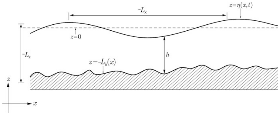
Fig. 4.16 Schematic drawing of a shallow water system
