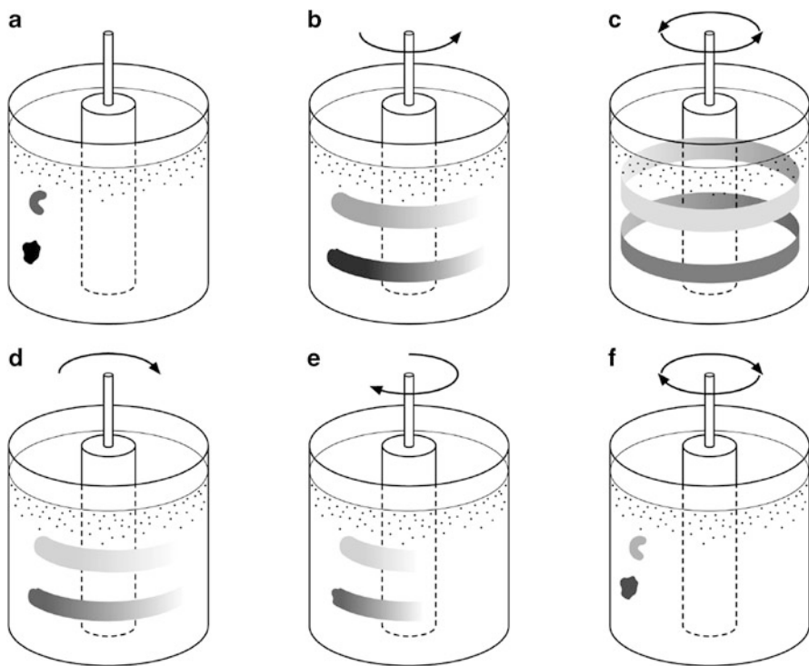
Fig. 3.6 The reversibility of Stokes flow: (a) initial dye patches, (b)–(c) spreading of the dye due to the rotation of the inner cylinder, (d)–(f) reversal of rotation causing the return to initial condition. During the motion some of the dye microscopic particles are lost to the unstained fluid due to molecular diffusion. This experiment has to be done very carefully because rapid accelerations violate the Stokes scaling
