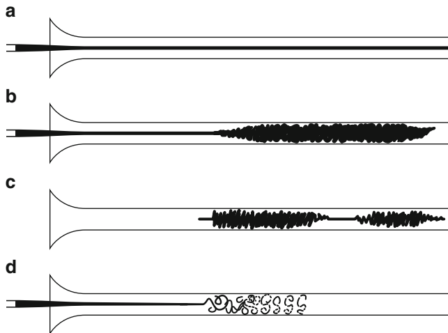
Fig. 7.2 The various types of flows, presented here schematically by the dye trace, in the Reynolds experiment. As Re is increased the flow changes from laminar (a) through transitional (b–c) to turbulent (d). Only one turbulent slug is visible in (b), while for successively higher Re values a sequence of such slugs appears, separated by laminar flow and merging finally into a fully turbulent flow along the entire pipe. The exact values of Re at the transition depend strongly on the disturbances at the entrance into the pipe (see text)
