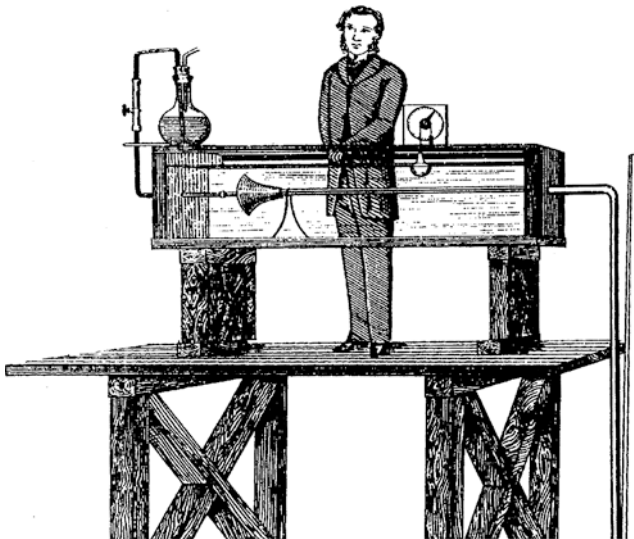
Fig. 7.1 A drawing from the original paper by O. Reynolds, describing the experimental setup
