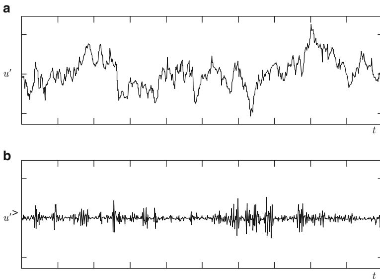
Fig. 9.12 An illustrative case of an intermittent signal in a turbulent flow, a jet in this case: (a) shows the fluctuating signal while (b) shows the high-pass filtered signal. After Y. Gagne's thesis (1980) cited in the Bibliographical Notes
