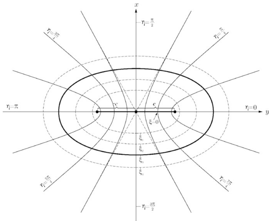
Fig. 2.8 Elliptical coordinates
