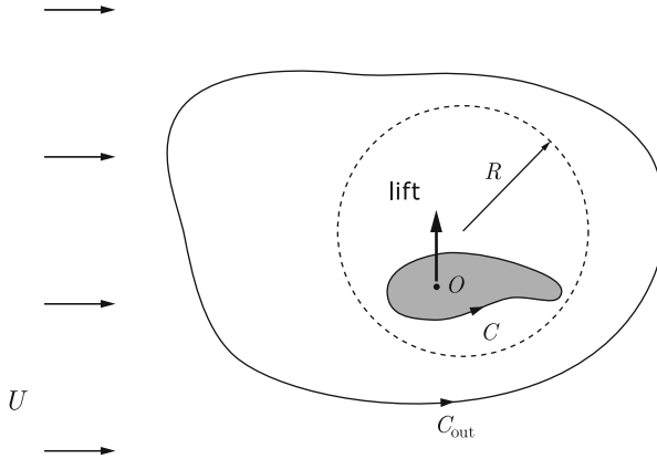
Fig. 2.5 Auxiliary sketch for the Kutta–Joukowski theorem
