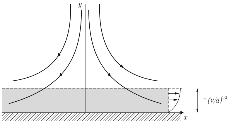
Fig. 3.4 Two-dimensional flow head on a wall, that far from the wall has the character of classic strained flow, i.e., u \rightarrow \alpha x and v \rightarrow -\alpha y as y \gg \sqrt{\nu/\alpha}
