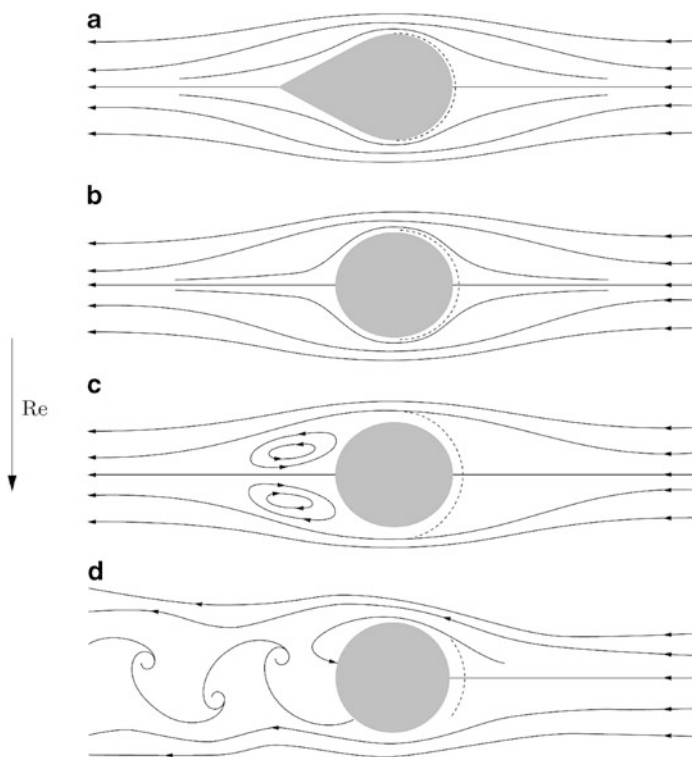
Fig. 2.2 Influence of a body on a two-dimensional flow: (a) streamlined body, (b) small wake, (c) flow reversal in laminar wake, (d) vortex street. Note that the bodies have cylindrical symmetry, in the sense that their profile is unchanged in the direction perpendicular to the page. Re increases downward
