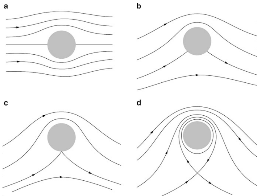
Fig. 2.4 Flow past a circular cylinder for different values of \beta representing circulation around the cylinder. For details see text: (a) \beta = 0 , (b) \beta < 2 , (c) \beta = 2 , (d) \beta > 2
