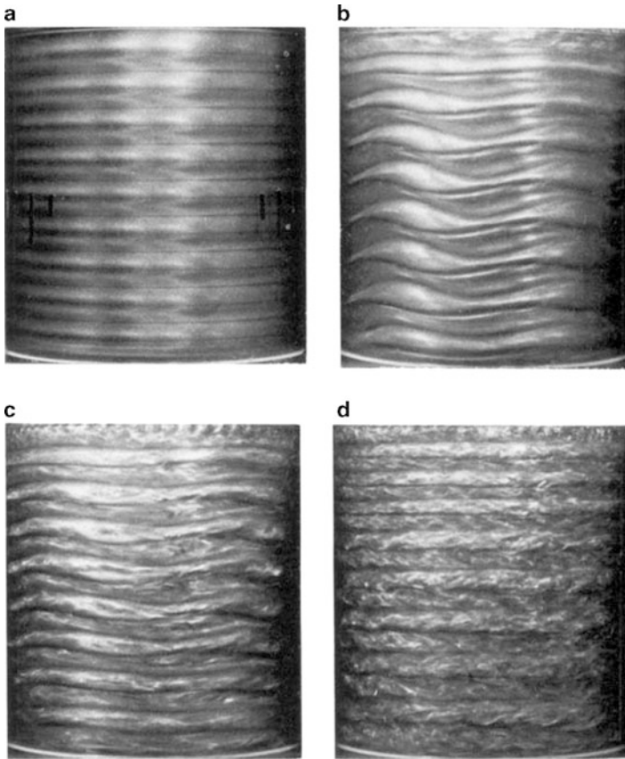
Fig. 7.3 Taylor–Couette cell; the inner cylinder is rotating, while the outer is stationary. As the rotation rate of the inner cylinder increases, the Taylor number Ta , see text, increases until vortices (a) appear, followed by wavy vortices (b)–(c), and eventually turbulence (d). Reproduced from Fenstermacher, Swinney and Gollub, J. Fluid Mechanics 94, 103, 1979 (used with permission)
