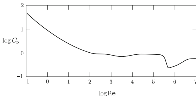
Fig. 9.4 Experimental results of the log of the drag coefficient C_D as a function of \log \text{Re} . These results are for a circular cylinder of radius d and thus a Reynolds number of \text{Re} = u_\infty d / \nu
