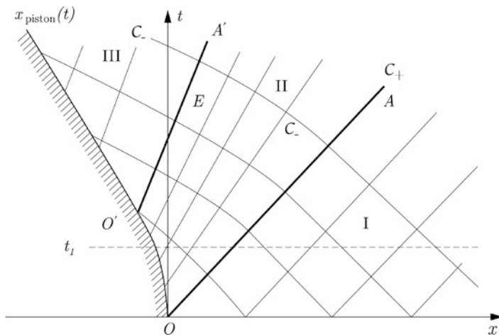
Fig. 6.8 A time-space diagram showing characteristics corresponding to a rarefaction wave. On the left there is a piston accelerating first to the left and from time t_1 continuing with constant velocity, -V . For details, see text
