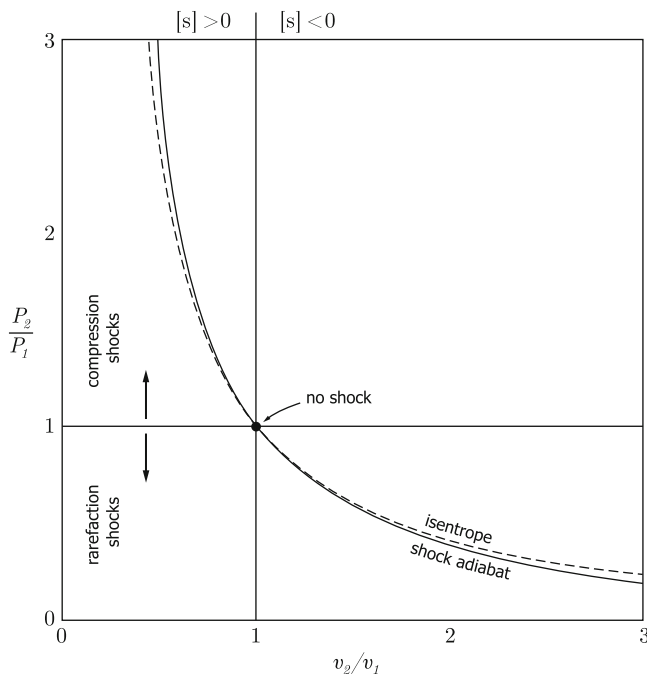
Fig. 6.15 The shock adiabat. The isentrope P \propto v^{-\gamma} is also displayed ( dashed line )
