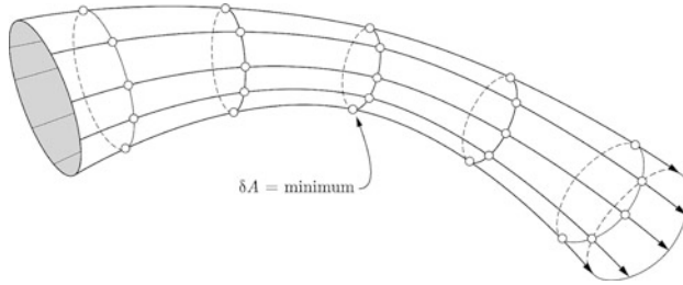
Fig. 6.3 A schematic view of a stream tube, defined by a surface composed of streamlines. A minimal cross-sectional area is indicated
