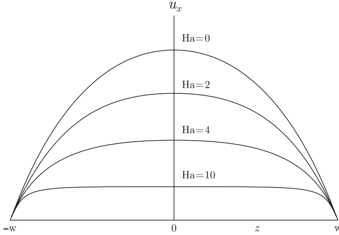
Fig. 10.2 Velocity u_x(z) profiles in Hartman flow for different values of the Hartman number for a flow in a channel of half-width w under a fixed pressure drop P_d . The maximal value of the velocity U_0 for each case can be straightforwardly expressed in terms of the pressure drop
