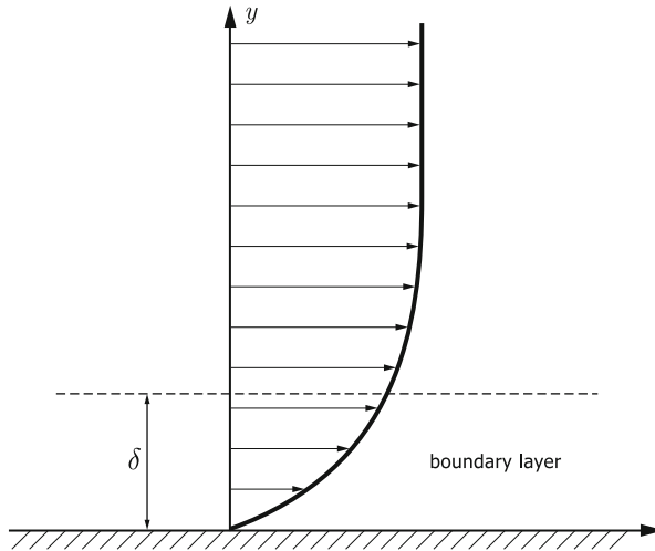
Fig. 3.9 Schematic drawing of a boundary layer forming on a plate, located at y = 0 in a flow proceeding parallel to the plate and above it. The x -axis in the figure plane direction, at the bottom, with x = 0 at the same position as y = 0 in the figure plane
