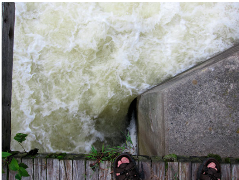
Fig. 3.10 Outflow from a New Jersey lake, after hurricane Irene, is forced to narrow by a concrete bridge support. Flow separation is clearly evident at the sharp bend and even though the flow is not laminar, the photograph illustrates well this phenomenon. (Author: Altac csi, licensed under the Creative Commons Attribution-Share Alike 3.0 Unported— http://creativecommons.org/licenses/by-sa/3.0/deed.en )
