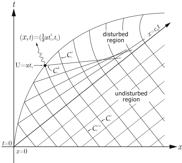
Fig. 6.12 Hydraulic jump space-time diagram. The undisturbed region is depicted for x > c_0 t . A plate with velocity U = \alpha t has a position given by x = (1/2)\alpha t^2 and the disturbed region is found between the two lines shown. All positive characteristics in disturbed region are straight lines following the same arguments of the dam break problem uniqueness
