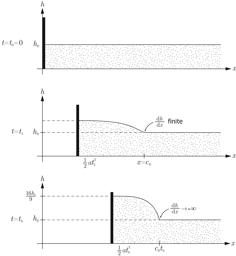
Fig. 6.10 Hydraulic jump schematic figure. For t < 0 the configuration is static with fluid at a level height h_0 . At t = 0 the vertical plate begins to move with the velocity U = \alpha t causing the fluid in front of it to pile up. The moment at which the hydraulic jump occurs is indicated as the first instant the negative gradient of the fluid height becomes infinite. This time occurs at t = t_b = 2c_0/3\alpha as given in the text. The height of the layer at the plate at this instant is 16h_0/9
