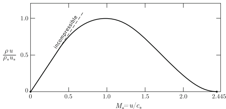
Fig. 6.4 Normalized mass flux density as a function of M_* for a perfect gas with adiabatic exponent \gamma = 1.4
