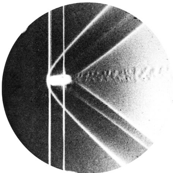
Fig. 6.2 A photograph, using a special (so-called Schlieren or stereoscopy) technique of a bullet, taken by Mach himself in 1888, demonstrating very well the cause of the double boom. [Public Domain (more than 70 years of copyright have expired). Courtesy of Ernst Mach]
