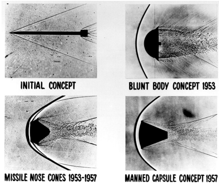
Fig. 6.16 Four shadowgraph images represent early re-entry vehicle concepts. A shadowgraph is a process that makes visible the disturbances that occur in a fluid flow at high velocity, in which light passing through a flowing fluid is refracted by the density gradients in the fluid resulting in bright and dark areas on a screen placed behind the fluid. A blunt body produces a shockwave in front of the vehicle that actually shields the vehicle from excessive heating. It was used in the Mercury, Gemini, and Apollo projects. (Public Domain. Author: NASA/Ames research center. Courtesy of NASA via Wikimedia commons— http://eol.jsc.nasa.gov/Info/use.htm )
