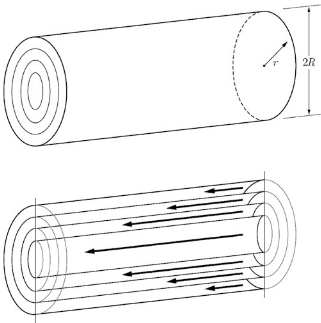
Fig. 3.1 A schematic depiction of pipe Poiseuille flow. For details see text
