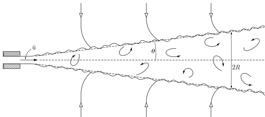
Fig. 9.2 A submerged jet emanating from a very thin (of size \sim d \ll R , for R in any region of interest) opening; for details, see text
