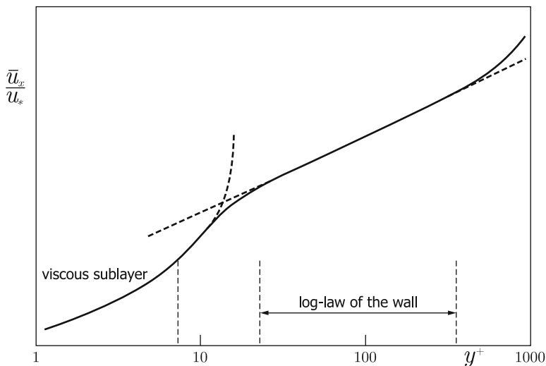
Fig. 9.1 A plot of the averaged horizontal velocity in the channel \bar{u}_x in units of u_* as a function of the nondimensional coordinate y^+ (\equiv yu_*/\nu) . The log-law of the wall and the region of its validity is clearly apparent
