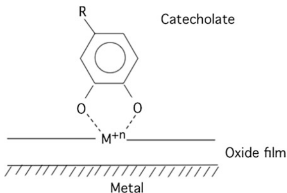
Fig. 1.29 A surface chelate formed between a catecholate and the oxide film on a metal
