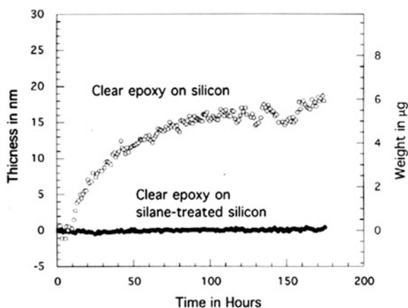
Fig. 2.3 Thickness and amount of water at the coating/substrate interface for clear epoxy coatings on silicon and silane-treated silicon. The epoxy coating thickness was 130–140 nm. Redrawn from Nguyen et al. [3] with the permission of Elsevier
