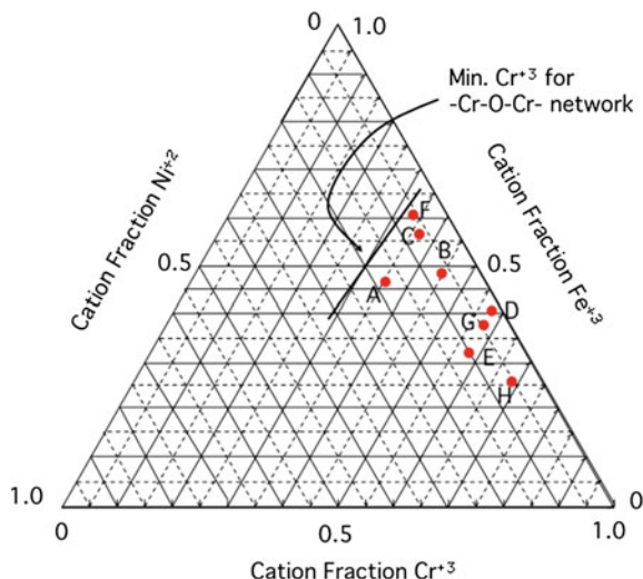
Fig. 3.7 Comparison of calculated and experimental compositions of oxide films on Fe-Cr-Ni alloys [8]. Reproduced by permission of ECS—The Electrochemical Society
