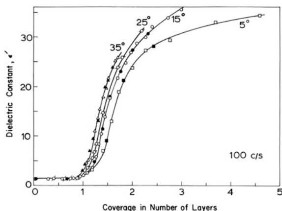
Fig. 5.3 Dielectric constant at 100 c/s as a function of coverage for various temperatures. ( Solid points indicate desorption). Reproduced from Ref. [2] with permission of the Royal Society of Chemistry
