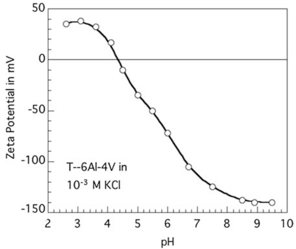
Fig. 1.4 The pH dependence of the zeta potential for the air formed oxide film on T-6Al-4V. Redrawn from Ref. [13] with the permission of Elsevier
