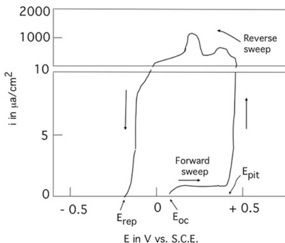
Fig. 1.31 Schematic representation of an anodic polarization curve marking the initiation of pits at the pitting potential E_{\text{pit}} and pit repassivation at the potential E_{\text{rep}} . E_{\text{oc}} refers to the open circuit (corrosion) potential. Redrawn from Fujioka et al. [117] by permission of Elsevier
