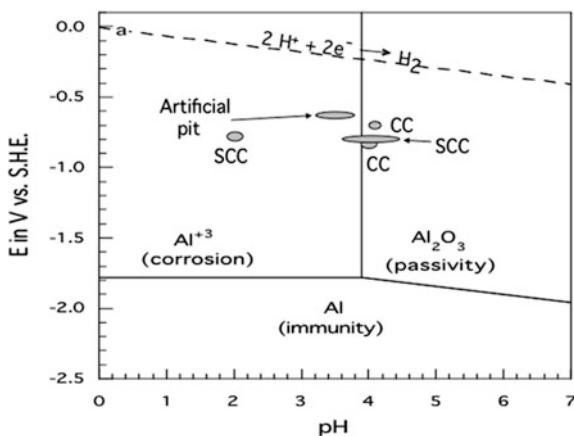
Fig. 4.5 The electrode potential and pH within localized corrosion cells on aluminum superimposed on a Pourbaix diagram for aluminum. CC refers to crevice corrosion [12, 13], and SCC to stress-corrosion cracking [14, 15]. The results for an artificial pit on aluminum are due to Hagyard and Santhipillai [16]
