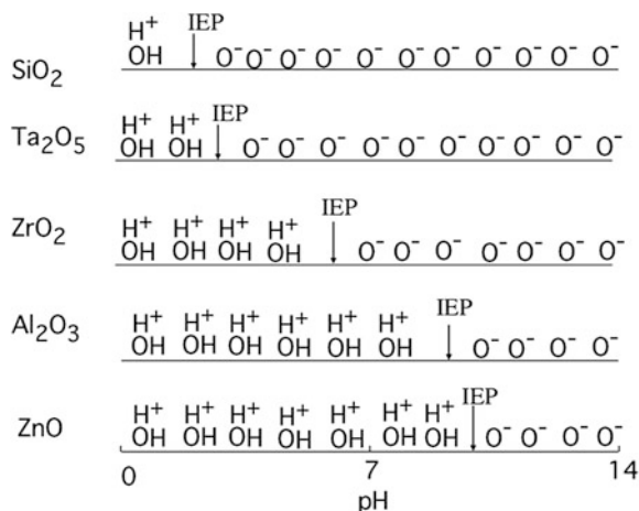
Fig. 1.15 Surface charge character of several oxide films. “IEP” refers to the isoelectric point of the oxide film
