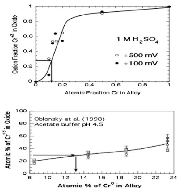
Fig. 3.4 \text{Cr}^{3+} content in the passive film on Fe-Cr binary alloys as a function of the chromium content in the alloy after immersion ( top ) in 1 M \text{H}_2\text{SO}_4 [4]. Reproduced by permission of Elsevier. ( Bottom ) After immersion in an acetate buffer [5]. Reproduced by permission of ECS—The Electrochemical Society
