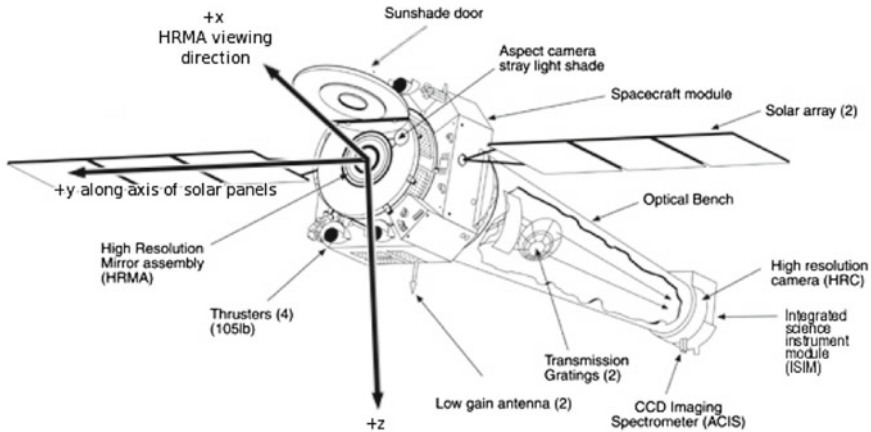
Fig. 1.7 Diagram of the Chandra X-ray observatory showing the location of the CCD Imaging Spectrometer (ACIS). This figure is from the Chandra website (Credit: NASA/CXC/NGST)
