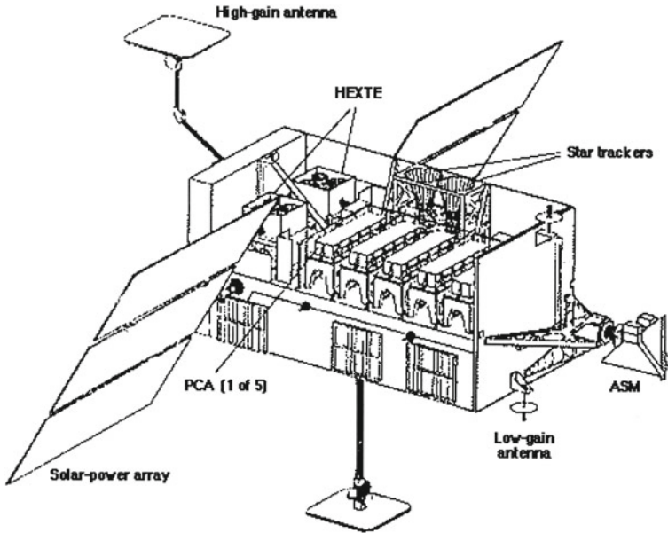
Fig. 1.8 Diagram of the Rossi X-ray Timing Explorer , showing the location of the main instruments. This figure is from the HEASARC website (Credit: NASA)
