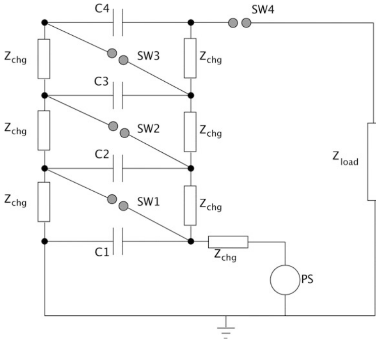
Fig. 4.10 Simplified Marx generator circuit
