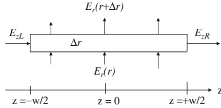
Fig. 6.9 Pillbox used to apply constraint of no net charge flow out of each \Delta r layer of the core
