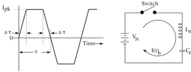
Fig. 4.4 Bipolar pulse train with finite rise and fall times and electrical circuit that generates sinusoidal currents
