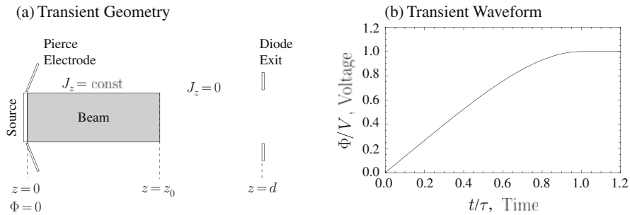
Fig. 9.3 Geometry for transient beam-head calculation (a) and the required voltage waveform for an ideal, sharp beam-head (b)
