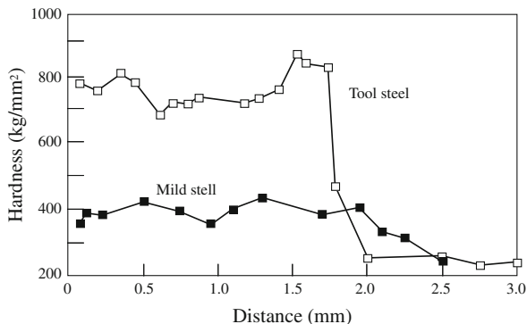
Fig. 8.11 Microhardness comparison of transformation tool steel and mild steel after the steel was bombarded by 6 MeV, 1.25 kA beam operating at 500 kHz. The surface fluence was \sim 20\text{ J/mm}^2 (reproduced from [43] with permission)
