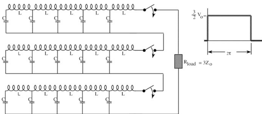
Fig. 4.7 Series connected PFNs
