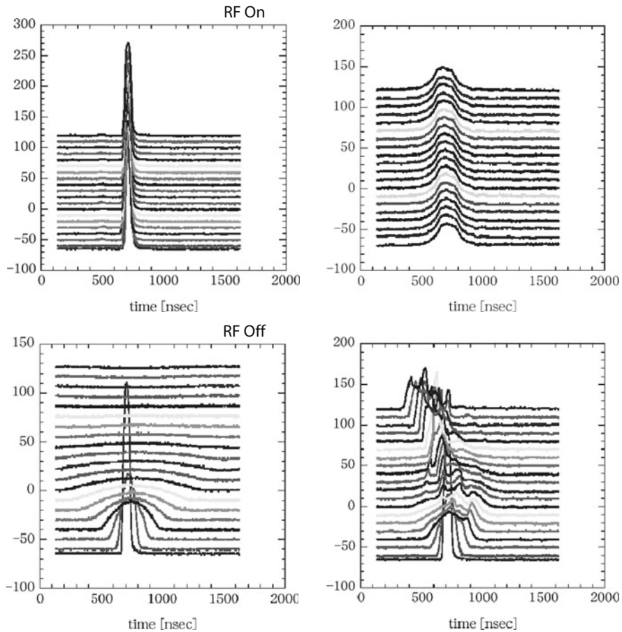
Fig. 11.25 Mountain views of the injected pulse in time. Lower left: RF off and just debunching of the injected pulse every 50 turns. Upper left: RF on and just RF trapping at 150 ms after injection every 50 turns. Lower right: Barrier voltage on and barrier trapping of the injected pulse just after injection every 50 turns. Upper right: barrier trapping at 150 ms after injection every 50 turns
