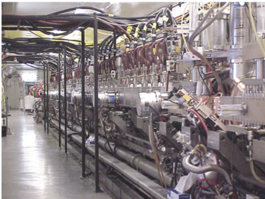
Fig. 7.3 The ETA-II accelerator at LLNL is shown above with the injector in the foreground. This accelerator consists of a 1 MeV injector with 9 induction cells followed by six 10-cell blocks. The machine produces a 5.3 MeV, 2 kA beam with a 50 ns pulsewidth and runs at 1 Hz. It has also operated at 2 kHz in burst mode as discussed in Chap. 2
