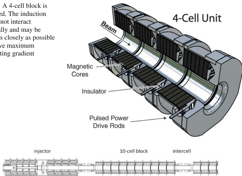
Fig. 7.2 Layouts of the ETA-II accelerator at LLNL is shown above. The machine consists of an injector with 9 induction cells and six 10-cell blocks
