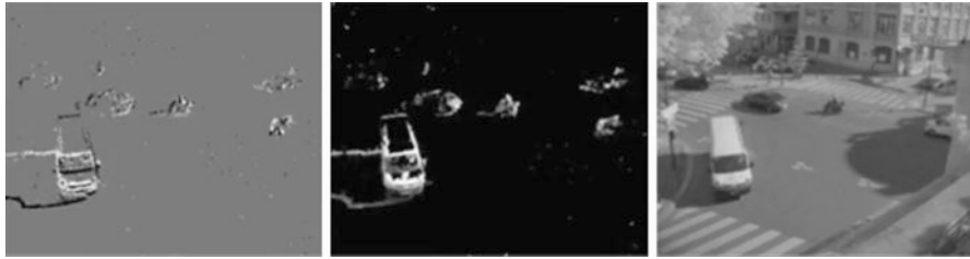
Fig. 8.3 Visual information provided by an ATIS image sensor. The ATIS image sensor provides not only the coordinates of changing pixel ( left ) but also actual light intensities at these changing pixels ( middle ). Those information enable to reconstruct the actual visual scene ( right )
