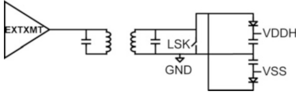
Fig. 7.4 Power and data transmission system. The transceiver block diagram shows the external transmitter and coil, secondary coil, secondary dual half-wave rectifier to establish V_{ddh} and V_{ss} , and LSK switch
