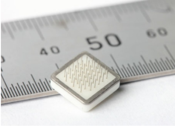
Fig. 17.3 An implant tile before Parylene coating
