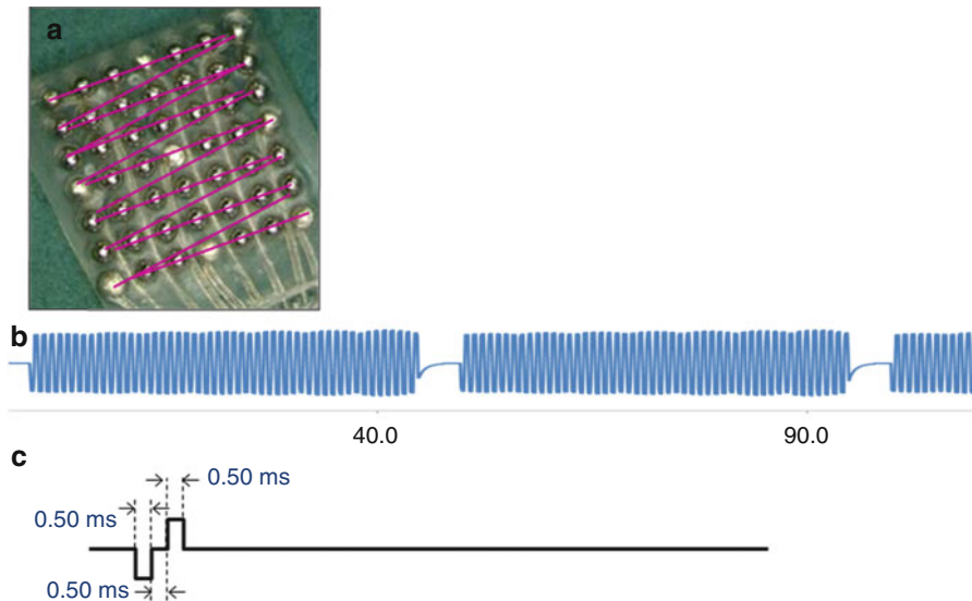
Fig. 11.6 Stimulus sequence of 49-channel electrode array. (a) Photograph of a 49-channel electrode array superimposed by bars representing the stimulus sequence. Stimulation starts from the upper left electrode and ends at the lower right electrode. (b) Representative waveforms of the stimulus artifacts derived from each of 49 electrodes sequentially at the cornea in an animal experiment. (c) Time scale of the biphasic pulse applied to each electrode
