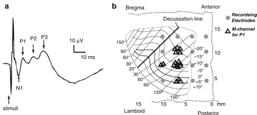
Fig. 13.3 (a) Waveform of multi-peaked EEPs, including N1, P1, P2, and P3 components. EEPs were elicited by a pair of ON-stimulating electrodes separated by 1 mm. (b) Spatial distribution of the M-channel locations ( open triangles ) of the P1 component of the EEPs superimposed on a visual field map modified from [30]. Data were obtained using a current strength of 100 \mu\text{A} with a pulse duration of 0.5 ms. Gray dots : positions of recording electrode array. The data were from 17 stimulating electrode pairs in seven rabbits. The figure represents a view of the skull/cortex from above
