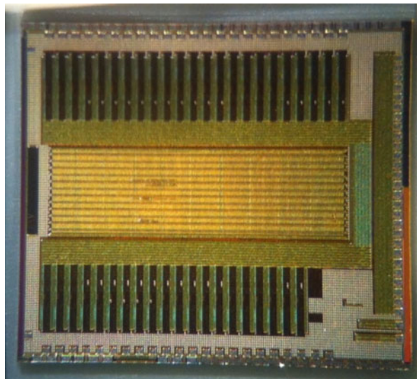
Fig. 17.2 As-fabricated mixed-signal ASIC photomicrograph
