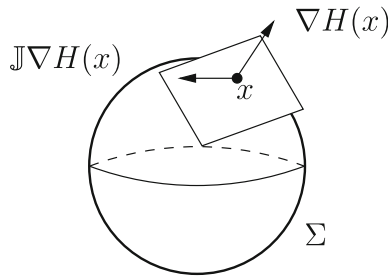
Figure 8.5.1 Gradient and Hamiltonian vector field
