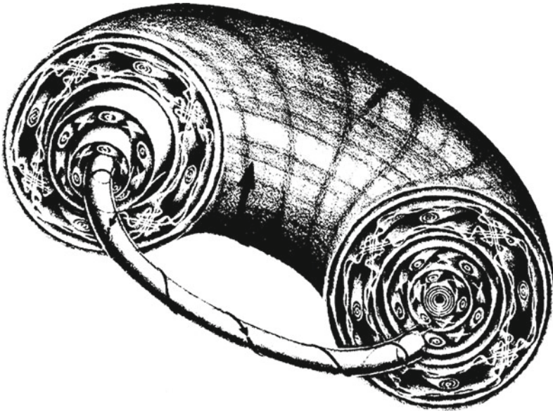
Figure 15.4.3 Phase space portrait of a Hamiltonian system with two degrees of freedom, with nested KAM tori. (Picture: RALPH ABRAHAM and JERROLD E. MARSDEN, from: Foundations of Mechanics . Addison-Wesley Publishing Company, Inc. 1982, second edition, fourth printing, Figure 8.3–3 [AM], c American Mathematical Society 2008.)
