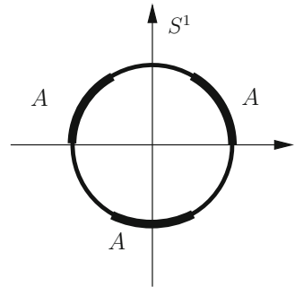
\Phi -invariant set A for \alpha = p/q with q = 3
