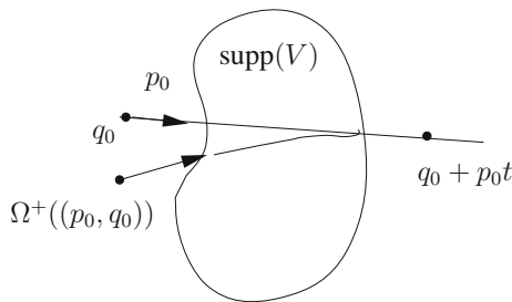
Figure 12.2.1 Definition of the Møller transformation \Omega^+ for a potential V with compact support
