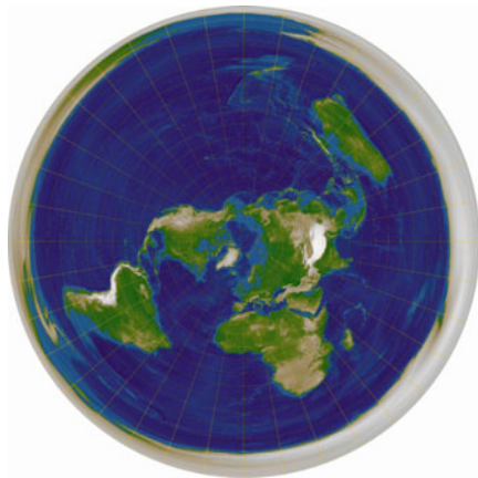
Inverse exponential map of the earth at the north pole, namely an equidistant azimuthal projection.
