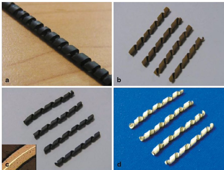
Fig. 9.8 Photographs of the samples, a graphite rod; b the deposits after burning out the graphite rod; c the deposits after sintering; d the deposits after poling
