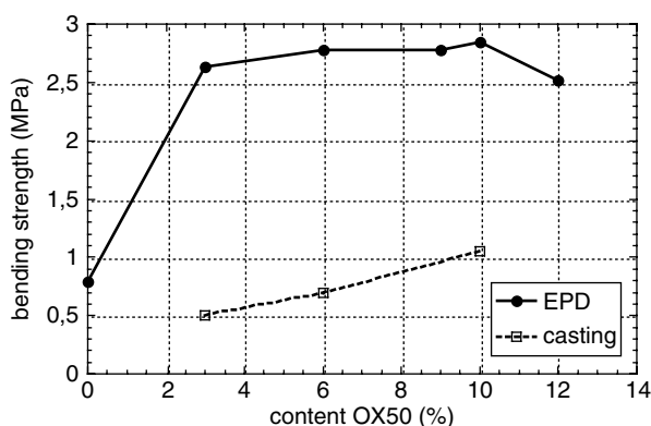
Fig. 6.17 Bending strength of compacts of mixtures of Excelica SE15 and Aerosil OX50
