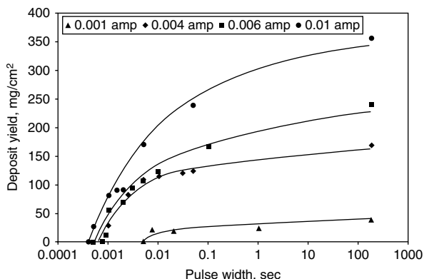
Fig. 5.8 Deposit yield as a function of pulse width during pulsed DC EPD at constant current mode (Suspension: 5 vol%, pH 4.5, Substrate: stainless steel (316 L), Pulse ON time: 3 min pulse duty cycle: 50%, Inter-electrode distance: 20 mm, pulse width of 180 s is equivalent to continuous DC EPD of 3 min). [46]
