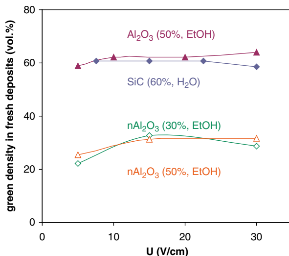
Fig. 8.17 Green density of nano-sized ( \text{nSiC} , \text{nAl}_2\text{O}_3 ) and submicron \text{Al}_2\text{O}_3 and \text{SiC} deposits as a function of applied voltage
