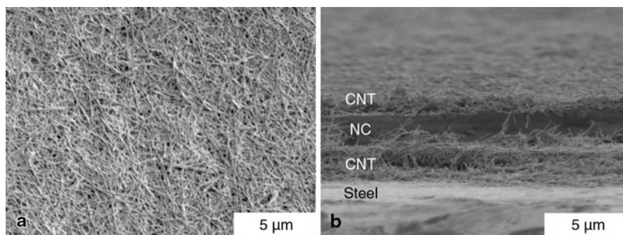
Fig. 4.5 a Top view and b side view SEM images of a composite tri-layered heterostructure: CNT mat-europium oxide nanocrystal film-CNT mat, produced by EPD. ([66] Reproduced with permission of Elsevier)
