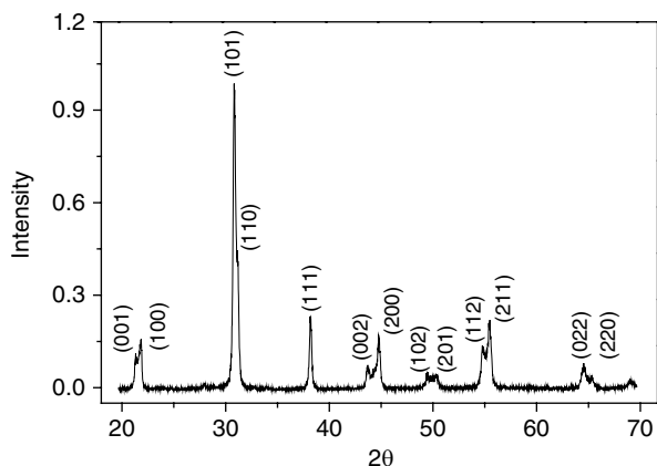
Fig. 9.9 XRD pattern of a tube sample
