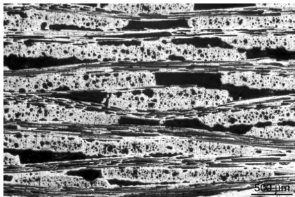
Fig. 8.8 Optical micrograph of polished cross-section of the \text{SiC}_f/\text{SiC} (CVI) composite
