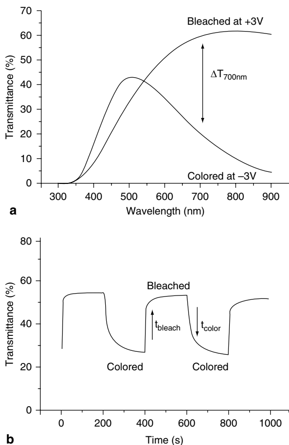
Fig. 9.27 a UV-Vis transmittance of \text{WO}_3 nanorods at bleaching (+3 V) and coloring (−3 V); b Switching study by applying a square wave signal \pm 3 V at 632.8 nm. All electrochemical studies were carried out in 1 M \text{LiClO}_4/\text{PC} electrolyte
