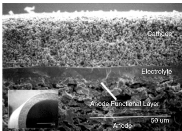
Fig. 5.11 SEM micrograph of cross-sectional fracture surface of a single cell [3]
