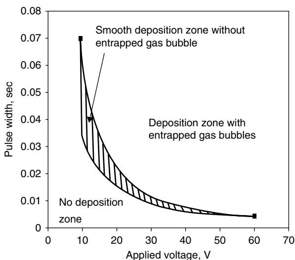
Fig. 5.9 Pulse width vs. applied potential diagram showing regions of bubble-free deposition from aqueous suspension for alumina suspension onto stainless steel (316 L) (powder concentration: 5.0 vol%, pH. 4.5, pulse ON time ( T_{on} )=3 min). [45]
