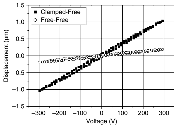
Fig. 9.13 Bending displacement in response to step voltage
