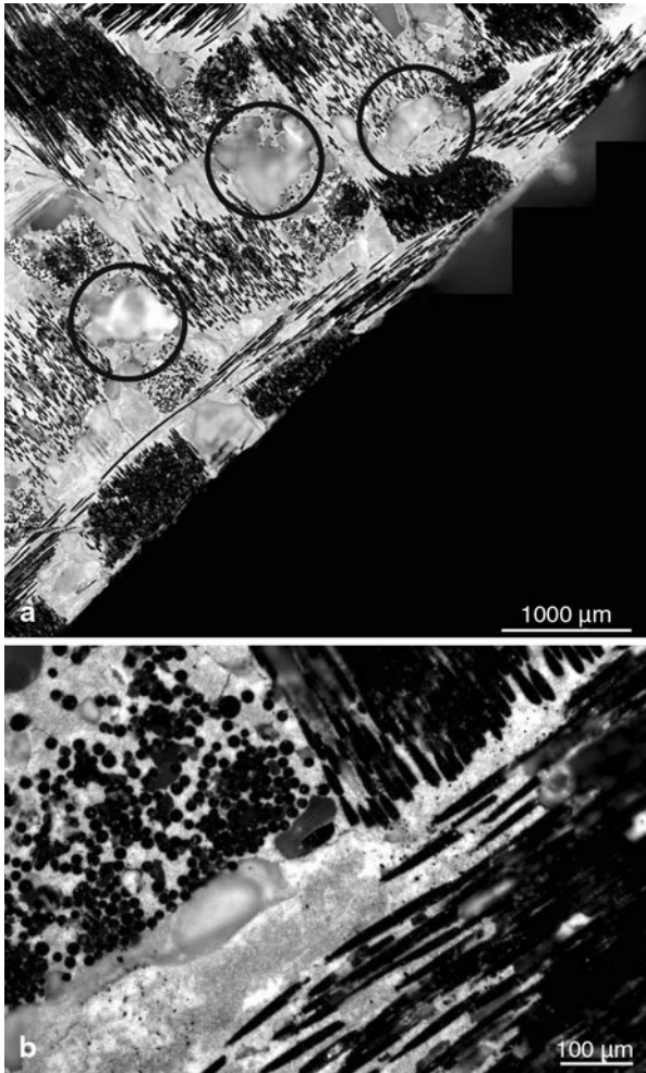
Fig. 8.37 Optical micrograph (polarised light) of polished cross-section of the 3-D SiC f /SiC composite prepared by EPI a composite picture; The circles show non-infiltrated regions and b at higher magnification showing infiltrated gaps between fibres in all directions
