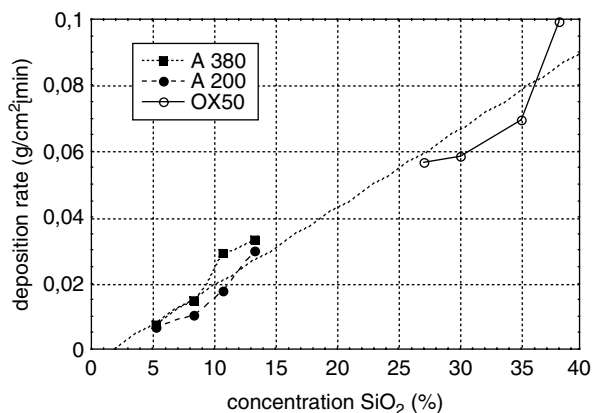
Fig. 6.13 Deposition rates of different Aerosil silica glass ( 3.75 \text{ V/cm} , 2 \cdot 10^{-2}\% TMAH/ \text{m}^2 Aerosil)
