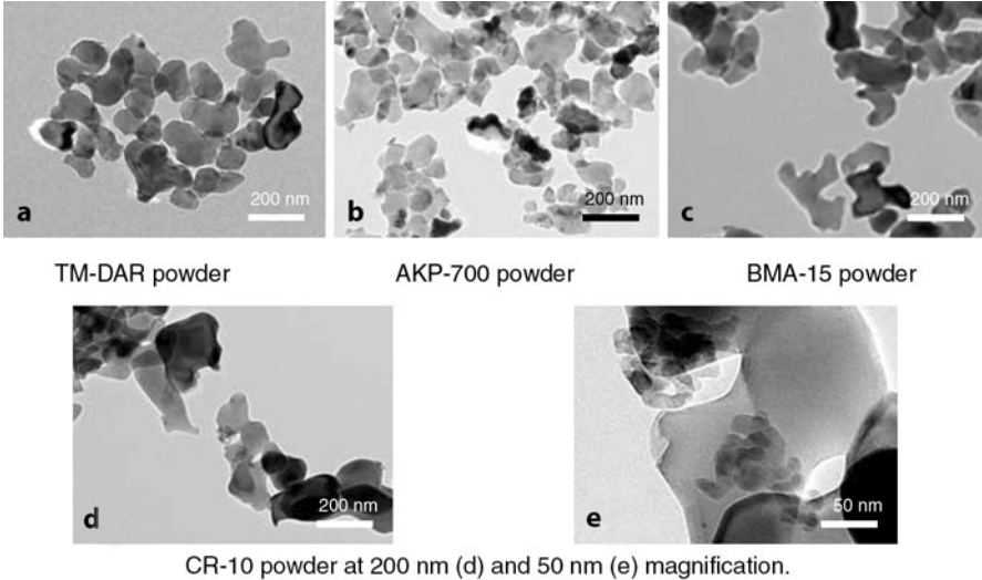
Fig. 6.28 TEM-images of submicron alumina powders used for the preparation of optoceramics. [18]
