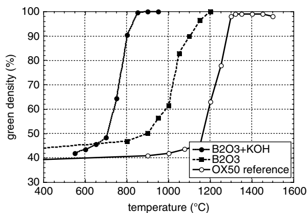
Fig. 6.24 Sintering shrinkage of pure and doped silica glass compacts. [36]
