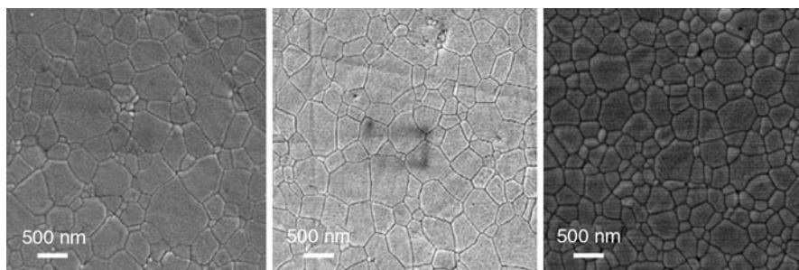
Fig. 6.31 HR-SEM images of non doped and doped samples after sintering (5 K/min) in air at 1,200°C with 48 h dwelling times. Left: undoped Al_2O_3 average grain size 890 nm, middle: Al_2O_3 with 250 ppm MgO average grain size 791 nm, right: Al_2O_3 with 250 ppm ZrO_2 average grain size 603 nm. [18]
