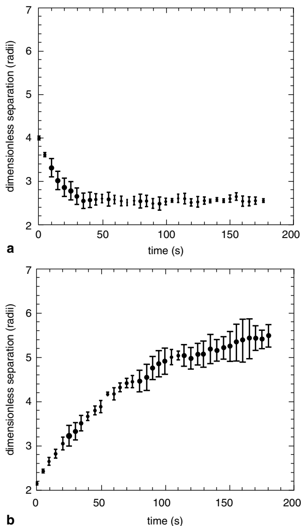
Fig. 1.11 Results from Kim et al. [30] demonstrating the effect of electrolyte in otherwise identical circumstances of ac polarization. The ordinates are dimensionless distance between two particles of a pair (normalization by radius). a Aggregation in bicarbonate. b repulsion in KOH at the same ionic strength. The frequency was 100 Hz. The critical range for comparison is dimensionless distances between 2 and 4. Particles moved somewhat faster during aggregation in bicarbonate than in KOH. Also, note the steady separation > 2 radii in bicarbonate, presumed to indicate induced dipole repulsion. (Reprinted in part with permission from Kim et al. [30], © 2002 American Chemical Society)
