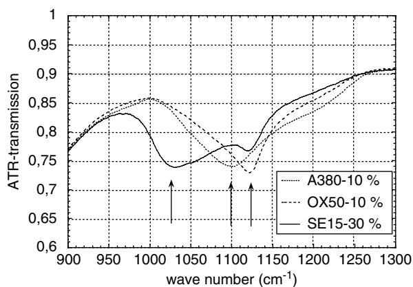
Fig. 6.6 ATR spectra of silica suspensions different particles sizes
