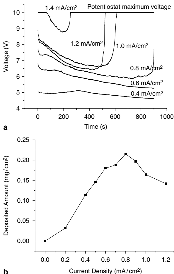
Fig. 9.25 a Constant current EPD of 10 \text{mg}/\text{cm}^3 \text{WO}_3 nanorods suspension for 900 s deposition, b Deposited amount of \text{WO}_3 nanorods on ITO glass for 900 s deposition duration at various current densities
