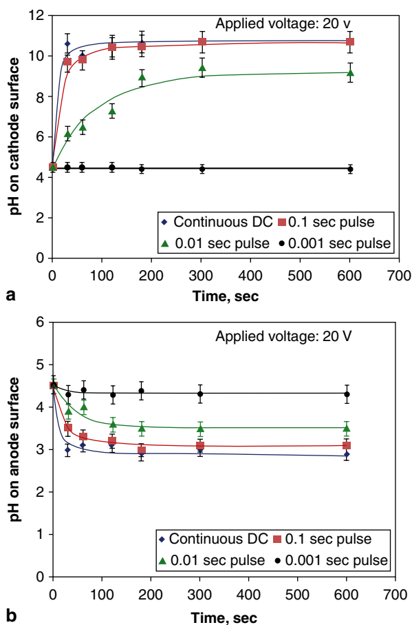
Fig. 5.3 pH localization during constant voltage electrolysis of water at a cathode/solution interface, and b anode/solution interface (initial bulk pH 4.5, conductivity = 110 \mu\text{S}/\text{cm} ; applied voltage = 20 V). [14]
