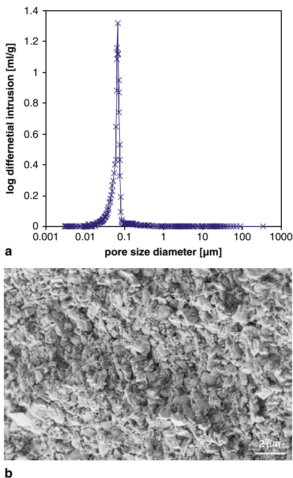
Fig. 8.20 a Pore size distribution of SiC deposit determined by high-pressure Hg-intrusion porosimetry; b SEM micrograph of fracture surface of the deposit
