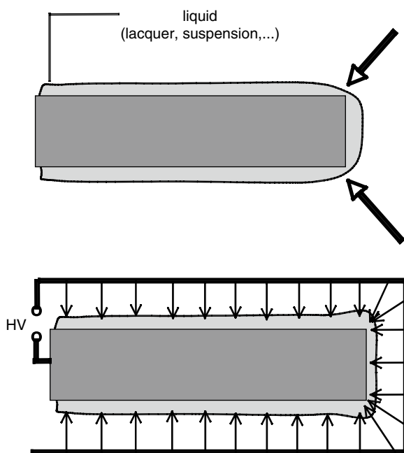
Fig. 6.51 Schematic presentation of the “sharp edge problem”
