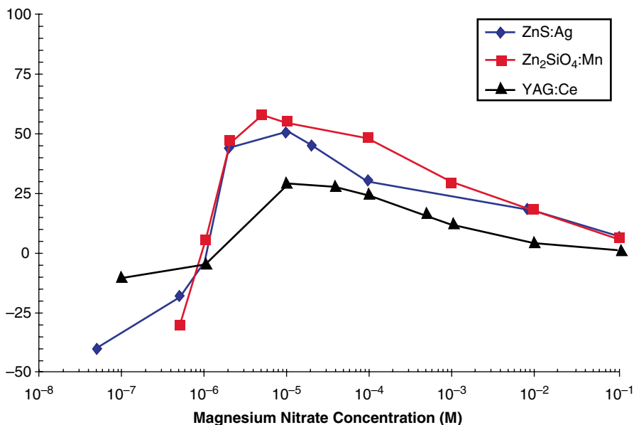
Fig. 7.1 Zeta potential of \text{ZnS:Ag} , \text{Zn}_2\text{SiO}_4\text{:Mn} , and \text{YAG:Ce} as a function of magnesium nitrate concentration in isopropanol
