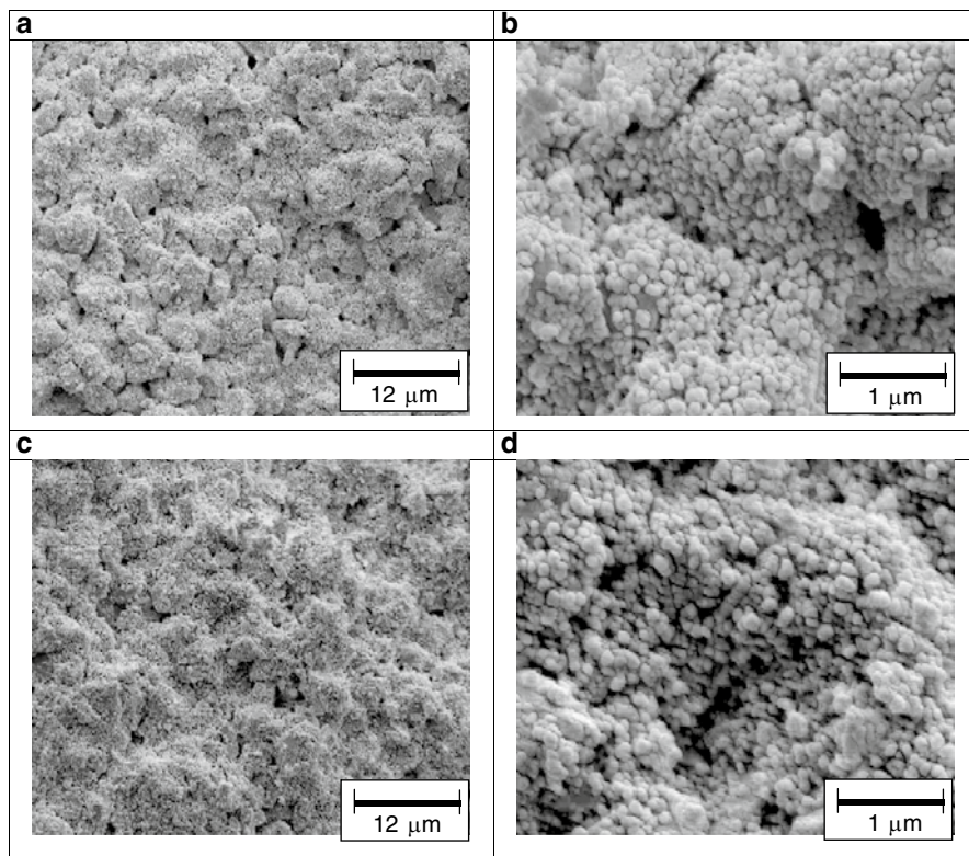
Fig. 6.40 H-REM-pictures of Ce 3.3 -TMDAR-compacts deposited with different amounts of the fine alumina powder (TMDAR). a 8 wt % fine powder, b 8 wt % fine powder, c 16 wt % fine powder, d 16 wt % fine powder. [116]
