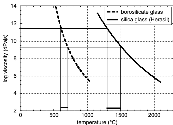
Fig. 6.25 Viscosity of borosilicate and silica glass with the sintering regime of silica (1,300...1,500°C) and borosilicate (600...700°C) nanopowders
