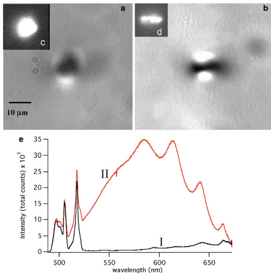
Fig. 3.12 (a and b) White light microscopy images of the end face of laser written waveguides in IOG-1. (c and d) Fluorescence images of color centers created by the fs laser. (e) PL spectra of IOG-1 (I) before and (II) after laser modification
