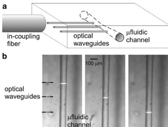
Fig. 14.5 (a) Schematic of the waveguides crossing the microfluidic channel; (b) microscope image of the microfluidic channel with the fluorescence excited by the optical waveguides, which are not visible due to the low refractive index change and scattering losses
