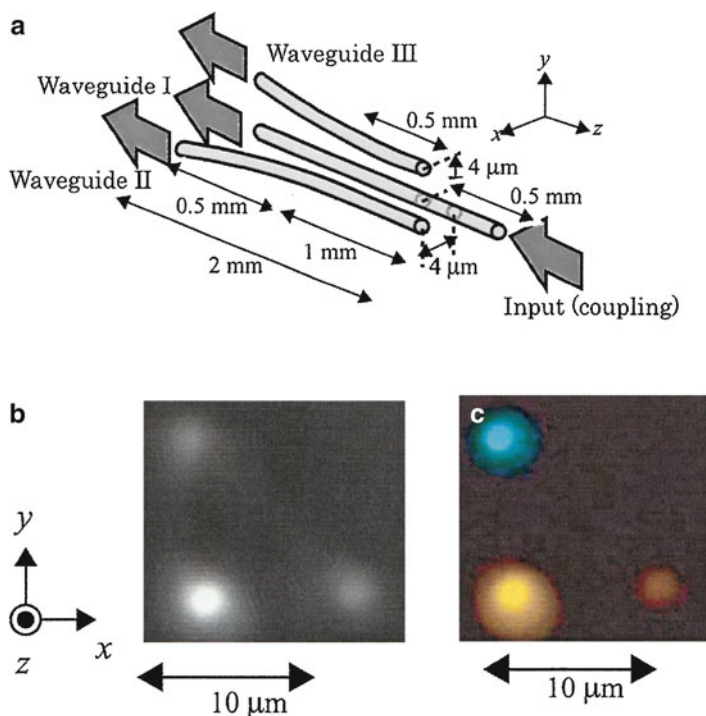
Fig. 7.17 Schematic of a three-dimensional directional coupler (a), near-field patterns of coupler output when (b) coupling to 633-nm HeNe, and (c) coupling to a broadband source (450–700 nm) showing wavelength filtering [45]
