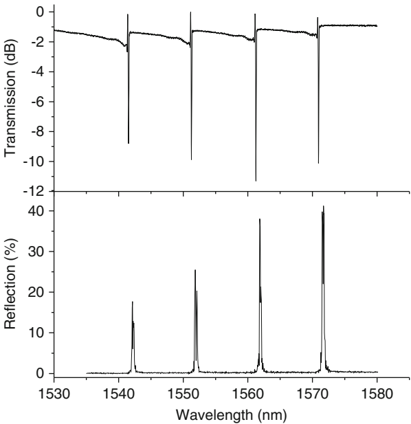
Fig. 9.19 Transmission and reflection spectral response of a serial BGW device with four different Bragg gratings inside a borosilicate glass block. The BGW was written using the kHz laser system
