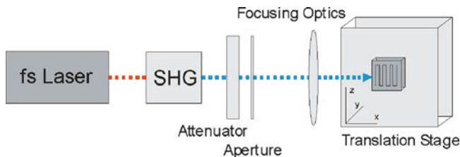
Fig. 12.1 Direct writing of a grating structure into bulk PMMA mounted on a translation stage using a frequency doubled fs laser
