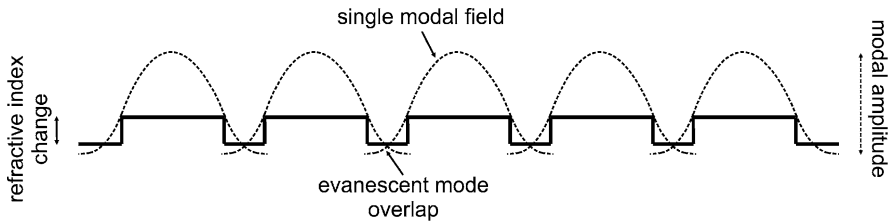
Fig. 13.1 In a waveguide array given by a periodic refractive index change, the evanescent tails of the modal fields of the individual guides overlap, which causes an energy transfer between adjacent guides
