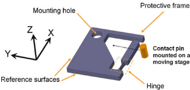
Fig. 16.11 Schematic of a test structure used to evaluate fused silica flexures. The part is cut out from a fused silica wafer. A contact pin moving along the Y -axis is used to load the hinge in bending
