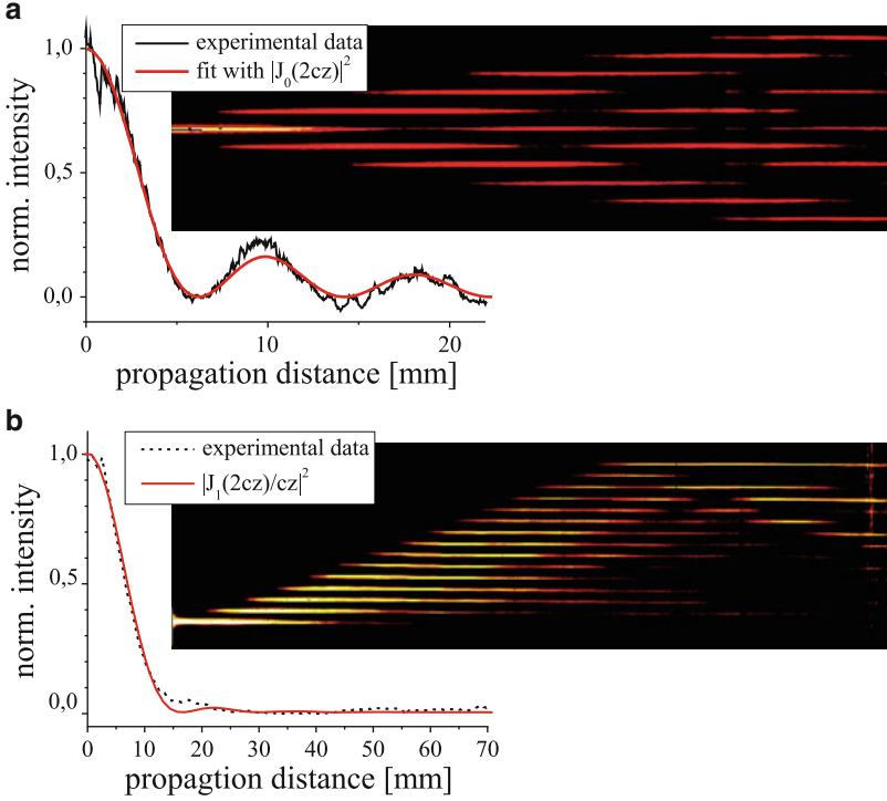
Fig. 13.7 Straight waveguide arrays excited (a) at the center and (b) at the boundary of the waveguide. Insets show measured powers of excited waveguides (black lines) and are fitted to theoretical predictions (red curves). From [47, 48]
