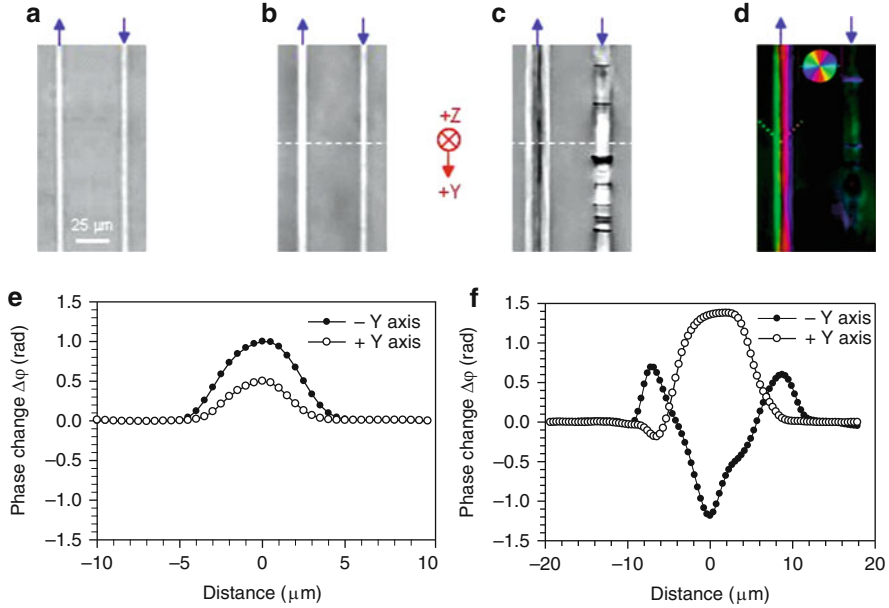
Fig. 6.10 Line structures written along the Y axis of the LiNbO 3 sample. (a–c) QPM phase images of the lines written along the –Y axis and the +Y axis of LiNbO 3 with pulse energies of: 1.2 μJ (a); 1.8 μJ (b); 2.4 μJ (c). (d) Quantitative birefringence image of the line structures. The brightness represents the retardance magnitude while the color represents the slow axis of the birefringence region. The color of the circular legend shows the direction of slow axis. The dashed lines show the slow axis of the birefringence region. Quantitative phase change profiles of the line structures written along the –Y and +Y axes at the dashed lines in b (e) and c (f), respectively. Writing directions of the structures in (a–d) are shown by arrows
