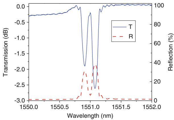
Fig. 9.8 Transmission ( solid ) and reflection ( dash ) spectral response of the borosilicate BGW written with 3- \mu J pulse energy and 100-fs pulse duration for the kHz laser system
