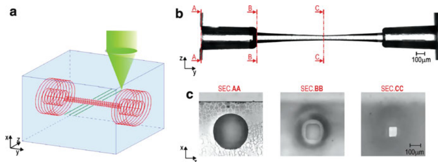
Fig. 14.18 (a) Sketch of the pre-etching path for channel formation and optical waveguides. (b) Picture of the fabricated microchannel after chemical etching. (c) Pictures of channel cross-section in different regions along the channel axis [78]
