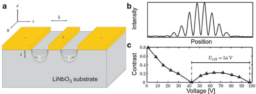
Fig. 11.8 Investigation of the nonlinear properties of type I structures in x-cut \text{LiNbO}_3 [6]. (a) Schematic of the experimental setup. Waveguides are represented by white ellipses , gold electrodes are marked yellow . (b) Interference pattern of two neighboring waveguides, recorded with a CCD line camera. (c) Fringe contrast as a function of the applied electrode voltage. The distance between the minima corresponds to a phase shift of \pm\pi/2 in both waveguides
