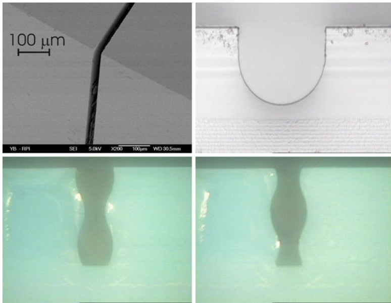
Fig. 16.9 A collection of microfluidic channels created by femtosecond laser irradiation followed by chemical etching. Top left , a deep straight channel. Top right , a channel with vertical walls and a rounded floor. Bottom left , a channel with narrowing at mid-height. Bottom right , a channel with maximum width at mid-height
