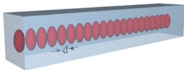
Fig. 9.1 Bragg grating waveguide composed of an array of partially overlapped refractive index voxels of period \Lambda = d . (Isolated voxels were drawn here for clarity of the concept.)
