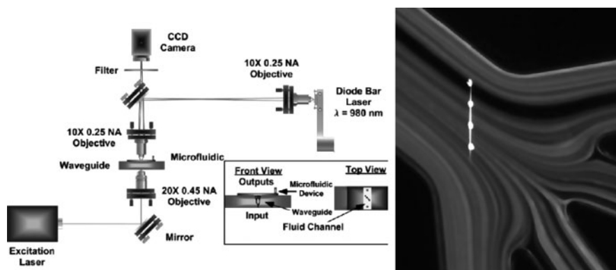
Fig. 14.6 (Left panel) Schematic of integrated FACS system based on integrated optical waveguides combined with laser trapping. The trapping laser is aligned over the waveguide outputs. (Right panel) Image of the junction in the microfluidic channel. The two outside channels are waste, while the central two channels are used for fluorescing and non-fluorescing sorted particles. The line focus of the laser diode bar and the four waveguide outputs are also shown
