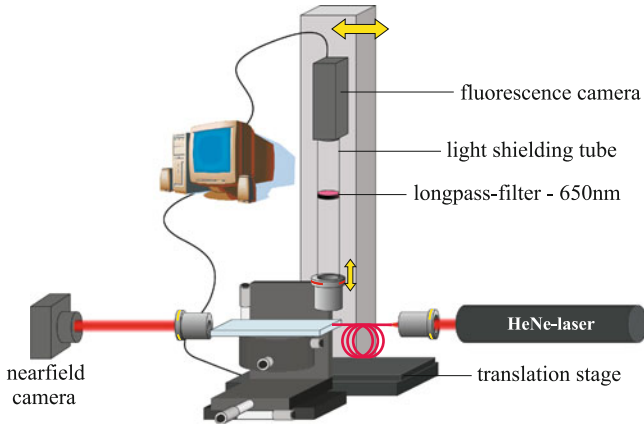
Fig. 13.4 Nearfield setup for microscope imaging of the waveguide fluorescence. The excitation source is a HeNe laser, and images from the top of the sample and of the nearfield can be recorded by CCD cameras
