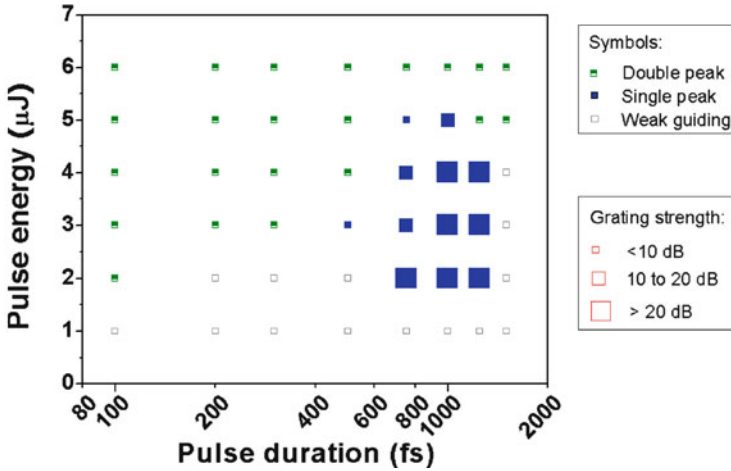
Fig. 9.6 Classification of BGWs properties as functions of laser pulse duration and energy. The devices were fabricated inside borosilicate glasses with the kHz ultrashort laser system
