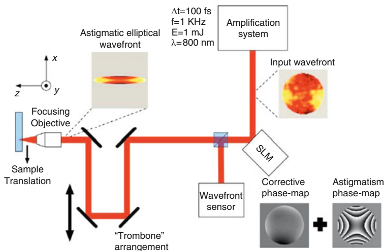
Fig. 5.16 Schematic diagram of the experimental setup used to shape waveguides using the spatial light modulator technique. (Taken from [48].)
