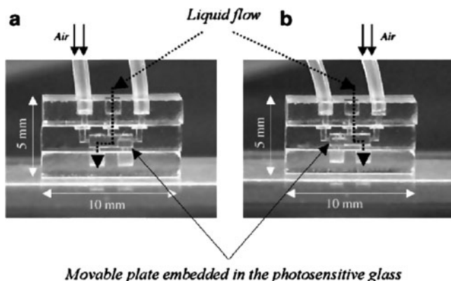
Fig. 15.9 Prototype of a microfluidic device with a freely moveable microplate that can switch the flow direction of a liquid sample. (a) By infusing compressed air from the left opening of the top part, the microplate blocks the right side. (b) If compressed air is infused from the top right opening, the microplate slides to the left
