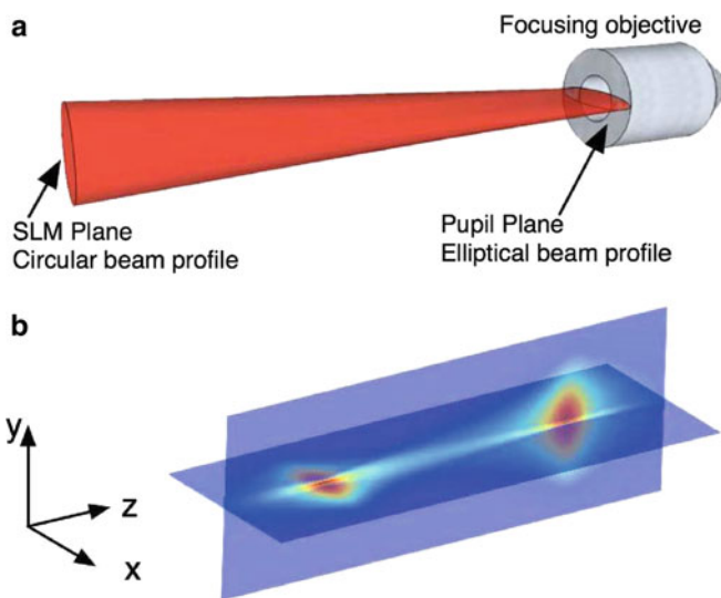
Fig. 5.17 Schematic drawing of the astigmatism and beam propagation effects on the beam profile at the entrance pupil of the focussing objective (a) and on the irradiance distribution in the focal region, showing two foci lying in orthogonal planes (b). (Taken from [48].)
