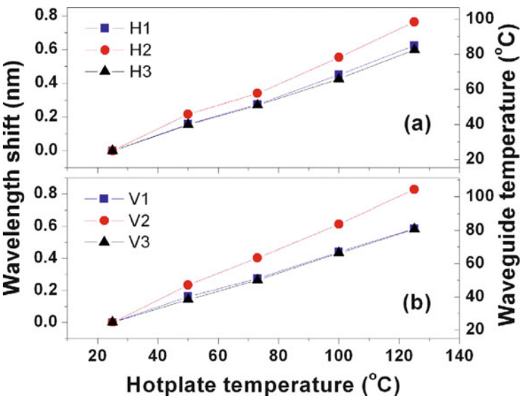
Fig. 9.27 Observed Bragg wavelength shift and the calculated local temperature of BGW segments (a) H1, H2, and H3 and (b) V1, V2, V3, in the 3D sensor network, for hotplate temperature from 25 to 125°C
