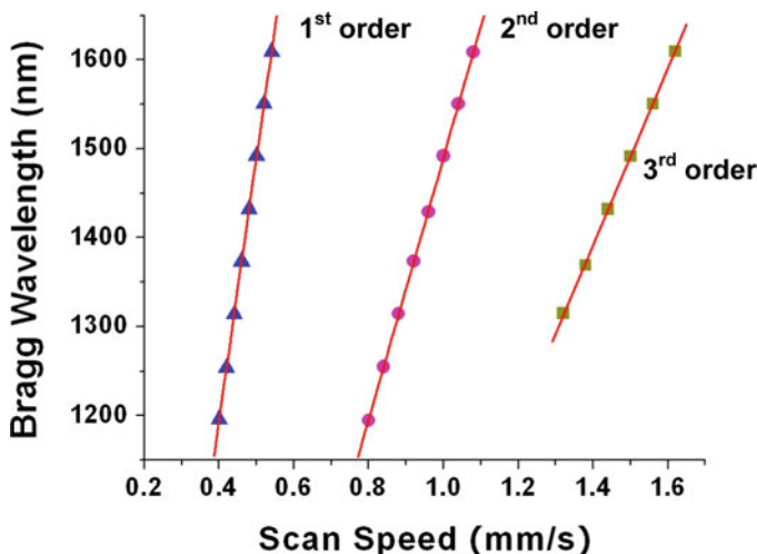
Fig. 9.18 Controllable selection of Bragg resonance wavelength versus scan velocities of the BGWs written in borosilicate glasses with the single-pulse technique, in the first, second, and third order
