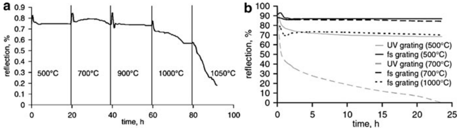
Fig. 8.6 (a) Evolution of reflectivity of a single PbP FBG after annealing at various temperatures for 20 h. (b) Evolution of grating reflectivity for a single UV-ns phase mask written and single IR-fs PbP written FBG over 25 h for various temperatures [36]
