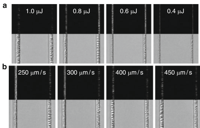
Fig. 6.2 Images in crossed polarizers ( dark part ) and Nomarski-DIC ( light part ) of the lines written in glass in opposite directions at repetition rate of 500 kHz with (a) a writing speed of 500 \mu m/s and different energies and (b) a pulse energy of 0.9 \mu J and different writing speeds
