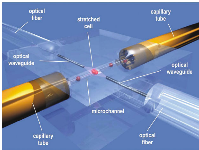
Fig. 14.17 3D rendering of the monolithic optical stretcher fabricated by femtosecond laser micromachining. The cells flowing in the microchannel are trapped and stretched in correspondence of the dual beam trap created by the optical waveguides. Connections to capillaries and optical fibers are also shown [77]
