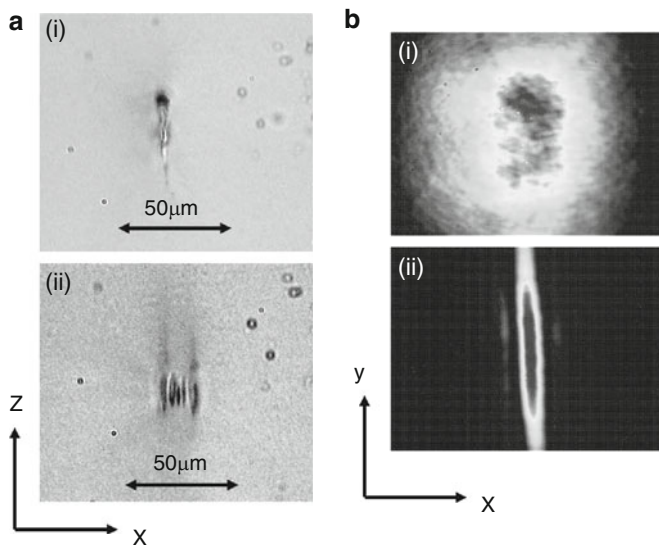
Fig. 5.15 (a) Transmission mode optical micrographs of structures inscribed using (i) a flat deformable mirror and (ii) the deformable mirror set to create a line focus in front of the microscope objective. (b) Beam profile images of the inscription laser directly before entering the microscope objective using (i) a flat deformable mirror and (ii) the deformable mirror set to create a line focus. The field of view of each image is \sim 6.5 \times 4.8 mm in the x - and y -axes, respectively. (Taken from [47].)
