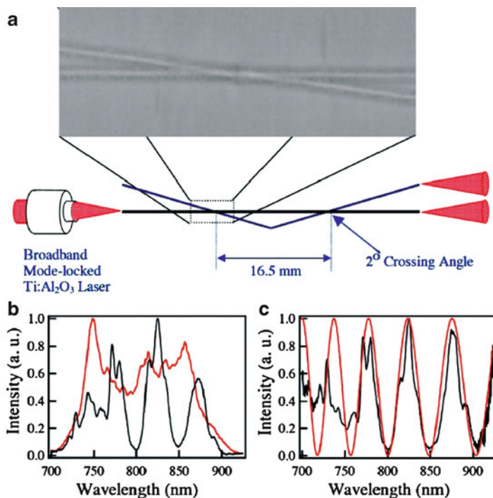
Fig. 7.28 (a) Schematic of Mach–Zehnder interferometer with phase-contrast microscope images of waveguides. (b) Input (red line) and output (black line) spectra. (c) Normalized output spectrum (black line) compared to the theoretical model (red line) [41, 46]
