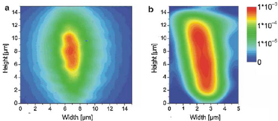
Fig. 5.7 (a) Measured near-field mode profile for 800 nm light confined by an ultrafast laser inscribed waveguide in fused silica and (b) corresponding refractive index profile recovered using the inverse Helmholtz technique. (Taken from [14].)
