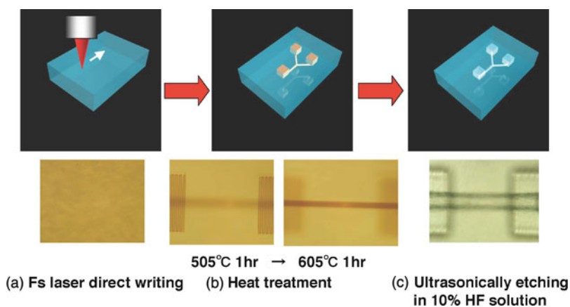
Fig. 15.3 Schematic illustration of the fabrication procedure for 3D hollow microstructures inside the photosensitive glass, together with optical microscope images of the sample after each step. (a) 3D latent images are written into the photosensitive glass by fs-laser direct writing. (b) The samples are subjected to a heat treatment to develop the modified regions. (c) The samples are soaked in a solution of 10% hydrofluoric (HF) acid diluted with water in an ultrasonic bath to selectively etch the laser-exposed regions and form hollow microstructures inside the glass
