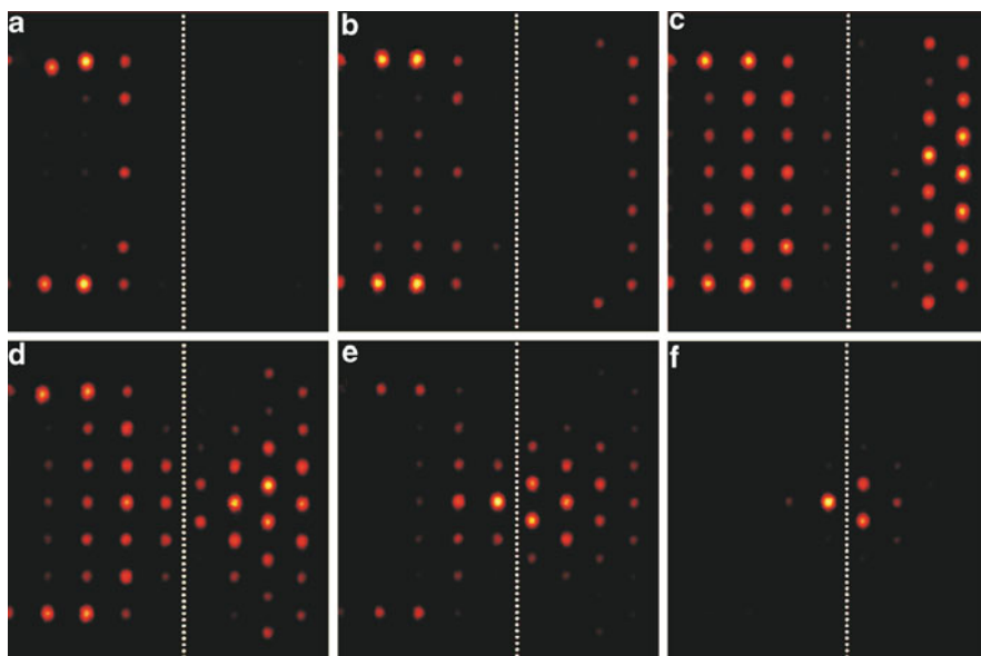
Fig. 13.35 Sequence of output patterns for light evolution in the vicinity of an interface at (a) 62 kW, (b) 1.4 MW, (c) 2 MW, (d) 2.3 MW, (e) 2.7 MW, and (f) 3.2 MW input peak power. From [80]
