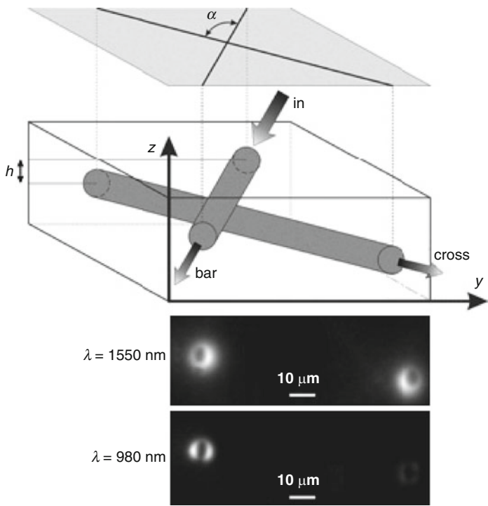
Fig. 7.21 Schematic of 1 × 2 splitter with measured near-field mode profiles of output face at 1550 and 980 nm [50]
