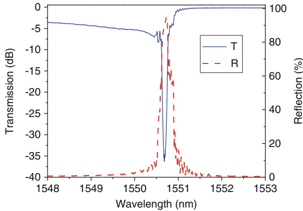
Fig. 9.7 Transmission ( solid line ) and reflection ( dashed line ) spectral response of the borosilicate BGW written with 3- \mu J pulse energy and 1-ps pulse duration for the kHz laser system
