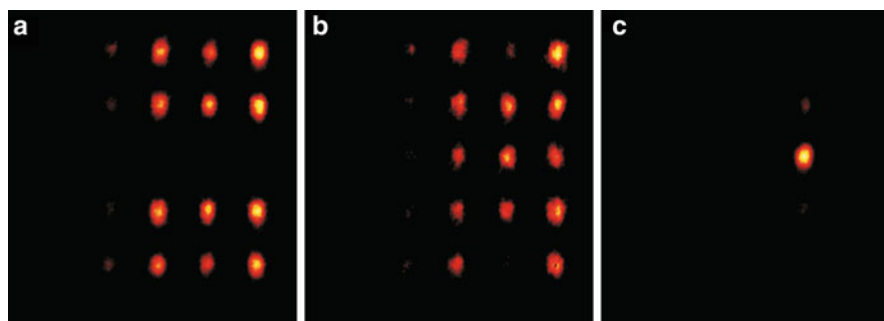
Fig. 13.32 Measured array output intensity patterns as a function of the input peak power. (a) shows the linear output pattern measured at P_{\text{peak}} = 40 \text{ kW} , (b) the measurement at P_{\text{peak}} = 700 \text{ kW} , and in (c) peak power is P_{\text{peak}} = 1,000 \text{ kW} . From [78]
