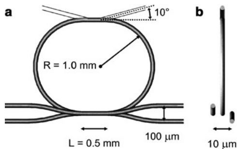
Fig. 7.31 Schematic of the 3D microring resonator. (a) Top view: the ring is fabricated in the plane of the substrate and composed of two semicircular arcs with 1-mm radii connected by 0.5-mm waveguides. (b) Side view: the waveguides are separated by 5\ \mu\text{m} with a total depth separation of 10\ \mu\text{m} [67]
