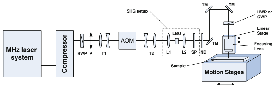
Fig. 9.10 MHz laser system and the waveguide writing arrangement. See text for definitions of symbols
