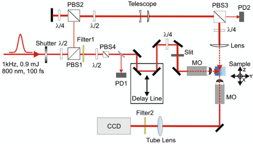
Fig. 2.9 (Taken from [50]). Femtosecond pump-probe bulk microscopy in transmission mode. The focal region of the pump beam (800 nm, 100 fs) is illuminated by a 800 nm probe beam at an angle of incidence of 90^\circ . The light transmitted by the sample is detected by a CCD camera after passing through a narrow band-pass filter (Filter 2) in order to remove the plasma emission contribution. If the probe beam is blocked and the band-pass filter removed, the signal corresponds to the time-integrated plasma emission image of the focal region. The variable slit in front of the focusing optics enables focal volume shaping
