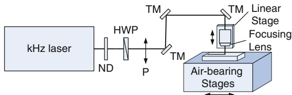
Fig. 9.3 The kHz laser system beam delivery arrangement for BGW writing. ND: neutral density filter; HWP: half-wave plate; P: linear polarizer; TM: turning mirror
