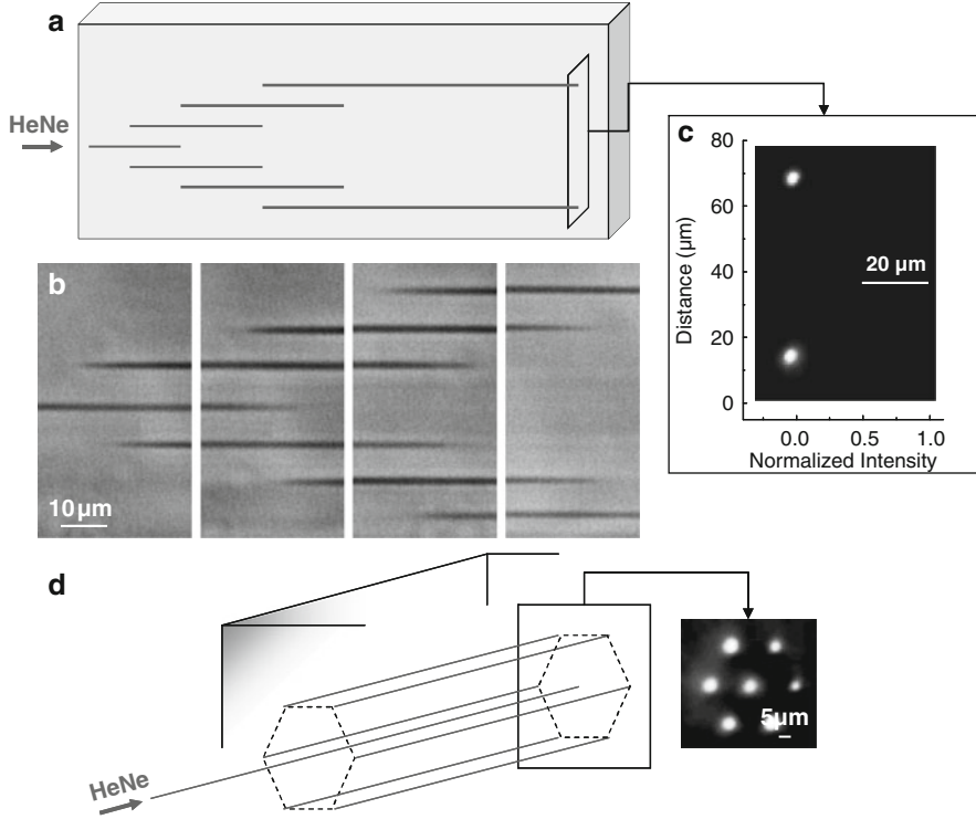
Fig. 4.9 Bulk dividers based on evanescent wave coupling in partial arrays achieved through double spot operation. The irradiation conditions are similar to Fig. 4.7. (a) Schematic view of the structure. (b) Assemblage of PCM side-pictures of the device, its total length is 8.2 mm and the lateral separation between tracks is 9 μm. The overlapping distances were determined to induce efficient evanescent coupling. (c) Near-field profile under 633 nm light injection. (d) Schematic view of a bulk photowritten 1 to 7 light divider. The length of the structure were chosen to enable evanescent coupling from the central to the external guides. Inset: Near-field profile under 633 nm injection in the central waveguide
