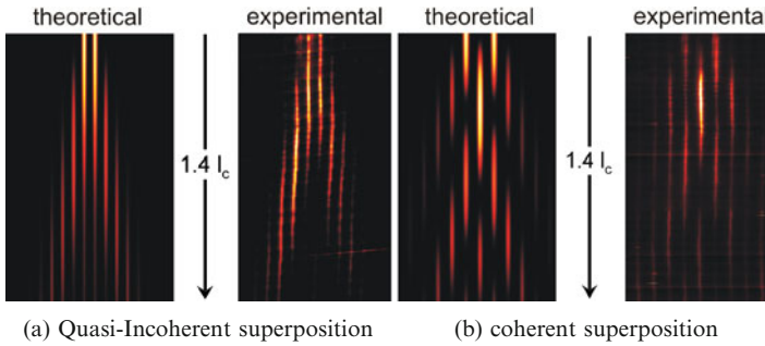
Fig. 13.10 Theoretical and experimental interference pattern in 50 mm long waveguide arrays with spacings of d = 20 \mu\text{m} for two point sources generated by a DOE. The spatial separation of the two foci was adjusted by position of the grating between the sample and microscope objective, so that (a) nearest neighbors are excited and (b) one waveguide is left for the illumination [40]
