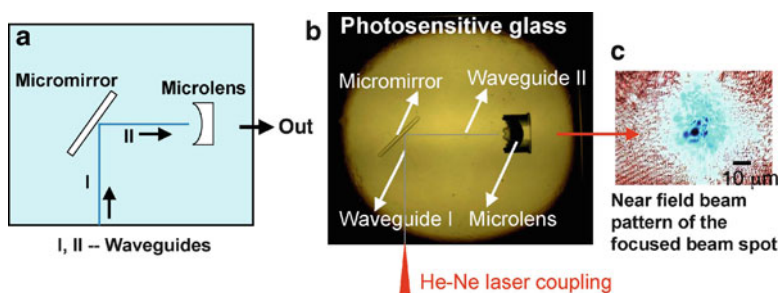
Fig. 15.12 (a) Schematic of the 3D integration of two waveguides with a micromirror and an optical plano-convex microlens in a single glass chip. (b) Optical microscope image and (c) characterization of the 3D microdevice. The solid gray lines in panel (b) mark the locations of the invisible waveguides inside the glass
