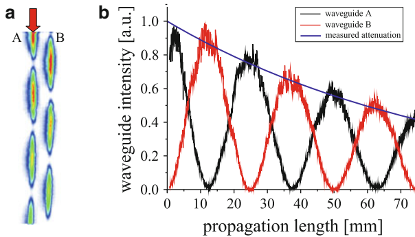
Fig. 13.5 (a) Fluorescence microscopy image of a directional coupler with d = 16 \mu\text{m} , the arrow marks the excitation of waveguide A (b) measured intensities in each waveguide A and B plotted vs. propagation length and exponentially decaying fit of the total power to determine propagation loss. The excitation wavelength is 633 nm and the waveguide spacing is 16 \mu\text{m}
