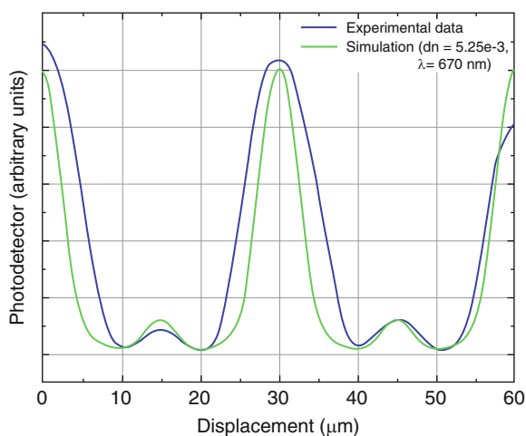
Fig. 16.25 Experimental results (blue curve) compared with simulation results (green curve). The figure shows the intensity seen for the last three waveguides (going from left to right). The lowest intensity peaks (on the right) corresponds to the last waveguide
