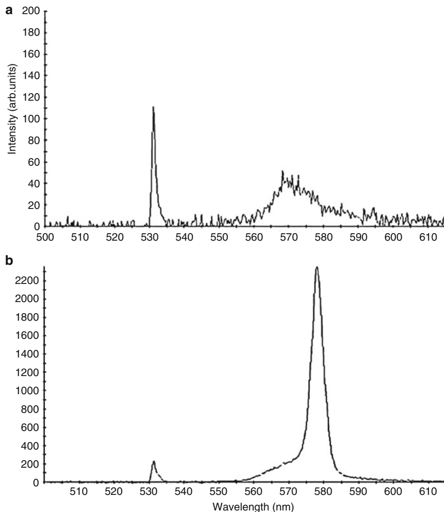
Fig. 15.14 Emission spectra of the microfluidic dye laser at pump powers of (a) 1.66 \text{ mJ cm}^{-2} and (b) 4.49 \text{ mJ cm}^{-2} . The peaks centered at 532 nm are scattered pump light
