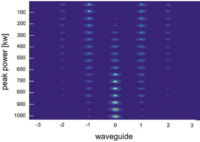
Fig. 13.27 Measured output pattern as a function of the input peak power. For low peak power, the light diffracts over several waveguides, while for high power a localization in the excited waveguide can be observed. From [74]
