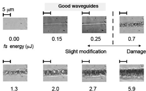
Fig. 3.6 White-light microscopy images showing the morphology of waveguides and damage lines written longitudinally inside fused silica at 40 \mu\text{m s}^{-1} using different laser pulse energies through a 50\times objective
