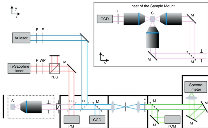
Fig. 3.5 Schematic diagram of the combined femtosecond laser writing/confocal microscope setup. The dashed lines indicate flip mounts that allow for easy removal of the optical element. F = filter, M = mirror, WP = half-wave plate, PBS = polarization beam splitter, BS = beam splitter, S = sample on stepper motor stages, PM = power meter, PCM = photon counting module
