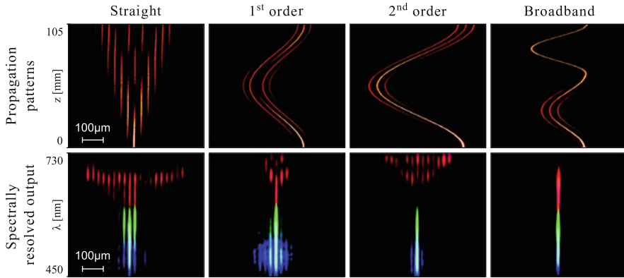
Fig. 13.17 Polychromatic self imaging in 105 mm long samples with a waveguide separation of 26 \mu\text{m} : Upper row shows propagation images and lower row the spectrally resolved output of (from left to right) straight lattice, 1st order dynamic localization, 2nd order dynamic localization, and broadband self collimation. From [60]
