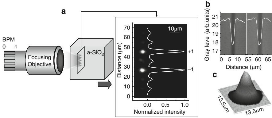
Fig. 4.7 (a) Figure of merit of double spot operation. BPM: Binary phase mask. Inset: Double spot intensity profile in the sample at the focus of the objective generated by a step phase grating. The arrow shows the motion of the sample for longitudinal photoinscription. Right: the result of double spot operation through an effective NA of 0.3. (b) PCM picture of two simultaneously photowritten waveguides through double spot operation at 800 nm, 5 \mu\text{m/s} , 10 kHz, 24 mW, superimposed with horizontal cross section of the index increase. (c) near-field profile of one of the waveguides pictured in (b) at 633 nm. Results are taken from [95]
