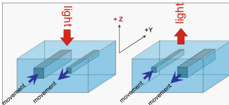
Fig. 6.9 In a non-centrosymmetric medium, modification of the material can be different when femtosecond laser beam propagates in opposite directions. Red arrow indicates light propagation direction; blue arrows show direction of sample's movement
