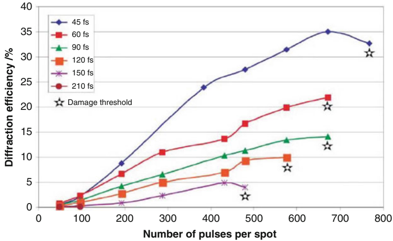
Fig. 12.8 First-order diffraction efficiency of refractive index gratings as a function of pulse duration and number of pulses per spot N_p for pulse duration between 45 and 210 fs, \Phi = 0.14 \text{ J cm}^{-2} , N_s = 2 - 32 , and wavelength of 800 nm [38]
