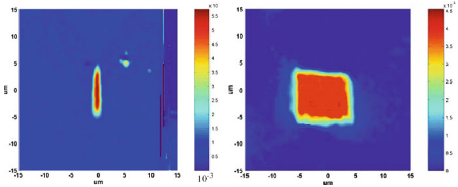
Fig. 16.4 (a, left ) Refractive index map of a single line written in a fused silica glass. The center of the line that has the highest index of refraction can be correlated with a local increase of glass density which in turn can be related with the local increase of etching rate. (b, right ) Illustration of an enlarged refractive index zone by writing multiple lines adjacent one to another [8]
