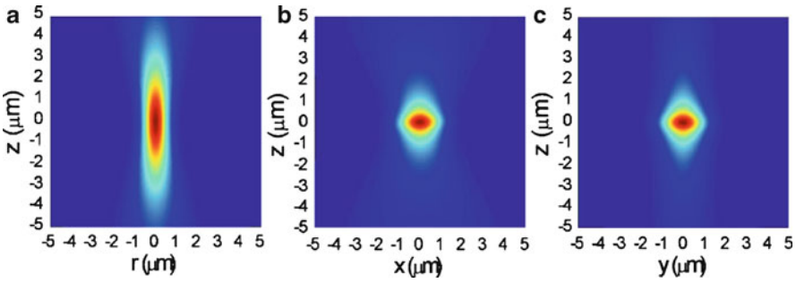
Fig. 5.19 Numerically calculated laser intensity distributions at the focus produced by an objective lens (a) without and (b and c) with temporal focussing technique in XZ and YZ planes, respectively. (Taken from [49].)
