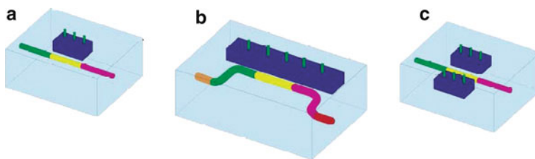
Fig. 14.16 Schematics of microfluidic sensor geometries: straight BGW single channel (a), S-bend BGW single channel (b), and straight BGW double channel (c) [66]
