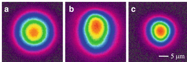
Fig. 7.12 Mode profile at 1550-nm wavelength for (a) standard SMF fiber, (b) 0.55-NA waveguide, and (c) 1.25-NA waveguide. The writing laser was incident from the top [35]
