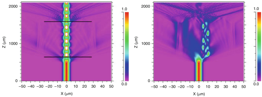
Fig. 16.22 Wave propagation in the ILE for two configurations as the array is moved from the right to the left. The horizontal line indicates the free space gaps
