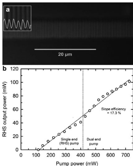
Fig. 10.9 (a) Transmission DIC micrograph of a typical first-order waveguide Bragg grating fabricated by the single-step writing process with a low repetition rate Ti:sapphire system [49]. The inset shows a section of the structure at 3\times magnification. Overlaid on the inset is a graph of the grating image intensity. (b) Output power of the DFB Yb-laser, at room temperature, as a function of pump power for single- and dual-end pump geometries using a 9.5-mm long waveguide Bragg grating. Reprinted with permission from [49,50]
