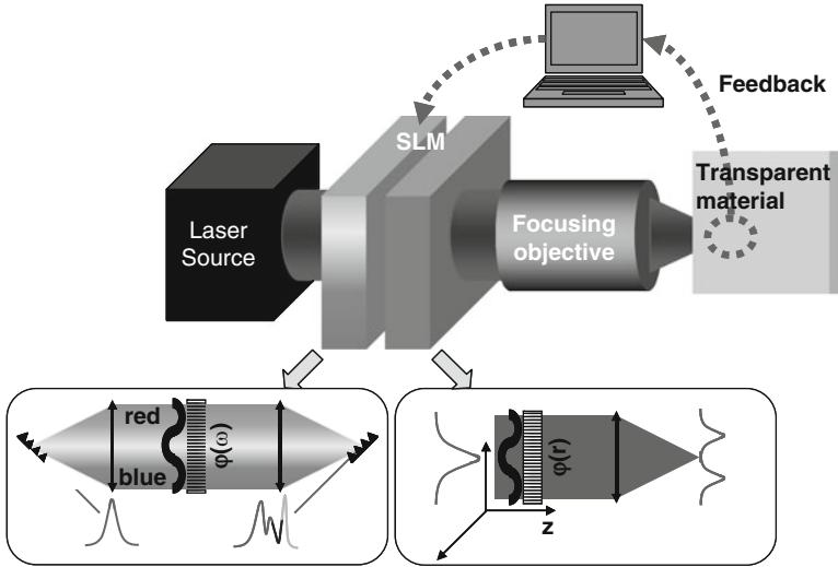
Fig. 4.2 Basic layout for spatial and temporal femtosecond pulse shaping integrated in a feedback loop. The left inset sketches the concept of temporal pulse tailoring via Fourier synthesis of frequency components. The right inset indicates the Fourier transformer for spatial beam shaping
