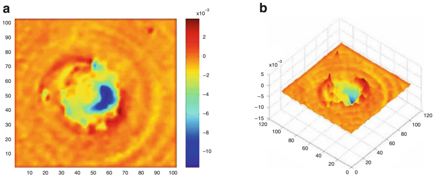
Fig. 5.6 Refractive index profile of an ultrafast laser inscribed waveguide in borosilicate glass obtained using QPM with digital holography. (Taken from [28].)
