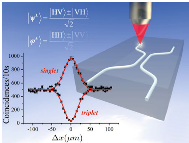
Fig. 7.20 Schematic of the femtosecond laser-written directional coupler in the bulk of a borosilicate glass. Inset shows characteristic Hong-Ou-Mandel interference for singlet and triplet polarization entangled Bell states [49]
