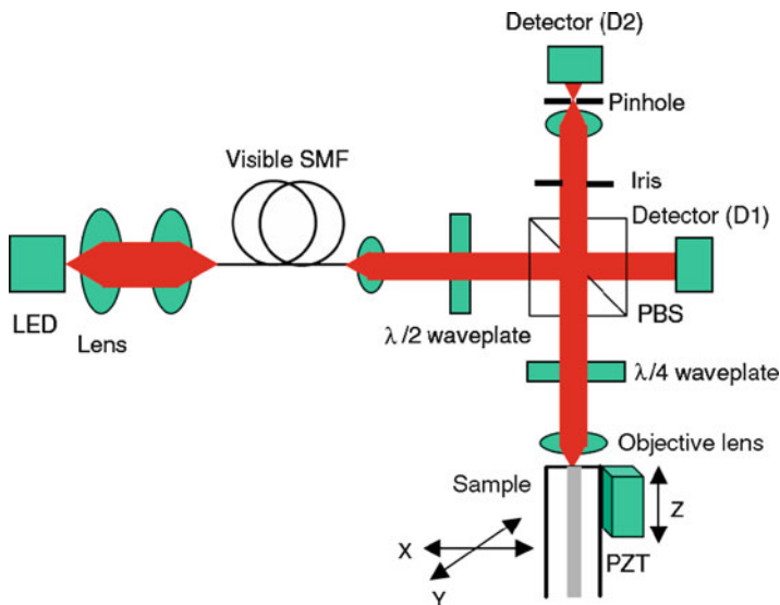
Fig. 5.4 Micro-reflectivity refractive index profiling experimental setup based on a confocal reflectance microscope. (Taken from [21].)
