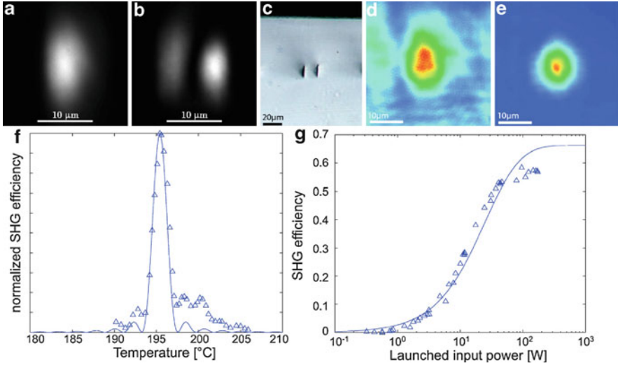
Fig. 11.10 Mode fields of a type II waveguide in \text{LiNbO}_3 [29]; (a) fundamental transverse mode at pump wavelength 1064 nm; (b) higher transverse mode at second harmonic 532 nm. Type II waveguide in PPLN [11]; (c) microscope image of end facet. Mode fields for the (d) fundamental wavelength 1064 nm, and (e) second harmonic 532 nm. (f) Thermal phase matching curve of the second harmonic output. (g) SHG efficiency as a function of the input peak power
