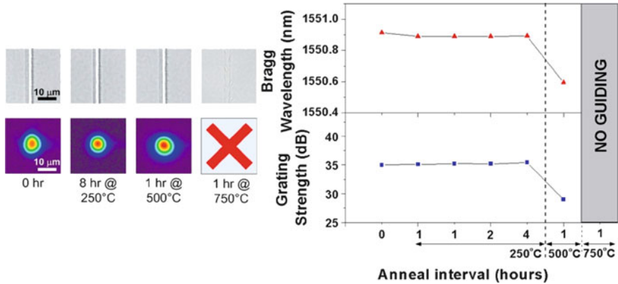
Fig. 9.16 Microscope images ( upper left corner ) and mode profiles ( lower left corner ) of the single-pulse written borosilicate glass BGW together with ( right ) plots of Bragg wavelength shift and transmission grating strength under various heat cycles
