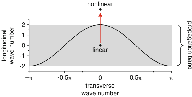
Fig. 13.24 With increasing input power, the propagation constant of the excited waveguide is shifted into the band gap, forming an isolated state
