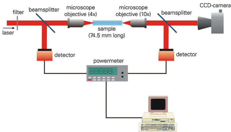
Fig. 13.25 Setup for the investigation of nonlinear propagation effects in the waveguide array. From [74]
