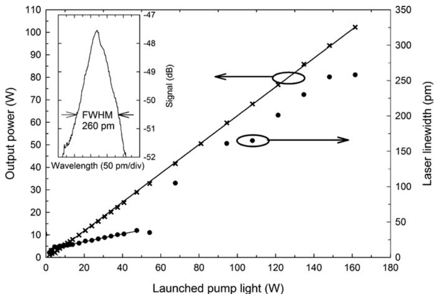
Fig. 8.12 Output power of a fibre laser with directly inscribed PbP FBGs as a function of launched pump power [13]
