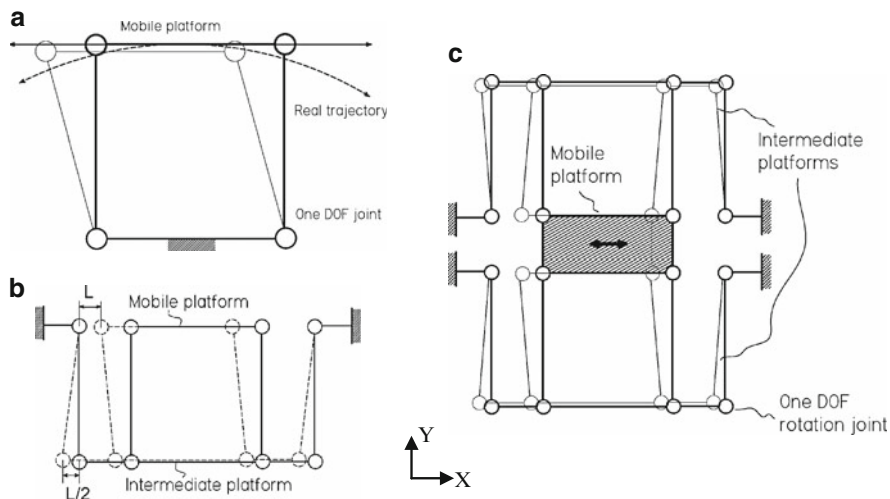
Fig. 16.18 Sensor kinematics: the circle represents ideal mechanical joints with one degree of freedom (rotation in the plane). Figure (a) shows a parallelogram four-bars mechanism; (b) represents a single compound design, and (c) a double-compound design
