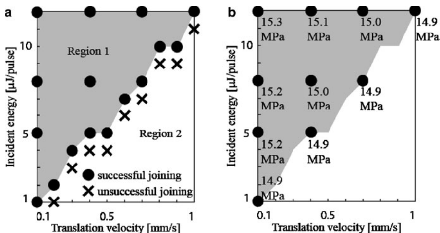
Fig. 17.7 (a) Dependence of laser-pulse energy and translation velocity on joining of borosilicate and fused silica substrates, whose coefficients of thermal expansion are different. (b) Joint strength after joining of fused silica substrates for various energies and translation velocities
