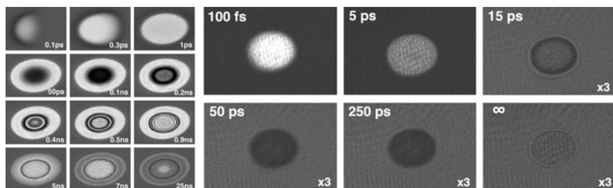
Fig. 2.3 Taken from [31]. Left set of frames : surface of a Si wafer at different delay times after irradiation with a fs laser pulse. Frame size: 300 \times 220 \mu\text{m} . Right set of frames : surface of BK7 glass after irradiation with a fs laser pulse. Frame size: 200 \times 130 \mu\text{m}
