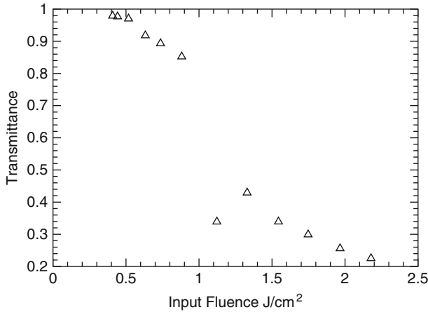
Fig. 15.4 Transmittance versus input fluence for Foturan irradiated with a fs laser at 800 nm (courtesy of X. Xu)
