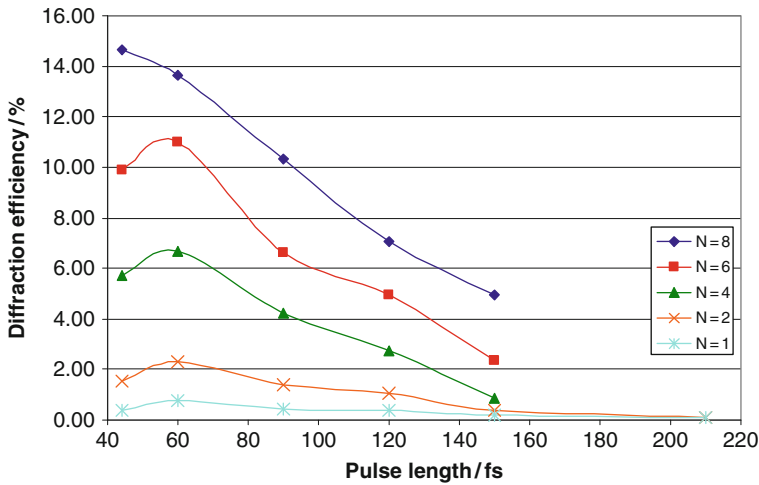
Fig. 12.9 Rearranged data from Fig 12.8 – diffraction efficiency depending on pulse length
