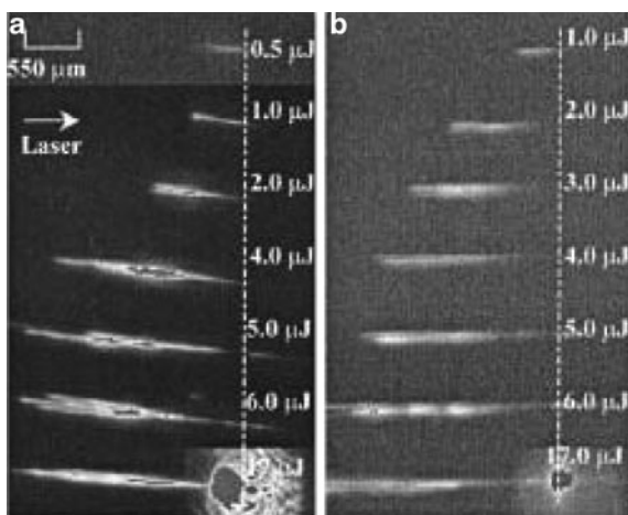
Fig. 12.13 CCD images of the accumulated laser scattering and plasma fluorescence signals in fused silica at different pulse energies. An objective lens with a power of 1\times ( f = 73.5 mm, NA: 0.03) was used to focus the beam inside the glass. The sample was irradiated by roughly (a) 10,000 shots and (b) 10 shots. (from [54])
