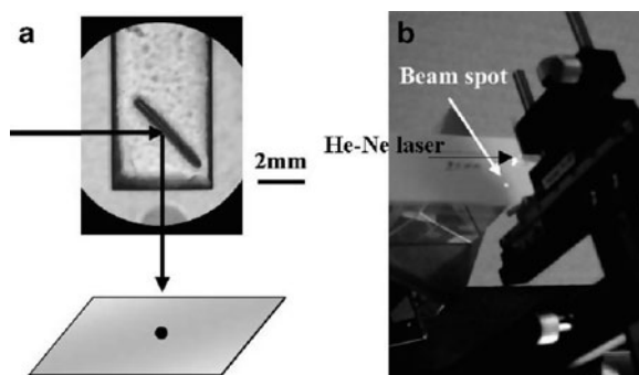
Fig. 15.10 (a) Top view of a 3D micromirror fabricated inside photosensitive glass with its optical path indicated by the arrows . (b) Beam spot reflected by the micromirror onto a receiving screen placed 10 mm away from the end of the glass chip
