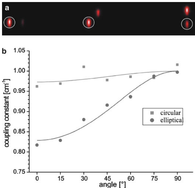
Fig. 7.18 (a) Output patterns at 633 nm for 10-mm long waveguide pairs with 20- \mu\text{m} separation at different orientations. The excited waveguide is marked by a white circle. (b) Comparison of the dependence of the coupling on the direction for 18- \mu\text{m} waveguide separation at 800-nm wavelength [47]
