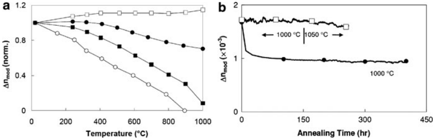
Fig. 8.8 (a) Evolution of the refractive index contrast of Type I-IR-fs (black squares), Type II-IR-fs (white squares), Type II-IR-ps (black circles) and Type I-UV-ns (white circles) written gratings [24]. (b) Evolution of the refractive index contrast of Type II-IR-fs (white squares) and Type II-IR-ps (black circles) written gratings as a function of time at constant temperatures [49]
