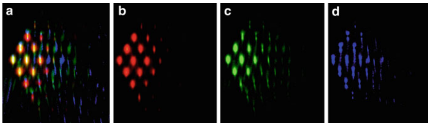
Fig. 13.13 Hexagonal array with 22\text{ }\mu\text{m} spacing. (a) Light is launched into the corner waveguide. The decomposition of the RGB image to the (b) red, (c) green, and (d) blue channels depicts the difference in coupling behavior. From [54]
