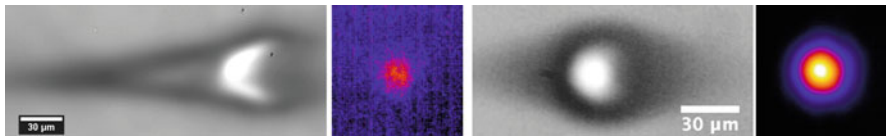
Fig. 2.14 (Taken and adapted from [67]). Static white light trans-illumination images (a, c) of femtosecond laser-written waveguides in Er:Yb co-doped phosphate glass at a depth of 1.56 mm using a 1 kHz repetition rate and slit shaping (slit width = 350 \mu\text{m} ). (a) Pulse duration = 100 fs, pulse energy = 6.4 \mu\text{J} , linear polarization; (c) 250 fs, 4.0 \mu\text{J} , circular polarization. Near field images of the corresponding guided modes at 1550 nm are shown in (b, d)
