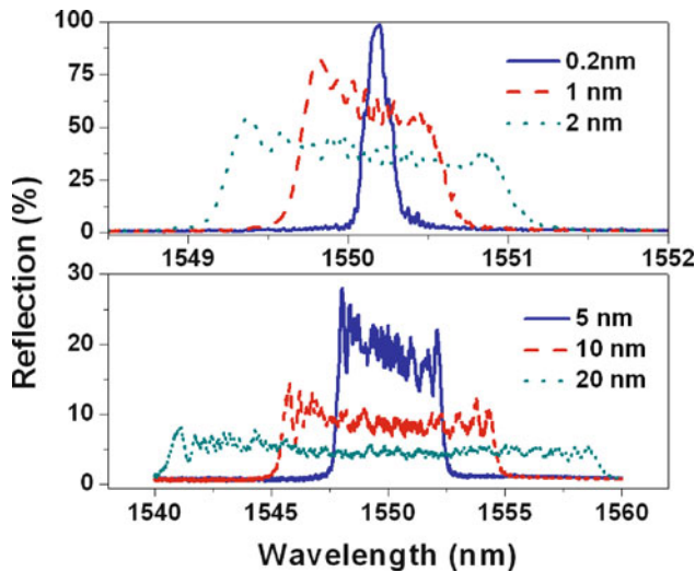
Fig. 9.21 Reflection spectra of chirped BGWs with designed bandwidth marked in the spectrum graphs. Burst laser writing was applied to fused silica glass
