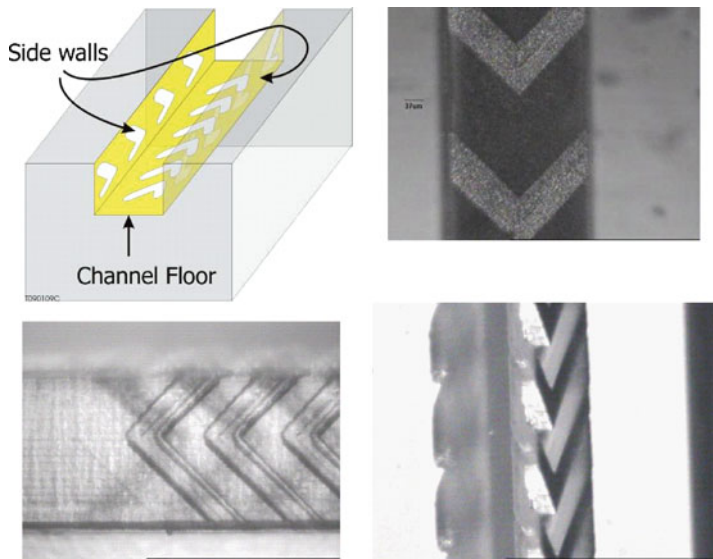
Fig. 16.10 Microfluidic channel with shaped walls and floor. Top left , a schematic representation of the channel with location of various pattern. Top right , floor with chevrons. Bottom left , sidewalls with chevrons (the back wall is out of focus). Bottom right , a side view of chevrons in a sidewall
