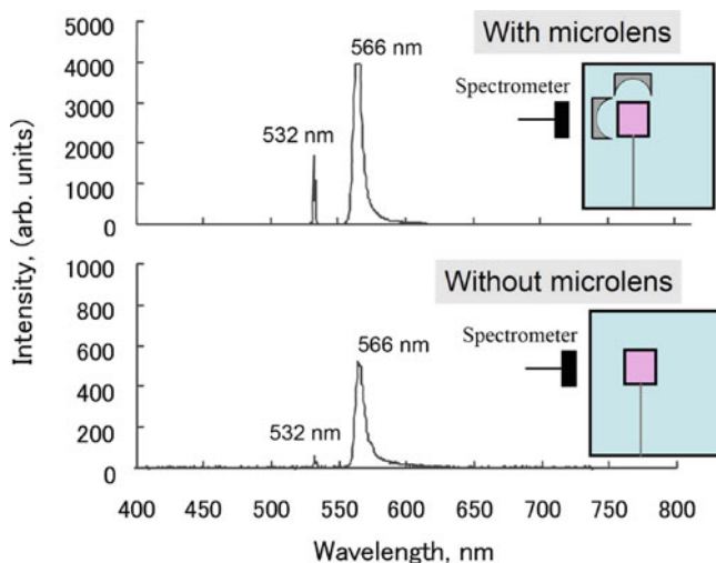
Fig. 15.16 Emission spectra from Rh6G laser dye pumped by the 2nd harmonic of an Nd:YAG laser at 32 mW. The images in the top and bottom panel were obtained using a microchip with and without a microlens, respectively
