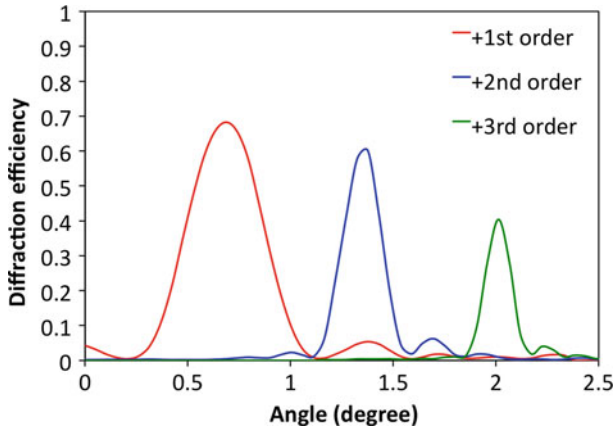
Fig. 12.19 Diffraction efficiency of 5 \times 5 \times 1 \text{ mm} thick, 22 \mu\text{m} pitch grating created using parallel processing
