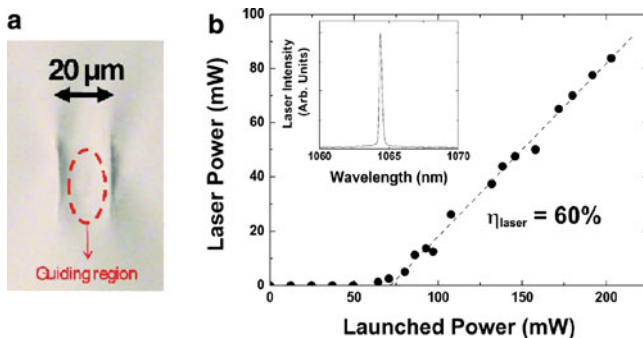
Fig. 10.10 (a) Microscope image of the end face of the active waveguide fabricated in Nd-doped YAG ceramic by two-line fs-laser writing technique. (b) Output power as a function of the launched pump power of the fs-laser written Nd waveguide laser. Inset shows the spectral dependence of the laser radiation. Reprinted with permission from [51]
