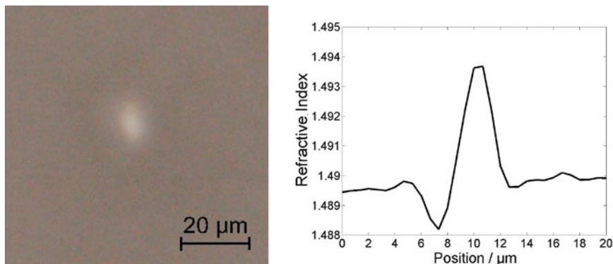
Fig. 12.4 Waveguide cross-section (beam diameter with D = 2 mm aperture, laser fluence \Phi = 0.35 \text{ J cm}^{-2} , scan speed s = 2 \text{ mm s}^{-1} ) and profile of a refractive index structure in clinical grade PMMA (at 633 nm, 23°C)
