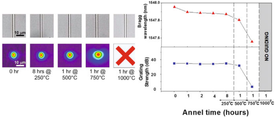
Fig. 9.17 Microscope images ( upper left corner ) and mode profiles ( lower left corner ) of BGWs written in fused silica glass with burst method of 60% AOM duty cycle, under various heat cycles of annealing together with ( right ) plots of Bragg wavelength and grating strength under various heat cycles
