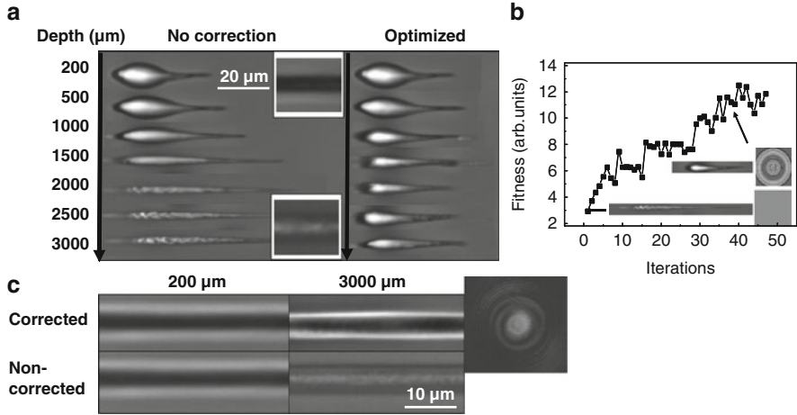
Fig. 4.6 (a) Non-corrected ( left ) and spatially corrected ( right ) static PCM structures induced in BK7 at different depths. The structures are generated by 10^5 pulses of 150 fs duration at 100 kHz and 125 mW average power. The input radiation wavelength is 800 nm and the effective focusing NA is 0.36. (b) Evolution of the trace fitness during the optimization run at the depth of 2500 \mu\text{m} . Example of traces and corresponding gray-level phase masks at different moments are given as well. (c) Longitudinal structures (PCM) at different working depths in corrected ( top ) and non-corrected ( bottom ) cases. The corrections enable a positive refractive index change over a distance of 3 mm. Scanning speed is 1 \mu\text{m/s} at 125 mW average power. Right, far-field pattern of the guided mode at 633 nm for the corrected guide [59]
