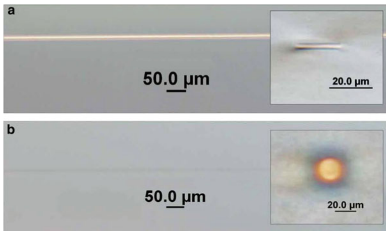
Fig. 5.13 Differential interference contrast images of two structures. One inscribed (a) without the use of a slit, and the other inscribed (b) with the use of a 500\text{ }\mu\text{m} slit placed before the focussing lens. (Taken from [39].)
