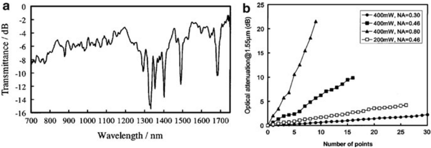
Fig. 8.10 (a) Transmission spectrum of a Type I-IR PbP LPG [6]. (b) Optical attenuation as a function of the number of refractive index modifications inscribed into the core of a fibre [56]
