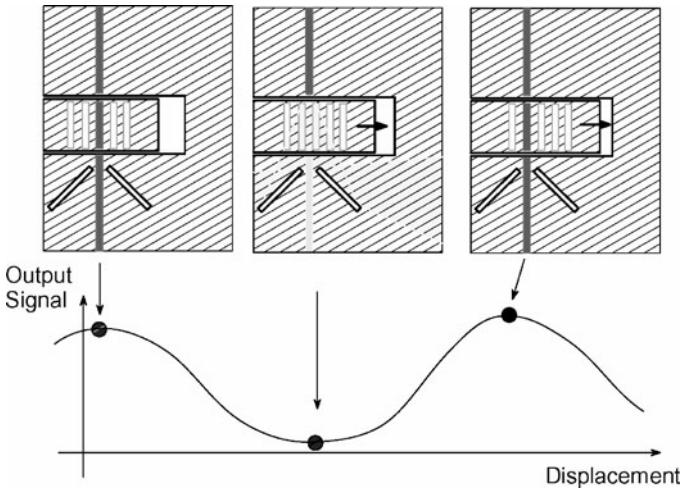
Fig. 16.20 “Waveguides-based linear encoders principles”
