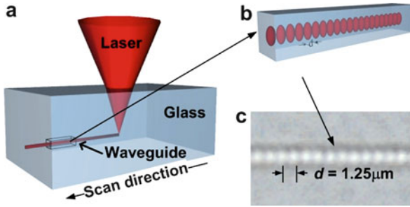
Fig. 9.2 Schematic illustration (a) of the waveguide fabrication process with the sample translated perpendicularly to the focused laser beam direction, and leading to an array of isolated focal volumes (b) under high ( >1 \text{ mm s}^{-1} ) scan velocities. An overhead microscope image (c) of a waveguide showing the isolated modification volumes written with 1.25 \text{ mm s}^{-1} scan speed
