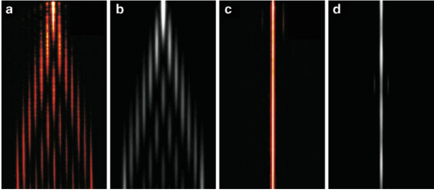
Fig. 13.30 In (a) and (b), the experimental and theoretical propagation patterns inside a homogeneous array are shown. Suppression of the coupling between adjacent guides due to the modulation of the refractive index is shown experimentally in (c) and theoretically in (d). From [76]
