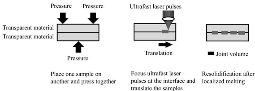
Fig. 17.2 Schematic diagrams of ultrashort laser microwelding/joining process
