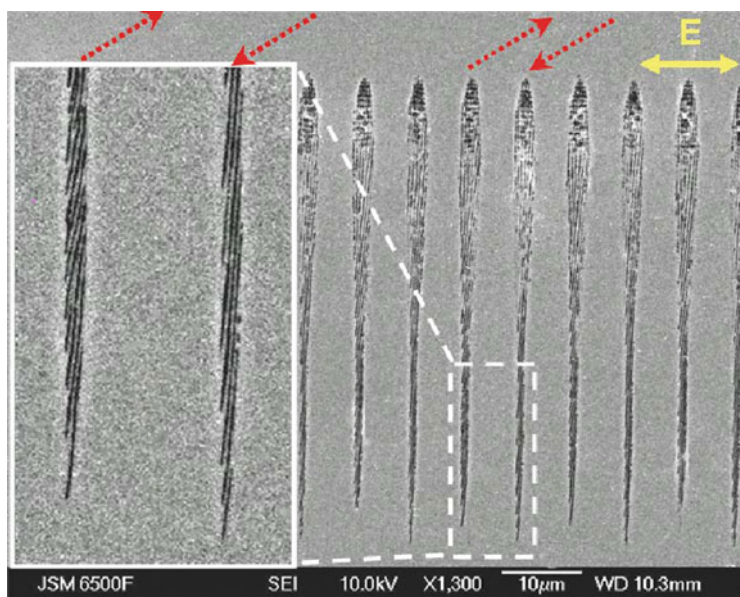
Fig. 6.1 SEM images of cross sections of the structures formed 0.5 mm below the surface of fused silica with a 0.55 NA lens. The distance between lines is 7 \mu\text{m}
