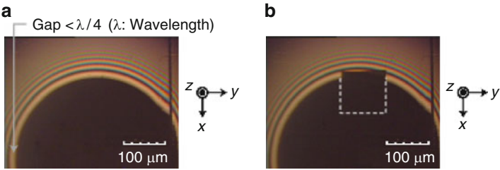
Fig. 17.5 White-light fringes of the welded samples, silica–glass substrate and lens, before (a) and after (b) irradiation by ultrashort laser pulses. The incident pulse energy was 1.0 μJ and the translation velocity of the filament was 5 μm/s. The dashed square indicates the joint area of 100 × 100 μm 2 in the sample. The figure indicates, by irradiation of the laser pulses, a bright area (one-quarter-wavelength gap) that was changed to a black area (zero gap) because one-quarter-wavelength gap was almost filled up
