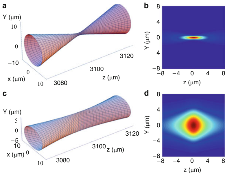
Fig. 5.12 (a) Beam evolution near focus not using slit, (b) energy distribution in YZ plane not using slit, (c) beam evolution near focus using slit and (d) energy distribution in YZ plane using a 500\text{ }\mu\text{m} slit orientated along the x -axis. (Taken from [39].)
