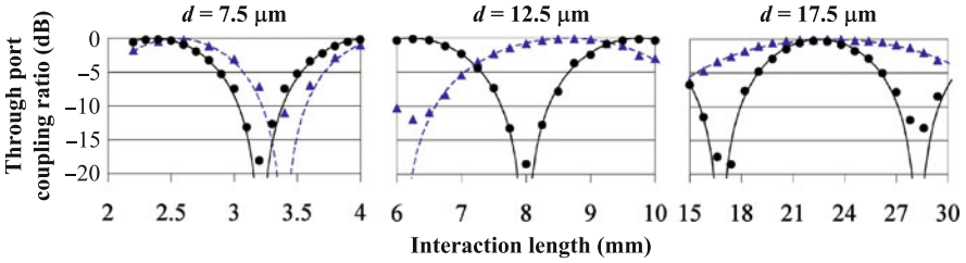
Fig. 7.24 Through port coupling ratio dependence on interaction length for separations d = 7.5 , 12.5 , and 17.5 \mu\text{m} at 1310 (triangles) and 1550 -nm (circles) wavelengths. Sinusoidal curve fits are shown as dashed and solid lines for 1310 and 1550 nm, respectively [2]
