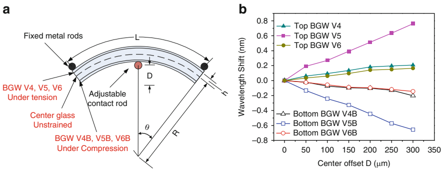
Fig. 9.28 Beam bending arrangement (a) for optical strain sensing in a 3D BGW network and correspond Bragg wavelength shifts (b) under increasing beam displacement
