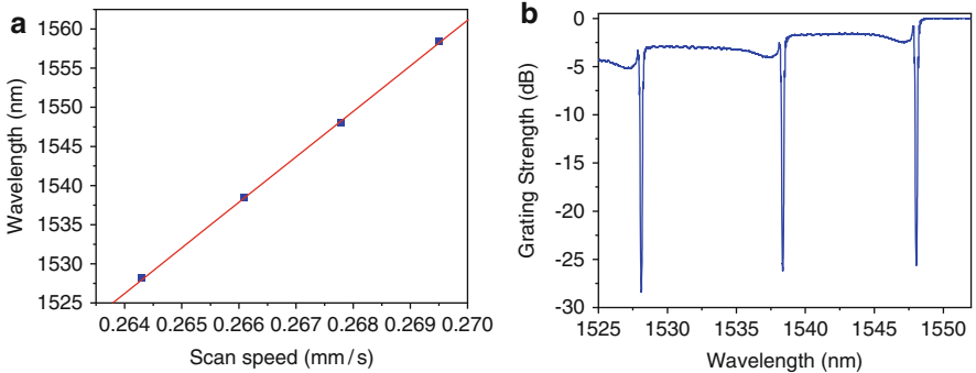
Fig. 9.20 First-order Bragg wavelength tuning by velocity change (a) and the transmission spectrum of the cascaded BGW (b). These BGWs were fabricated in fused silica glass with the burst fabrication method, using the MHz laser system
