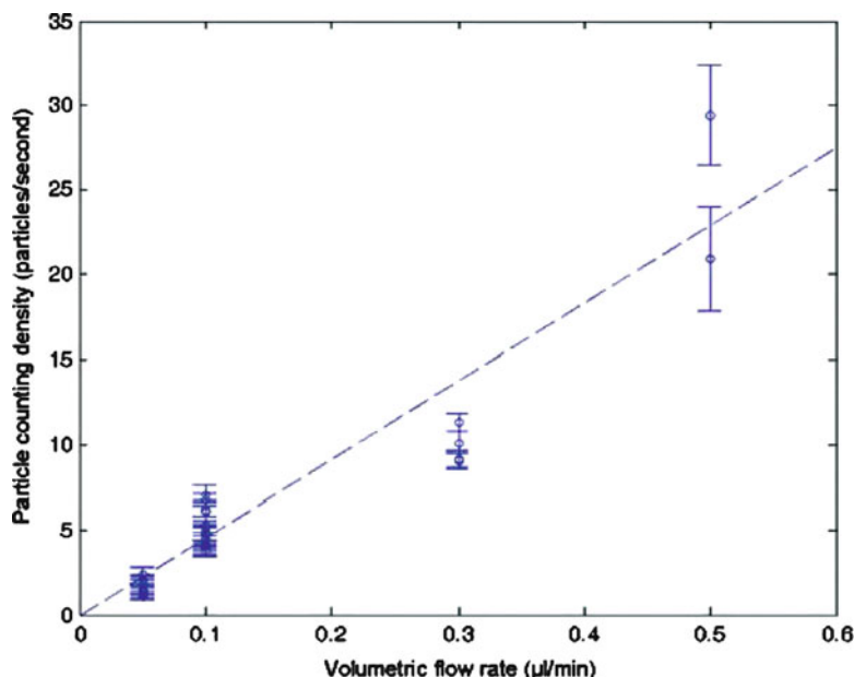
Fig. 14.15 Measured particle counting density with respect to volumetric flow rate ( \mu\text{l min}^{-1} ). Each data point is an average of measured values for 30 s and error bar represents the standard error of the mean. Dashed line represents calculated particle counting density given particle concentration and volumetric flow rate [62]
