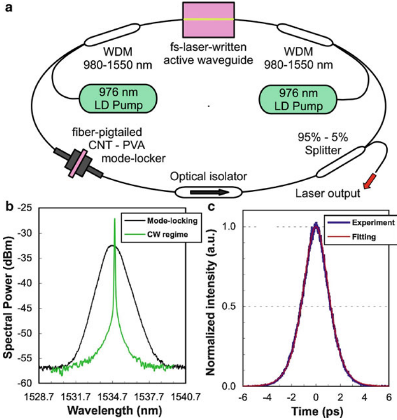
Fig. 10.11 (a) Schematic of the Er:Yb ring laser cavity for mode-locking operation. (b) Laser power spectra in continuous-wave and passive mode-locking regimes. (c) Autocorrelation trace of the laser pulses. Reprinted with permission from [44]
