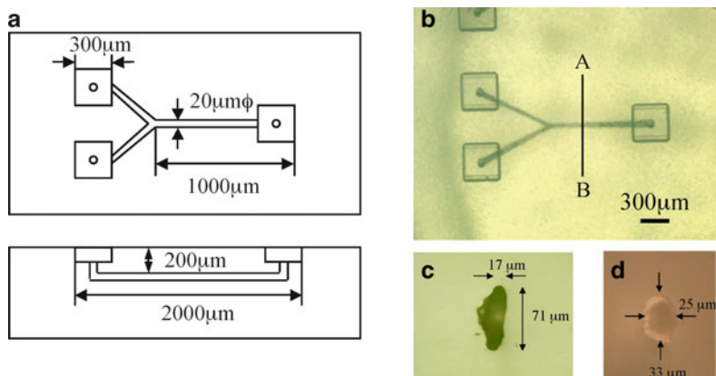
Fig. 15.8 (a) Configuration of a horizontal Y-shaped microchannel structure. Photos of (b) a top view of the fabricated structure, and (c) a cross-section of the microchannel after it was mechanically cut along line A–B. (d) Rounder cross-sectional shape of the microchannel by using a slit with a width of 0.2 mm
