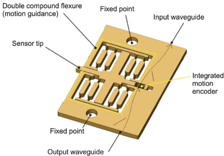
Fig. 16.17 Drawing of a glass-based force-sensing device. The mobile “sensing” platform has a cross shape and is prolonged by a sensor tip
