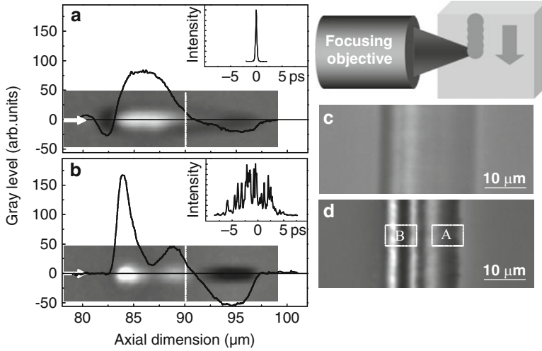
Fig. 4.4 Refractive index flip in borosilicate crown BK7 under multipulse (a) short (150 fs) and (b) optimally tailored irradiation (4.5 ps). Pulse energy 0.17 \mu\text{J} , irradiation dose 10^5 pulses at 100 kHz, with the 800 nm pulses focused from the left via an NA of 0.42. Phase contrast microscopy images of refractive index changes (white and black colors represent negative and positive refractive index changes, respectively) with corresponding pulse envelopes given in the insets. The axial index profiles are indicated by the solid lines. The onset of a significant compression zone is visible under optimal conditions (intense black color). Transverse trace written by (c) short pulses and (d) optimal laser pulses at a scan velocity of 50 \mu\text{m/s} and pulse energy of 1.1 \mu\text{J} . Two regions of positive refractive index changes are indicated by the labels A and B. Data were extracted from [17]
