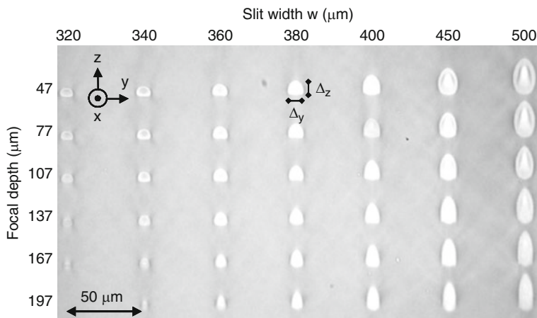
Fig. 7.13 Cross sectional microscope image of waveguides written in bismuth borate glass showing dependence on focal depth and slit width [37]
