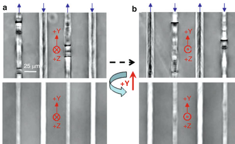
Fig. 6.13 Phase images of line structures in the flip experiment. (a, b) QPM phase images of lines written along the Y axis with 2.4 \mu\text{J} (top) and 2 \mu\text{J} (bottom) pulse energies. The lines were written by propagating the laser beam along the +Z axes (a) and the -Z axes (b) of the crystal respectively
