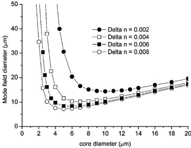
Fig. 5.2 1/e^2 mode field diameter (MFD) of the fundamental mode as a function of the core diameter for circular-core step-index waveguides with different refractive index contrasts. The free-space wavelength of the guided light in the model was set to 1.55\ \mu\text{m}
