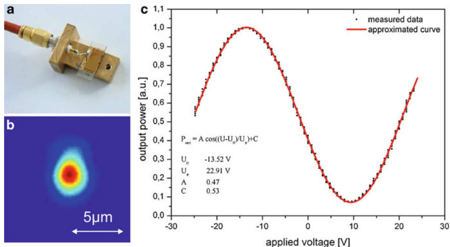
Fig. 11.13 (a) X-cut LiNbO 3 sample containing the femtosecond laser written modulator for TM polarized light. (b) Guided mode in the maximum of transmission. (c) Modulation of the output intensity depending on the applied voltage [34]
