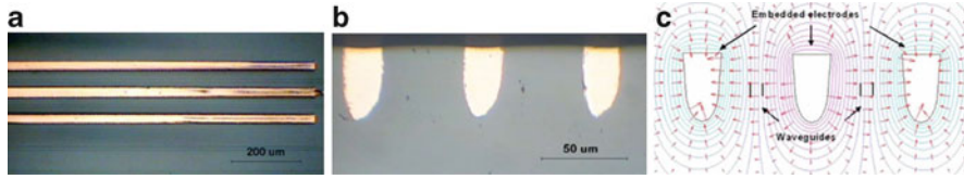
Fig. 11.12 (a) Top and (b) end views of optical micrographs of the embedded electrodes and optical waveguides; (c) contour plots of the equipotential contour of the embedded electrodes [33]
