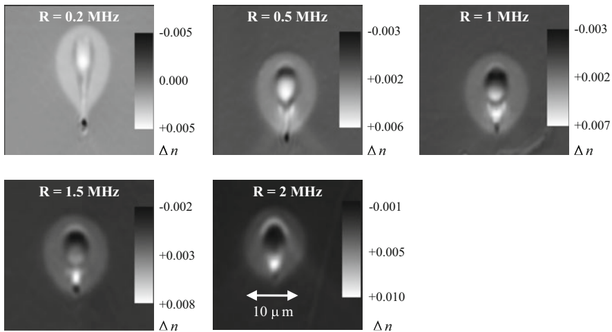
Fig. 7.7 Cross sectional refractive index profiles of waveguides written with 200-mW power, 25-mm/s scan speed and repetition rates of 0.2, 0.5, 1, 1.5, and 2 MHz. The writing laser was incident from the top and the refractive index scale is shown on the right [10]
