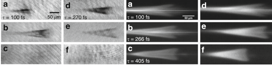
Fig. 2.13 (Taken from [50]). Left two columns : time-resolved transmission images recorded in bulk Er:Yb codoped phosphate glass at 1.56 mm depth with circularly polarized transform limited, 100 fs pump laser pulses of 8 \mu\text{J} energy [(a)–(c)] and stretched pulses (270 fs) [(d)–(f)] at several time delays t = 0.65 ps in (a), (d), 1.2 ps in (b), (e), and 50 ps in (c), (f). In all images the laser beam impinges from the left. Right two columns : time-integrated plasma emission images recorded for various pump pulse durations \tau_{\text{pump}} under the same experimental conditions, i.e., pump energy, processing depth. In (a)–(c) plasma emission images for horizontal polarization are shown, whereas (d)–(f) show plasma emission images for circularly polarized laser light with the same values of \tau_{\text{pump}} as in (a)–(c)
