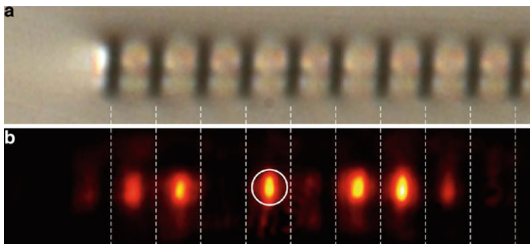
Fig. 11.15 Planar array of evanescently coupled type II waveguides [42]. (a) Micrograph of the end facet. (b) Discrete diffraction pattern for excitation at 633 nm (excited site is marked by the circle)
