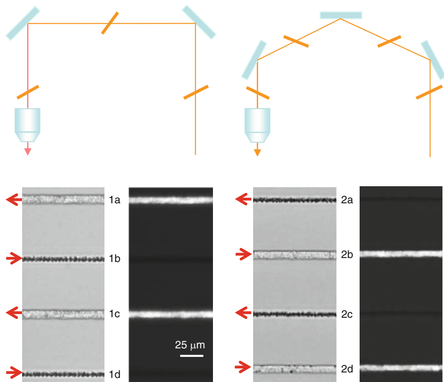
Fig. 6.6 “Quill” effect – lines written in opposite directions have different morphology. In crossed polarizers, one can clearly see that birefringent modification is induced only in one direction. The effect can be reversed by reversing tilt direction by reflecting beam from a mirror
