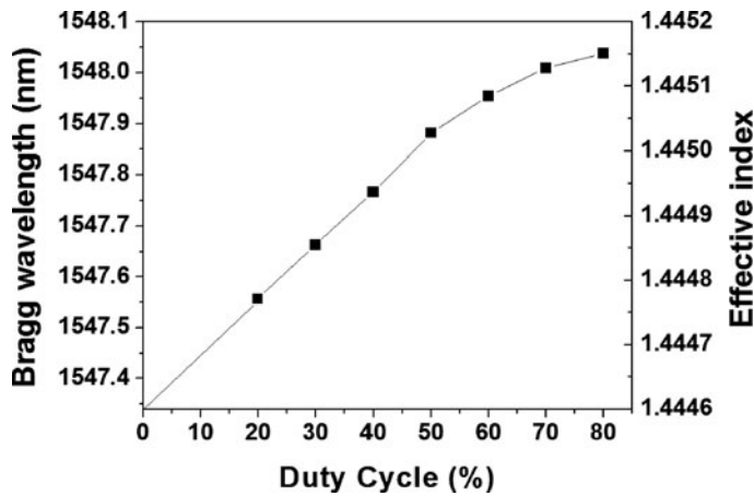
Fig. 9.14 Bragg wavelength dependence of the grating waveguides on the AOM modulation duty cycle. The BGWs were written inside fused silica with the 500-kHz laser system
