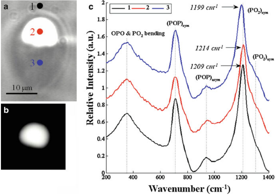
Fig. 3.14 (a) White-light transmissions image of modification induced under fs laser condition of 885 kHz rep rate, 320 nJ pulse energy, and 50 \mu\text{m s}^{-1} scan speed. 1. Unmodified bulk glass; 2. modified high index guiding region; 3. modified non-guiding low index region; (b) He-Ne transmission near field image. (c) Normalized Raman spectra of Er-Yb doped phosphate glass for: 1. unmodified bulk glass; 2. modified high index region; 3. modified low index region
