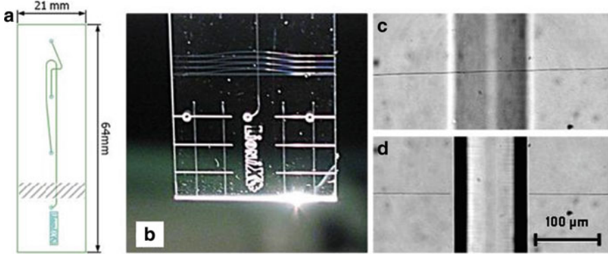
Fig. 14.12 (a) Schematic of the commercial LOC for MCE (LioniX BV). MZIs are fabricated in a region at the end of the separation channel indicated by the shaded area . (b) Picture of the commercial LOC with 4 MZIs inscribed across a microchannel; the grid of microchannels at the bottom of the chip facilitates the sealing of the device and has no fluidic function. Microscope images of (c) the reference arm passing over the microchannel and (d) the sensing arm crossing it
