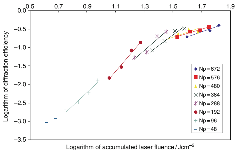
Fig. 12.10 Yield of photoreaction at constant pulse duration ( \tau = 60 fs) versus laser fluence, accumulated over a number of pulses N_p at four constant laser fluences ( \Phi = 0.1, 0.12, 0.14 , and 0.16 \text{ J cm}^{-2} ); line gradients indicate the order of the non-linear process (Table 12.2) [38]
