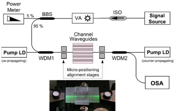
Fig. 10.3 A typical all-in-fiber experimental set-up for active waveguide characterization. ISO : optical isolator. VA : variable attenuator. BBS : broad-band splitter. WDM1 and WDM2 : wavelength-division multiplexer. OSA : Optical spectrum analyzer. Inset shows an Er:Yb-doped channel waveguide under bi-propagating pumping scheme exhibiting the characteristic green up-conversion fluorescence from erbium ions
