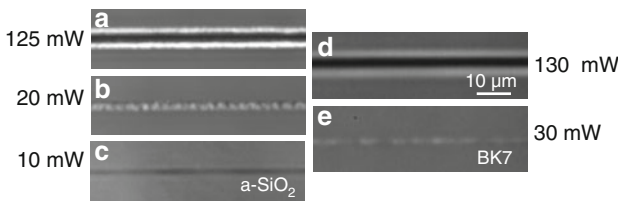
Fig. 4.1 The effect of the irradiation dose on the structure morphology during longitudinal photoinscription of refractive index modification traces using focused ultrafast laser radiation. The structural changes are observed in phase-contrast microscopy and the black color denotes a positive index change. The left parts (a–c) describe various trace types in fused silica at different input powers and a scan velocity of 50 m/s. The photoinscription character varies from an incubative type at low intensities, relying on electronically-triggered structural effects which determine positive index changes, to the onset of thermo-mechanical effects at moderate and higher incident powers resulting in visible dense and rarefied regions. The right parts (d,e) indicate morphological changes in borosilicate BK7, where most observable are rarefaction and compaction effects. The incident pulse duration is 150 fs and the pulse repetition rate is 100 kHz. The focusing numerical aperture for the incident 800 nm laser radiation is NA = 0.42
