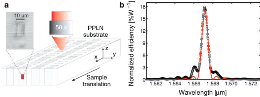
Fig. 11.9 (a) Schematic of the multiscan writing setup, inset : microscope image of the waveguide end face [9]. (b) Normalized SHG efficiency as a function of pump wavelength: experimental data (circles) and theoretical fit (solid line) [9]
