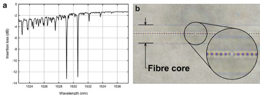
Fig. 8.3 (a) Graph showing the spectral characteristics of a phase-modulated sampled grating fabricated in SMF-28 fibre using PbP inscription [38]. (b) A micrograph of one of the \pi/2 phase modulations of the sampled grating
