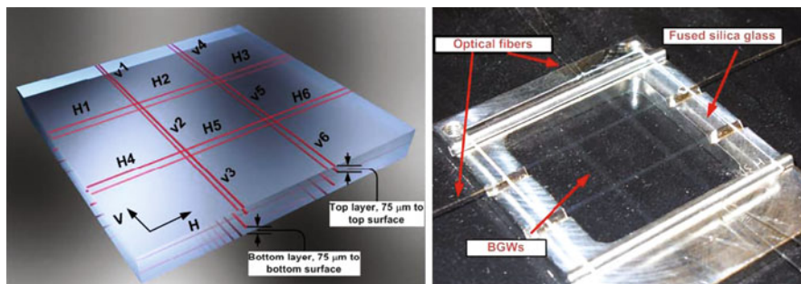
Fig. 9.24 A 3D sensor network in a fused silica plate (50 mm × 50 mm × 1 mm) consisting of multi-wavelength BGW segments (red lines) laid out as shown in the schematic of (a) and the photograph of (b). Single-mode fibers are shown epoxied for butt-coupling to six of the BGW segments here
