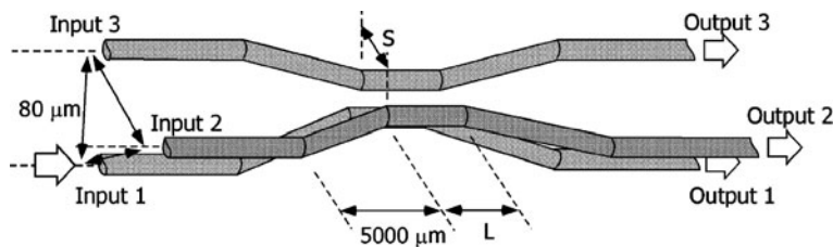
Fig. 7.22 Schematic configuration of a 3 × 3 directional coupler [51]
