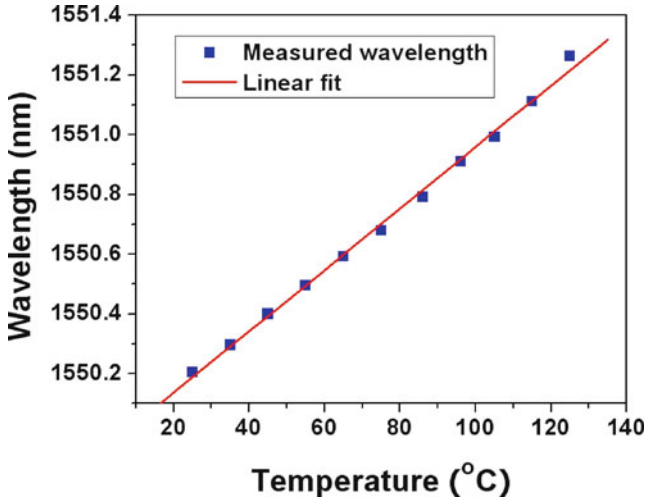
Fig. 9.26 BGW resonance wavelength plotted with respect to temperature of the hotplate
