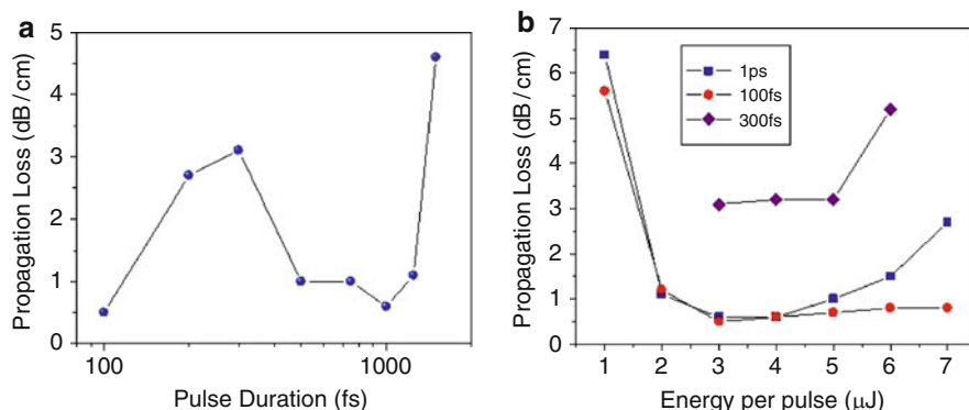
Fig. 9.4 Propagation loss of BGWs written with (a) 3- \mu J pulse energy for increasing the pulse duration and with (b) 100 fs, 300 fs, and 1 ps pulse durations with increasing pulse energy. These devices were written inside borosilicate glasses with the kHz laser system
