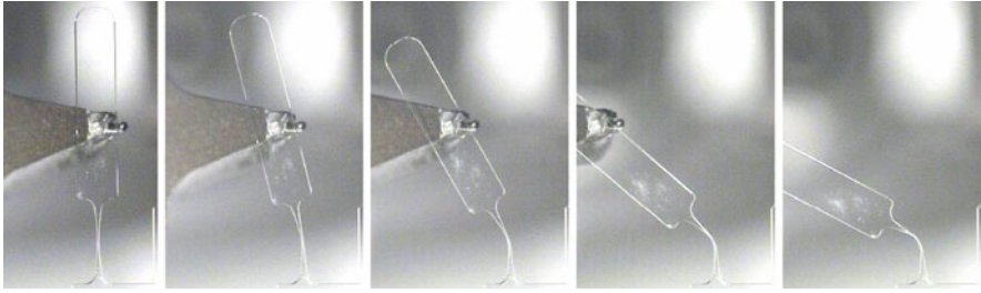
Fig. 16.13 Flexure bending tests sequence: the flexure is 40\text{ }\mu\text{m} wide at the neck. The bending is completely reversible. Note the severe deflection of the microhinge
