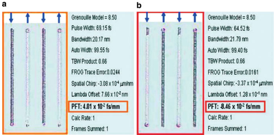
Fig. 6.5 Microscope bright field image of the line structures written using femtosecond pulses with positive pulse front tilt (a) or negative pulse front tilt (b). The distance between the lines is 25 \mu\text{m} . The writing direction is shown by the arrow. The respective screen shots containing measured laser pulse parameters by GRENOUILLE device are shown
