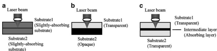
Fig. 17.1 Schematic diagrams of conventional laser welding/joining
