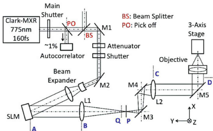
Fig. 12.16 Energetic 1 mJ, 775 nm, 160 fs pulses are reflected by mirrors M1 and M2, attenuated then expanded to 8 mm diameter before reflection from the SLM liquid crystal device where a CGH is displayed. Diffracted beams are re-imaged to the input aperture (plane D) of the microscope objective with a 4f optical system where distance AD = 4f and distance AB = BP = PC = CD = f . CGHs are applied to the SLM representing the desired intensity distribution at the focal plane of a long working distance objective (0.15 NA) and carefully focused below optical substrate surface positioned on a three-axis stage
