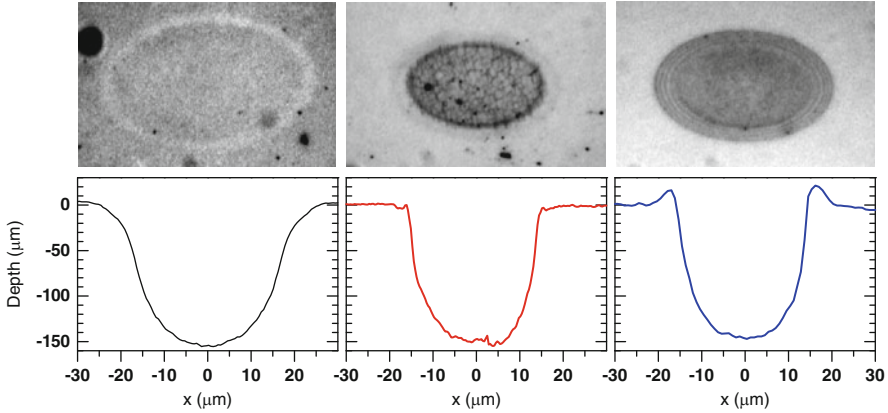
Fig. 2.8 Static white light reflection images ( R_{WLM} ) and surface topography profiles from white light interferometry ( D_{WLI} ) of laser-irradiated regions in fused silica (left, 11.9 \text{ J cm}^{-2} ), sapphire (middle, 12.5 \text{ J cm}^{-2} ) and phosphate glass (right, 5.2 \text{ J cm}^{-2} )
