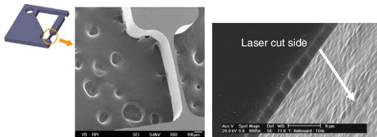
Fig. 16.12 Micromachined flexure: the RMS roughness is approximately 300 nm at the edges, and 200 nm at mid-height
