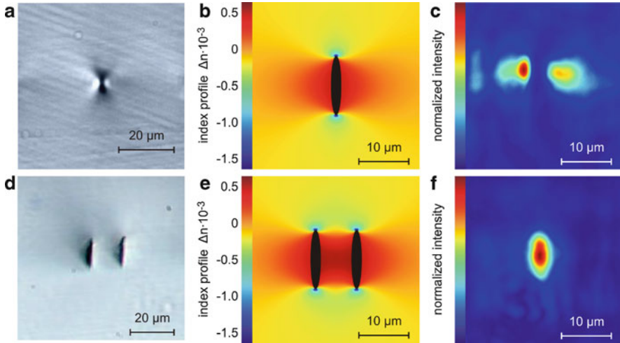
Fig. 11.5 Single type II modification in z-cut LiNbO 3 : (a) Microscope image, (b) simulated stress-induced index-increase ( n_e ) and (c) exemplary guided mode at 633 nm [5]. Dual-line waveguide based on type II modifications: (d) microscope image [11], (e) simulated stress-induced index-increase ( n_e ), and (f) exemplary guided mode at 633 nm
