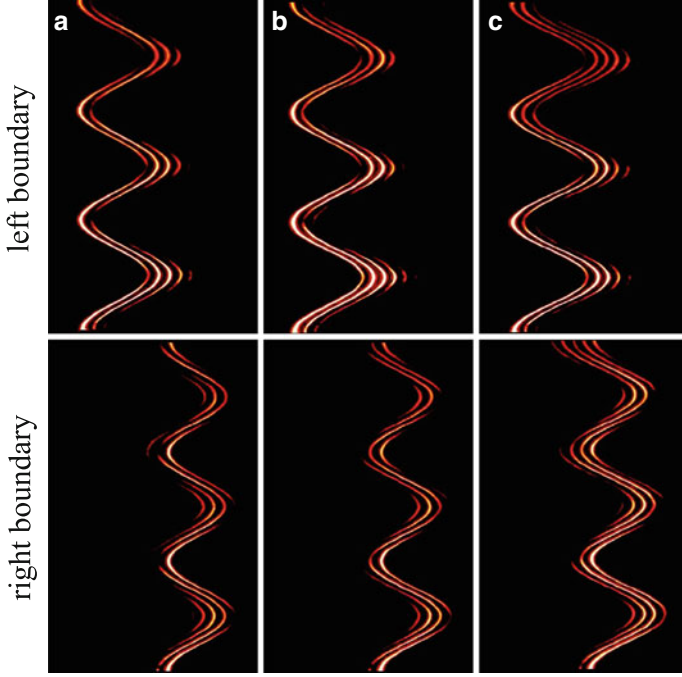
Fig. 13.18 Surface phenomena in periodically curved arrays with a waveguide spacing of d = 14 \mu\text{m} . The surface assists the formation of bound states also in a region around the resonance. The amplitude of the curving profile F was detuned from the resonance amplitude F_0 for the left ( upper row ) and right ( lower row ) boundary waveguide. The detuning F/F_0 is (a) 1.0, (b) 1.05, and (c) 1.1. From [63]
