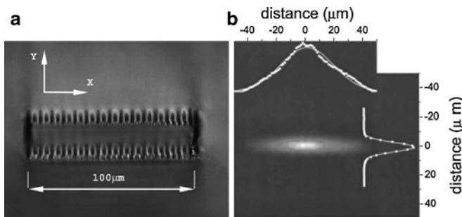
Fig. 11.7 (a) End view of a depressed cladding waveguide inscribed in \text{Nd}^{3+} :YAG; (b) near-field image of the laser beam. Field profiles and Gaussian fitting curves are shown as scatter graphs and solid curves , respectively [20]
