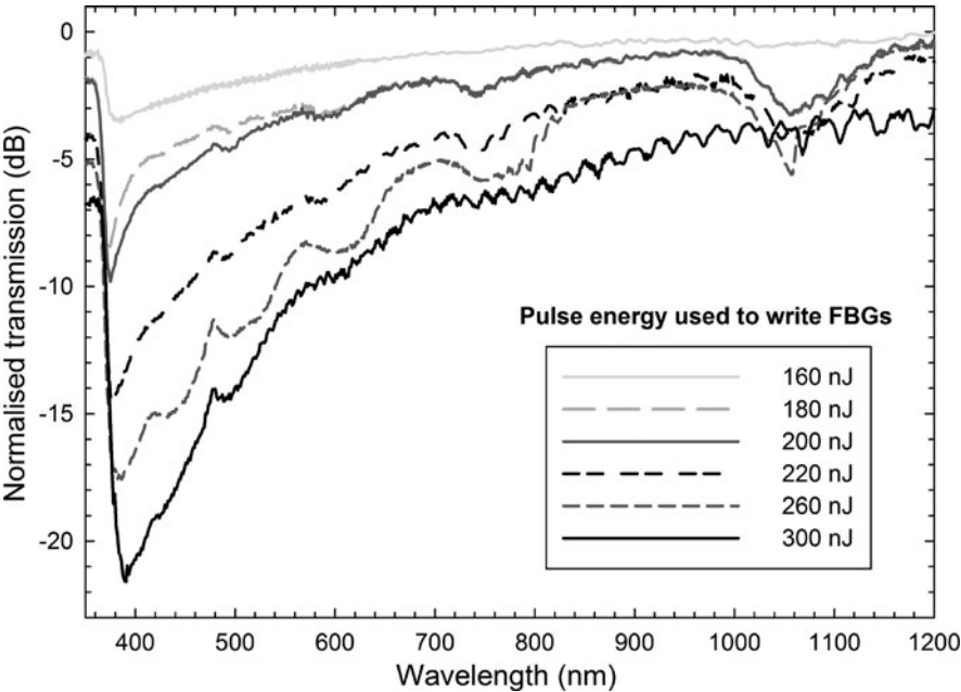
Fig. 8.11 Normalised transmission spectra for Type II-IR femtosecond inscribed PbP FBGs in SMF-28 [57]
