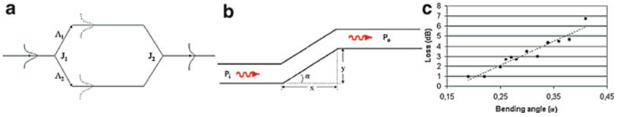
Fig. 11.11 (a) Schematic diagram of a simple MZI with single input and output waveguides. (b) Schematic diagram showing the offset transition with sharp corner bend design utilized in this approach. (c) Losses for the configuration shown in (b) as a function of the bending angle [32]
