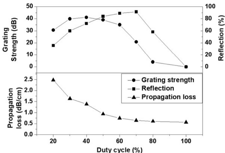
Fig. 9.15 Change of grating strength, peak reflection percentage, and the propagation loss of the fused silica BGWs with respect to the AOM duty cycle
