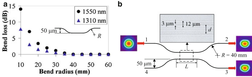
Fig. 7.23 (a) Bend loss versus radius of curvature at 1310 and 1550 nm. Inset shows one arm of the coupler under test with four bends of radius R . (b) Schematic of directional coupler and optical microscope image of waveguides in coupling region (top) together with mode profiles of 1550-nm light from launch fiber at port 1 and from output facets at ports 2 and 3 [2]
