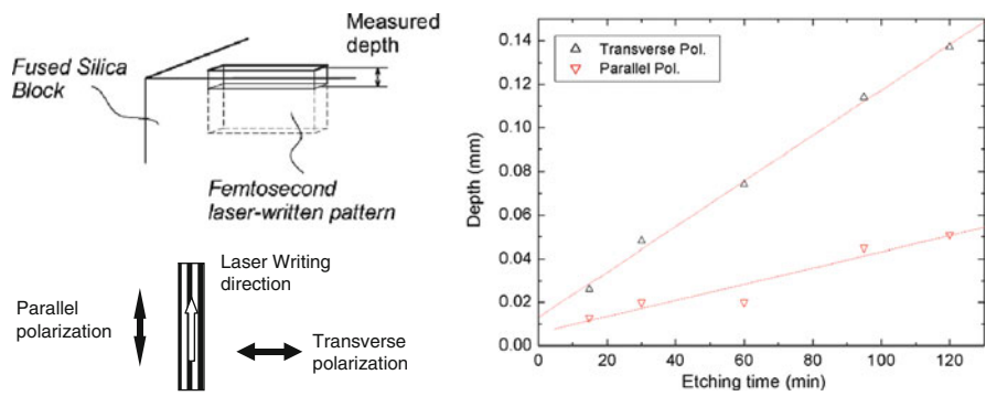
Fig. 16.7 Etching rate as a function of the polarization (The convention used to define parallel and transverse polarization is shown on the left.)
