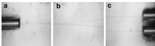
Fig. 7.15 Fiber aligned one-input (a) and two-output channels (c) of U-grooved Y-junction (b) optical splitter [42]
