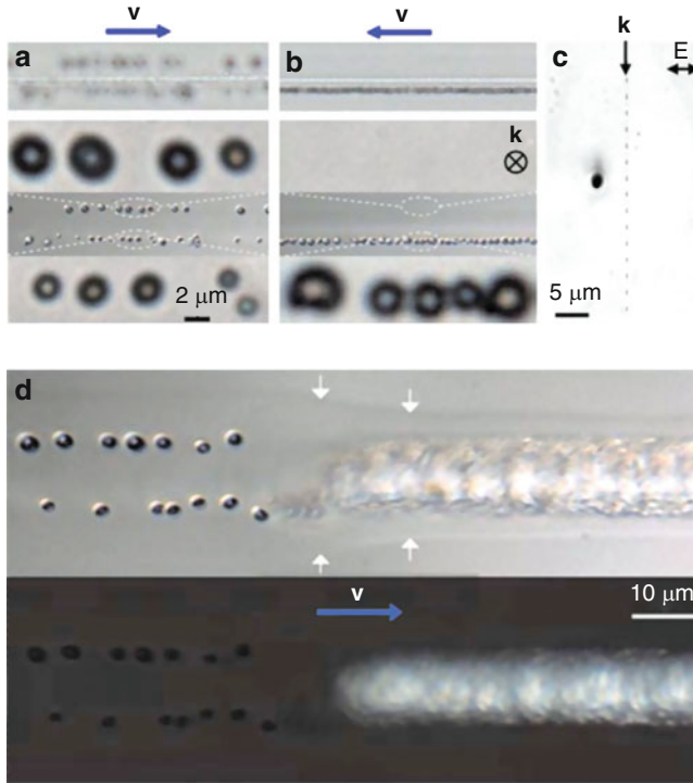
Fig. 6.8 [a and b] Bright field images with different magnifications of the line structures fabricated in opposite directions (a) and (b) with 2.4 \mu\text{J} pulse energy and scan speed of 50 \mu\text{m/s} . (c) Image of a cross section of the line structure shown in (b). (d) Images of the transition region without and with crossed polarizers. \mathbf{V} is the writing velocity, \mathbf{k} is the wave vector of the writing laser, and \mathbf{E} is the electric field of the writing laser
