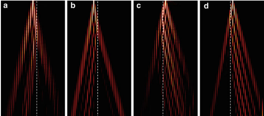
Fig. 13.9 Dissimilar waveguide arrays with a spacing of 13\,\mu\text{m} and 15\,\mu\text{m} and homogeneous refractive index modulation of \Delta n = 2 \times 10^{-4} . (a) Experimental and (b) theoretical transmission through an interface to a denser medium ( \kappa_1 = 1.09\,\text{cm}^{-1} and \kappa_2 = 1.557\,\text{cm}^{-1} ). (c, d) same array as (a, b) but for the excitation in the denser fraction [51]
