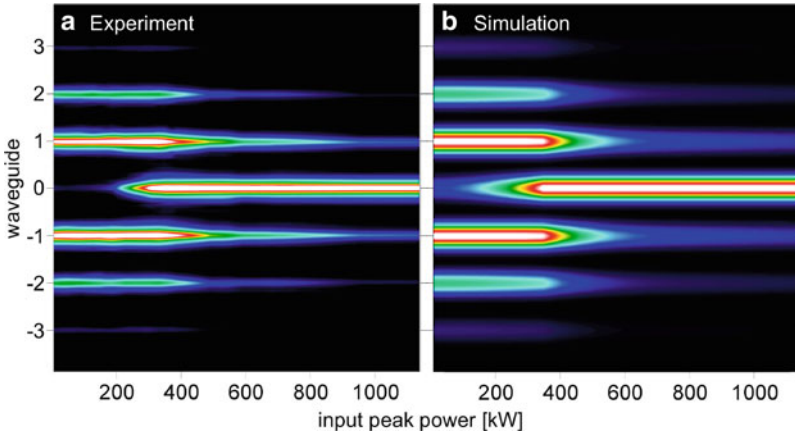
Fig. 13.28 Comparison of the evolution of the output pattern between the experimental data ( left ) and the numerical analysis ( right ). The amplitude in the n th waveguide is shown as a function of the input peak power. From [74]
