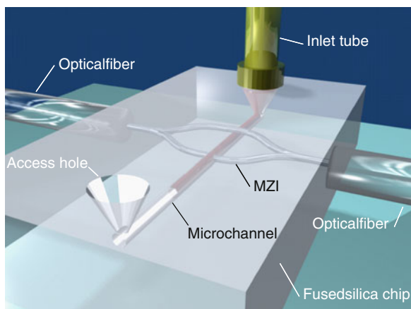
Fig. 14.11 Schematic of the femtosecond-laser-fabricated microfluidic channel and integrated MZI. The sensing arm crosses orthogonally the channel, while the reference one passes over it [60]
