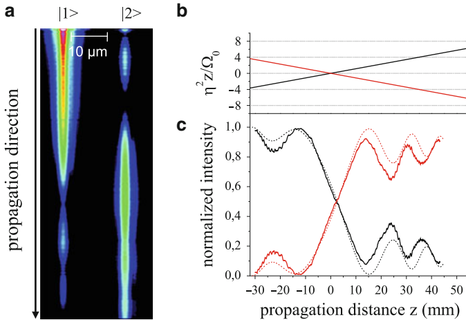
Fig. 13.21 Landau-Zener dynamics in a cubically curved waveguide coupler with a spacing of 17 \mu\text{m} corresponding to a coupling constant of \kappa = 0.063 \text{ mm}^{-1} : (a) Curved space fluorescence measurement, (b) applied energy level crossing, and (c) measured and calculated spatially resolved occupation of the states |1\rangle and |2\rangle . From [68]
