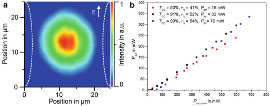
Fig. 11.14 (a) Near-field image of the guided mode of a Nd(1%):YAG waveguide laser at 330 mW laser power. (b) Efficiency curve for different output coupling percentages [23]
