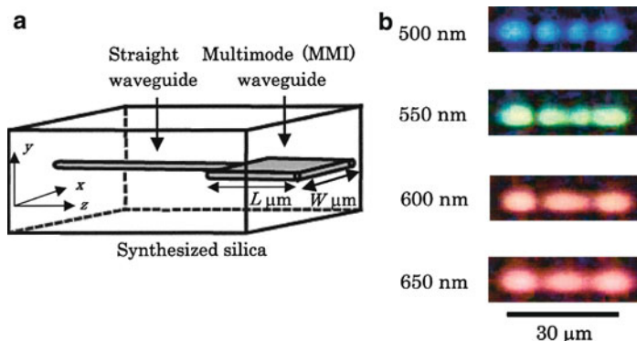
Fig. 7.30 (a) Schematic of a MMI waveguide device in fused silica. (b) Near-field pattern at the MMI waveguide output for various wavelengths, with W = 30 \mu\text{m} . The central wavelengths of the interference filters are indicated [66]
