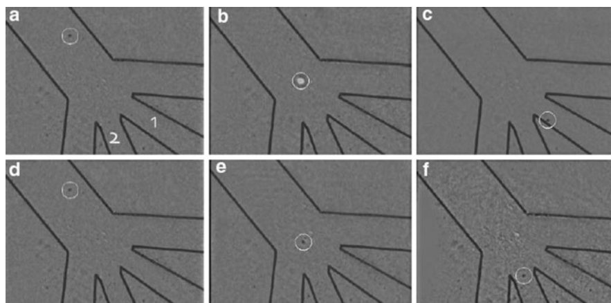
Fig. 14.7 Images of a non-fluorescing colloid and a fluorescing colloid being sorted into different output streamlines, labelled 1 and 2 in frame a . Frames a–c show the path of the fluorescing colloid going into the outlet labelled 1. In frame b the colloid is fluorescing over the waveguide output aligned with outlet 1. Frames d–f show the non-fluorescing colloid path
