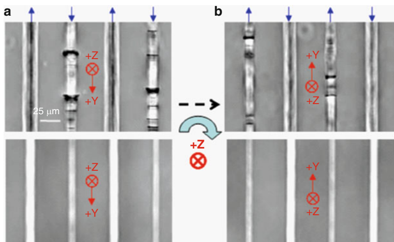
Fig. 6.12 Phase images of line structures in the rotation experiment. (a, b) QPM phase images of lines imprinted along the Y axis with 2.4 \mu\text{J} (top) and 2 \mu\text{J} (bottom) pulse energies. The lines were written before (a) and after rotating by 180^\circ around the Z axis (b) of the crystal, respectively
