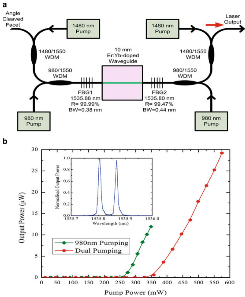
Fig. 10.7 (a) Schematic diagram of the waveguide laser in oxyfluoride silicate glass. (b) Laser output power versus pump power. Inset graph shows laser output spectrum recorded by an optical spectrum analyzer with 0.01 nm resolution bandwidth. Reprinted with permission from [45]
