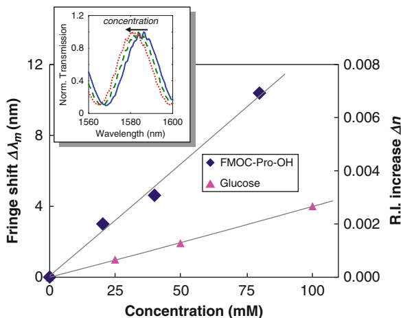
Fig. 14.13 Measured fringe shift from spectral data for different concentrations of glucose-D in water ( inset : 0 mM solid ; 50 mM dashed ; 100 mM dotted ); the correspondent refractive index increase is also shown in the right axis
