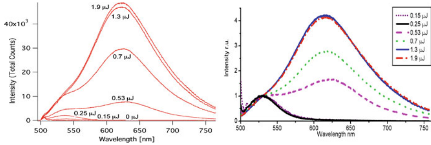
Fig. 3.7 (a) PL spectra of fs-laser modified fused silica; 488 nm light from an Ar + laser was used as the excitation source; the different curves in (a) represent different fs pulse energies used for modification. (b) Same spectra as in (a) normalized to the 530 nm band
