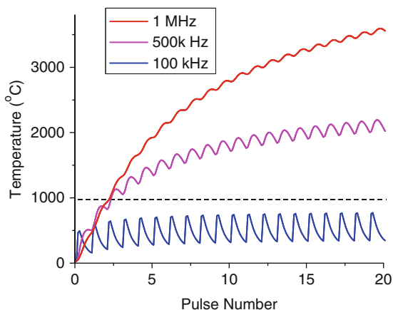
Fig. 7.5 Model of glass temperature versus exposure at repetition rates of 100 kHz, 500 kHz, and 1 MHz, at a radial position of 3\text{ }\mu\text{m} from the center of the laser beam. The absorbed pulse energy of 200 nJ was the same at each repetition rate [6]
