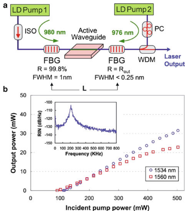
Fig. 10.6 (a) Optimized linear cavity setup for the Er:Yb-doped phosphate waveguide laser in the C-band. ISO : Optical Isolator. PC : Polarization Controller at \lambda/2 . WDM : Wavelength-Division Multiplexer. (b) Input–output characteristics of the laser at 1534 nm and at 1560 nm. Inset shows a typical RIN spectrum of the laser at 1534 nm. Reprinted with permission from [44]
