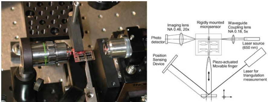
Fig. 16.23 Experimental setup: ( left ) partial view and ( right ) sketch
