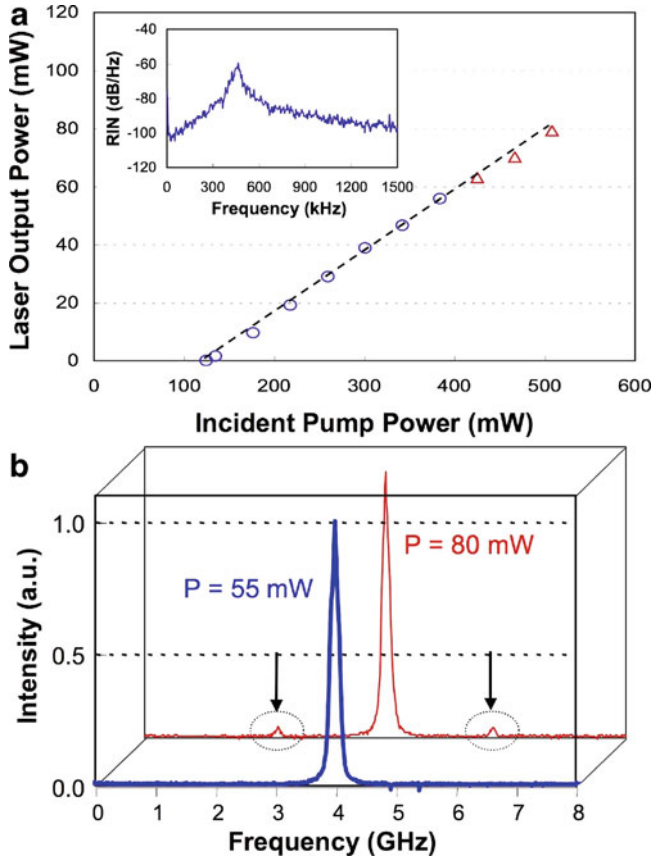
Fig. 10.8 (a) Input–output characteristic of the Er:Yb-phosphate glass ultra-compact cavity. Inset shows the RIN spectrum of the laser in single mode operation. (b) Fabry–Perot spectra at maximum output power in single mode ( circles in panel (a) ) and slightly multimodal regime ( triangles in panel (a) ). Reprinted with permission from [44]
