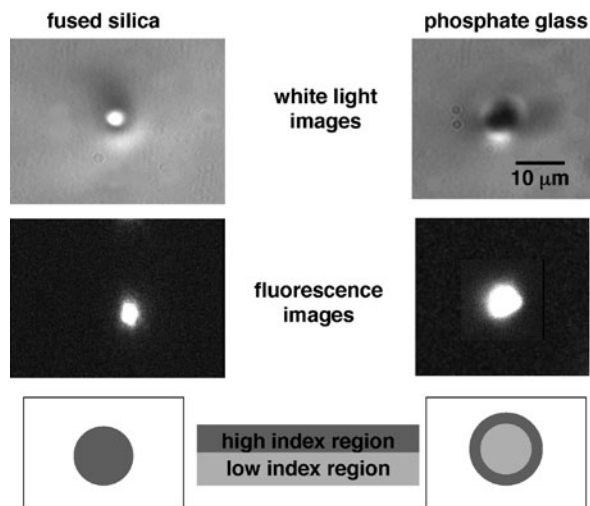
Fig. 3.13 White light ( top ) and fluorescence ( center ) images for fs-laser modified fused silica and IOG-1 glass together with an illustration of the induced index changes
