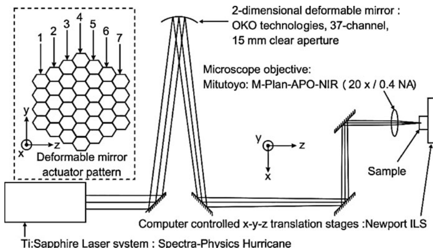
Fig. 5.14 Schematic diagram of the experimental setup used to shape waveguides using the deformable mirror technique. (Taken from [47].)
