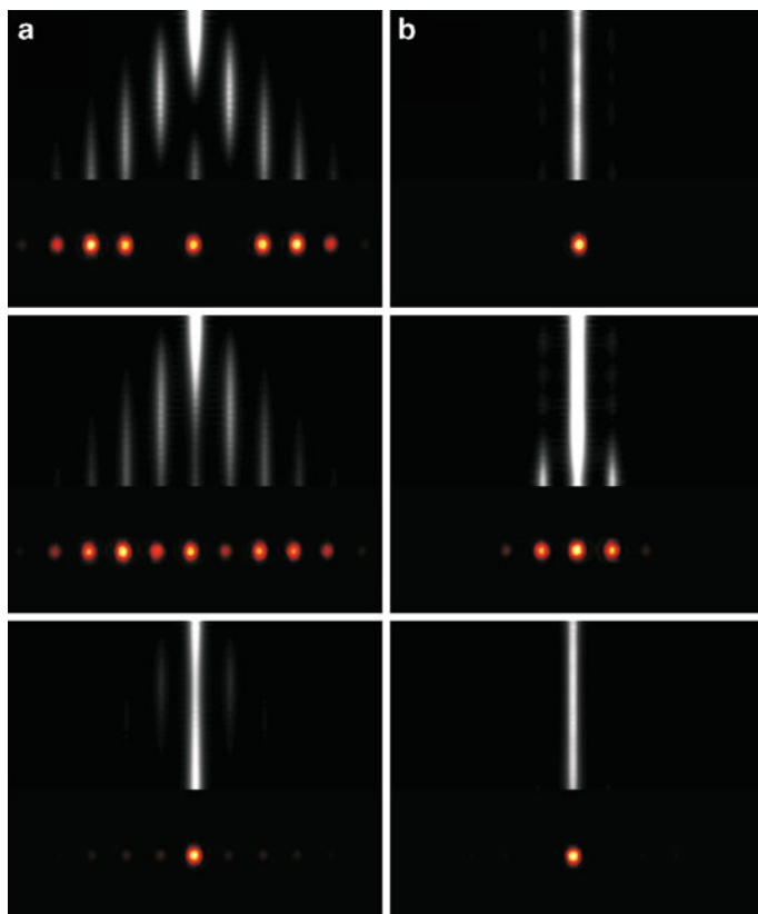
Fig. 13.31 The beam evolution at low ( first row ), medium ( second row ), and high ( third row ) input power is shown. In (a) the array is homogeneous, while in (b) the refractive index is modulated. From [76]
