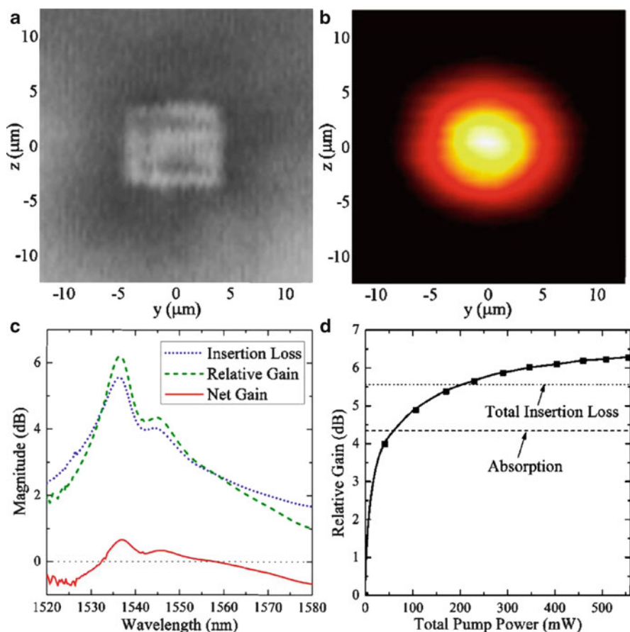
Fig. 10.5 (a) Facet image of optimal waveguide fabricated in Er:Yb-doped oxyfluoride silicate glass. (b) Near-field mode image of the waveguide. (c) Relative gain, insertion loss, and net gain spectra. (d) Relative gain vs pump power at the peak of the gain spectrum using dual wavelength pumping (62%, 980 nm; 38%, 1480 nm). Reprinted with permission from [39]
