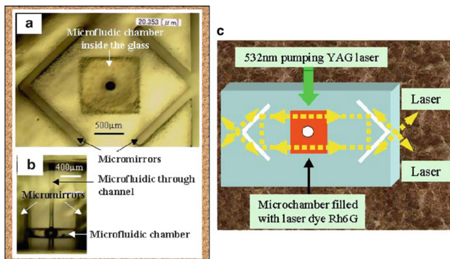
Fig. 15.13 Optical micrograph of (a) a top view and (b) a side view of a microfluidic dye laser. (c) Illustration of the optical path inside the dye laser
