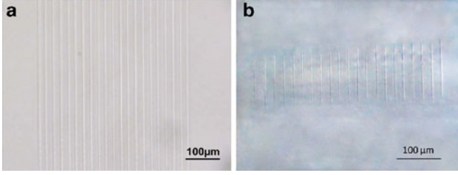
Fig. 12.17 (a) Parallel modification of PMMA with 21 diffracted beams to create a grating, scan speed 1 \text{ mm s}^{-1} and 0.6 \mu\text{J} per pulse per beam, (b) the cross-section of the RI structures showing nearly uniform modifications
