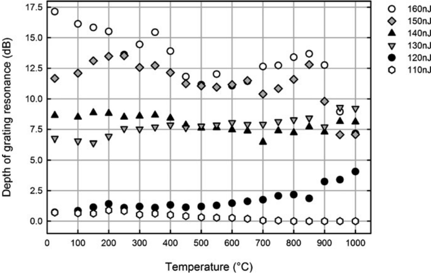
Fig. 8.7 Graph showing the evolution of the grating depth resonance for PbP gratings written with various pulse energies as a function of temperature [26]
