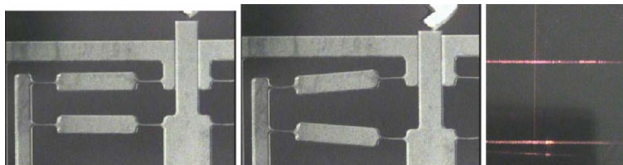
Fig. 16.24 (left and center) Hinges in deformed and non-deformed configurations Sensor prototype: optical microscope view (right), close-view of the ILE in a configuration where waveguides are all aligned
