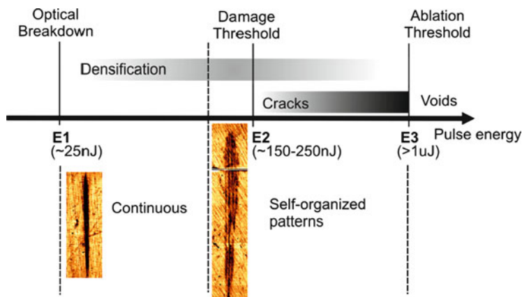
Fig. 16.3 Effect on fused silica for different pulse energies. One can distinguish three typical regimes. The effective levels of pulse energies depend on the focusing optics (numerical aperture in particular). [The order of magnitude provided for the pulse energies correspond to pulse-length of 100 fs and for an objective with a numerical aperture (NA) of 0.55.]
