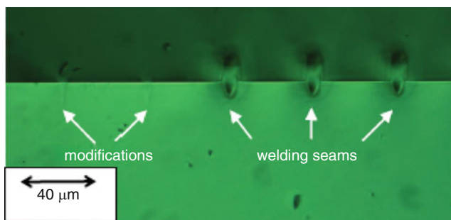
Fig. 17.9 Cross-section welding seams at the interface when welding of borosilicate glass is achieved by focused high-repetition rate ultrashort laser radiation (350 fs, 1045 nm, 1 MHz). Reprinted with permission from [20]
