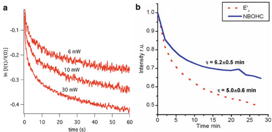
Fig. 3.10 (a) Decay of NBOHC fluorescence from modified fused silica continuously exposed to different powers of 488 nm light. (b) Decay of E and NBOHC fluorescence in fiber Bragg gratings
