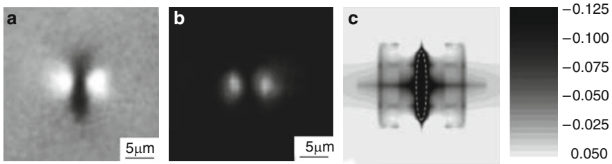
Fig. 11.1 Lines written with a pulse energy of 14\ \mu\text{J} in a quartz crystal: (a) polarization-contrast optical microscope image (end view) of the modifications; (b) near-field distribution of 514-nm radiation guided in the produced structure; (c) hydrostatic pressure distribution in a quartz matrix after a single-shot exposure according to FEM calculations (the “irradiated” ellipsoid region is marked) [4]
