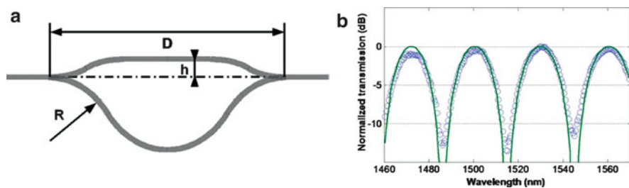
Fig. 7.29 (a) Schematic of the unbalanced MZI with h = 50 \mu\text{m} , R = 30 \text{ mm} and D = 17 \text{ mm} . (b) Open circles: measured transmission spectrum of the MZI. Solid line: least-squares fit of the experimental data [64]
