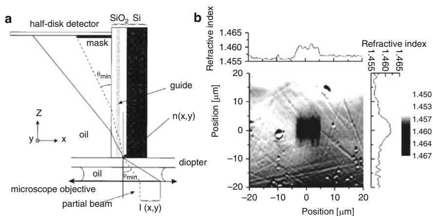
Fig. 5.3 (a) Schematic diagram of a typical refracted near-field experimental setup. (Taken from [17].) (b) Refractive index profile of an ultrafast laser inscribed waveguide whose cross-section was controlled using the multiscan technique described in Sect. 5.6.5. (Taken from [18].)
