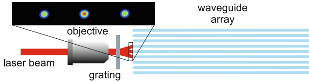
Fig. 13.6 Schematic experimental setup to excite three waveguides. The DOE is placed between focussing objective and sample, and the inset shows the focal distribution of a tri-pattern. From [46]
