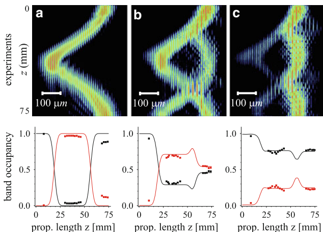
Fig. 13.20 Bloch-Zener dynamics in a curved binary waveguide array with a waveguide spacing of 11\text{ }\mu\text{m} and a curvature radius R = 1.90\text{ m} corresponding to a Bloch period of 75\text{ mm} . Upper row : fluorescence images; Lower row : measured band occupancy by integrating over the spatially separated beams corresponding to the minibands. (a) No band gap, (b) small band gap \delta\beta = 0.44\kappa , and (c) large band gap \delta\beta = 0.82\kappa . From [65]
