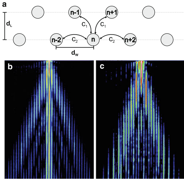
Fig. 13.8 (a) Sketch of zigzag arrangement. Fluorescence images of waveguide arrays with (b) an in-plane waveguide spacing of d_W = 24 \mu\text{m} and a layer separation d_L = 12 \mu\text{m} yielding 30% second order coupling. (c) Same as (b) but d_W = 16 \mu\text{m} , d_W = 20 \mu\text{m} and 280% second order coupling. From [50]
