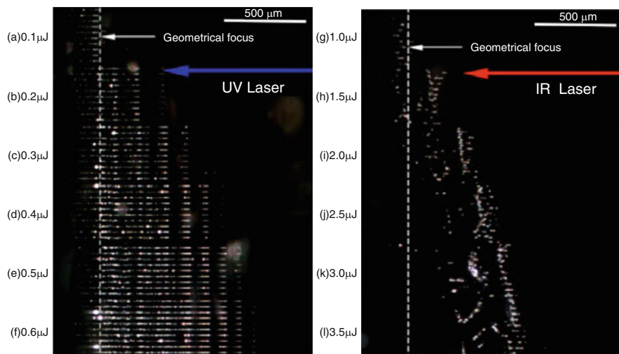
Fig. 12.15 Filamentation in PMMA with 160 fs, 775 nm (right) and 387 nm (left) pulses focused with NA \sim 0.15 . Note the difference in pulse energies and the highly periodic structuring at 387 nm. Exposure time t = 0.5 s (500 pulses). Light scattering shows that there is also dielectric breakdown at higher pulses energies
