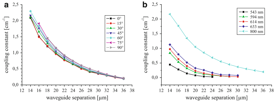
Fig. 13.3 Measurements of coupling constants dependent on the waveguide separation for (a) different angular orientations and (b) different wavelengths [38]
