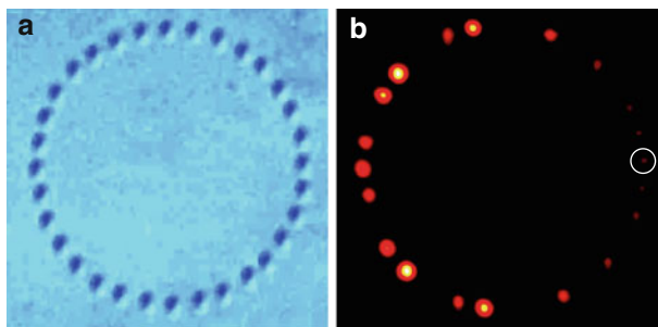
Fig. 13.14 Quasi infinite planar waveguide array with circular geometry, containing 32 waveguides and with a diameter of 286\text{ }\mu\text{m} . (a) Microscopy image and (b) propagation pattern for an excitation wavelength of 633\text{ nm} [38]. White circle indicates coupling location
