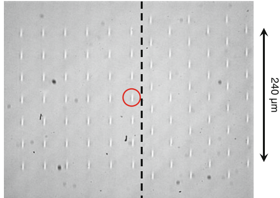
Fig. 13.34 Microscope image of a waveguide array exhibiting two different regions with square (left) and hexagonal (right) topology. The waveguide excited in the experiments (see Fig. 13.35) is marked with a red circle . From [80]
