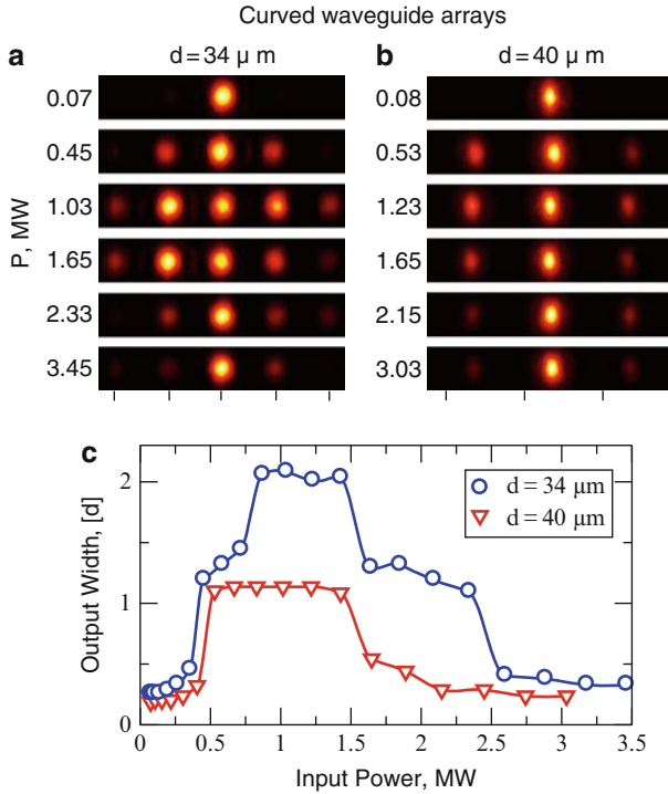
Fig. 13.29 Comparison of the evolution of the output beam broadening between the experimental (a) strong and (b) weak coupling. (c) The output width is shown as a function of the input peak power. From [75]
