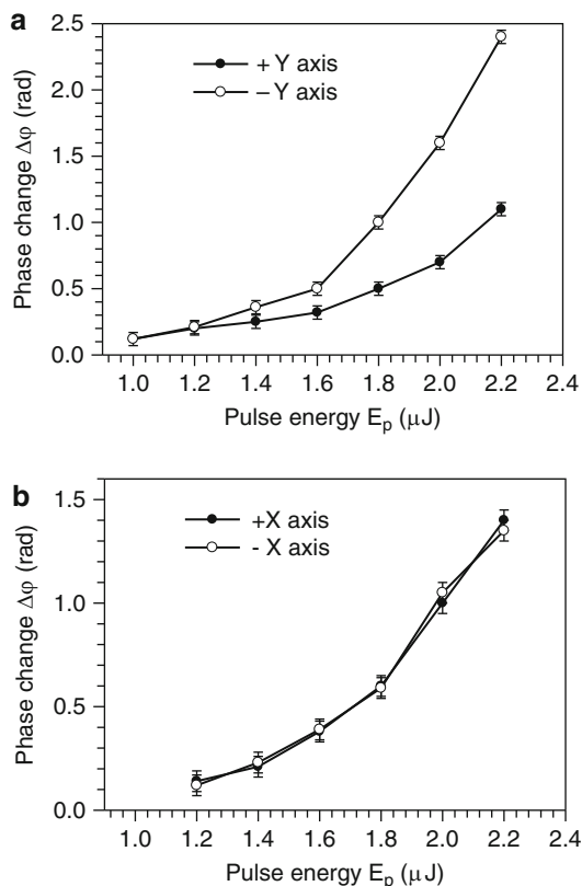
Fig. 6.11 Comparison of the line structures imprinted along the Y axis and along the X axis. (a, b) Measured phase change of the line structures versus pulse energies for the lines written along the Y axis of the LiNbO 3 sample (a) and the X axis of the LiNbO 3 sample (b). The error bar is due to the variation in phase value for the unexposed region of the LiNbO 3 sample
