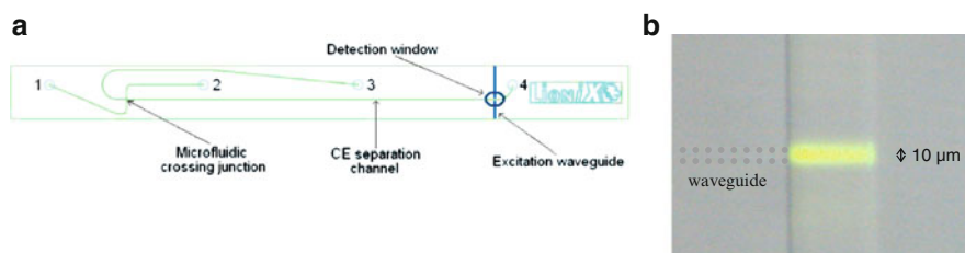
Fig. 14.9 (a) Schematic of the MCE device. The line connecting the four reservoirs represent microfluidic channel fabricated by standard technologies, whereas the vertical thick line represents an optical waveguide inscribed by femtosecond laser and providing the fluorescence excitation source; (b) microscope image of the fluorescence excited in the microchannel by an optical waveguide [49]
