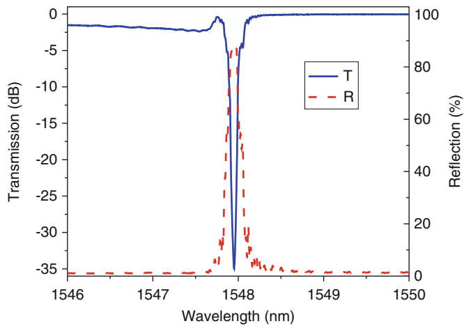
Fig. 9.13 The transmission and reflection spectra of the BGW written in fused silica with 60% AOM modulation duty cycle. The laser repetition rate was 500 kHz and AOM modulation frequency was 500 Hz. The grating strength is 35 dB and the maximum reflection is ~90%
