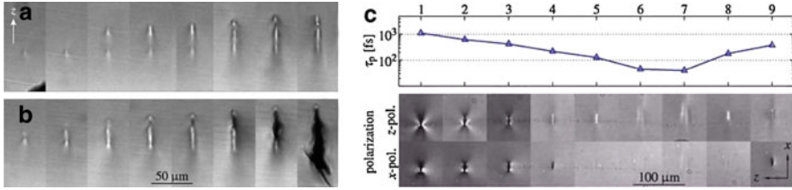
Fig. 11.3 Transmission microscope images of the end facet of z-cut LiNbO 3 illuminated with z-polarized light. The pulse duration was (a) 130 fs and (b) 420 fs. Pulse energies were 0.2, 0.3, 0.4, 0.5, 0.6, 1, 3, and 4.5 μJ from left to right. The writing laser was incident from the bottom. Bright and dark regions correspond to extraordinary index increases and decreases, respectively [6]. (c) Influence of the pulse duration \tau_p on the waveguide properties in x-cut LiNbO 3 . Shown are transmission microscope images for z- or x-polarized light. The minimum pulse duration was 40 fs while the pulse energy was 0.2 μJ for all structures; the same results were obtained for negatively and positively chirped pulses. The writing laser was incident from the bottom [6]
