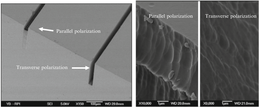
Fig. 16.8 Effect of polarization: the left photograph shows two trenches etched with the same energy and writing speed parameters but with two different polarizations. Detailed views of the wall morphology are shown on the right
