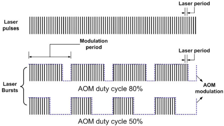
Fig. 9.11 AOM modulation for burst generation. The continuous high-repetition rate laser pulses ( top ) were modulated by the AOM with a square waveform ( dotted envelopes in middle and bottom rows ) generating a series of laser pulse bursts. The modulation frequency and duty cycle were controlled by an external function generator
