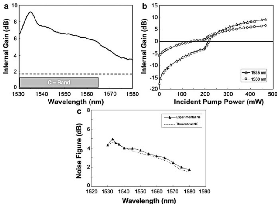
Fig. 10.4 (a) Measured internal gain spectrum obtained with an incident pump power of 460 mW in bi-directional pumping configuration. The dashed line indicates the total insertion losses. (b) Internal gain of the 37-mm long Er-Yb waveguide amplifier as a function of the incident pump power for two different signal wavelengths: 1535 nm ( triangles ) and 1550 nm ( circles ). (c) Experimental ( triangles ) and theoretical ( dotted line ) noise figure. Reprinted with permission from [34]
