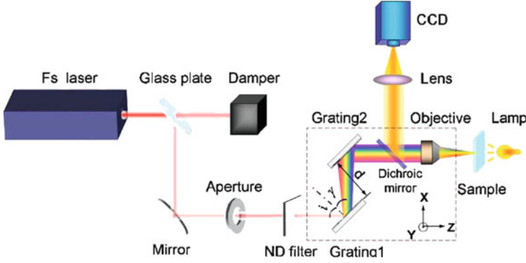
Fig. 5.18 Schematic diagram of the experimental setup used by He et al. for spatiotemporal focussing. (Taken from [49].)
