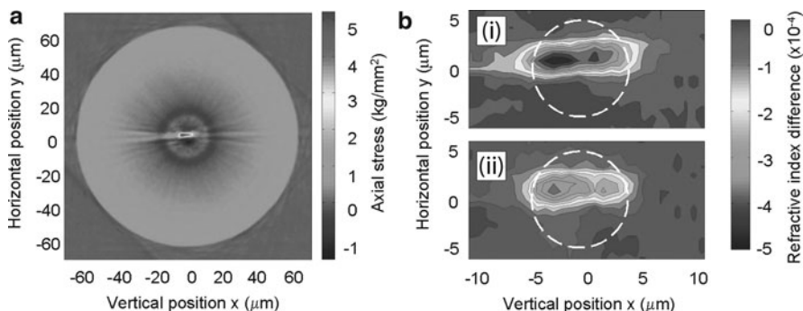
Fig. 8.9 (a) Axial stress profile of a femtosecond modification in SMF-28 fibre. (b) Stress-induced change for the x (i) and y (ii) component of the refractive index contrast. The dotted circles indicate the core of the fibre [51]
