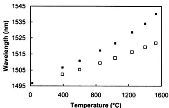
Fig. 8.13 Variation of Bragg resonance in sapphire fibre grating with temperature. Black squares are the measured \lambda_{\text{FBG}} as a function of temperature while the white squares are the calculated \lambda_{\text{FBG}} based on pitch variation resulting from fibre elongation [11]
