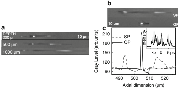
Fig. 4.5 (a) PCM images of static permanent structures induced by a single short pulse (SP) in bulk irradiated \alpha -SiO 2 for various working depths (NA=0.45). The elongation of the focal region becomes visible, increasing with the processing depth. Irradiation parameters: 160 fs and 1 \mu J for 800 nm radiation wavelength. (b) Short pulse (SP) and optimal pulse (OP) induced structures at a depth of 500 \mu m and 1 \mu J input energy indicating the spatial confinement of the OP structure even in the presence of aberrations. (c) The corresponding axial cross-sections of the resultant index patterns. The inset shows the optimal pulse shape [64]
