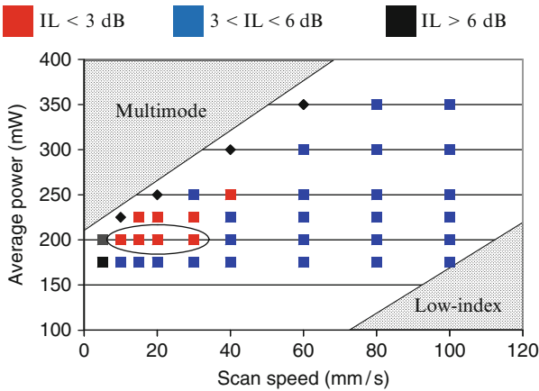
Fig. 7.8 Processing window map: waveguide properties as a function of average power and scan speed for 1.5-MHz repetition rate [10]
