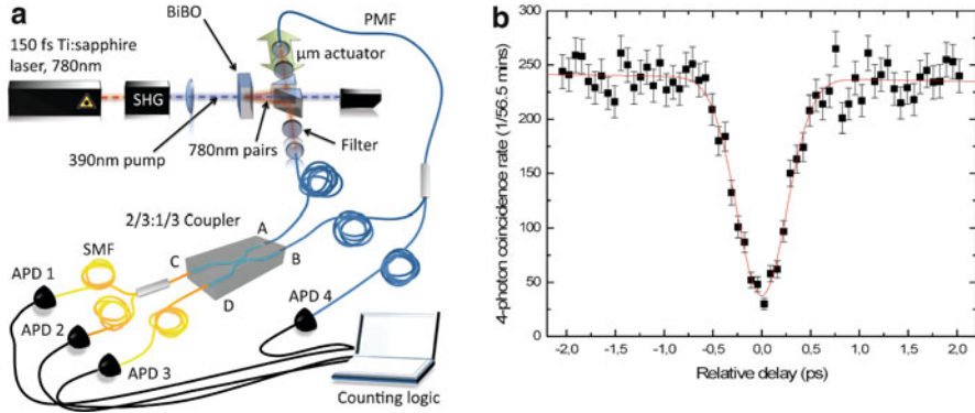
Fig. 7.19 Quantum interference with three photons. (a) Measurement setup with spontaneous parametric down conversion source based on frequency doubled Ti:Sapphire femtosecond oscillator. (b) The number of coincident detections are shown as a function of the arrival delay between two interfering photons with an observed interference dip for three photons [48]
