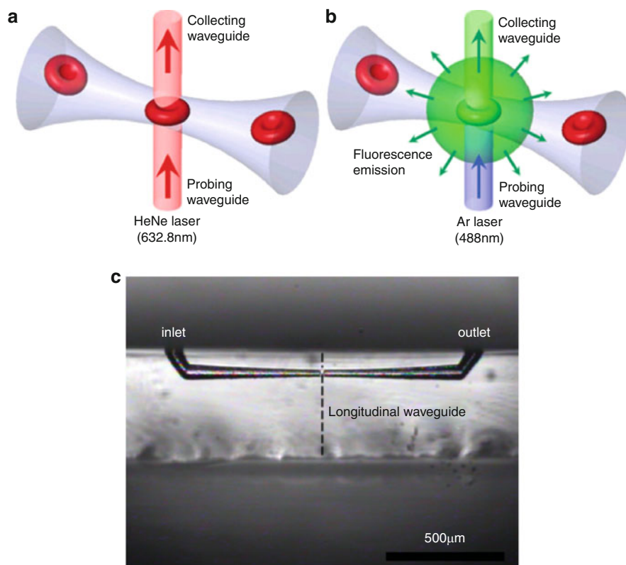
Fig. 14.14 Schematic of the integrated cell detection using (a) light transmission and (b) fluorescence. (c) Microscope image of the actual device [62]
