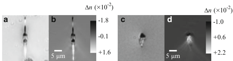
Fig. 7.11 Cross sectional microscope images (a,c) and refracted near field profiles (b,d) of optimum waveguides fabricated with 0.55-NA (a,b) and 1.25-NA (c,d) objectives. The writing laser was incident from the top [35]
