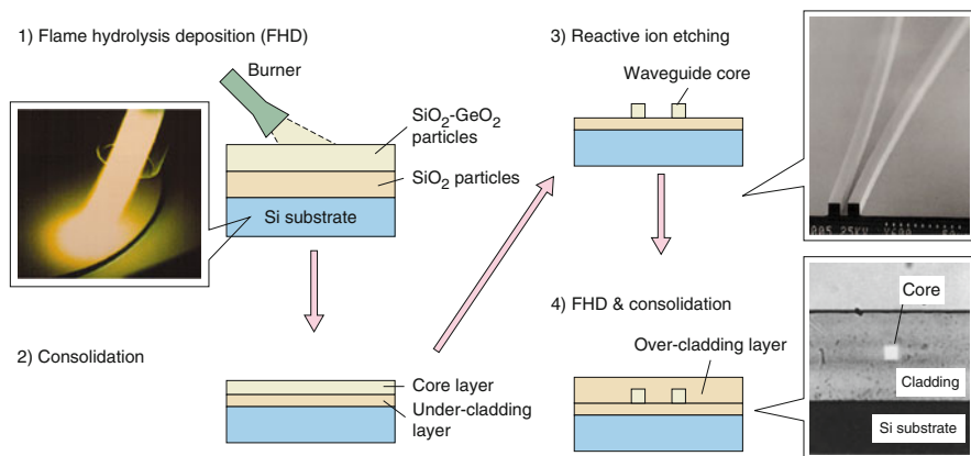
Fig. 7.1 Fabrication steps in flame hydrolysis method for producing planar lightwave circuits in glass [1]
