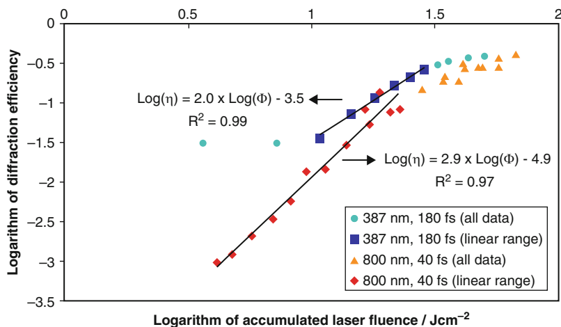
Fig. 12.11 Determination of the order of the photomodification process in pure PMMA for 800 nm, 40 fs, and 387 nm, 180 fs by plotting photoreaction yield versus integrated fluence; line gradients of 2.9 and 2.0 indicate three- and two-photon absorption at 800 nm and 387 nm, respectively [38]
