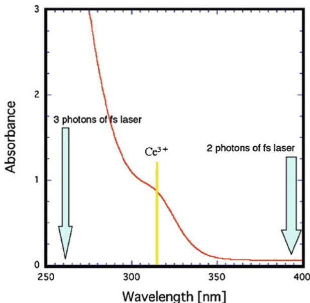
Fig. 15.1 Absorption spectrum of a typical photosensitive glass (Foturan) between 250 and 400 nm in wavelength
