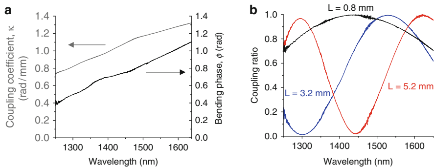
Fig. 7.25 (a) Coupling coefficient and bending phase versus wavelength for a directional coupler with separation of d = 10\mu\text{m} . (b) Measured coupling ratio versus wavelength for separation of d = 10\mu\text{m} and interaction lengths of L = 0.8, 3.2 , and 5.2 mm [54]
