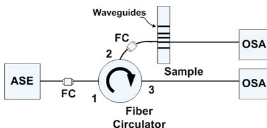
Fig. 9.5 Spectral response arrangement of BGWs. The broadband light from an ASE is guided to the waveguide by the fiber circulator which also routed the waveguide reflection signal. An OSA was used to analyze both the transmitted and reflected light. FC: fiber connector; OSA: optical spectrum analyzer; and ASE: broadband light source
