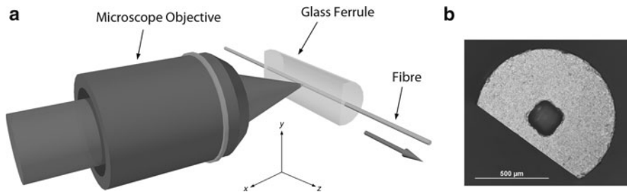
Fig. 8.2 (a) PbP grating fabrication incorporating a fixed glass ferrule and translating fibre configuration. (b) Micrograph of a D-shaped glass ferrule
