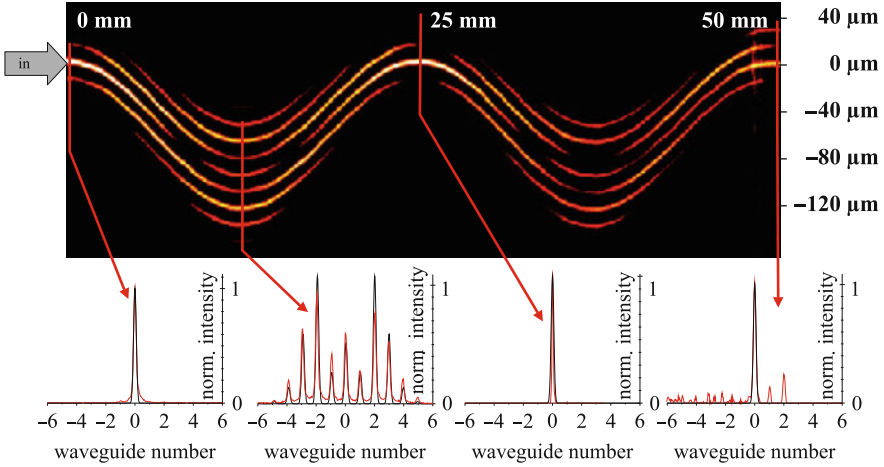
Fig. 13.16 Dynamic localization: Fluorescence image with two periods of 25 mm and a full amplitude of 95\ \mu\text{m} satisfying the dynamic localization condition for 633 nm. The waveguide spacing is 14\ \mu\text{m} resulting in a coupling constant \kappa = 0.185\ \text{mm}^{-1} . Additional cross sections are plotted for selected propagation distances ( red lines ) and compared to solutions of the coupled mode equations ( black lines ). From [47]
