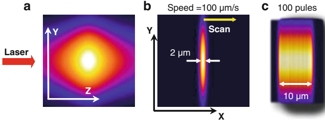
Fig. 2.11 (a and b) Sketch of the calculated cross sections of the beam intensity distribution in the focal region for a beam shaped with a slit. The sample is scanned along the X -direction. The propagation axis is taken as Z while the slit short axis is taken as Y . The beam (800 nm, 1 kHz rep. rate, 7.4 mm ( 1/e^2 ) diameter) passes through a 350 \mu\text{m} slit before being focused with a 0.26 NA lens. The material refractive index used in the calculation is n = 1.56 and the processing depth is d = 1.56 mm. Intensity cross sections are shown along the Y-Z plane (a) and Y-X (b) plane. During the writing procedure the sample scanning speed is 100 \mu\text{m s}^{-1} . (c) Shows schematically the Y-X cross section of the volume affected by 100 pulses during the scan
