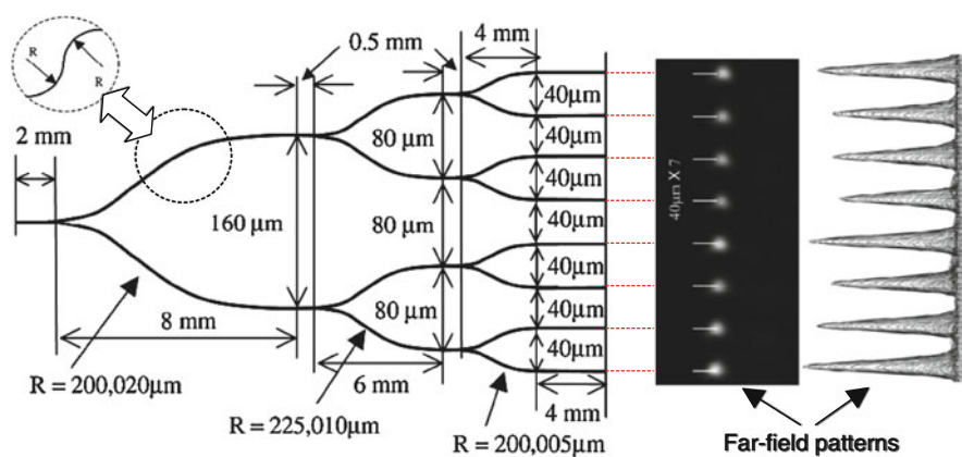
Fig. 7.14 Schematic design diagrams of a 1 \times 8 optical waveguide power splitter and near-field patterns [40, 41]
