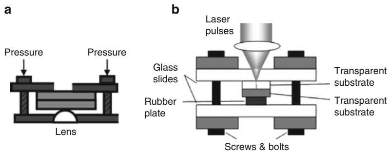
Fig. 17.3 Schematic of the fixture for holding samples to be joined. (a) Fixing of two substrates using sample holder and a pressing lens. (b) Fixing of two substrates using rubber plate
