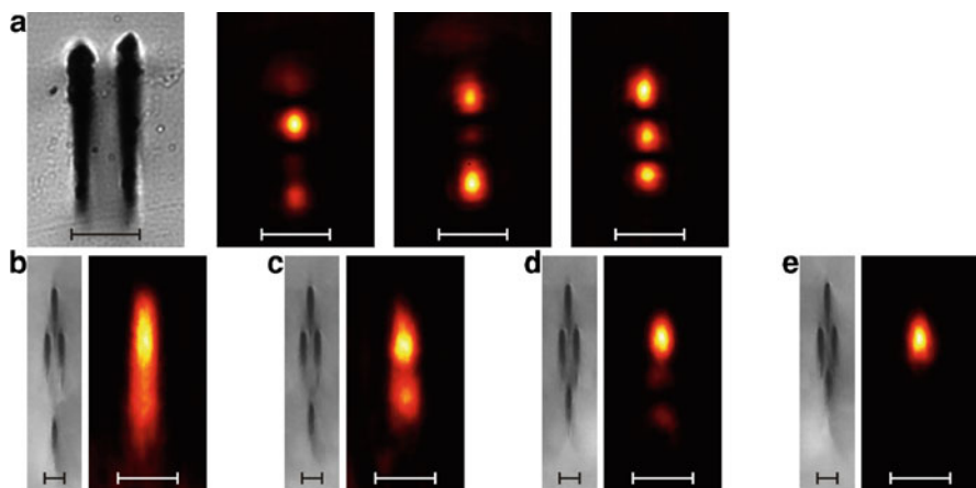
Fig. 11.6 Type II waveguides in BBO [14]. (a) Dual line geometry ( left : microscope image) supporting multiple vertical modes ( right ) at a wavelength of 633 nm. (b–e) Improved vertical confinement in various quad line geometries. All scale bars indicate 20 \mu\text{m}
