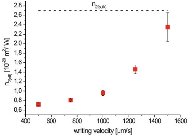
Fig. 13.23 Dependence of the effective nonlinear refractive index n_{2(eff)} on the writing velocity for fixed pulse duration of 150 fs and pulse energies of 0.3 \mu\text{J} . From [39]
