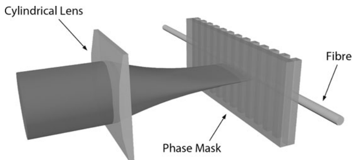
Fig. 8.4 Phase mask writing technique
