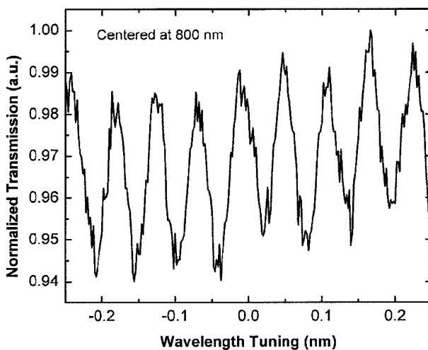
Fig. 7.32 Normalized transfer function of the ring resonator. The fringe spacing of 57 pm at 800 nm concurs with the 58-pm calculated for a ring length of 7.3 mm [67]
