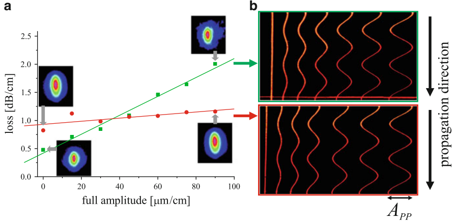
Fig. 13.15 (a) Curvature losses for waveguides written with 0.22 \mu\text{J} (green line) and 0.28 \mu\text{J} (red line) gained from (b) fluorescence images. From [47]
