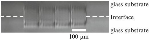
Fig. 17.6 Microscopic optical image of side view after ultrashort laser joining with pulse energy of 1.0 μJ and a translation velocity of 0.1 mm/s in borosilicate glass
