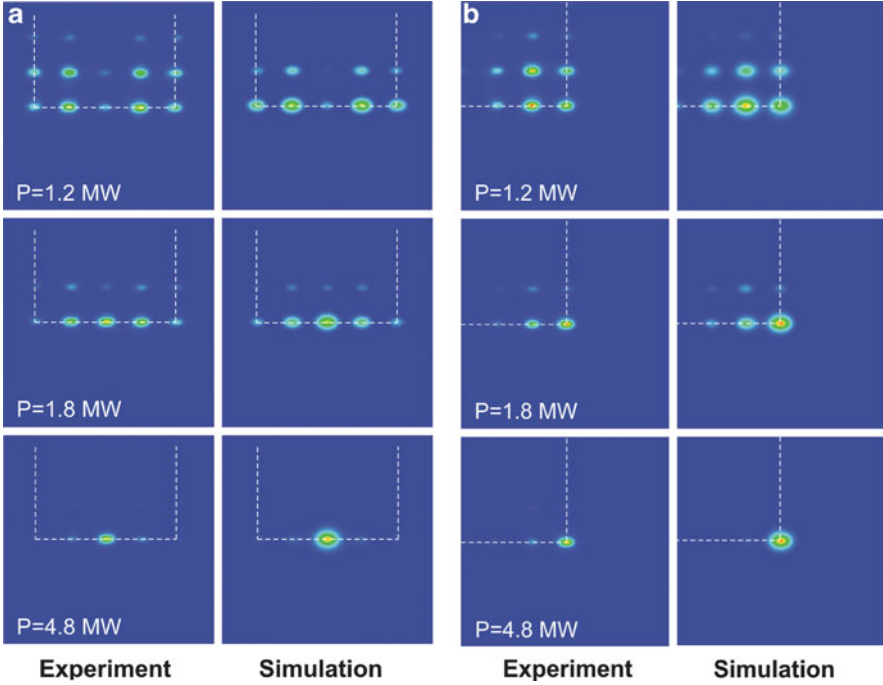
Fig. 13.33 (a) Excitation of a surface wave in the central waveguide of the first array row. (b) Excitation of a surface wave in the corner waveguide of the array. The dashed lines indicate the array surfaces position. From [79]
