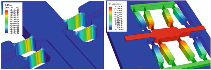
Fig. 16.19 FEM analysis – stress distribution in four hinges ( left ) and displacement distribution of the entire structure ( right )
