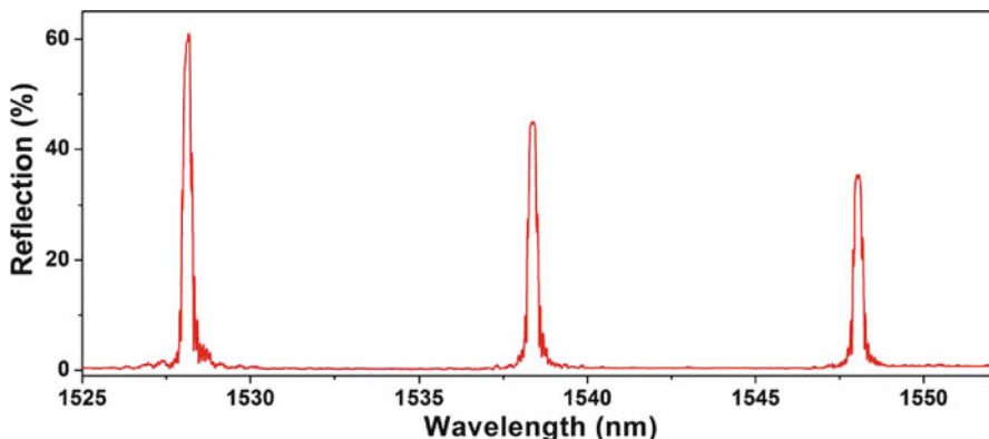
Fig. 9.25 Reflection spectrum of BGW segments H1, H2, and H3 (left to right)
