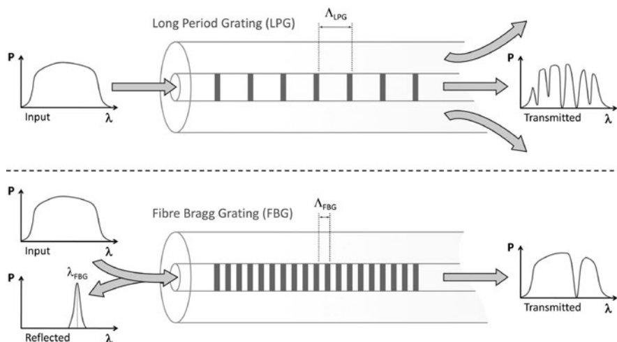
Fig. 8.1 Schematic of a (top) long period grating and (bottom) fibre Bragg grating
