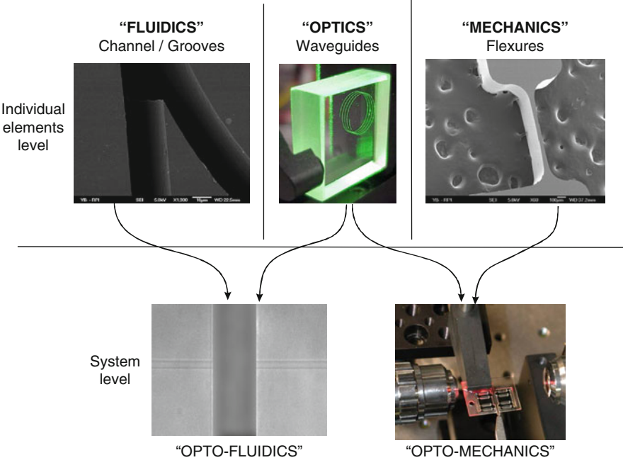
Fig. 16.14 Monolithic system integration by combining individual elements
