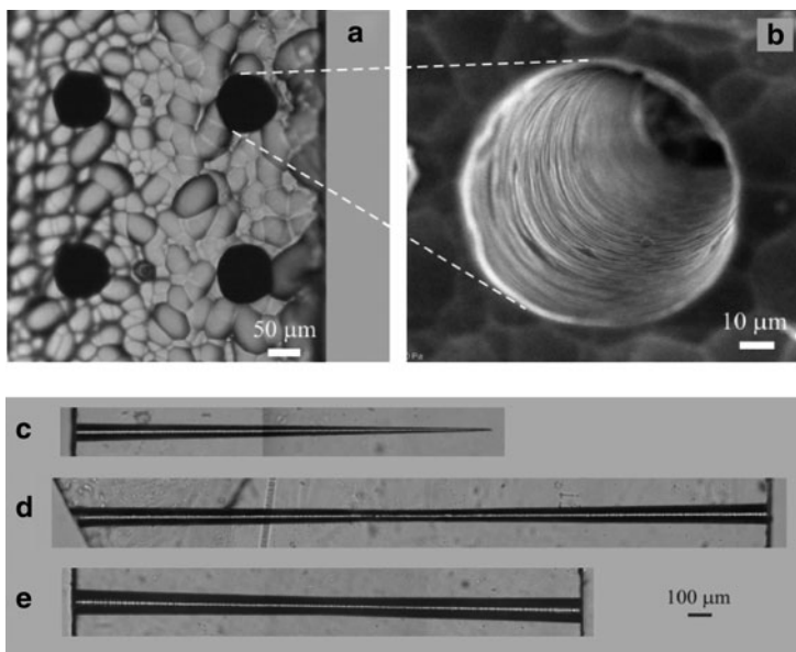
Fig. 14.2 (a) End-face microscope image of a 2 \times 2 matrix of microchannels; (b) SEM image of one channel; (c) top view of a dead-end microchannel; (d) and (e) top views of two-side etched microchannels with different degrees of overlap
