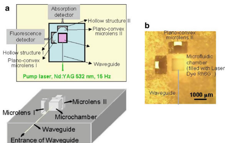
Fig. 15.15 (a) 2D and 3D configurations and (b) optical microscope image of two plano-convex lenses and an optical waveguide integrated with a microfluidic chamber in a single glass chip. The solid gray line in panel (b) marks the location of the invisible waveguide inside the glass
