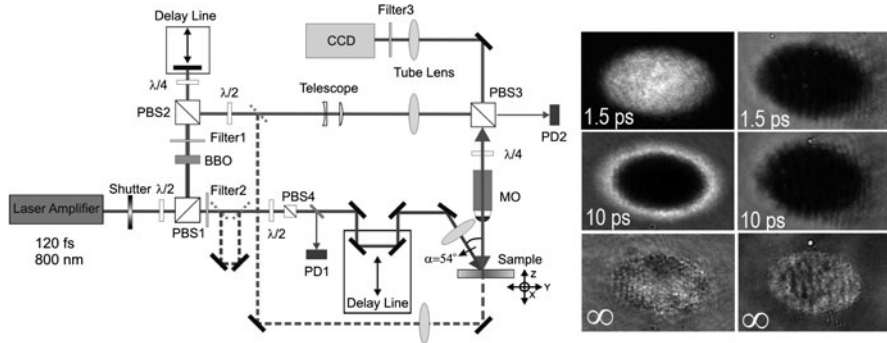
Fig. 2.5 Taken from [37]. Left : femtosecond dual-mode pump-probe microscope. The reflection mode is drawn with solid lines, the transmission mode with dashed lines. A polarizing beamsplitter (PBS1) reflects a small fraction of the pump beam (800 nm, approximately 100 fs) to generate the probe beam, which is then frequency-doubled to 400 nm. Right set of frames : Time-resolved surface reflectivity ( left column ) and transmission ( right column ) images recorded for fused silica at different delay times (see labels) after exposure to a pump pulse with a peak fluence of 11.9 \text{ J cm}^{-2} , above the ablation threshold
