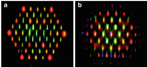
Fig. 13.12 Hexagonal waveguide arrays with spacings of (a) 16 \mu\text{m} and (b) 20 \mu\text{m} illuminated with white light and recorded with a color CCD camera. From [54]
