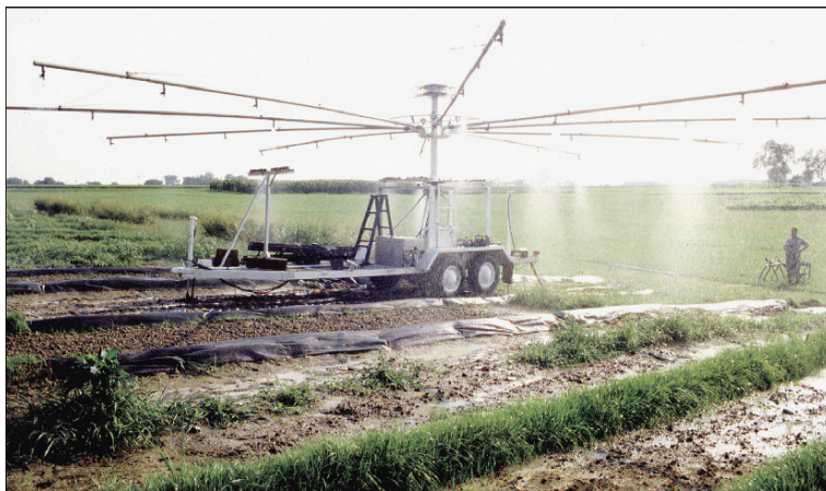
Plate 9 The Swanson type rotating boom rainfall simulator (Photo by H. Blanco). The simulator booms are equipped with nozzles positioned at radii of 1.5, 3.0, 4.5, 6.0, and 7.6 m. Booms and nozzles rotate in a circle, and the wetted diameter is about 16 m
