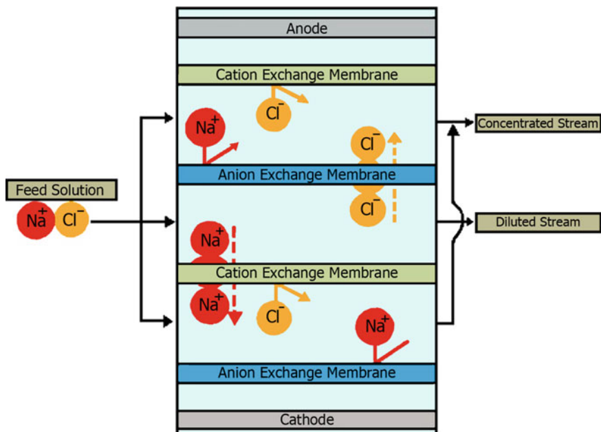
Fig. 3.1 Principle of the desalination process by Electrodesalination
