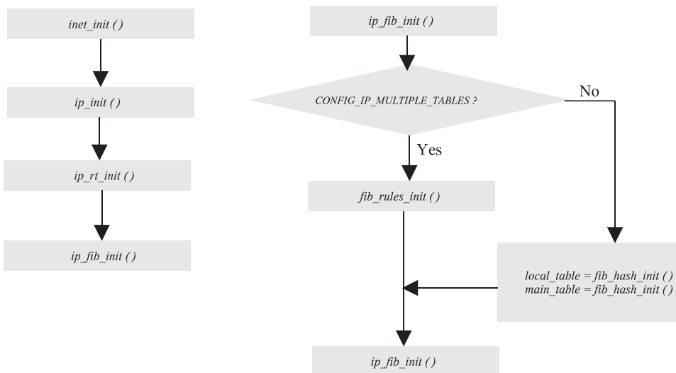
Figure 14.15. FIB initialization flow diagram.
