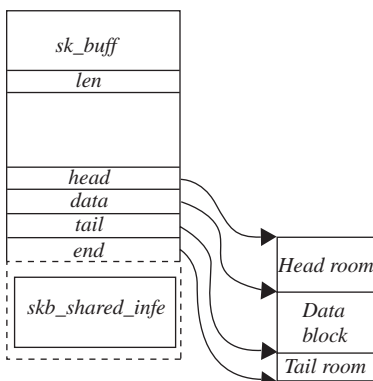
Figure 1.1. Network buffer, sk_buff .
