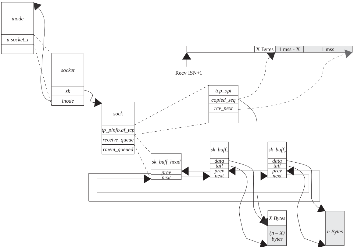
Figure 8.2. X bytes copied to the application buffer.
