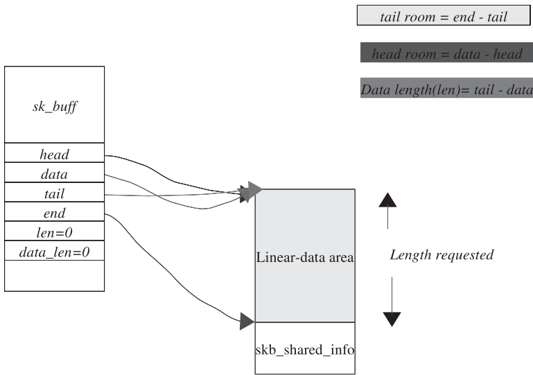
Figure 5.6. Status of sk_buff after it is allocated.
