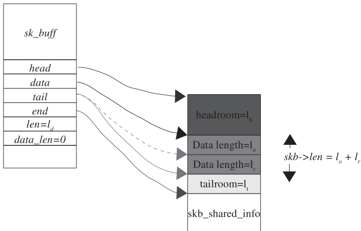
Figure 5.8. Status of sk_buff after call to skb_put() .
