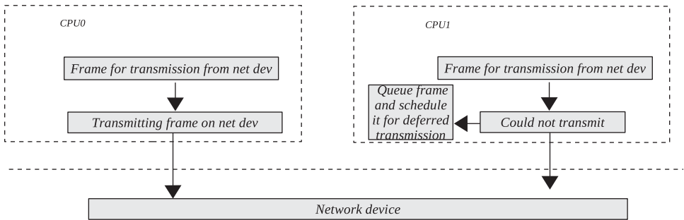
Figure 17.1. Tx net softIRQ.
