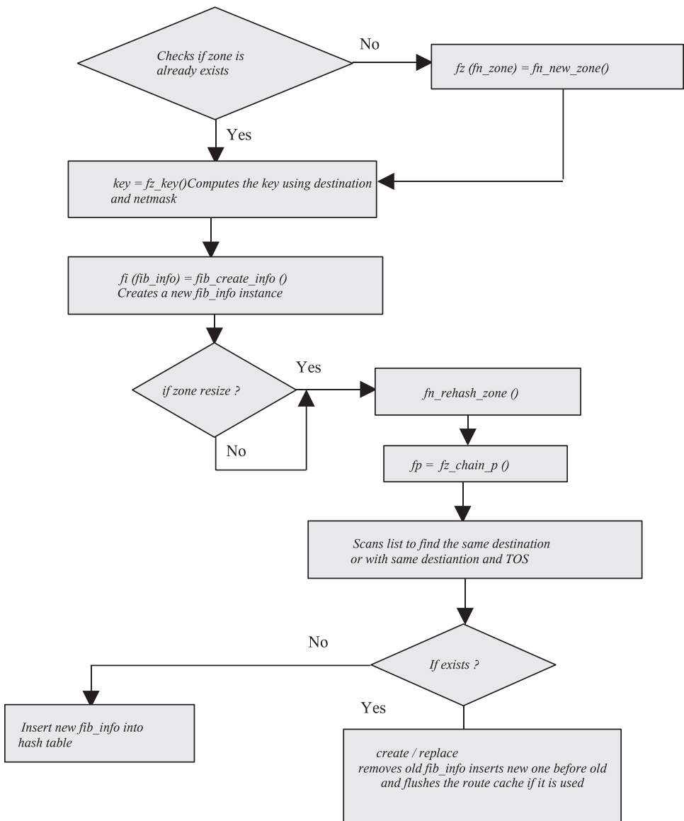
Figure 14.14. fn_hash_insert () flow.
