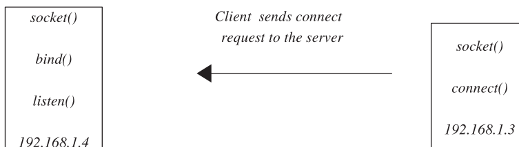
Figure 4.14a. Client generates connection request for nonaccepting listening sockets.
