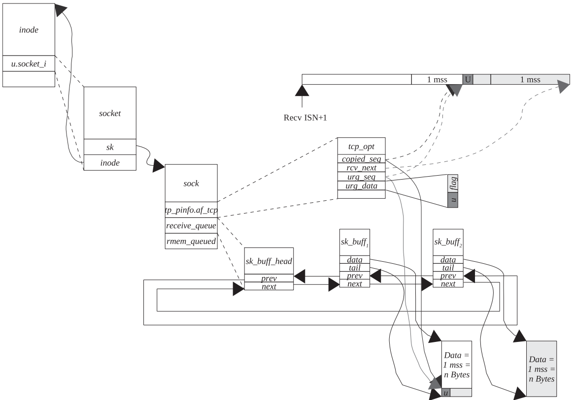
Figure 8.12. Application is returned data until an urgent pointer.
