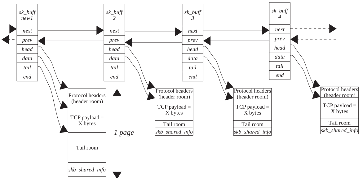
Figure 9.4. The new buffer is allocated and the first buffer is copied to the new buffer.
