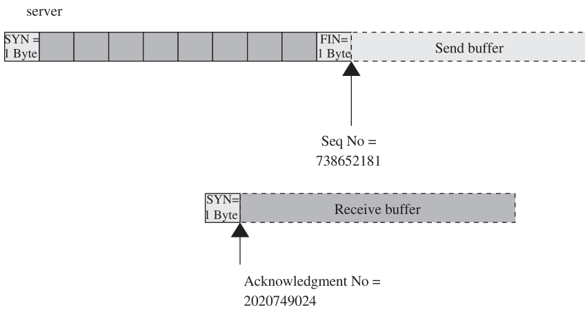
Figure 2.17f. FIN sent by the server.
