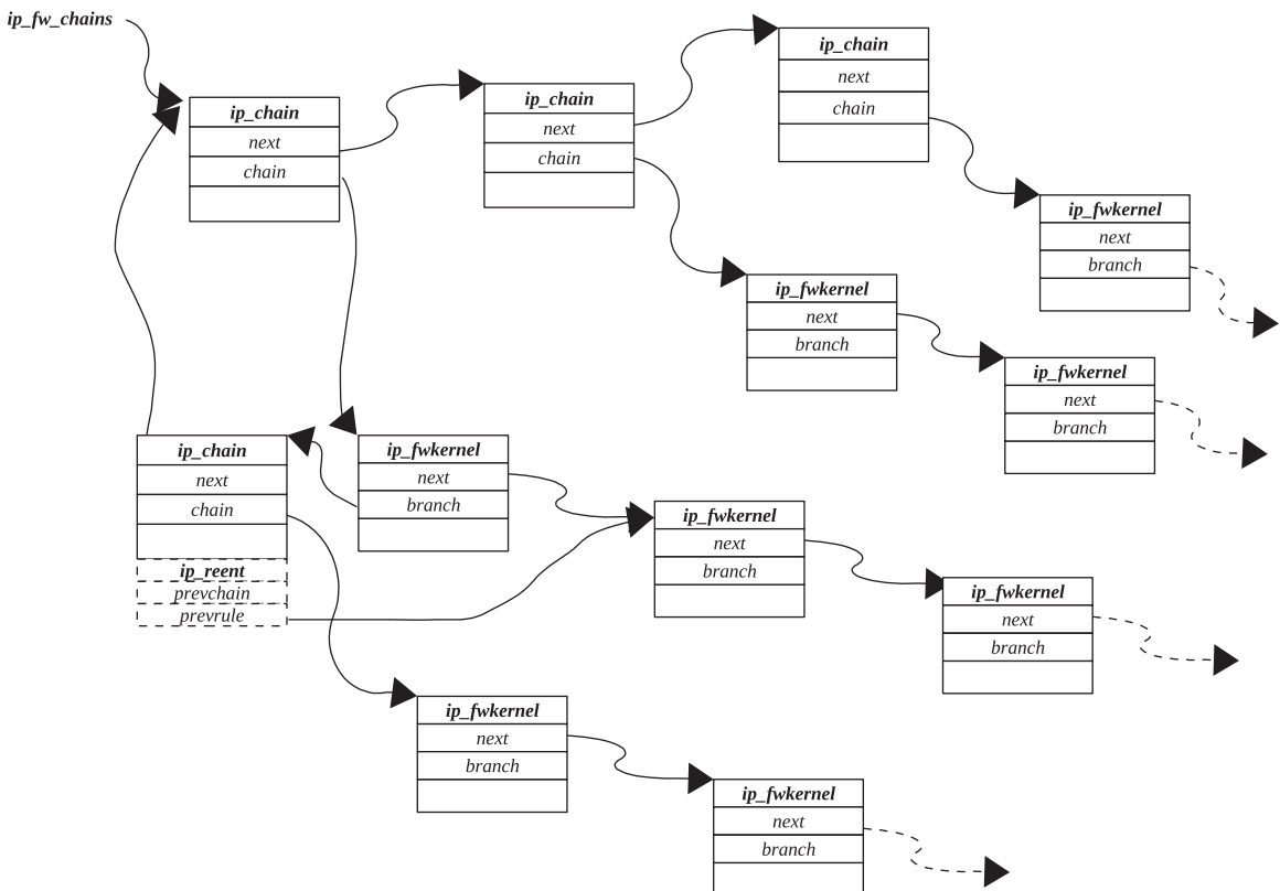
Figure 16.3. Ipchains filter rules and chains.
