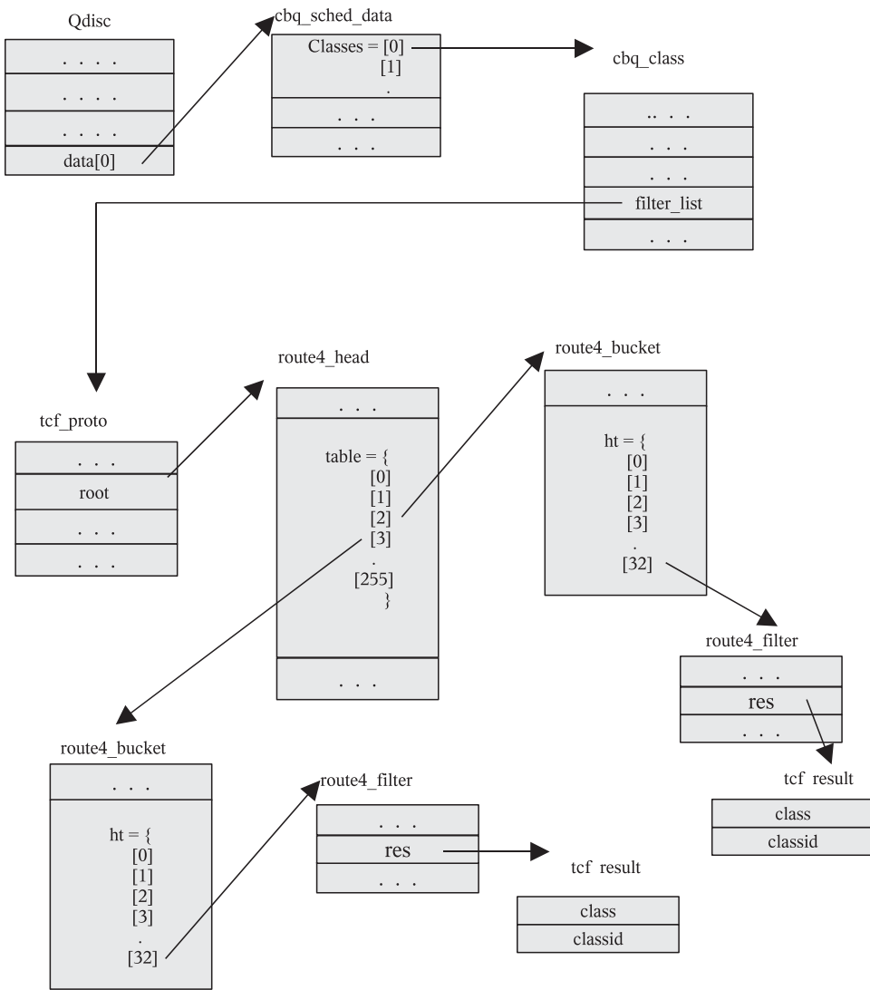
Figure 15.11. Route filter implementation overview.
