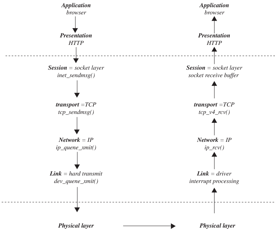
Figure 1.4. Linux network stack and OSI model.
