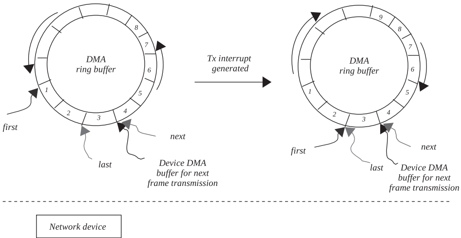
Figure 18.9. Tx interrupt generated and two buffers in the Tx ring buffer and freed from the ring.
