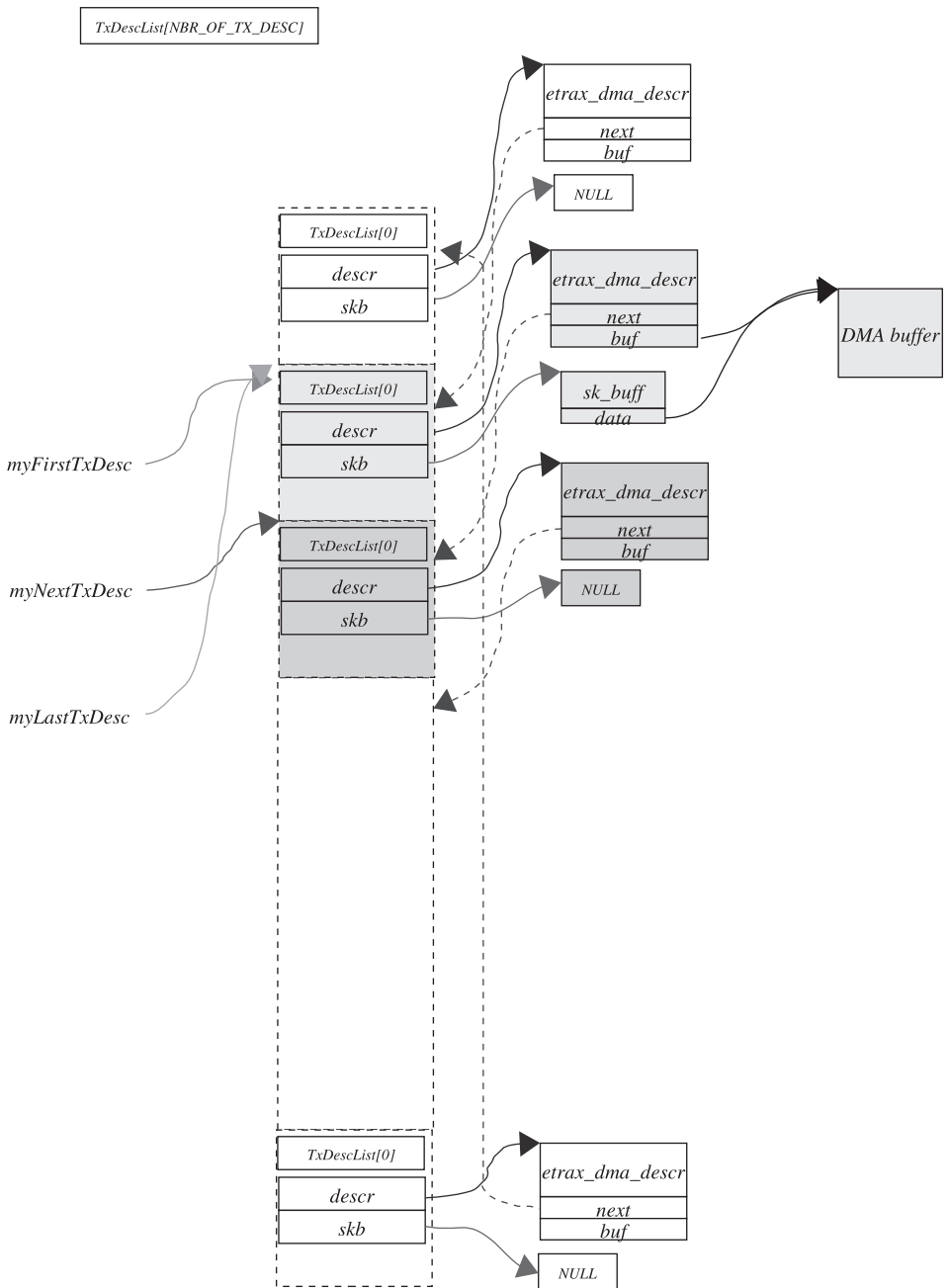
Figure 18.16. Tx interrupt is generated and the first packet on the Tx ring buffer is freed.
