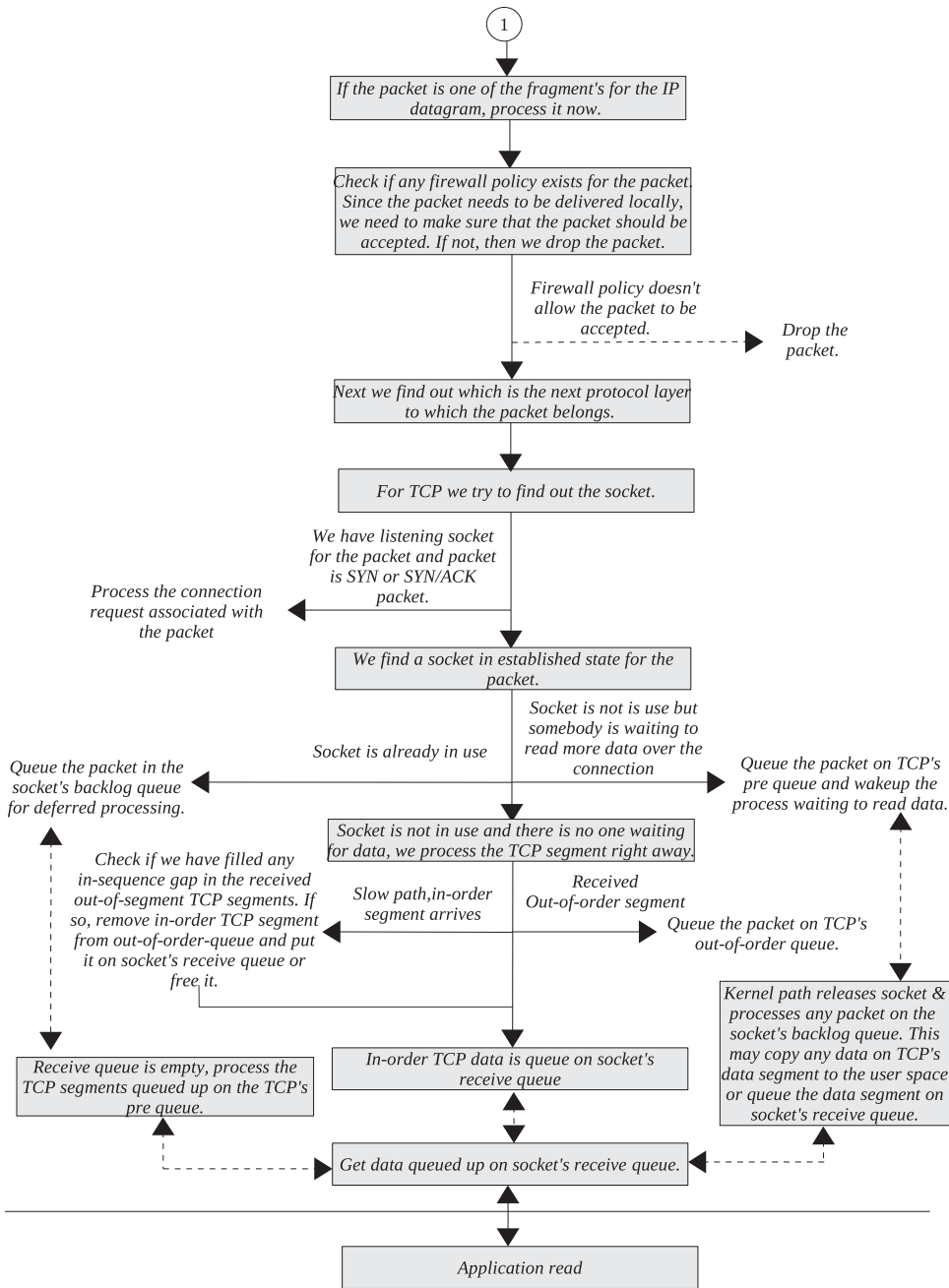
Figure 6.4b. Traversal of a packet up the TCP/IP stack (continued).
