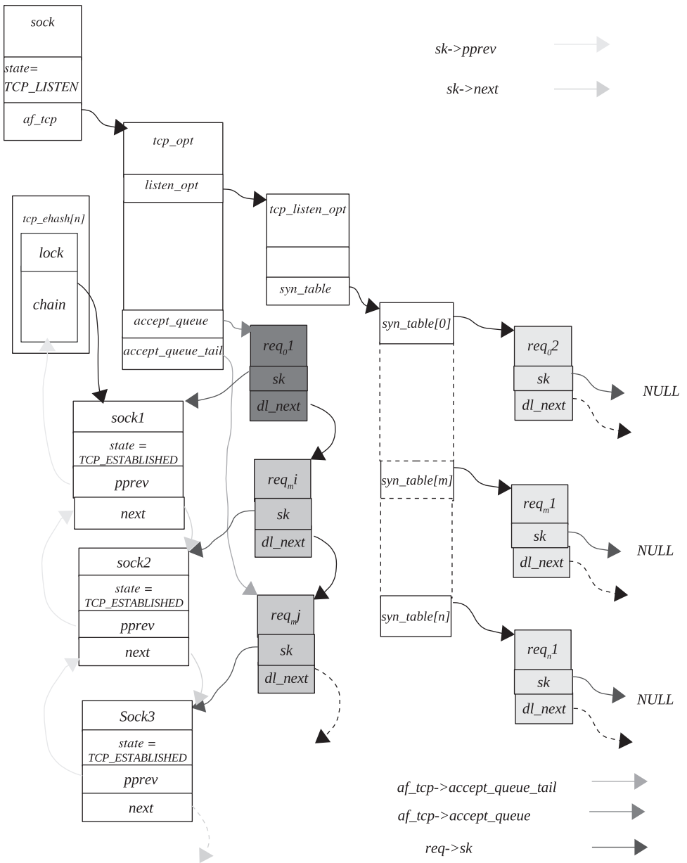
Figure 4.18. Connection request converted into established socket and placed in to accept queue after the three-way handshake is over.
