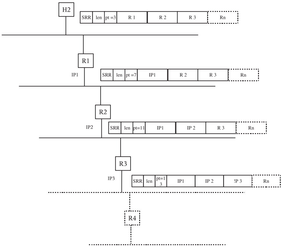
Figure 14.9. Packet with SRR IP option being modified as it emerges from each router interface.
