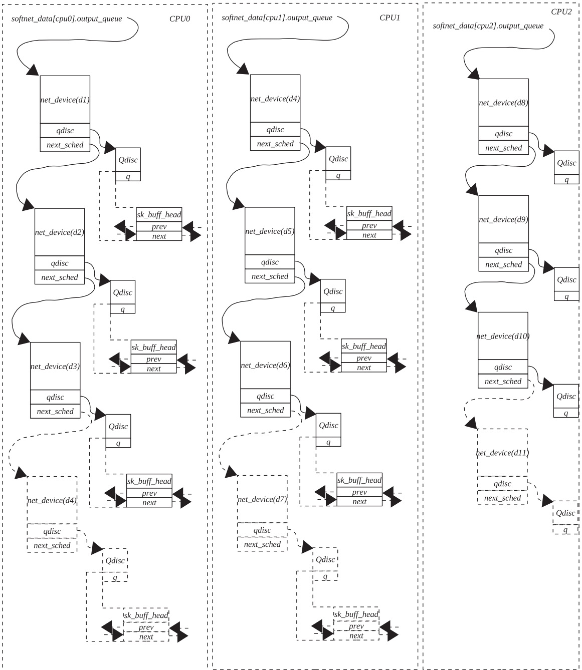
Figure 17.9. Packets being transmitted from different devices using Tx softIRQ framework on SMP machine.
