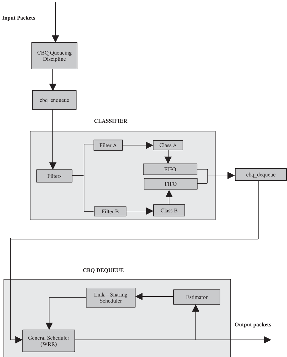
Figure 15.14. CBQ block diagram.
