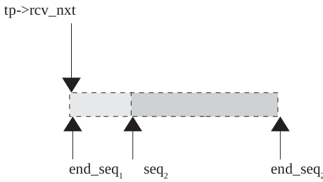
Figure 11.31. Sequence space after shuffling of a segment from an out-of-order queue to a receive queue.
