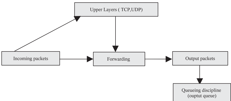
Figure 15.1. Block diagram of Linux traffic control.
