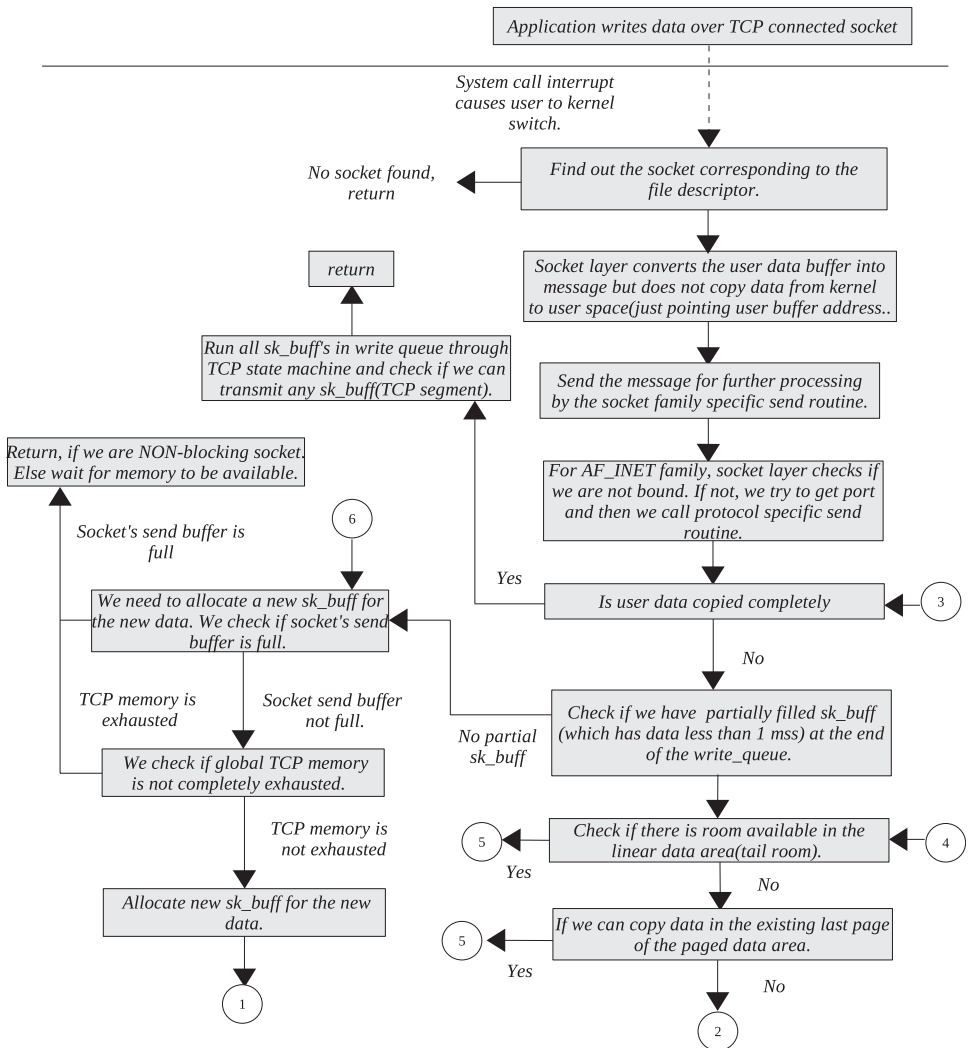
Figure 7.5a. Data flow of the TCP send process.
