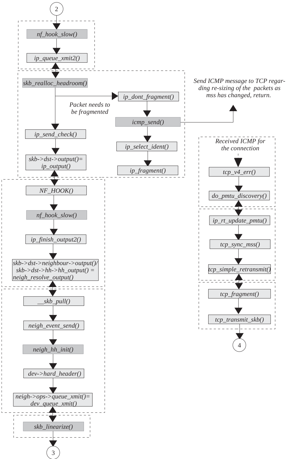
Figure 6.3b. Flow of packet down a TCP/IP stack in kernel 2.4.20 (continued).
