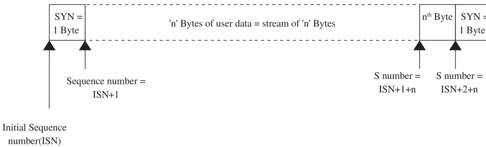
Figure 2.15. TCP sequence number association with stream of bytes.
