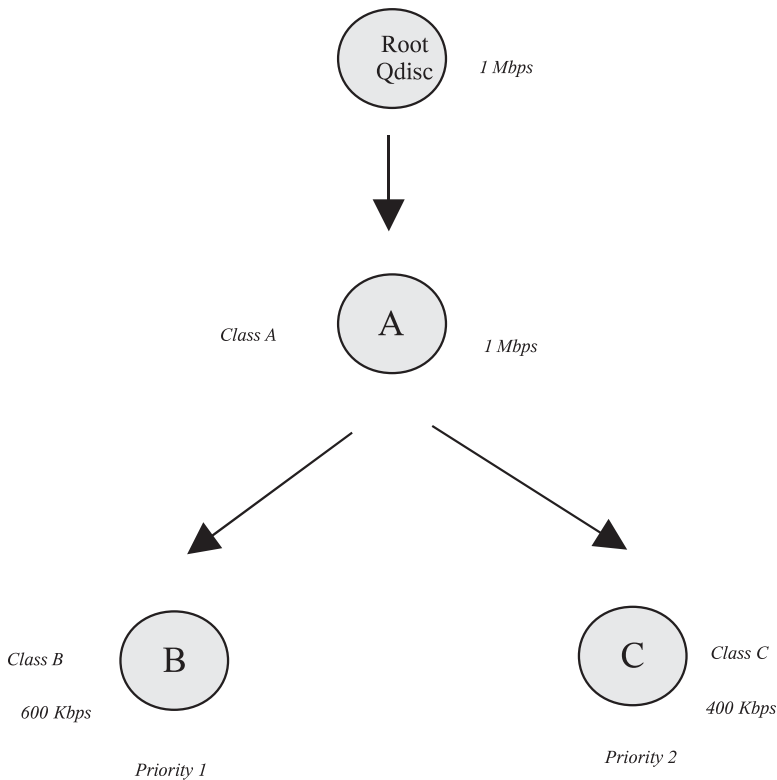
Figure 15.15. CBQ example.
