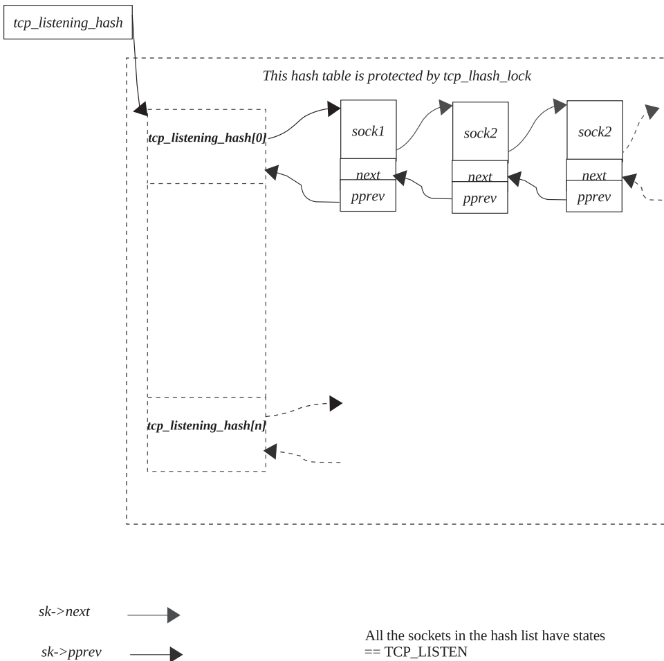
Figure 4.5. System-wide hash chain for all listening sockets having states == TCP_LISTEN.
