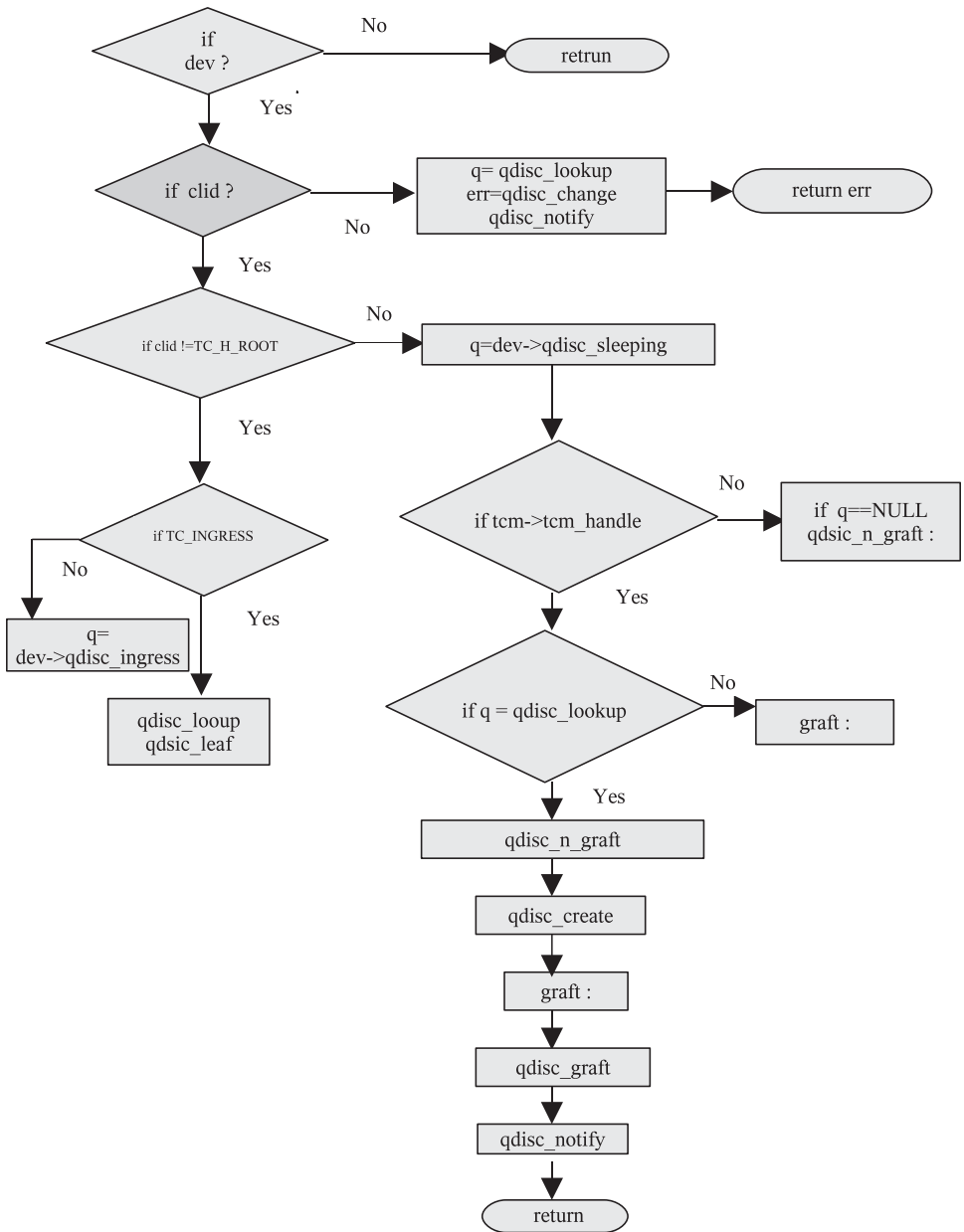
Figure 15.7. tc_modify_qdisc flow diagram.
