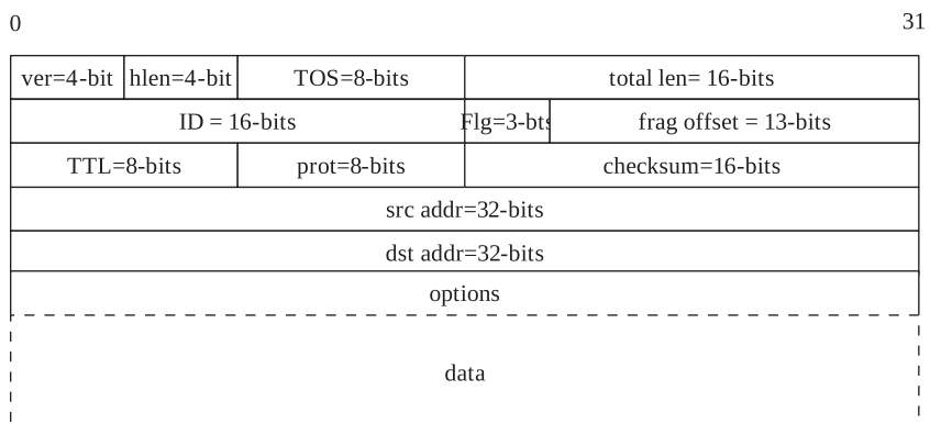
Figure 2.31. IPv4 header format.
