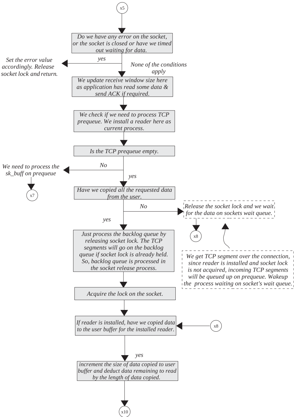
Figure 8.14c. Receive process (continued).
