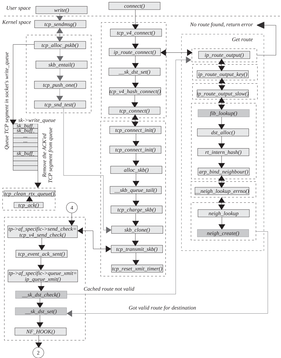
Figure 6.3a. Flow of packet down a TCP/IP stack in kernel 2.4.20.
