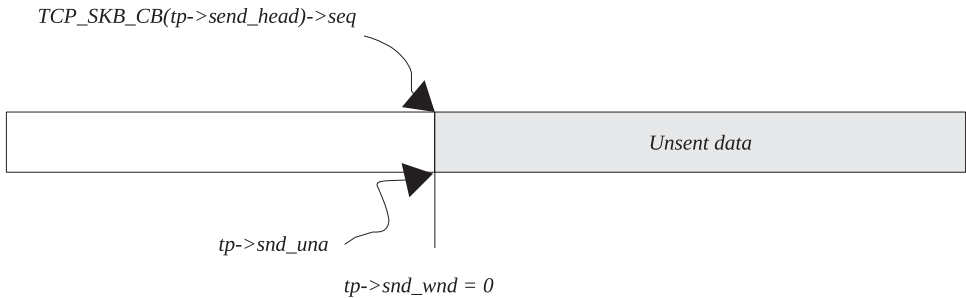
Figure 10.2. The window has not opened to transmit new data.
