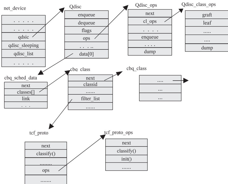
Figure 15.13. CBQ implementation.
