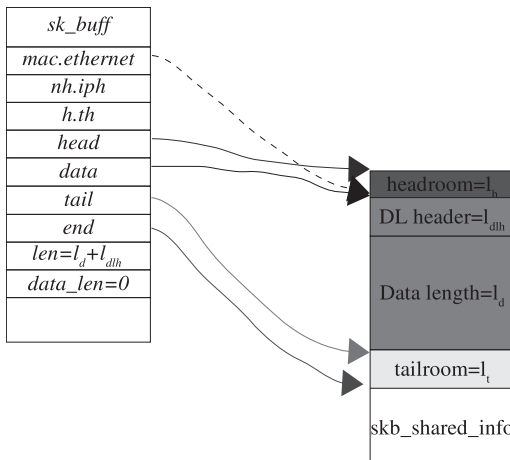
Figure 5.14. Status of sk_buff when new packet arrives on the interface, data points to start of data link header.
