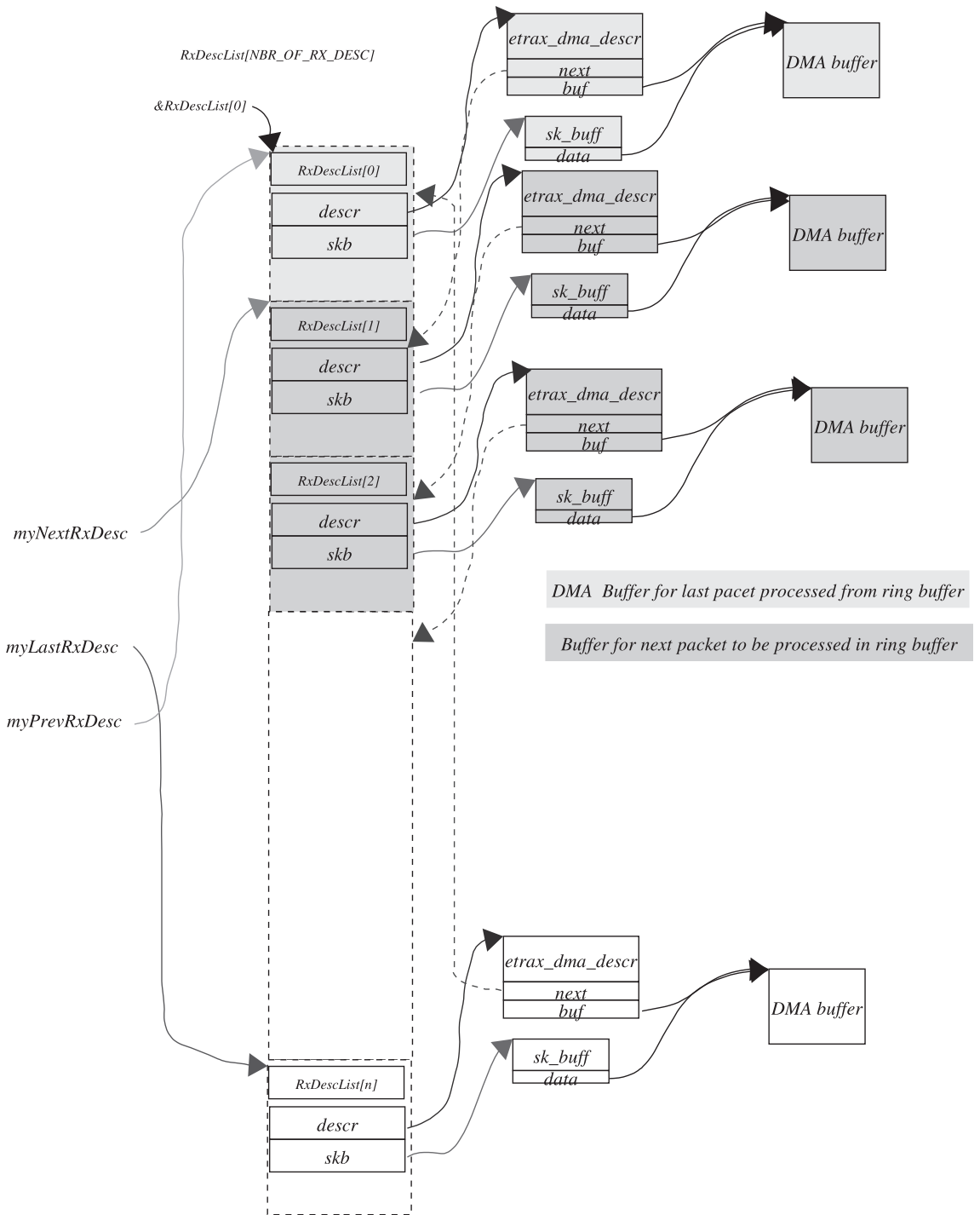
Figure 18.13. One packet taken out of Rx ring buffer for processing.
