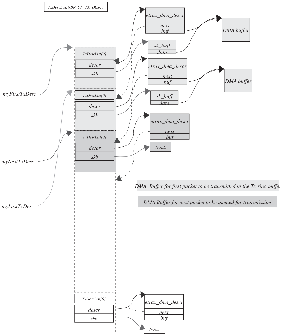
Figure 18.15. Two packets queued on Tx ring buffer for transmission.
