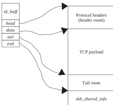
Figure 9.2. Memory layout of network buffer.
