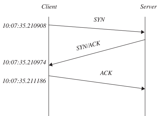
Figure 1.31. Time-line diagram for three-way handshake.
