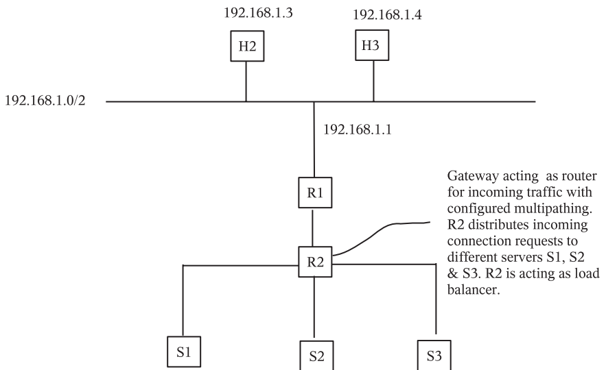
Figure 14.5. Multipathing and policy-based routing.
