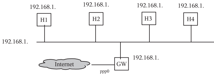
Figure 14.2. Network segment pointing to default gateway to access internet.
