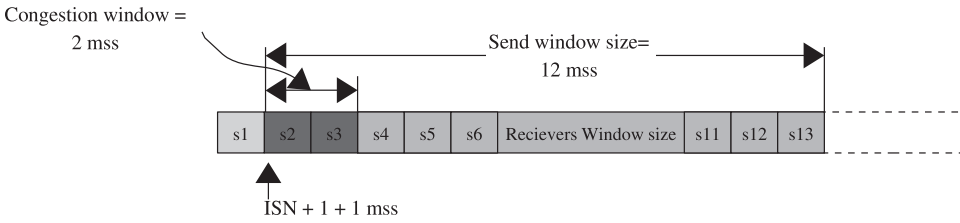
Figure 2.28b. Congestion window when 1 segment is ACK'ed.
