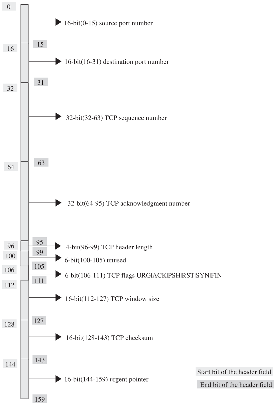
Figure 2.1. TCP header.
