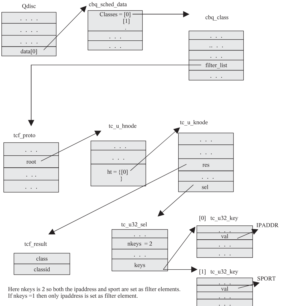
Figure 15.10. u32 filter implementation overview.
