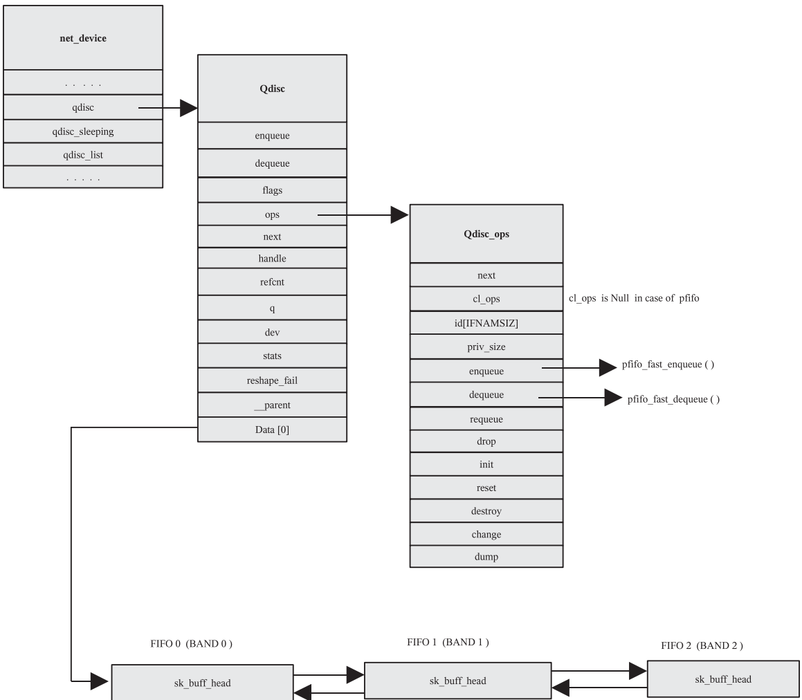
Figure 15.4. pfifo_fast qdisc implementation overview.
