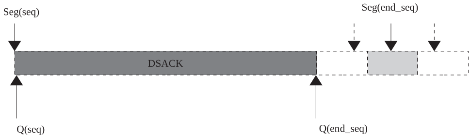
Figure 11.17. DSACK blocks generated in case new out-of-order segment completely covers segment in out-of-order queue.
