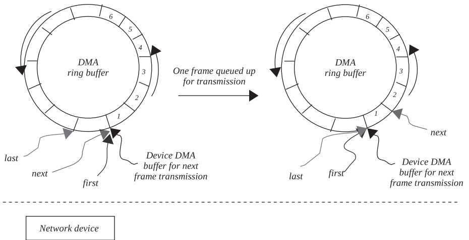
Figure 18.7. Single frame queued to a network controller that is not yet transmitted.
