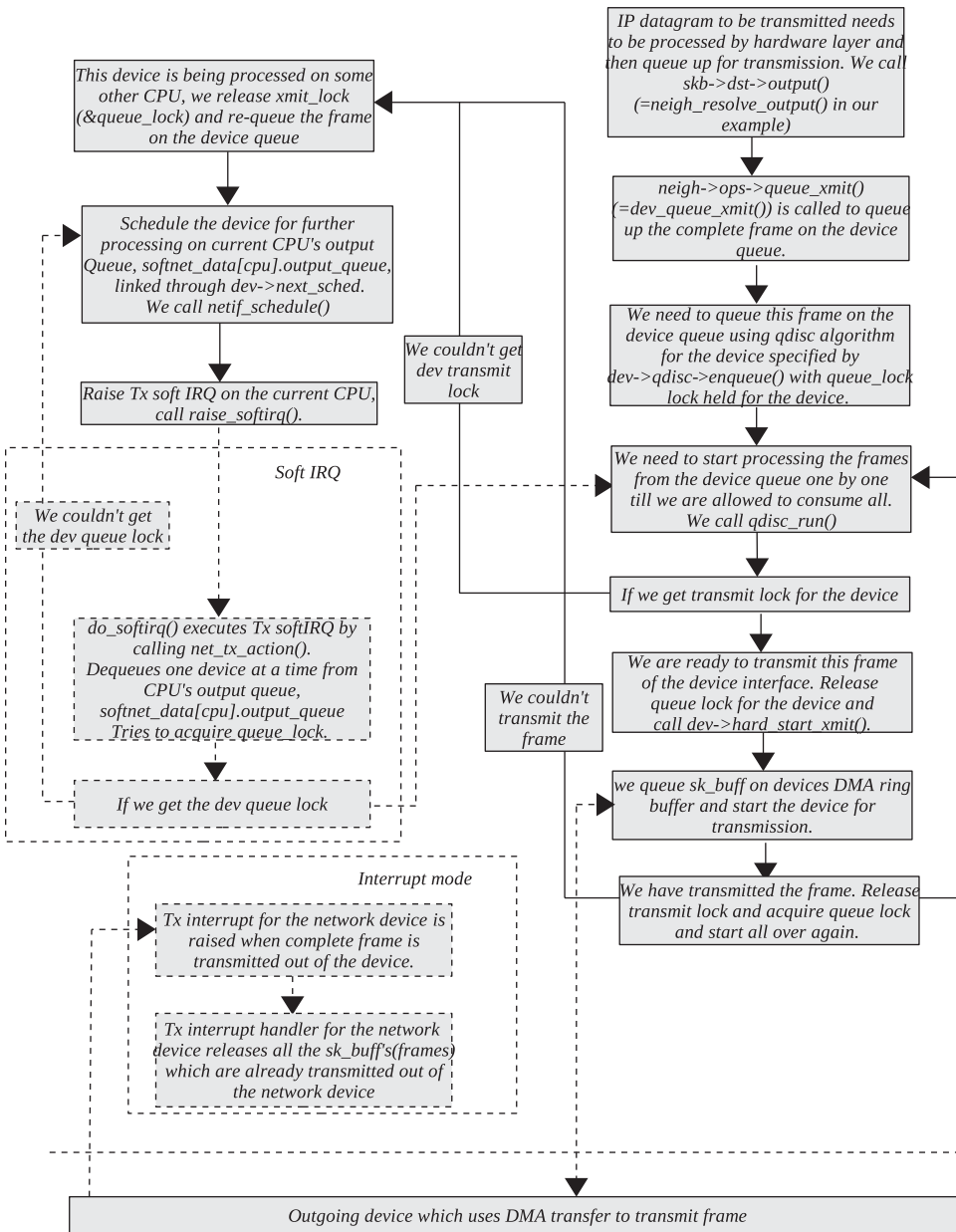
Figure 17.7. Packets being transmitted using Tx softIRQ framework.
