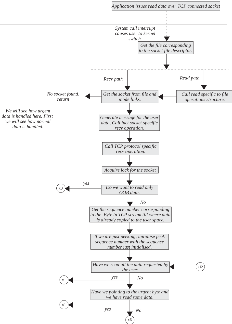
Figure 8.14a. Receive process.
