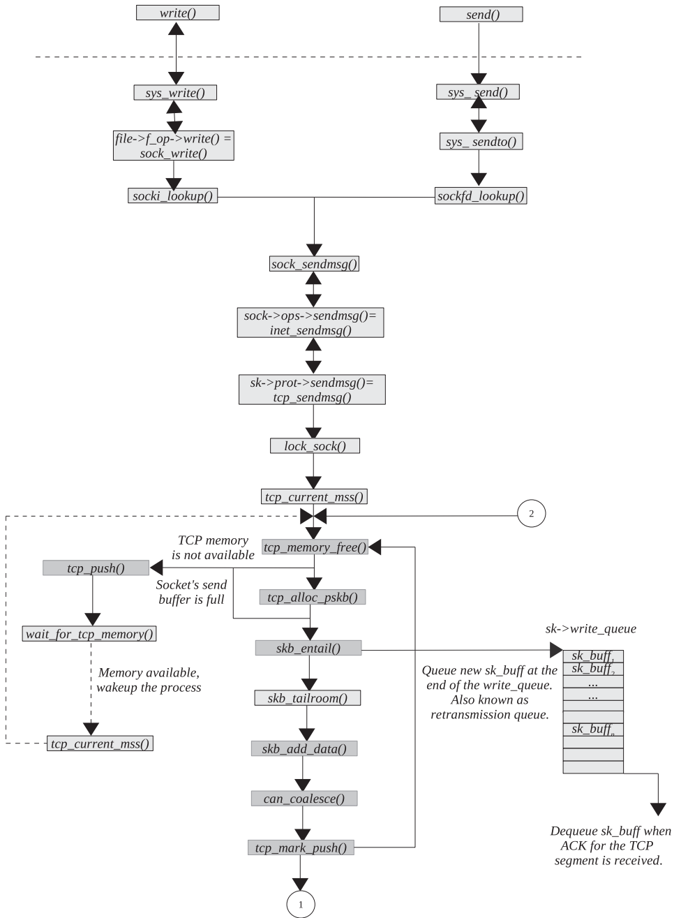
Figure 7.6a. Functional flow of TCP send process.
