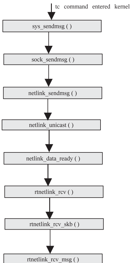
Figure 13.5. TC command flow in kernel space.
