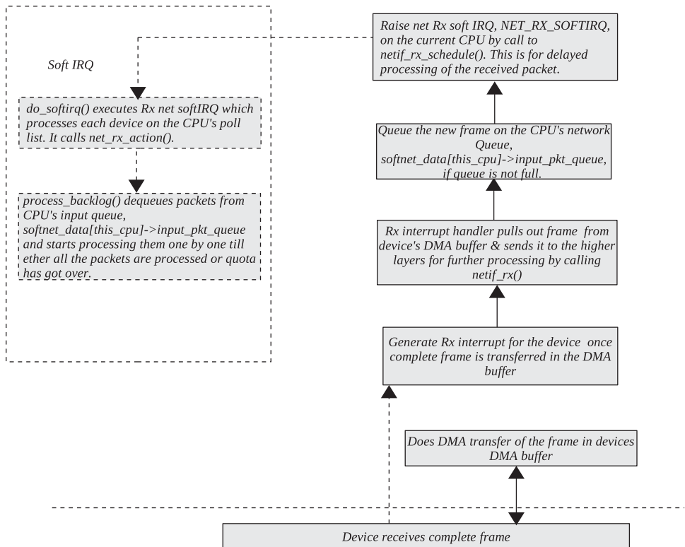
Figure 17.3. Processing of packets with softIRQ framework.
