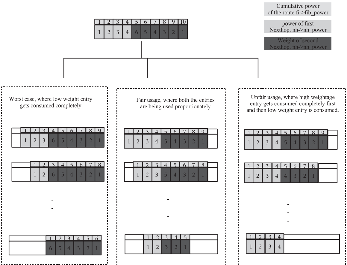
Figure 14.7 . Selection of nexthops with multipathing enabled.
