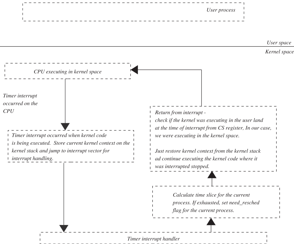
Figure 1.9b. Interrupt happened while executing in the kernel space.
