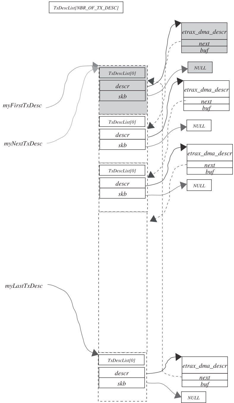
Figure 18.14. Tx ring buffer initialized.
