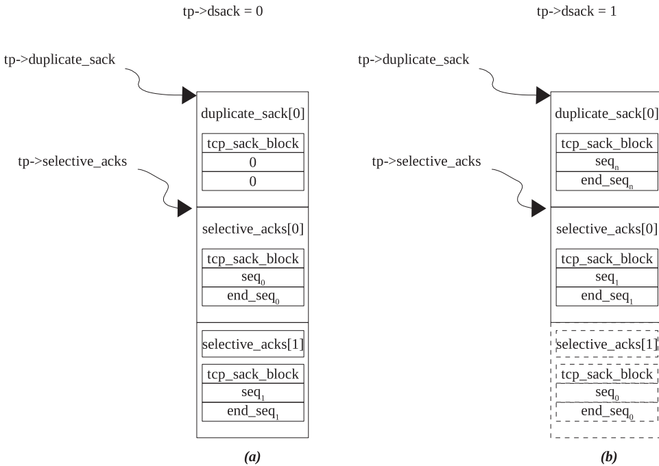
Figure 11.15. Generating DSACK blocks.
