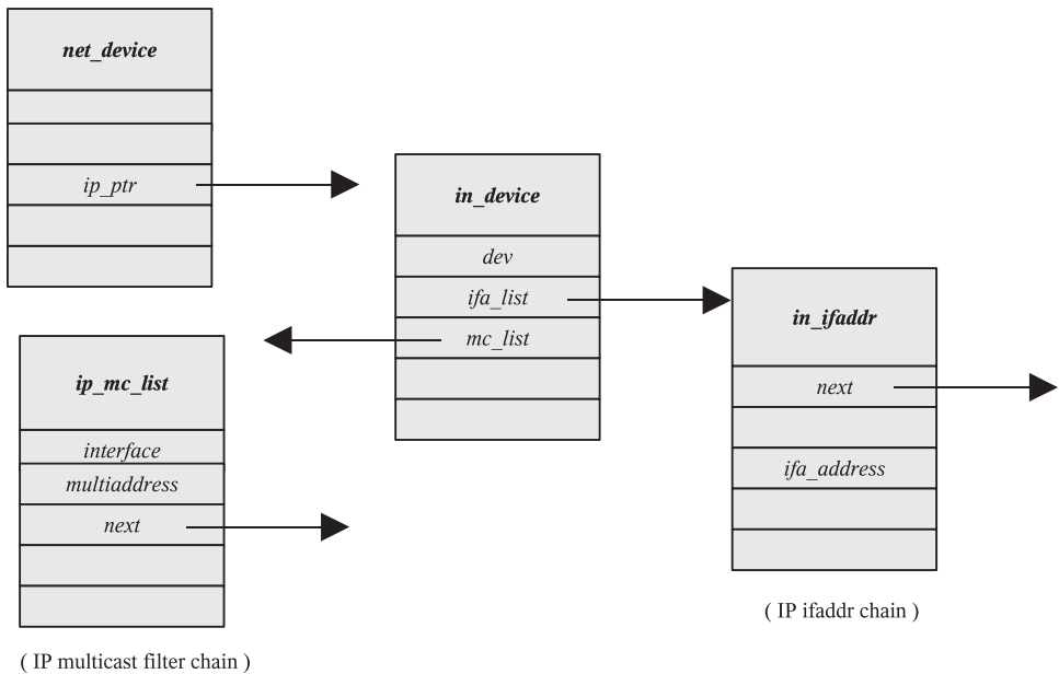
Figure 14.17. ifa_list and mc_list .
