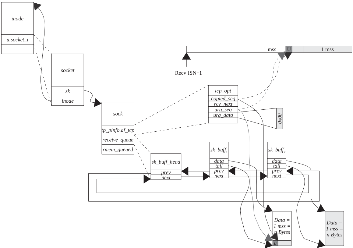
Figure 8.13. Application is returned data until an urgent pointer.
