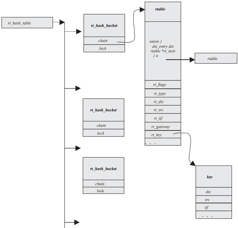
Figure 14.11. Routing cache implementation overview.
