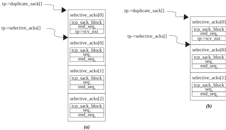
Figure 11.36. SACK blocks adjusted to follow the DSACK format.
