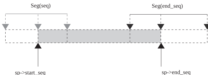
Figure 11.24. Overlapping sequence spaces, eligible for SACK extension.
