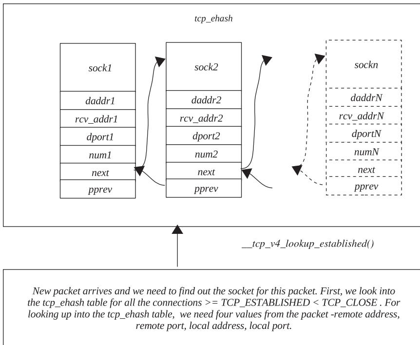
Figure 4.16. System-wide hash list for established sockets.
