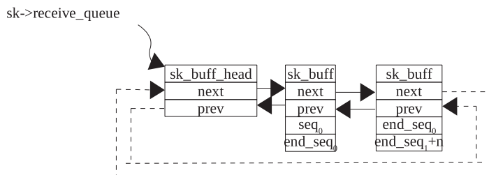
Figure 11.33. New segment is queued on the receive queue.
