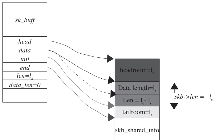
Figure 5.10. Status of sk_buff after call to skb_push() .
