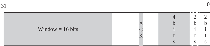
Figure 11.3b. Calculation for building prediction flags tp \rightarrow pred\_flags (continued).
