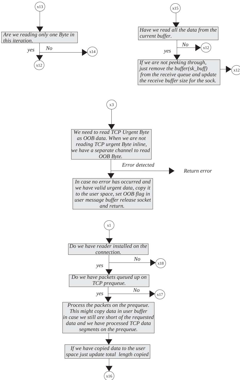
Figure 8.14e. Receive process (continued).
