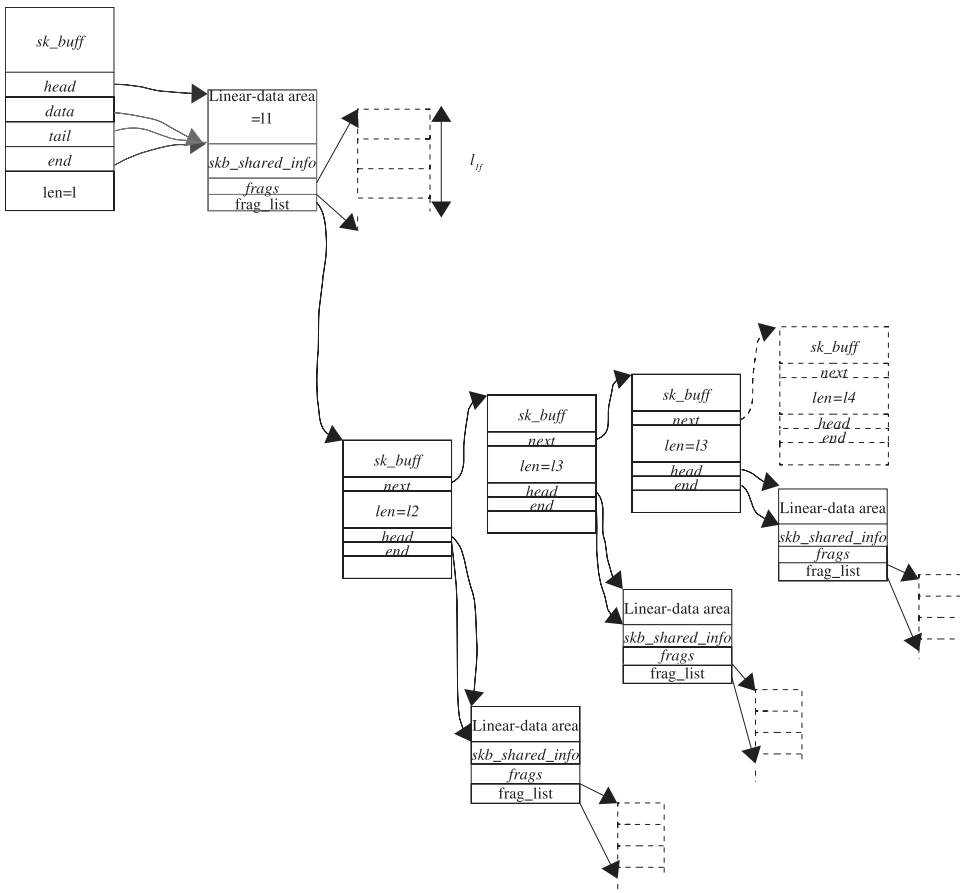
Figure 5.5. Fragmentation and paged data area for sk_buff .
