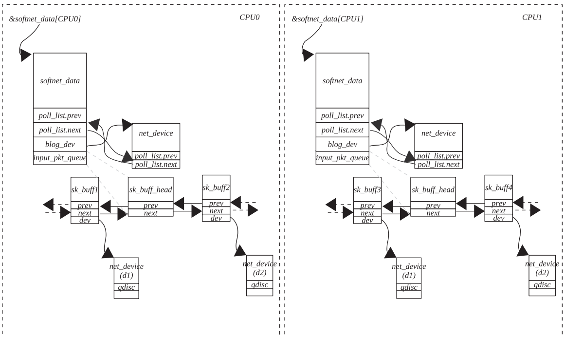
Figure 17.5. Packets being queued on per CPU input queue.
