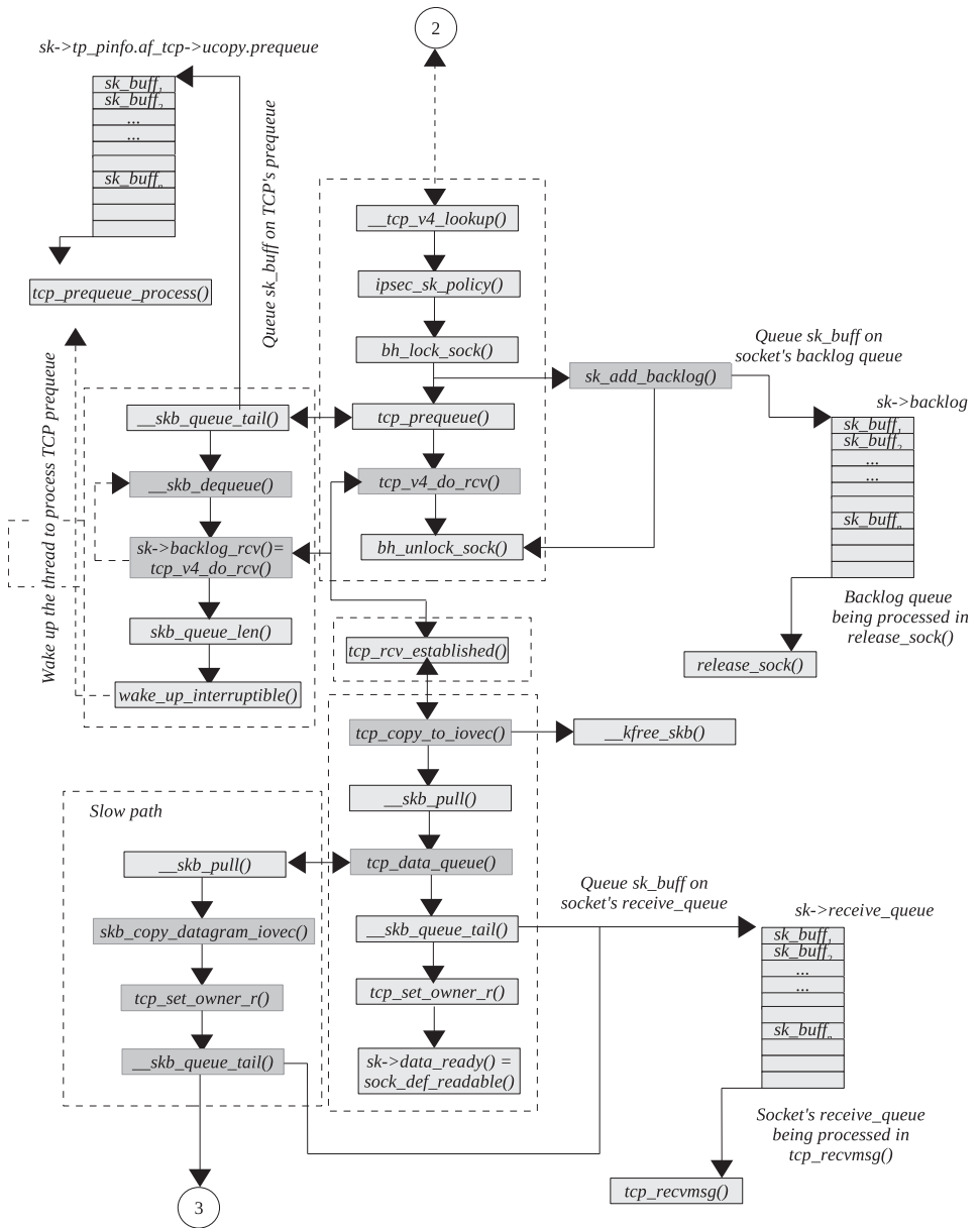
Figure 6.5c. Flow of a packet up a TCP/IP stack in kernel 2.4.20 (continued).
