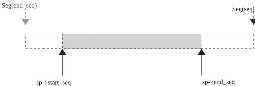
Figure 11.23. Sequence spaces are not overlapping, not eligible for SACK extension.
