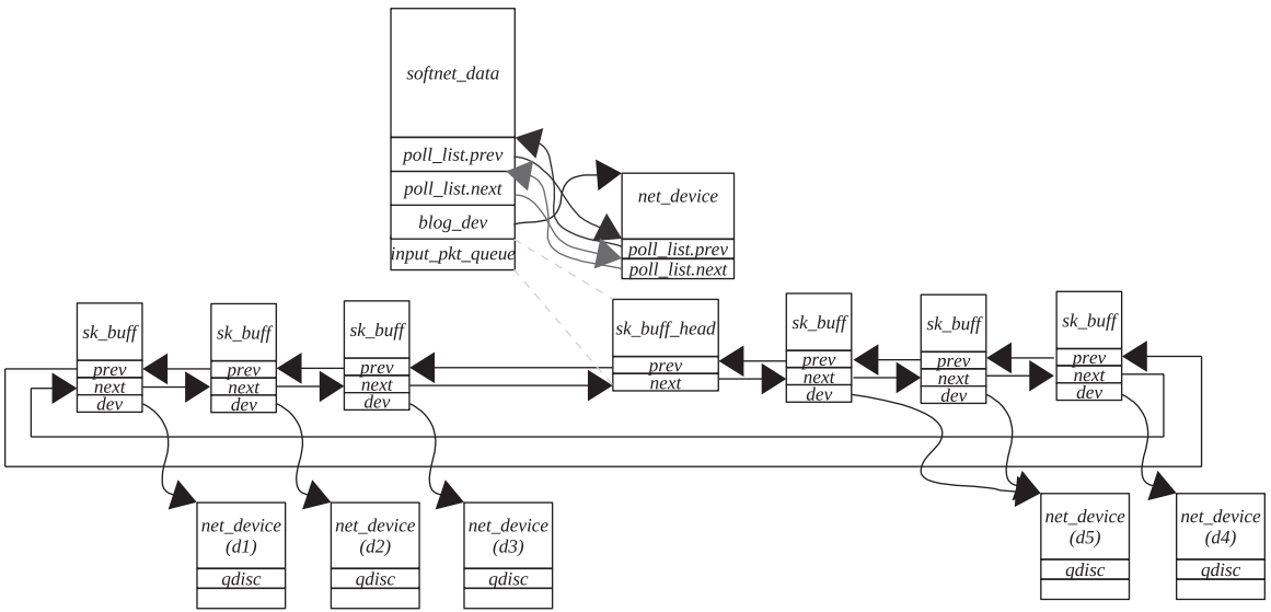
Figure 17.4. Packets being queued on CPU input queue.
