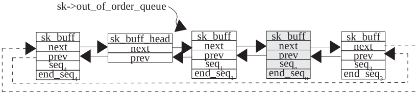
Figure 11.20. Segment 2 is eaten by new segment.
