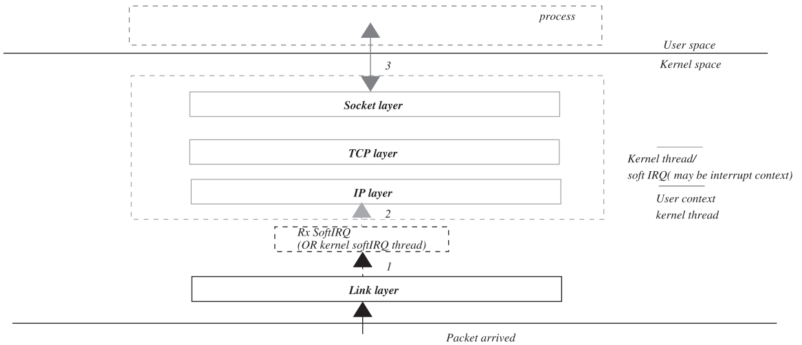
Figure 1.8. Packet reception and different kernel control paths.
