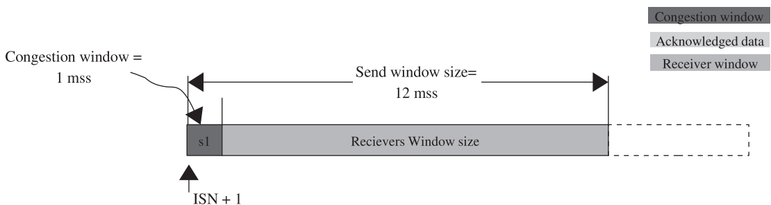
Figure 2.28a. Congestion window when no data is sent.
