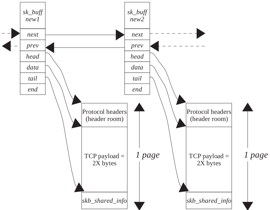
Figure 9.6. Finally we have two new buffers replacing four old buffers after collapsing the queue.
