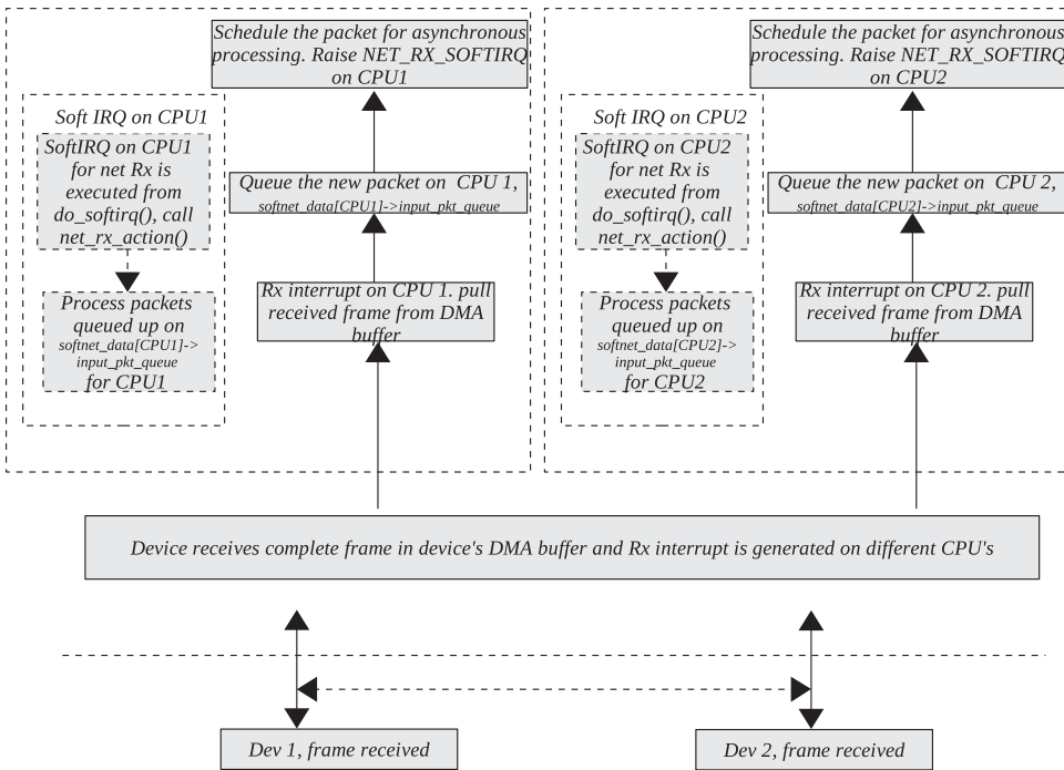
Figure 17.6. Two packets from the different devices being received on different CPUs.
