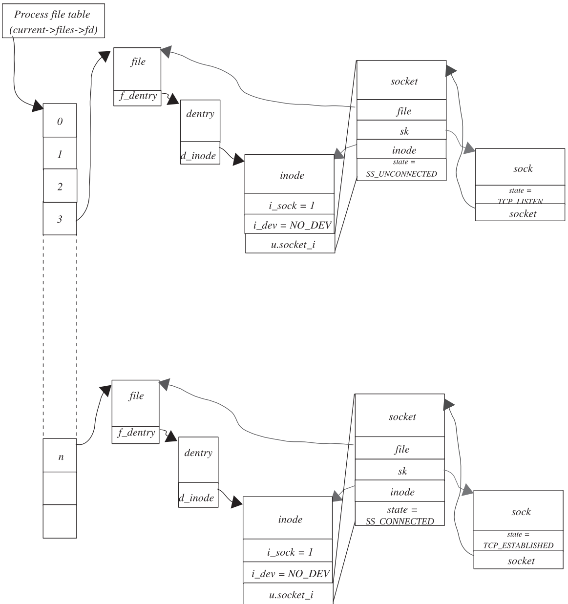
Figure 4.22. Linking of various data structures when a connection request is accepted by a listening socket.
