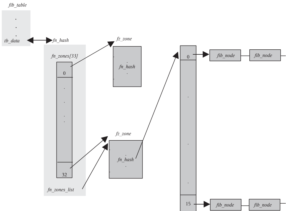
Figure 14.18. fn_hash table.
