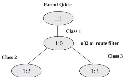
Figure 19.24. CBQ setup.
