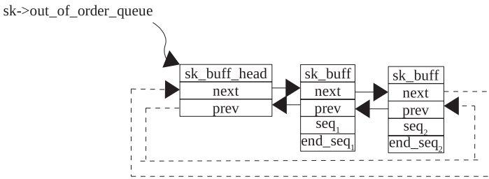
Figure 11.26. Out-of-order segments.
