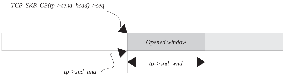
Figure 10.3. The window has opened enough to transmit new data.
