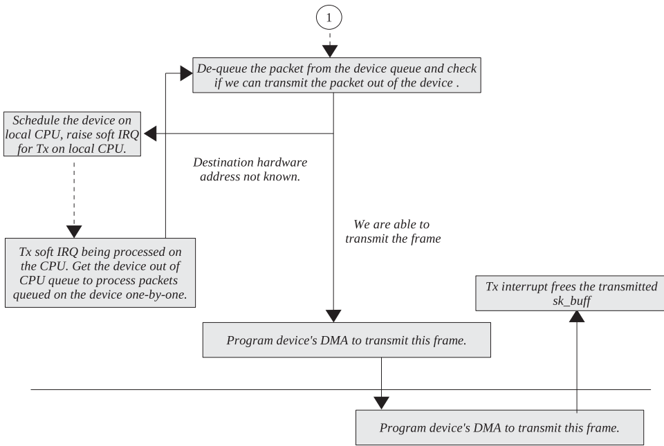
Figure 6.1b. Packet traversal down TCP/IP stack.
