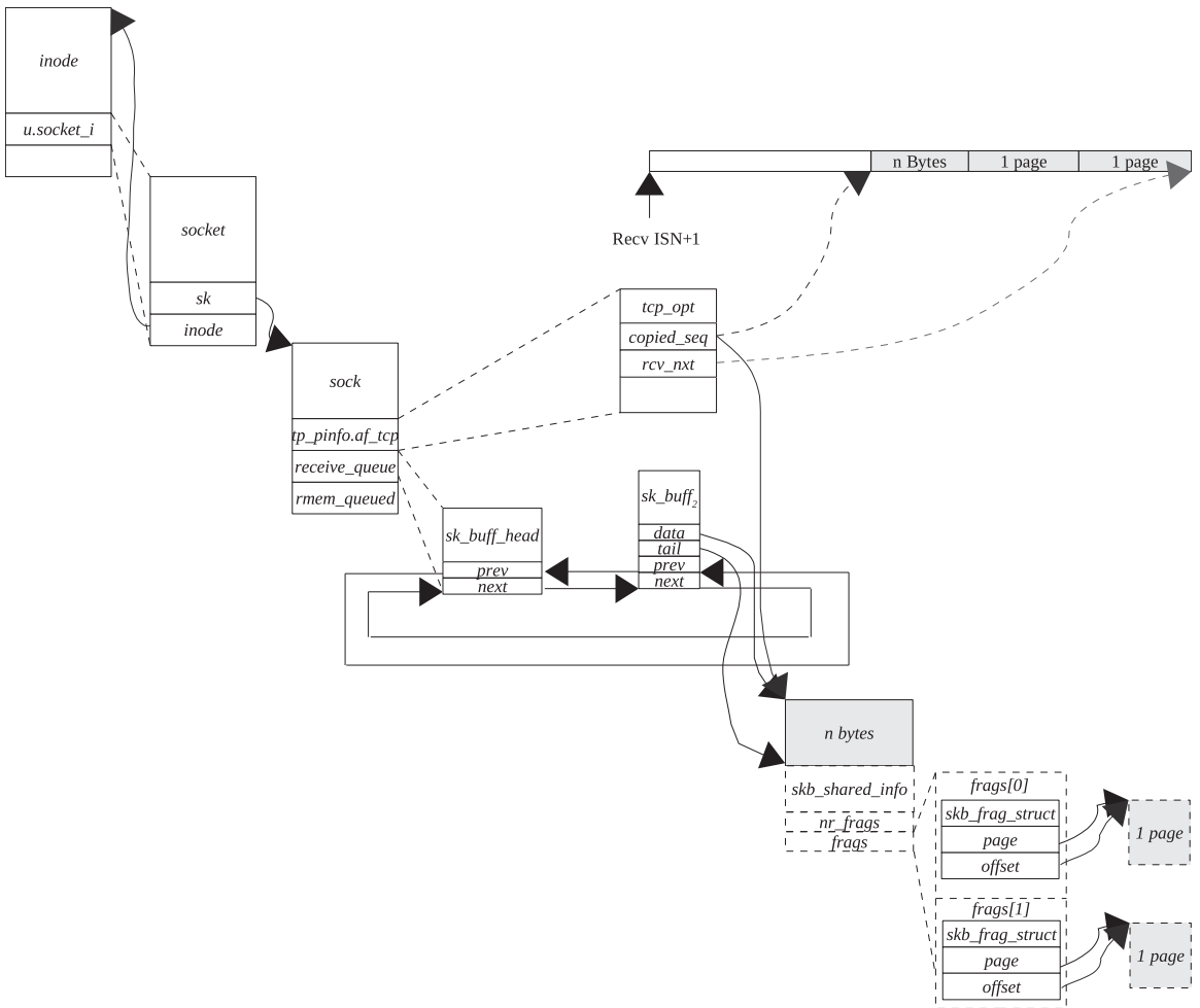
Figure 8.5. Data in a linear and paged data area of socket.
