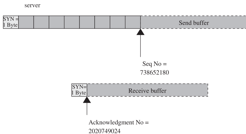
Figure 2.17d. 8-bytes transmitted by server.
