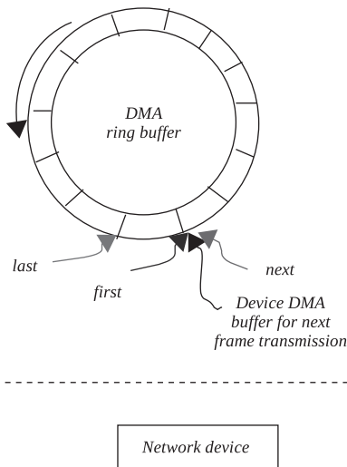
Figure 18.10. On return from the Tx interrupt, all three buffers in Tx ring buffer are freed.
