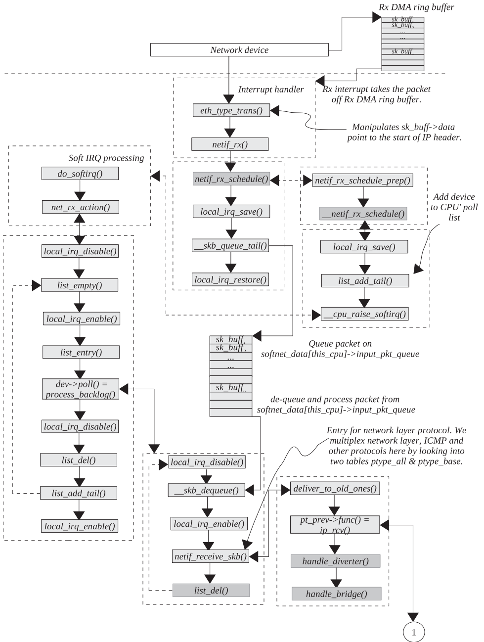
Figure 6.5a. Flow of a packet up a TCP/IP stack in kernel 2.4.20.
