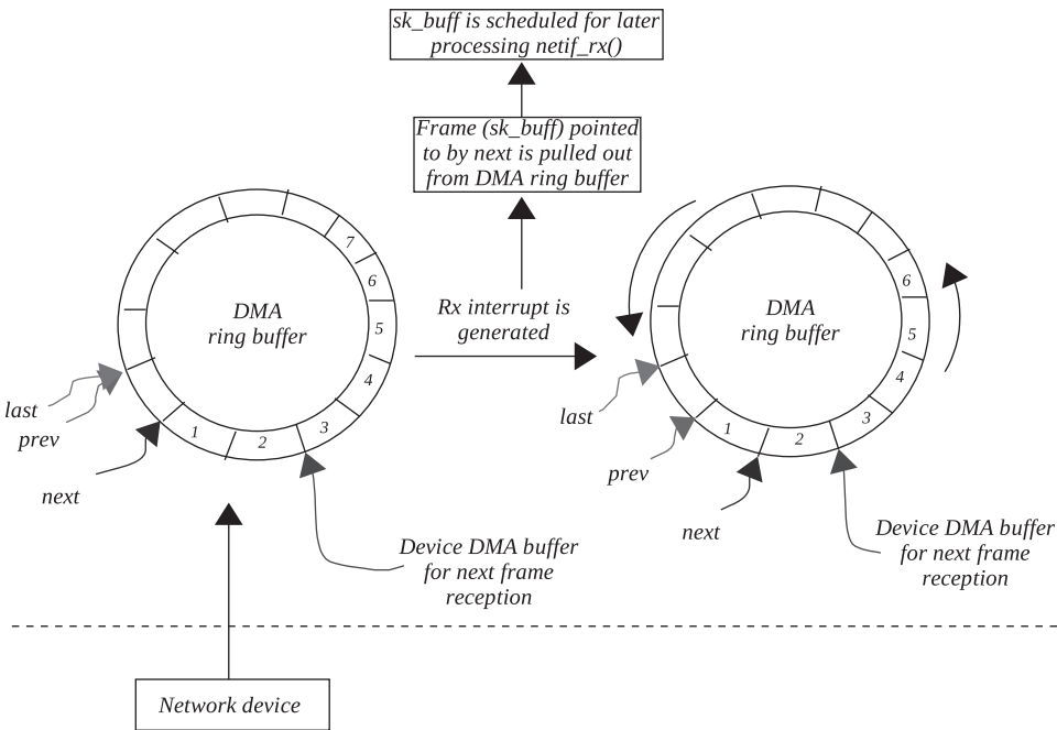
Figure 18.4. Interrupt is generated and first packet from ring buffer is processed.
