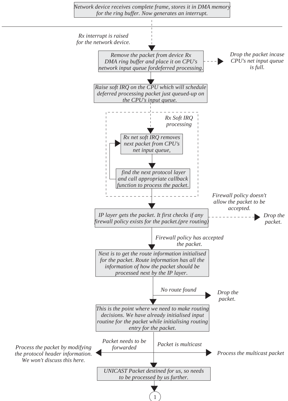
Figure 6.4a. Traversal of a packet up the TCP/IP stack.
