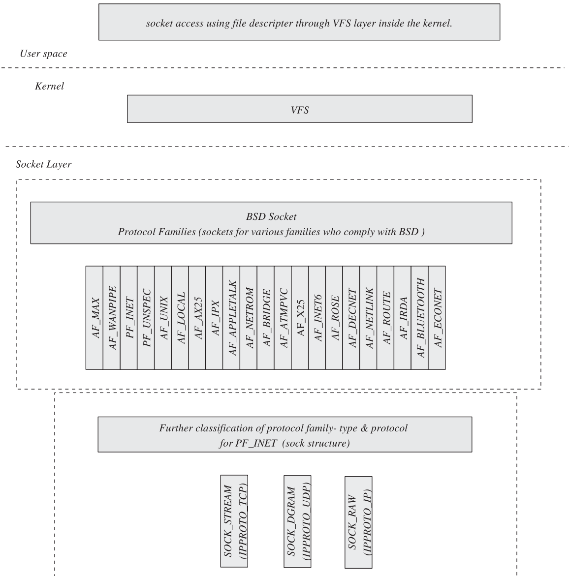
Figure 3.1. Socket architecture.
