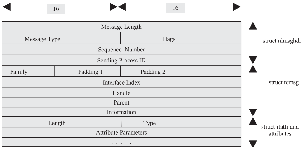
Figure 13.3. Netlink packet format.
