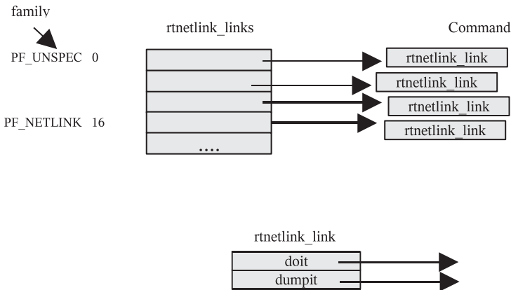
Figure 13.2. rtnetlink_links and rtnetlink_link data structure.
