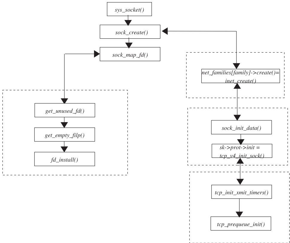
Figure 3.10. Flow for socket system call.
