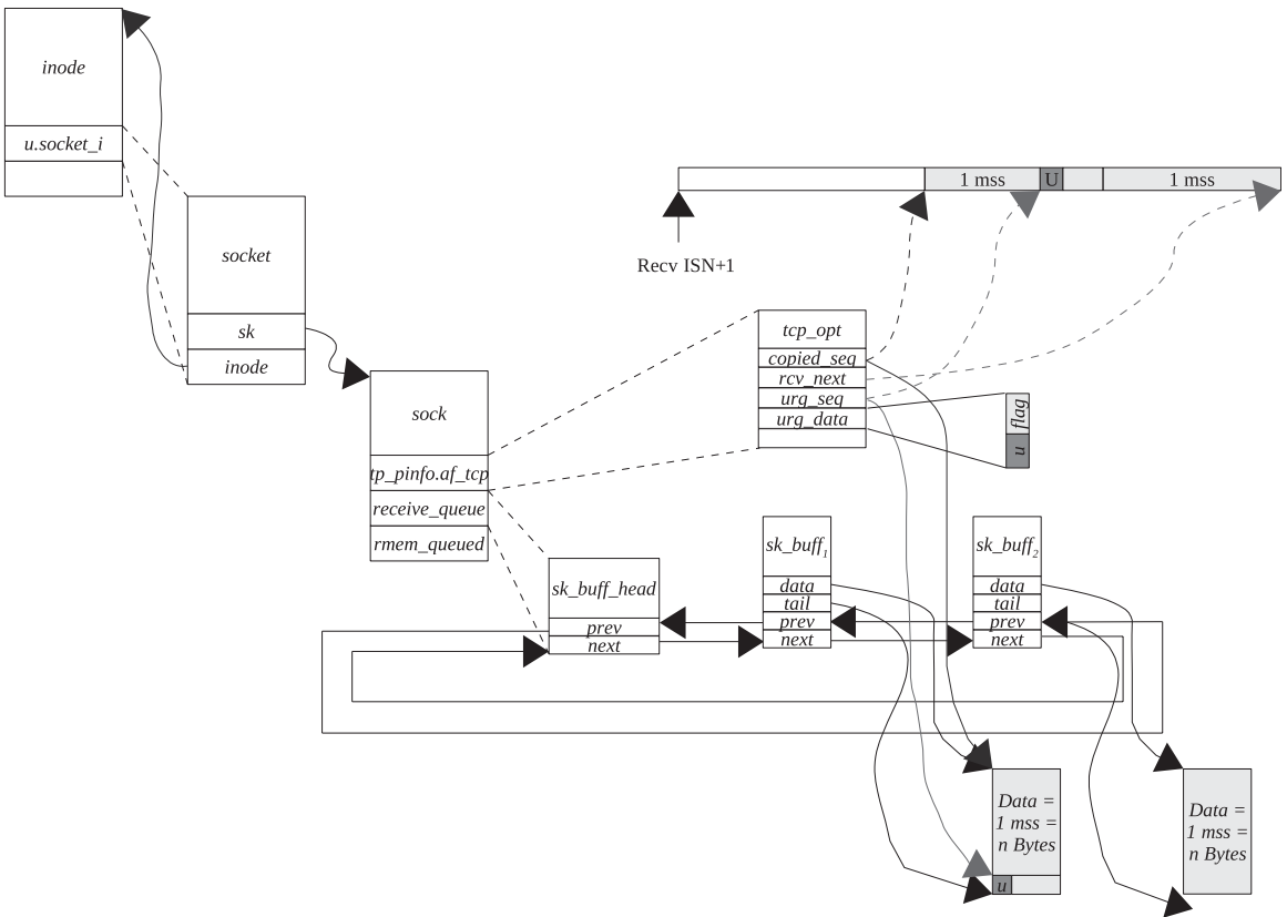
Figure 8.8. Urgent byte is received.
