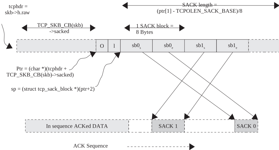
Figure 11.4. Organization of SACK blocks in TCP header.
