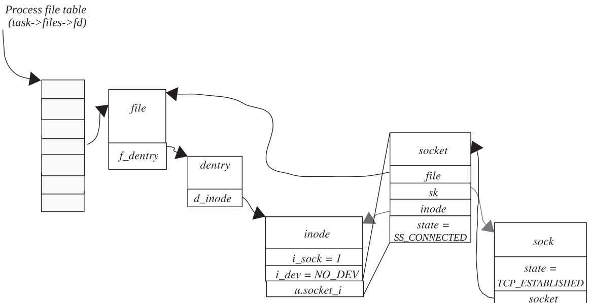
Figure 3.2. Socket accessed through process file table.
