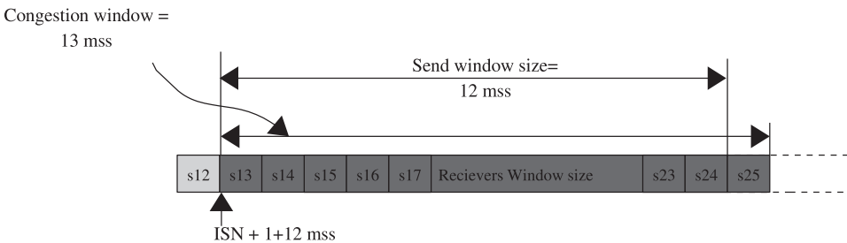
Figure 2.28e. Congestion window is more than the send window (saturation point).
