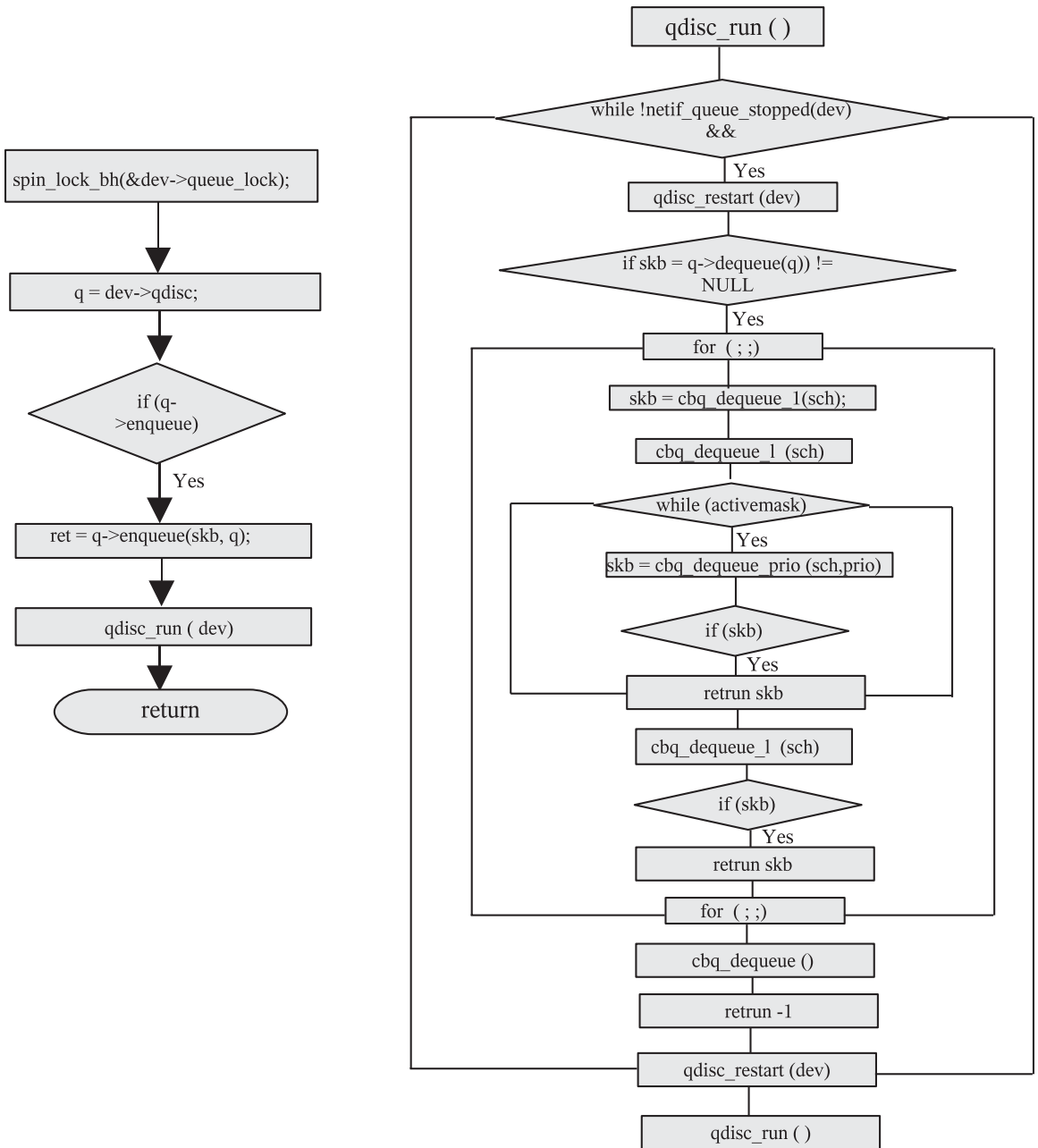
Figure 15.16. CBQ enqueueing and dequeuing flow.
