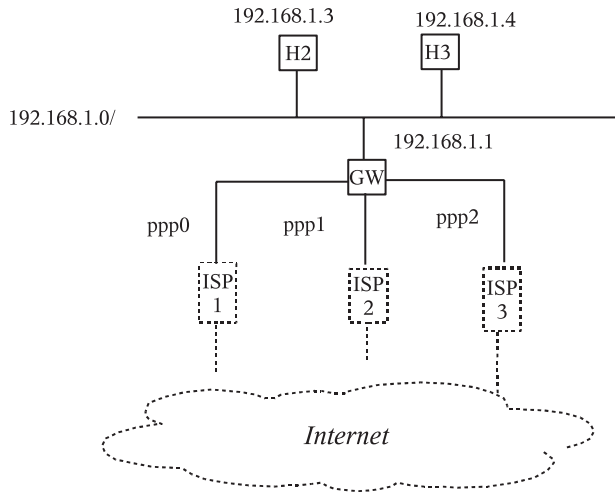
Figure 14.4. GW does multipathing.
