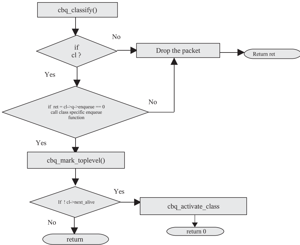
Figure 15.12. cbq_enqueue() flow diagram.
