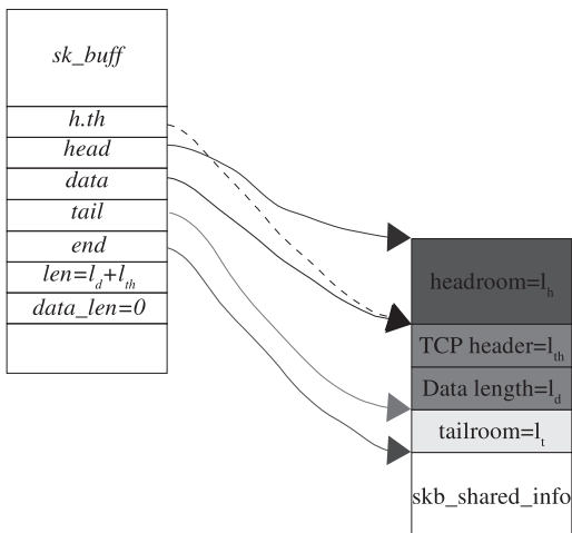
Figure 5.11. Status of sk_buff after TCP header is added to the outgoing packet.
