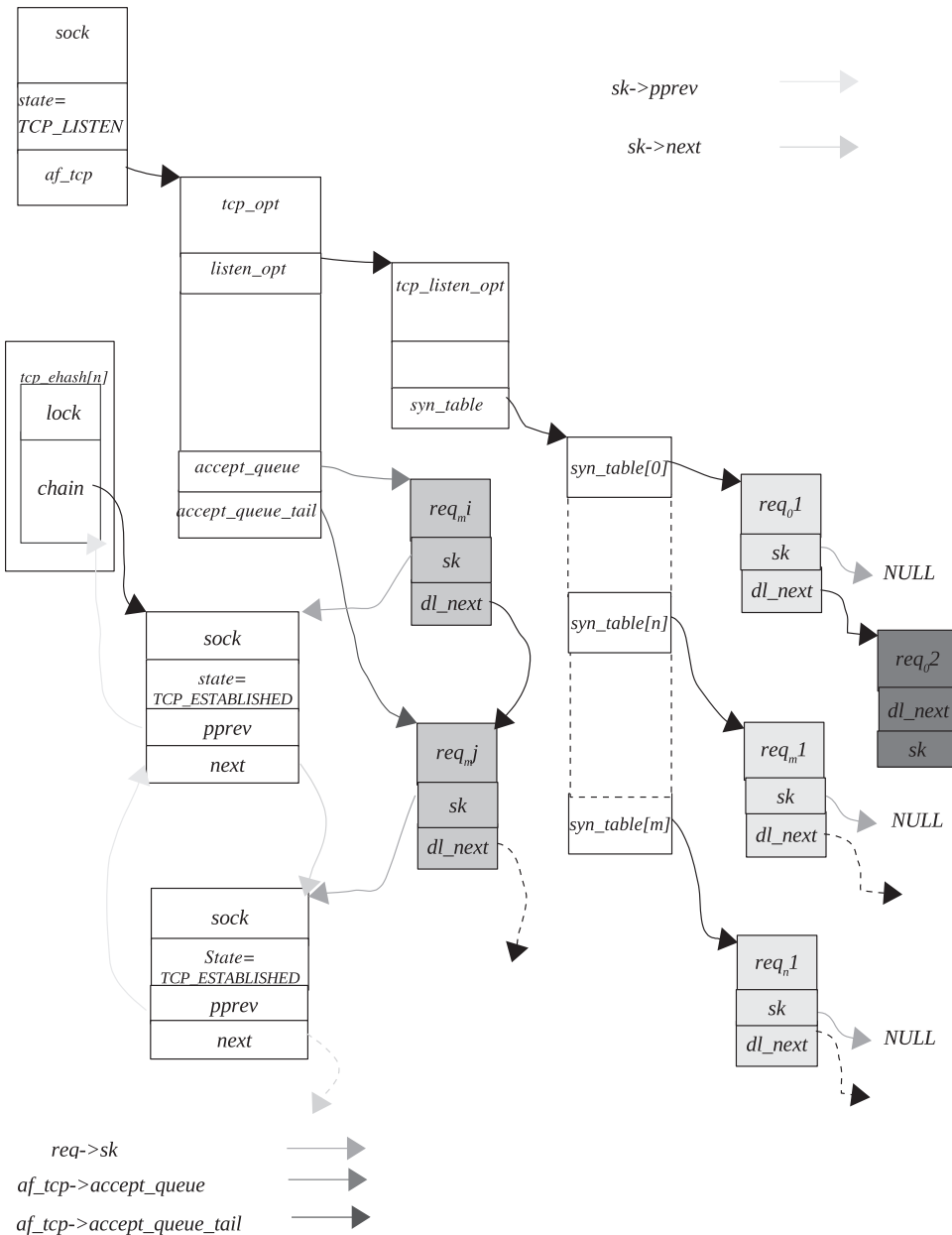
Figure 4.17. Open connection request waiting in SYNQ until the three-way handshake is over.
