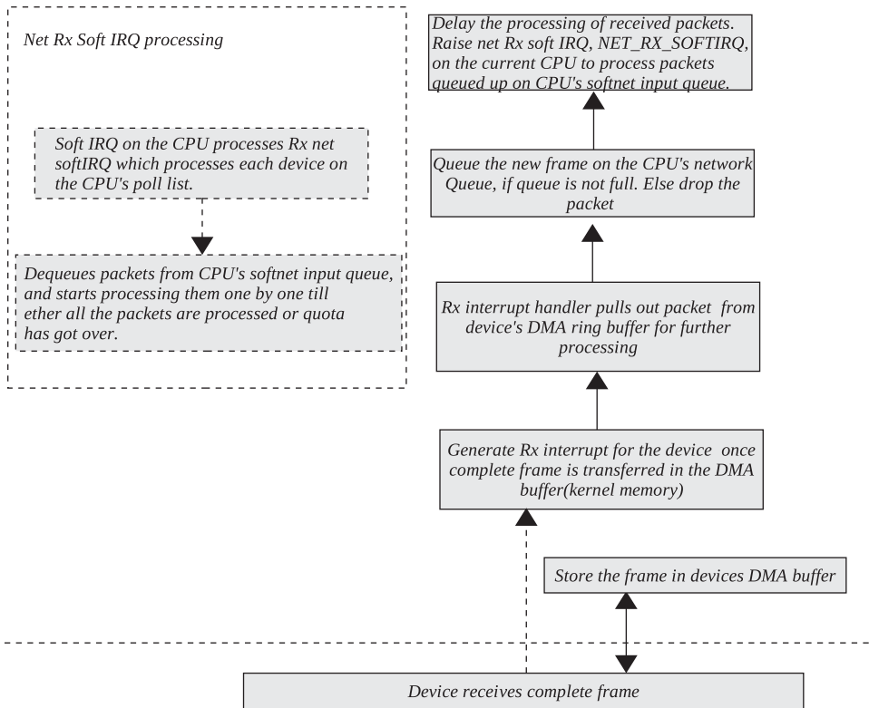
Figure 18.1. Network frame is received into kernel memory and processed further.
