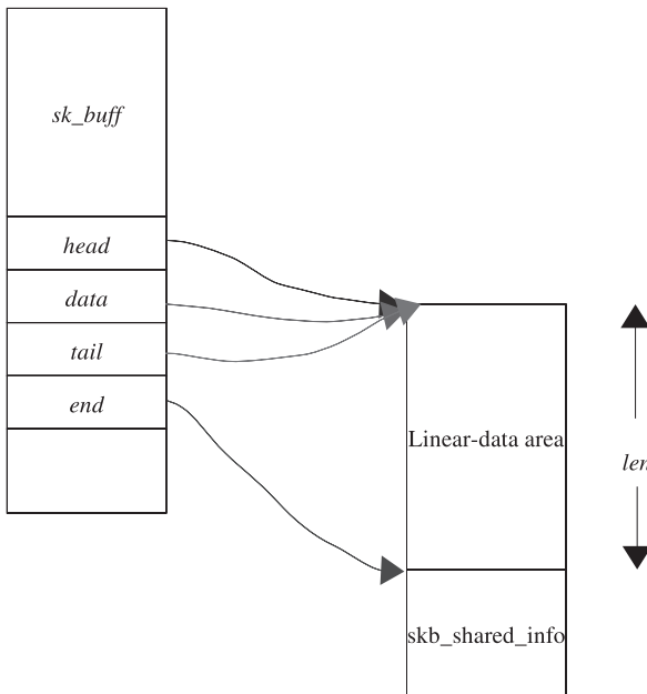
Figure 5.2. sk_buff when it is just as returned by skb_alloc() .
