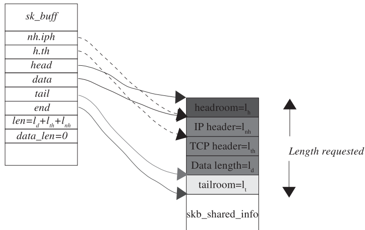
Figure 5.12. Status of sk_buff after IP header is added to the outgoing packet.
