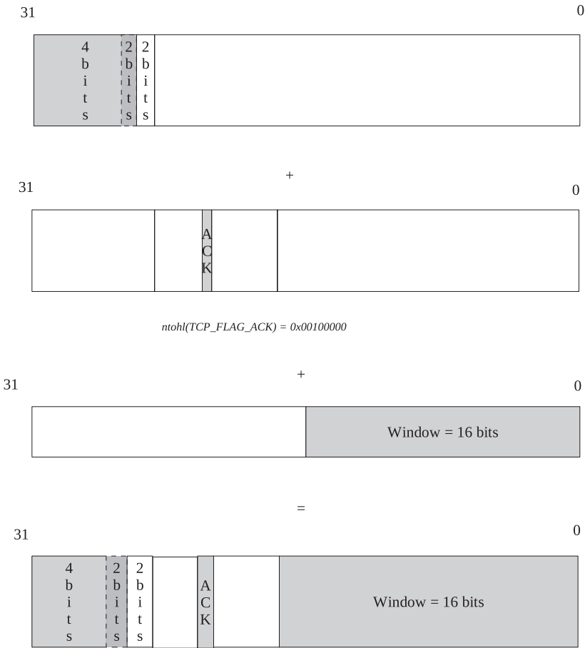
Figure 11.3a. Calculation for building prediction flags tp \rightarrow pred\_flags .
