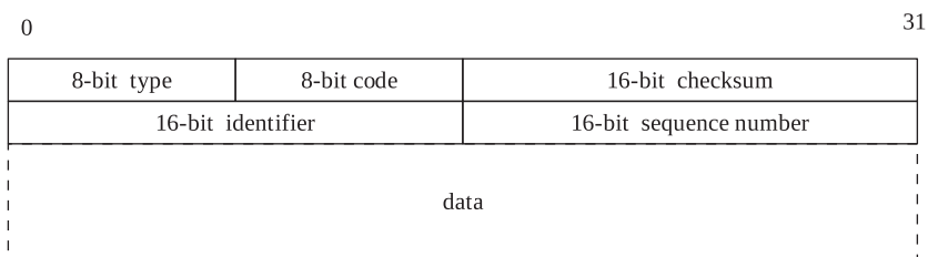
Figure 2.36. ICMP header format for echo request-reply message.
