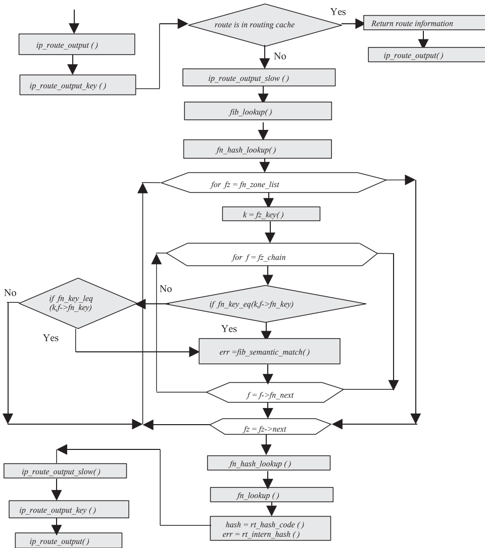
Figure 14.16. FIB traversal flow diagram.
