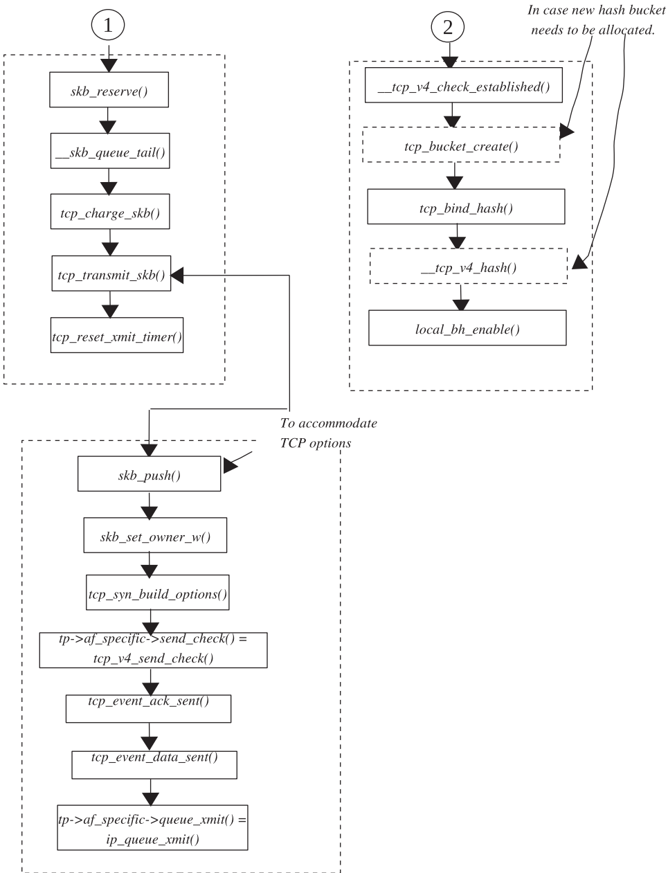
Figure 4.25b. Code flow for connect process (continued).
