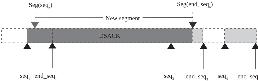
Figure 11.21. DSACK generated for the new segment.
