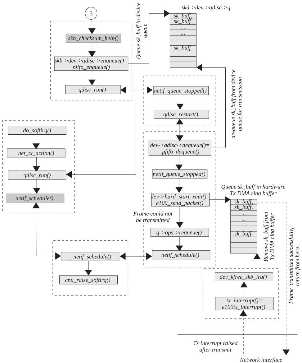
Figure 6.3c. Flow of packet down a TCP/IP stack in kernel 2.4.20 (continued).
