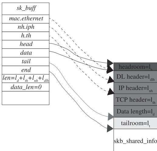
Figure 5.13. Status of sk_buff after link layer header is added to the outgoing packet.
