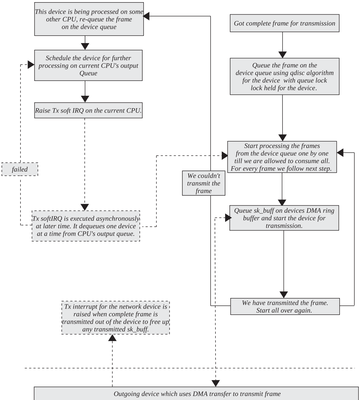
Figure 18.6. Process of packet transmission.
