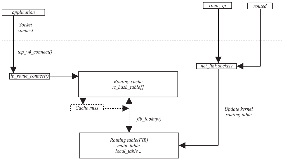
Figure 14.10. Route cache and FIB.
