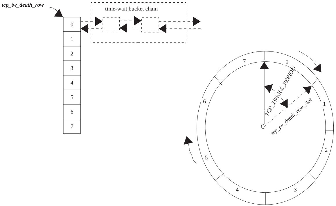
Figure 10.5. Time-wait timer schedule for the non-recycle mode.
