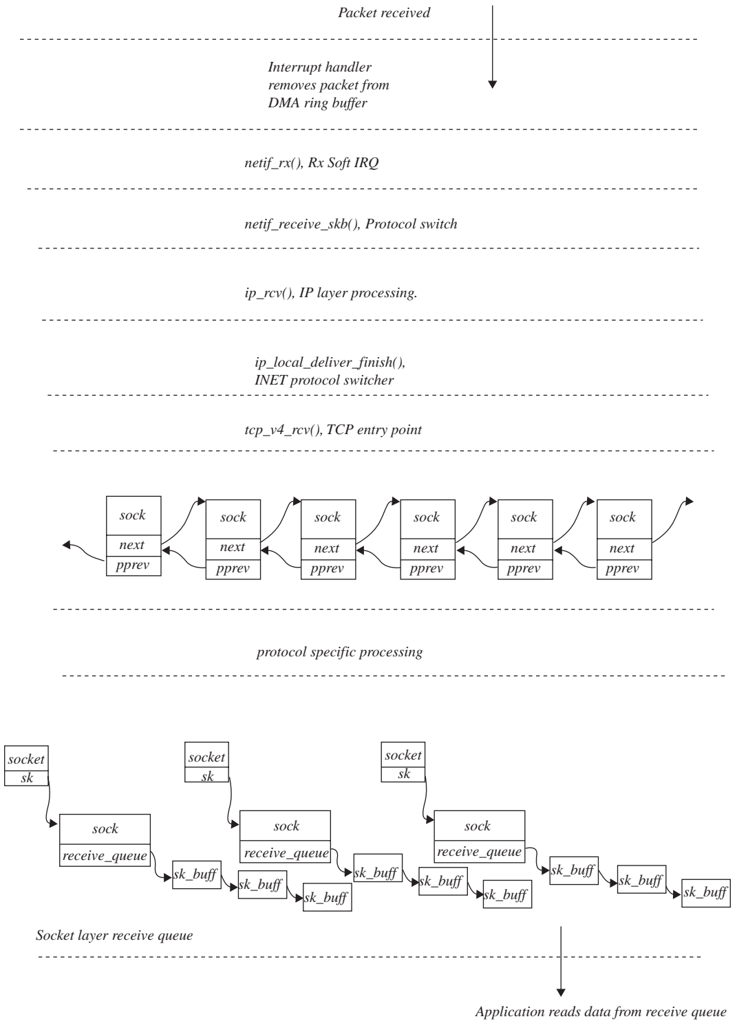
Figure 1.3. TCP packet moving up the stack.
