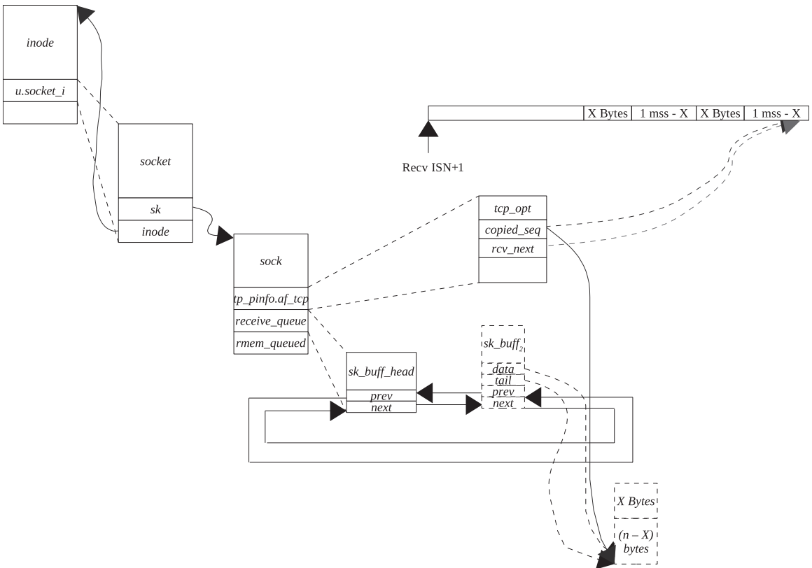
Figure 8.4. Complete data from a socket buffer are copied to a user buffer.
