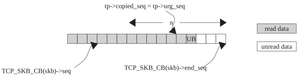
Figure 8.10. Application is returned data until an urgent pointer.
