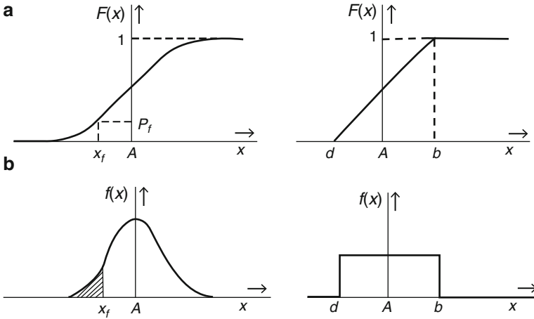
Fig. 3.1 (a) Cumulative distribution function of a normally ( left ) and uniformly ( right ) distributed continuous random quantity and (b) Corresponding probability density functions
