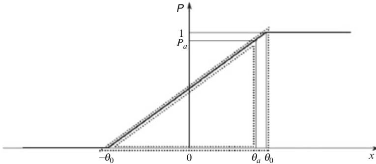
Fig. 4.3 Computing limits of confidence interval for uniformly distributed random error
