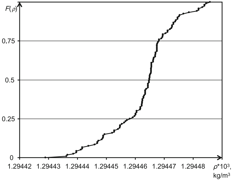
Fig. 8.2 The cumulative distribution function of realizations \rho_t
