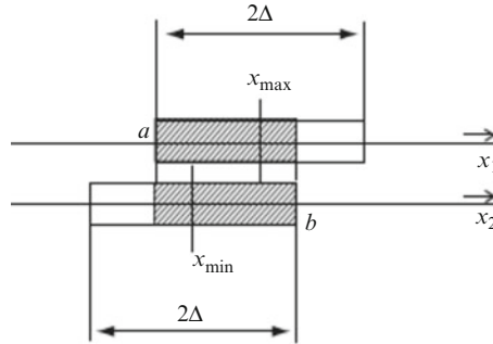
Fig. 7.1 The highest ( x_{\max} ) and lowest ( x_{\min} ) indications of the group of the instruments used to measure the same quantity; the interval of possible error of the combined measurement result is hatched
