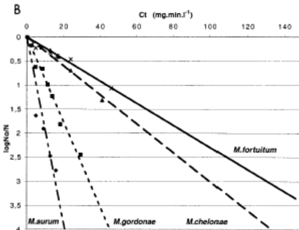
Fig. 11.2 Disinfection of mycobacteria by free chlorine. Experimental conditions: pH 7.0, 25 °C, initial free chlorine concentration 0.5 mg/l. Reprinted from Le Dantec et al. 2002a.
