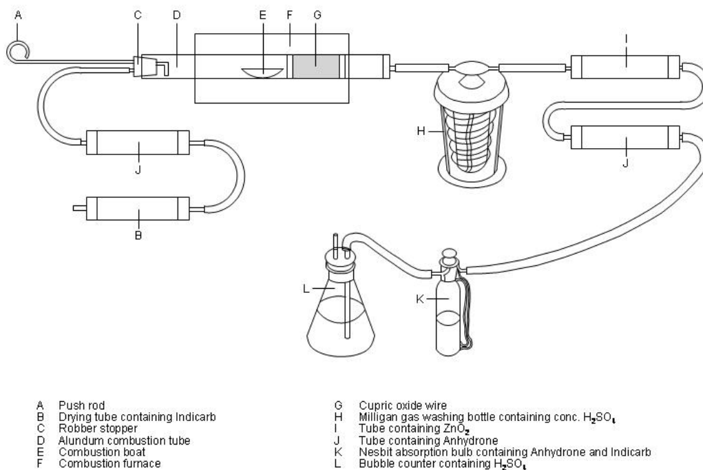
Figure 6. Apparatus used for organic carbon determination by dry combustion, carbon dioxide evolution II (6A2b).
