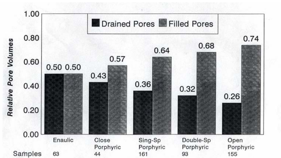
Figure 16. Relative pore volumes at 30 kPa for soil fabric coarse-fine distributions for some U.S. soils.
