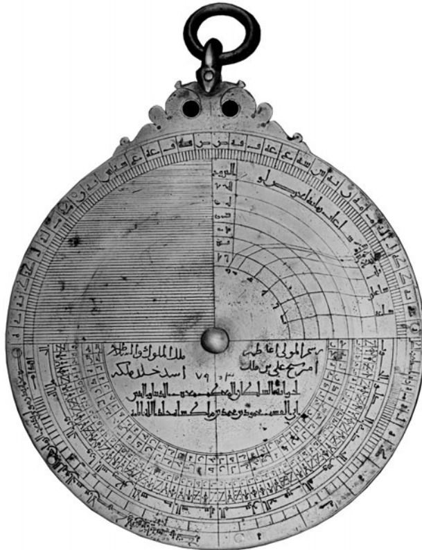
Figure 8.10. The back of a brass astrolabe made by Badr ibn ‘Abdallah ca. 1130 probably in Baghdad. 18.8 × 13.4 cm. Note the Persian writing and the absence of an alidade sighting bar. Courtesy of the Adler Planetarium & Astronomy Museum, Chicago, Illinois, A-84. See also Color Section 3.
