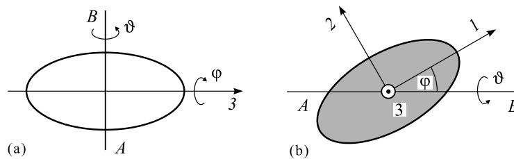
Fig. 13.10. Homogeneous three-axial ellipsoid: (a) side view, and (b) top view
