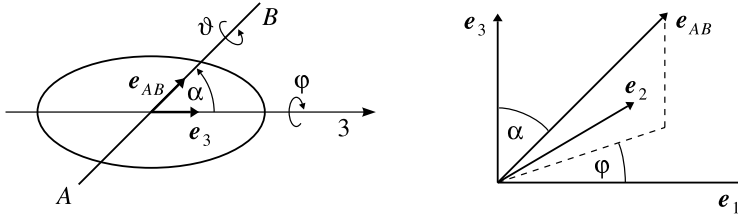
Fig. 13.11. The axis \overline{AB} tilted from the third axis by \alpha : Positions of the axes are shown in perspective
