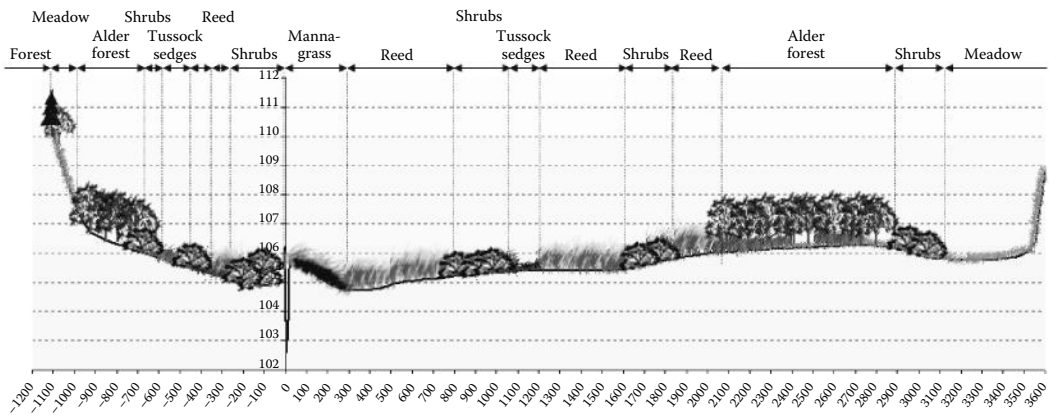
FIGURE 21.27 Cross section in the Lower Biebrza Basin; scenario—natural succession. (From Szporak, S. et al., Ann. Warsaw Unive. Life Sci.—SGGW Land Reclamat. , 40, 45, 2008.)
