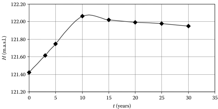
FIGURE 21.32 Forecast of water surface ordinates fluctuation of the Vistula River at the cross section at kilometer no. 371 Q = 6120 \text{ m}^3/\text{s} due to overgrowing of isles with willow vegetation.
