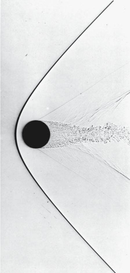
FIG. 8.3 Bow wave of a flying sphere
