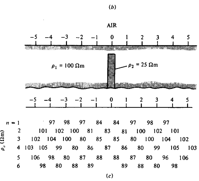
Figure 8.52. Effect of terrain on dipole-dipole resistivity survey. (a) Pseudodepth plot of \rho_a over 2-D ridge. (b) Model results for a 30° ridge. (c) Results over a buried vertical conductive dike.
