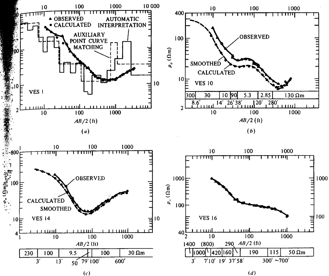
Figure 8.44. Soundings used to obtain geoelectric section in Figure 8.43. \blacktriangle and \circ denote observed and calculated values. (Note the alternative plotting methods used in (a) and (b); see also Figs. 8.29 and 8.42.) (After Zhody, Anderson, and Muffler, 1973.) (a) VES 1 interpreted by partial curve matching (6-layer) and complete curve matching (19-layer). (b) VES 10, partial curve matching (7-layer). (c) VES 14, partial curve matching (6-layer). (d) VES 16, complete curve matching (9-layer).
