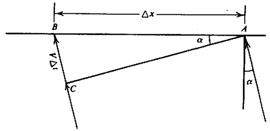
Figure 4.25. Finding the angle of approach of a wave.
