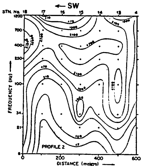
Profile 2 pseudo-section.
