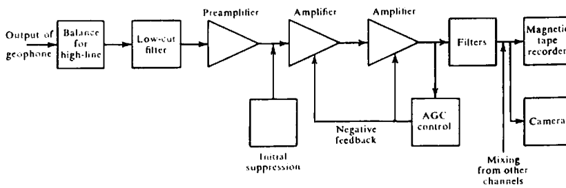
Figure 4.55. Block diagram of analog seismic amplifier.
