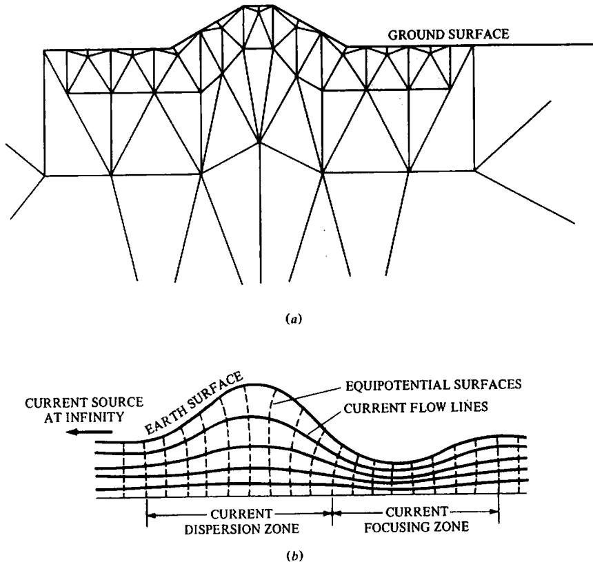
Figure 8.15. Effect of a 2-D ridge on a uniform field. (After Fox et al. 1980.) (a) Finite-element mesh used to calculate terrain effect of ridge. (b) Distortion of uniform field by ridge.
