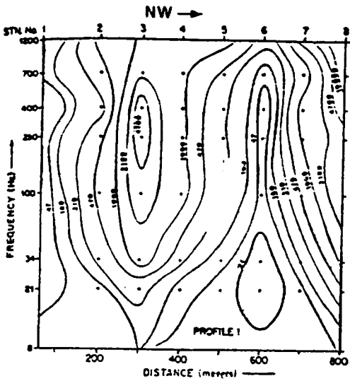
Profile 1 pseudo-section.
