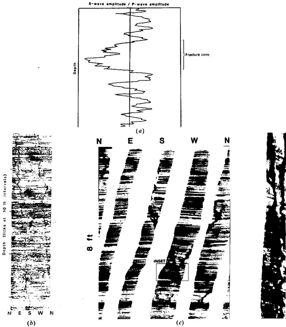
Figure 11.29. Fracture detection. (a) Fracture finder log showing low S-wave/P-wave amplitudes in a fractured zone. (After Labo, 1987.) (b) Fracture seen by a borehole televiwer. (Courtesy Gearhart Industries.) (c) Formation microscanner showing fractures. The microscanner uses a number of electrodes on each of four pads pressed against the borehole walls to give four swaths of closely spaced electric log responses. The sonde was twisting somewhat during this log run. (Courtesy Schlumberger.)
