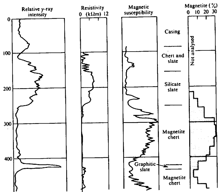
Figure 11.48. Gamma-ray, susceptibility, and resistivity logs in chert and slate beds.
