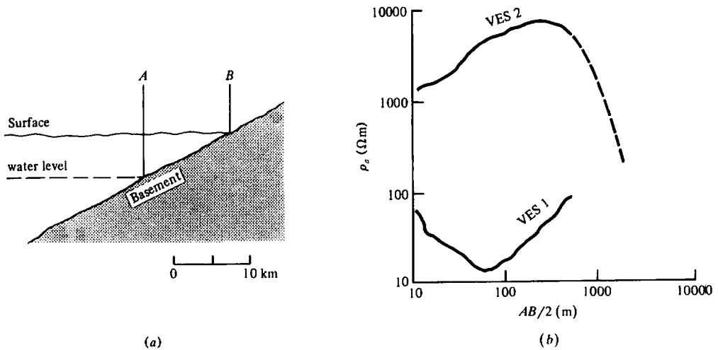
Figure 8.51. Example of "dry wedge" and related electric soundings for groundwater. (a) Vertical section. (b) Vertical sounding over the section.
