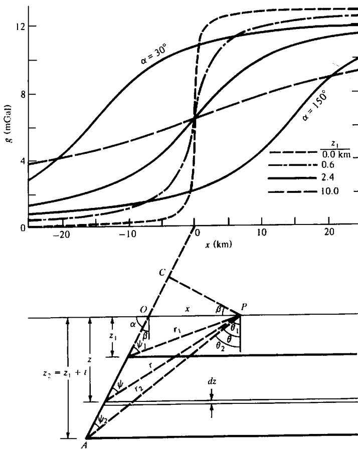
Figure 2.30. Gravity effect of a semiinfinite slab. t = 300 \text{ m} , \alpha = 90^\circ except where otherwise noted on the curves. \rho = 1 \text{ gm/cm}^3 .
