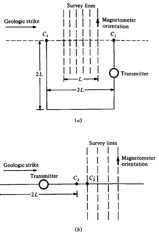
Figure 9.9. Magnetic IP arrays. (After Seigel, 1983.) (a) Horseshoe array for reconnaissance. (b) Linear array for detail surveying.
