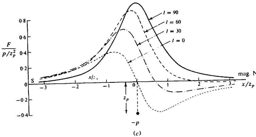
Figure 3.14. (Continued) (b) Contours of |\mathbf{H}_R| = |\mathbf{H} + \mathbf{H}_e| for H_{max} = H_e = 0.38 . (c) F profiles for various inclinations. (After Smellie, 1967.)
