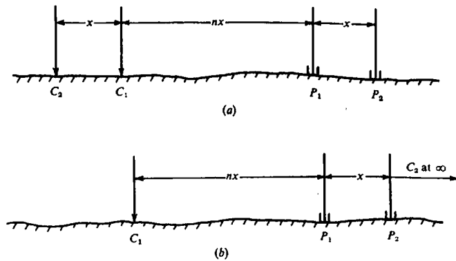
Figure 9.8. Typical IP spreads. (a) Double-dipole. (b) Pole-dipole.
