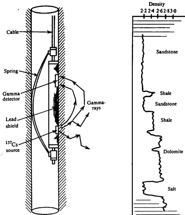
Figure 11.35. Density log schematic and typical log.
