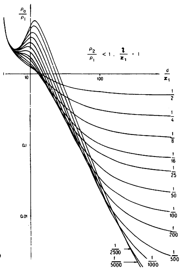
Figure 7.76. Master curves of late-time (\rho_s/\rho_1) versus (d/z_1) . [Parts (a) and (b): After McNeill, 1980; parts (c) to (f): After Kaufmann and Keller, 1983.] (a) Two-layer curves for resistive basement. (b) Same as (a) except for conductive basement.
