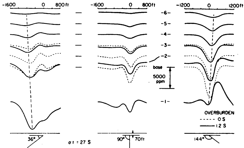
Figure 7.90. Model profiles over dipping half-plane ( \sigma t = 27 S, depth to top = 70 ft) under conductive overburden. Dashed line indicates shift of anomaly peak from early to late time. (After Palacky, 1975.)
