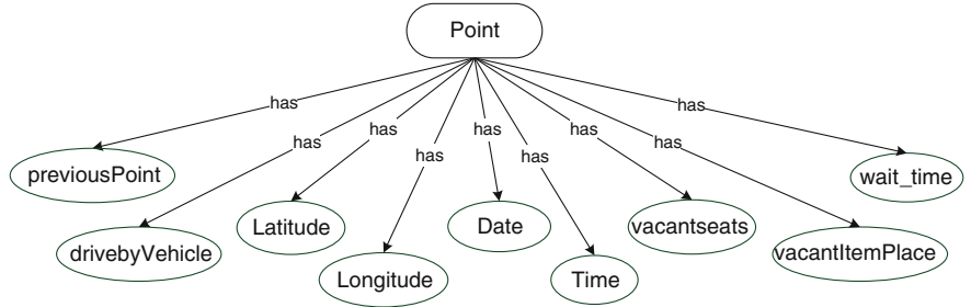
Fig. 4 Class “Point”
