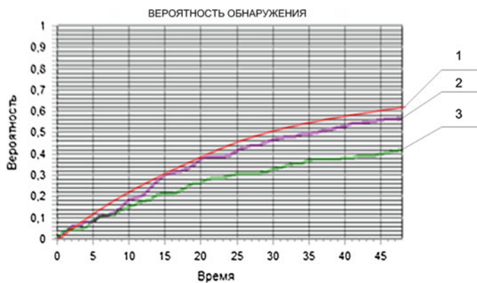
Fig. 8 Modeling results
