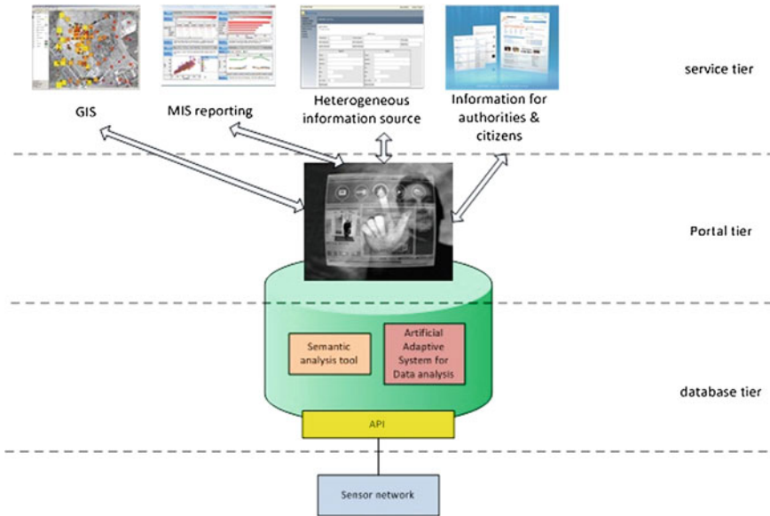
Fig. 4 System architecture
