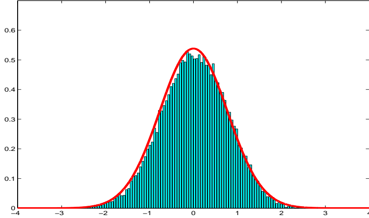
Fig. 3.5 Histogram of \Delta n_R for a Rayleigh-faded channel with n_T = 5 and n_R = 10 . The transmit antennas are correlated as per (3.182) while the receive antennas are uncorrelated. Solid line indicates the corresponding limiting Gaussian distribution.
