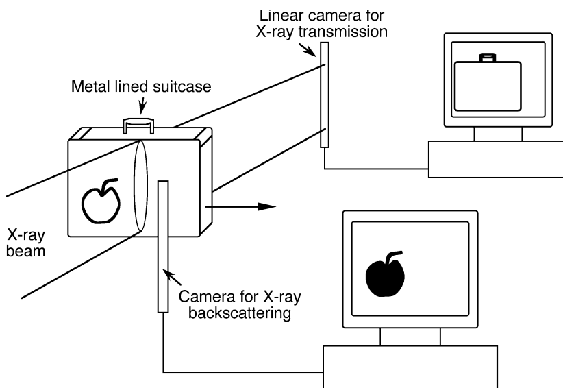
Fig. 4.40 Detection of biological and other organic material behind a metal layer with X-ray backscattering: since the absorption of biological material is much smaller than that of metal, the biological material is difficult to detect in single-wavelength X-ray absorption measurements. X-ray backscattering provides much better contrast in this application. However, the quantum efficiency of X-ray scattering is low and thus relatively large exposures and sensitive cameras must be used
