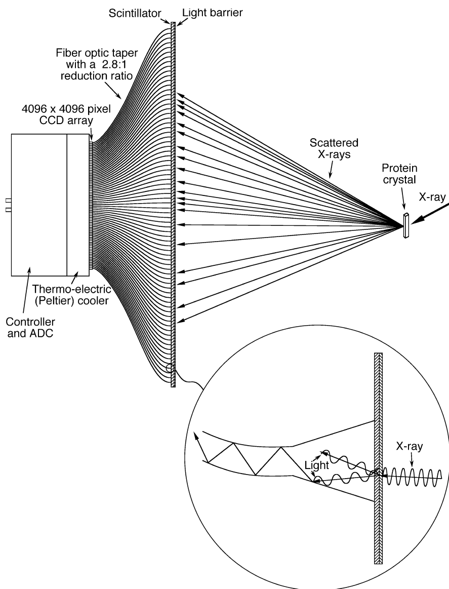
Fig. 4.20 A CCD area detector used for recording of X-ray diffraction patterns. For reduction of the dark current, this CCD is operated at -40^{\circ}\text{C} , allowing it to detect single photons. The fiber optic taper serves also for blockage of X-rays and thereby prevention of radiation damage to the sensitive CCD array. At a pixel size of 20\ \mu\text{m} \times 20\ \mu\text{m} , the full well capacity is typically several 100,000 electrons per pixel, enabling the necessary high dynamic range
