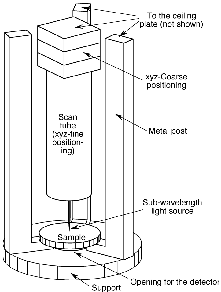
Fig. 7.25 A design of a SNOM with a xyz-coarse positioning and a xyz-fine positioning
