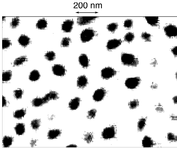
Fig. 7.33 Absorption of latex beads with approximately 100 nm diameter taken with a SNOM at a resolution of about 50 nm (OMICRON, Taunusstein, Germany)
