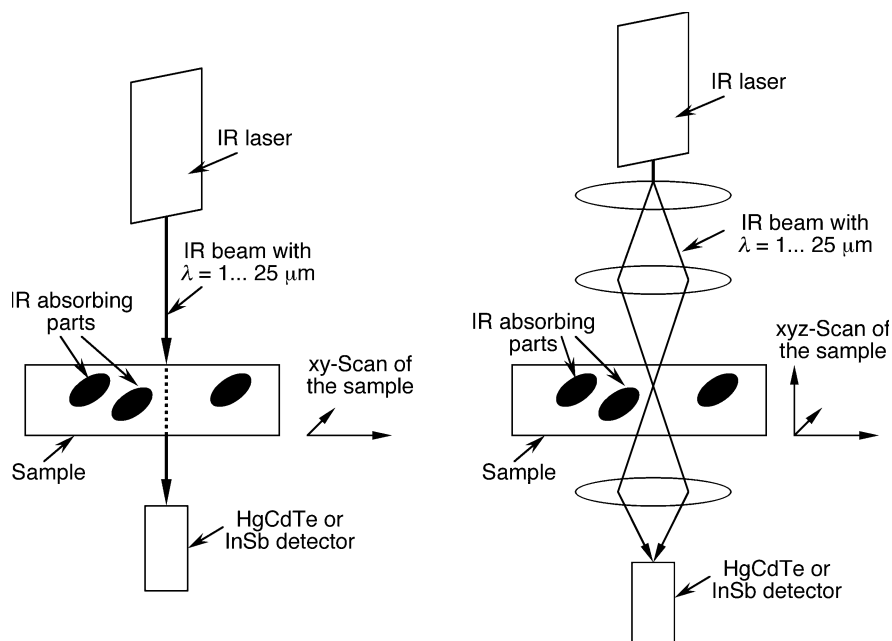
Fig. 5.14 Scanning IR microscope. The focussed beam from an IR laser is passed through the sample and detected. Left: simple microscope with planar resolution, especially suitable for thin layer samples. Right: microscope with three-dimensional resolution: for acquisition of the image, the sample is moved in xyz-directions
