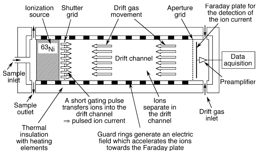
Fig. 10.5 Design of an IMS (Cohen and Karasek, 1970; Karasek, 1970; Caroll et al., 1971; Eiceman and Karas, 1994; Matz and Schröder, 1996, 1997; IUT Institute for Environmental Technologies, Berlin, Germany; Bruker Daltonik, Bremen, Germany; Graseby Dynamics, London, U.K.; Barringer Instruments, Warren, NJ). The ionization source ionizes sample molecules. Guard rings generate an electric field which accelerates the sample ions towards the shutter grid where they accumulate. After a few seconds, a voltage pulse is applied to the shutter grid causing the release of the sample ions into the drift channel. Now the electric field can further move the sample ions towards the ion detector (Faraday plate). Different ions interact differently with the drift gas molecules in the drift channel. This causes the ions to spread out according to their different mobilities. The recorded ion mobility spectrum corresponds to differences in the time of flight of the sample ions. Typically, the drift channel has a length of a few cm, and the electric field strength of in the drift channel is 100\text{--}1000\text{ V cm}^{-1} . At this field strength and length, small organic compounds which have mobilities of a few \text{cm}^2\text{ V s}^{-1} need about 1–100 milliseconds to reach the detector. Biomacromolecules typically travel about 1–3 orders of magnitude slower. Drift channel and reaction area are enclosed in a thermal isolation with heating elements. The operating temperature for the detection of biological agents is typically 100\text{--}150\text{ }^{\circ}\text{C}
