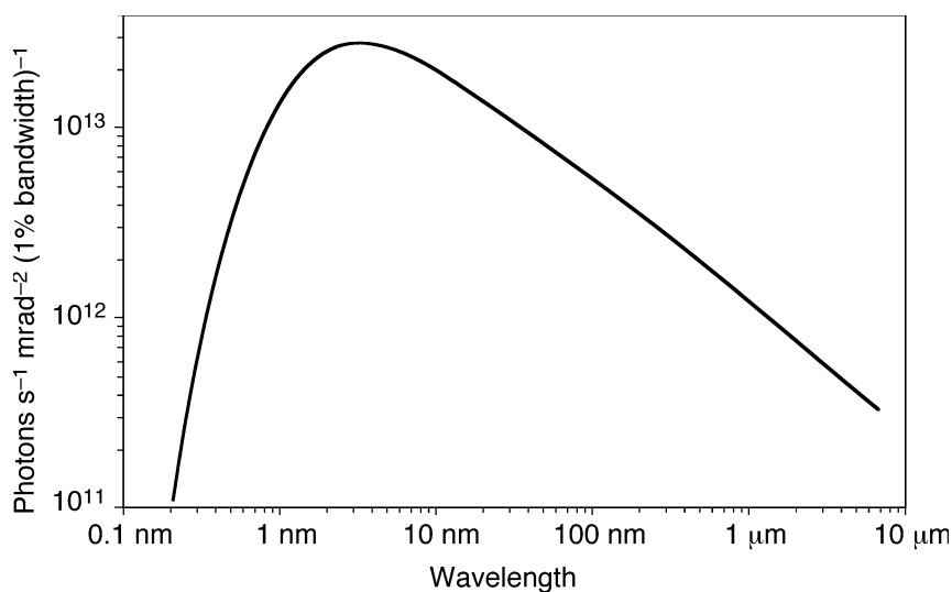
Fig. 4.24 Emission of the Berlin Electron Synchrotron Storage Ring (BESSY I)
