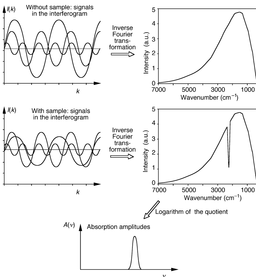
Fig. 5.6 Principle of operation of a FTIR spectrometer. IR intensities at the detector are recorded both for the sample cell filled with solvent and for the sample cell filled with sample. Inverse Fourier transformation of the two interferograms yields the IR intensities. The IR absorption spectrum is calculated using the logarithm of the intensity quotient
