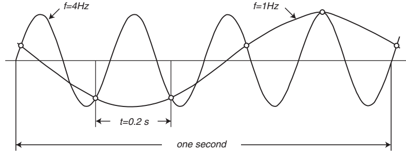
Figure 16.4 Sampling a 4 Hz sine wave (heavy line) every 0.2 s aliases the frequency to 1 Hz (light line). The critical frequency is 1/(2 \times 0.2\text{ s}) = 2.5\text{ Hz} , which is less than 4 Hz.
