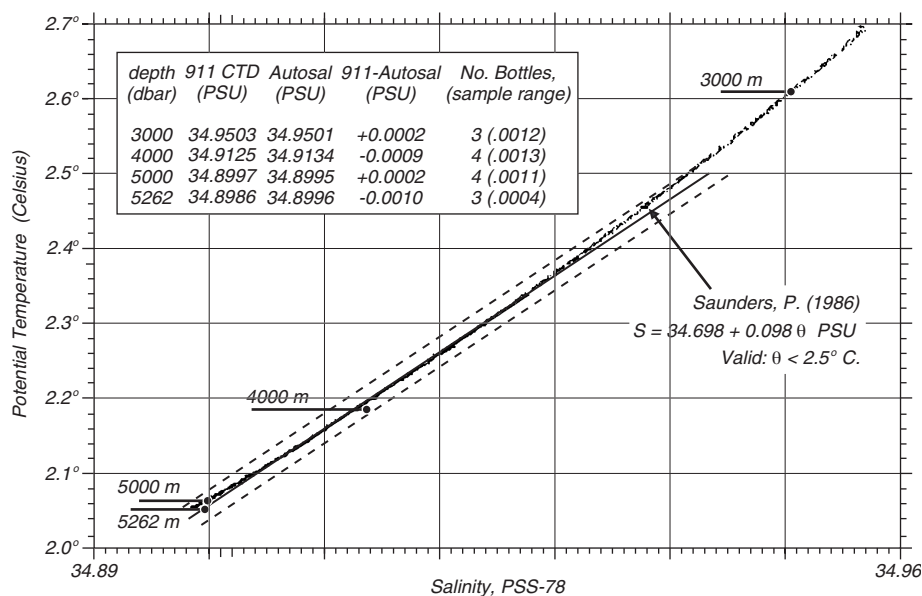
Figure 6.15. Results from a test of the Sea-Bird Electronics 911 Plus CTD in the North Atlantic Deep Water in 1992. Data were collected at 43.17^{\circ} \text{N} and 14.08^{\circ} \text{W} from the R/V Poseidon. From Sea-Bird Electronics (1992).
