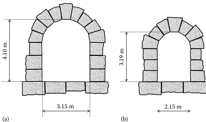
FIGURE 9.20 Sections of the wastewater collector of the Cloaca Maxima in Rome: (a) near Forum Augustum and (b) near Via del Velabro .
