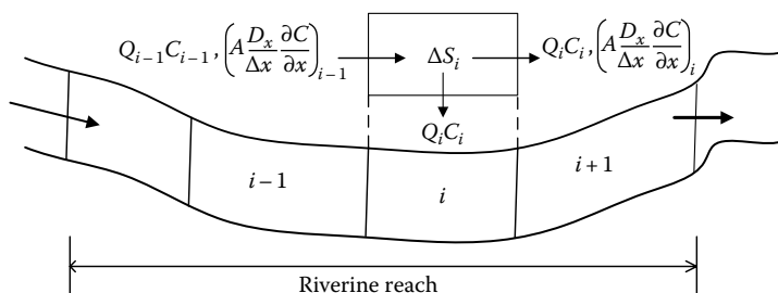
FIGURE 13.5 A conceptualization of the 1D river reach constituent transport and mass balance model.
