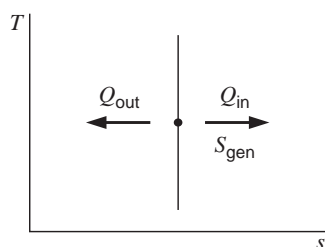
FIGURE 8.16 Change of entropy due to heat transfer and entropy generation.
