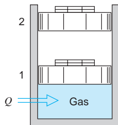
FIGURE 5.7 The constant-pressure quasi-equilibrium process.
