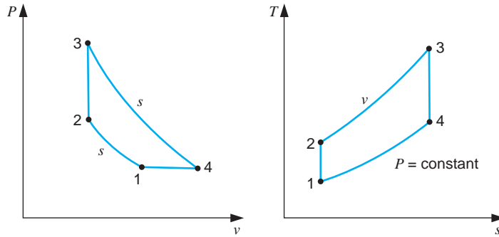
FIGURE 12.18 The Atkinson cycle.
