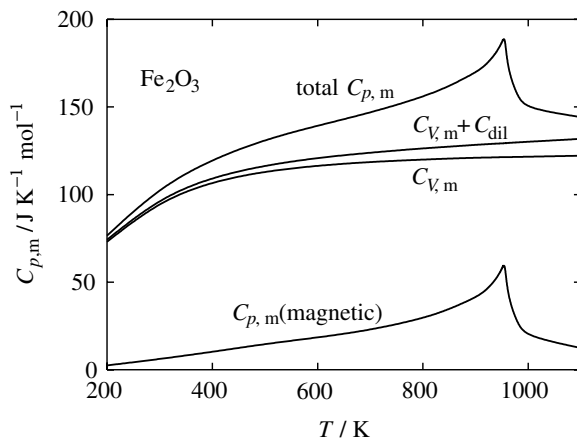
Figure 8.23 Heat capacity of Fe 2 O 3 [18]. The heat capacity is deconvoluted to show the relative magnitude of the main contributions. C_{\text{dil}} = C_{p,m} - C_{V,m} = \alpha^2 TV / \kappa_T .
