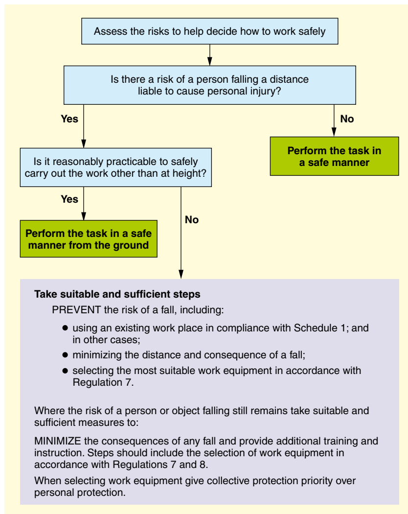
Figure 15.9 Work at Height – flowchart
