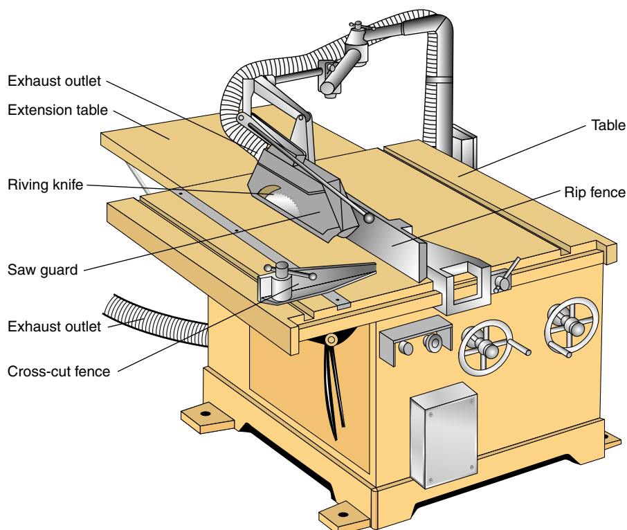
Figure 9.30 Typical bench mounted circular saw
