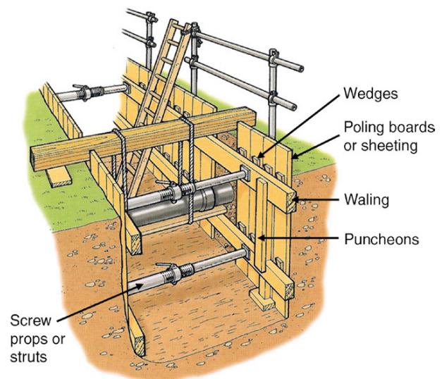
Figure 6.20 Timbered excavation with ladder access and supported services (guard removed on one side for clarity).
