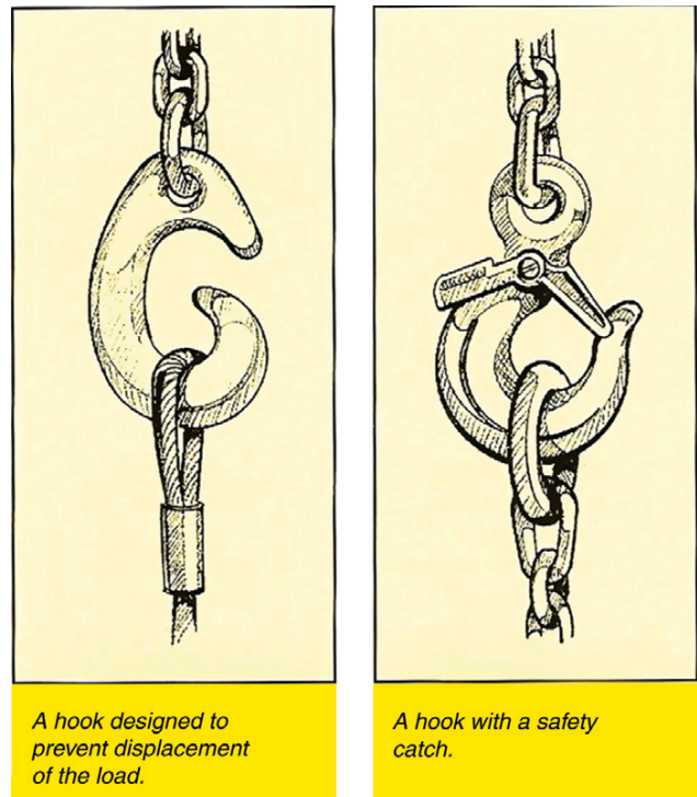
Figure 8.16 Specially designed safety hooks. Source HSE
