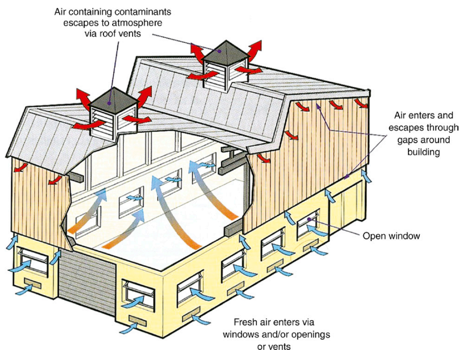
Figure 6.2 Natural ventilation in a building. Source HSE.
