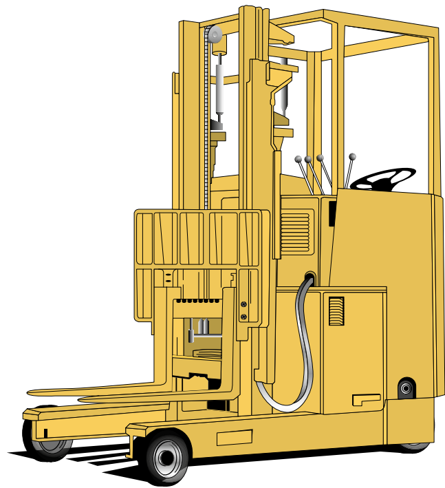
Figure 8.13 Reach truck, designed so that the load retracts within the wheel base to save space
