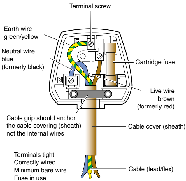
Figure 10.14 UK standard 3-pin plug wiring
