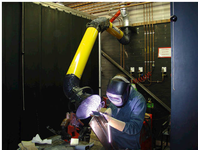
Figure 12.12 a) An LEV system, b) Welding with an adjustable LEV system to remove dust and fumes
