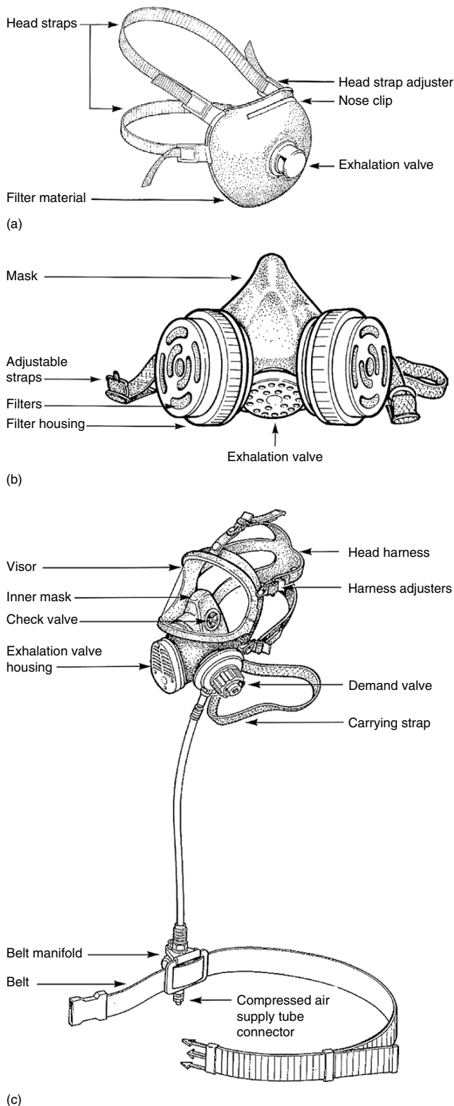
Figure 12.15 Types of respiratory protective equipment. a) Filtering half-mask; b) half-mask – re-usable with filters; c) compressed air-line breathing apparatus with full face fitted with demand valve. Source HSE
