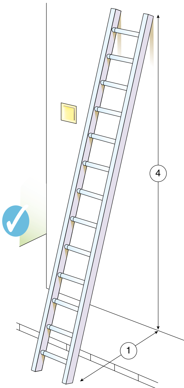
Figure 6.14 Ladder showing correct 1 in 4 angle (means of securing omitted for clarity of illustration)
