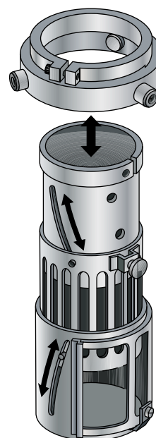
Figure 9.14 Adjustable guard for a rotating shaft, such as a pedestal drill
