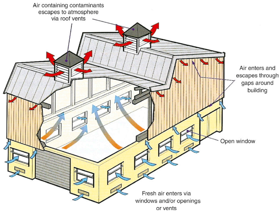
Figure 12.13 Natural ventilation in a building. Source HSE
