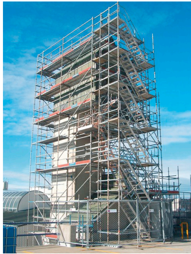
Figure 14.16 Scaffolding with good access stairs
