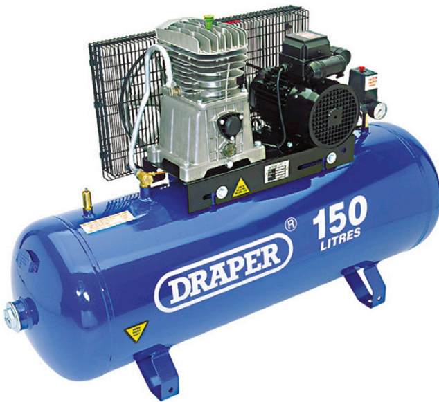
Figure 9.4 Typical electrically powered compressor with air receiver
