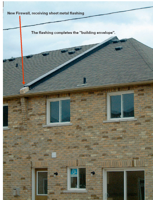
Figure 11.17 Fire break wall between dwellings
