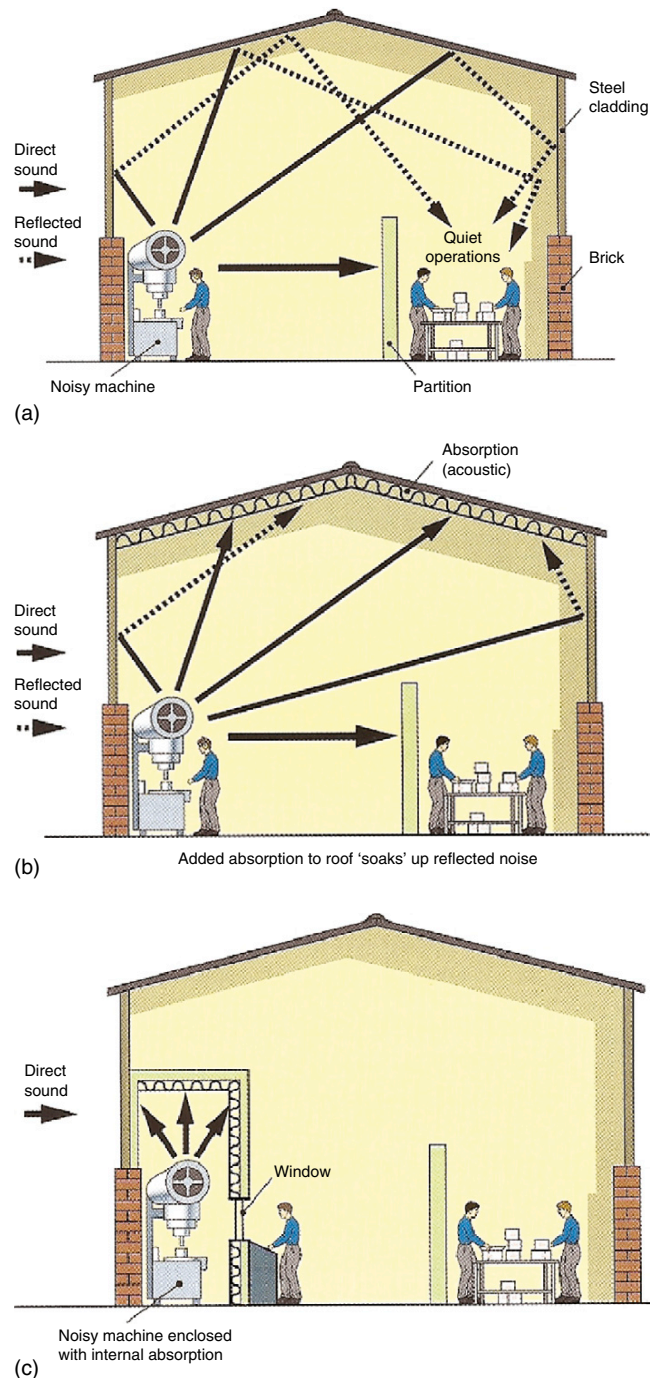
Figure 13.4 a) Noise paths found in a workplace. The quiet area is subjected to reflected noise from a machine elsewhere in the building, b) The correct use of roof absorption will reduce the reflected noise, c) Segregation of the noisy operation will benefit the whole workplace.
