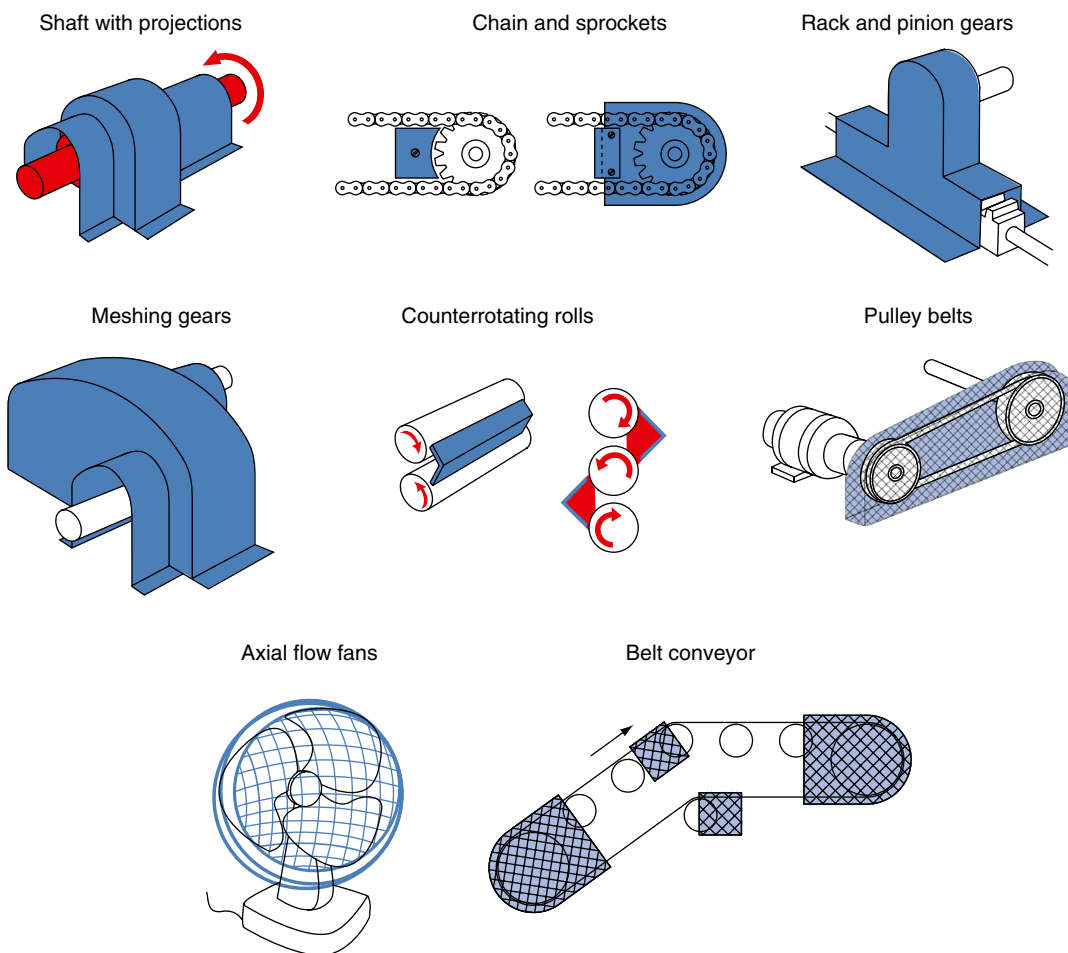
Figure 9.13 Range of fixed guards
