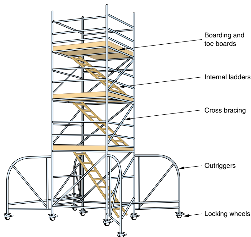
Figure 6.18 Typical prefabricated tower Scaffold
