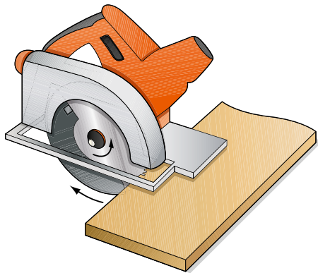
Figure 9.15 Self-adjusting guard on a circular wood saw
