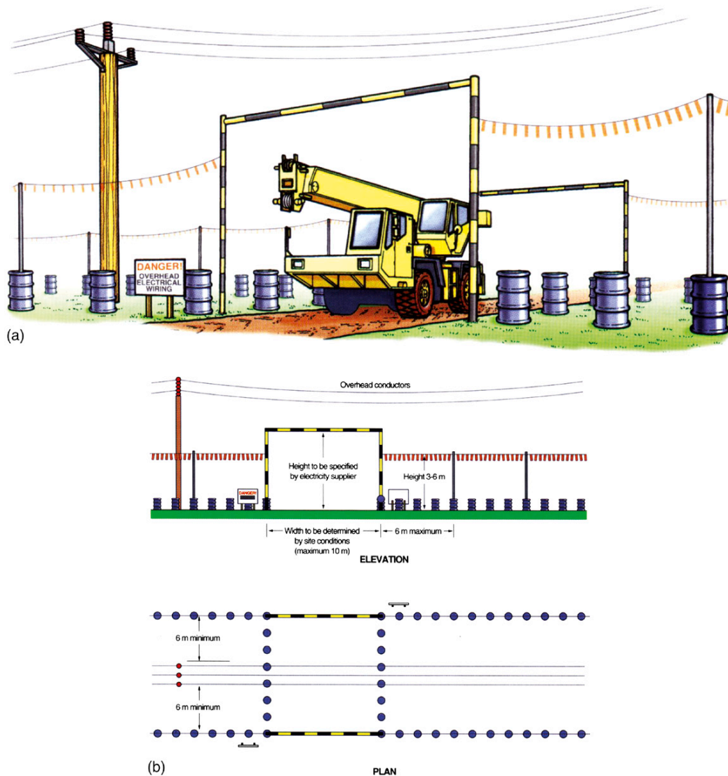
Figure 10.12 a) Precautions for overhead lines: ‘goalpost’ crossing points beneath lines to avoid contact by plant, b) Diagram showing normal dimensions for ‘goalpost’ crossing points and barriers. Reproduced from HSG185 Health and Safety Excavations
