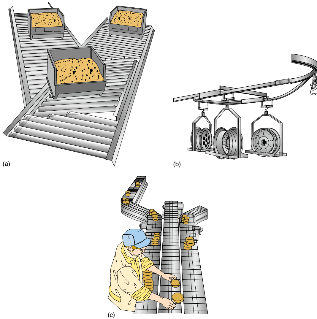
Figure 8.11 Conveyor systems: (a) roller conveyor (these may have powered and free running rollers); (b) an overhead conveyor moving wheels. Other designs of overhead conveyor are useful for transferring components and garments between workstations, in, for example, manufacture of machines or clothing; (c) a slat conveyor in use in a food factory
