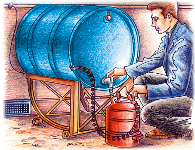
Figure 11.18 Earth bonding of containers to prevent a static discharge – Cotton outer clothing and conductive footwear should be used
