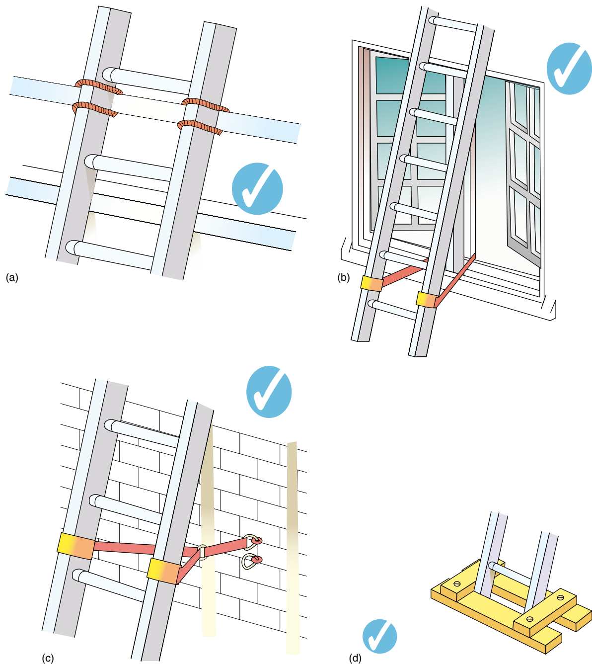
Figure 6.15 (a) Ladder tied at top style (correct for working on, not for access); (b) tying part-way down; (c) tying near base; (d) securing at base.
