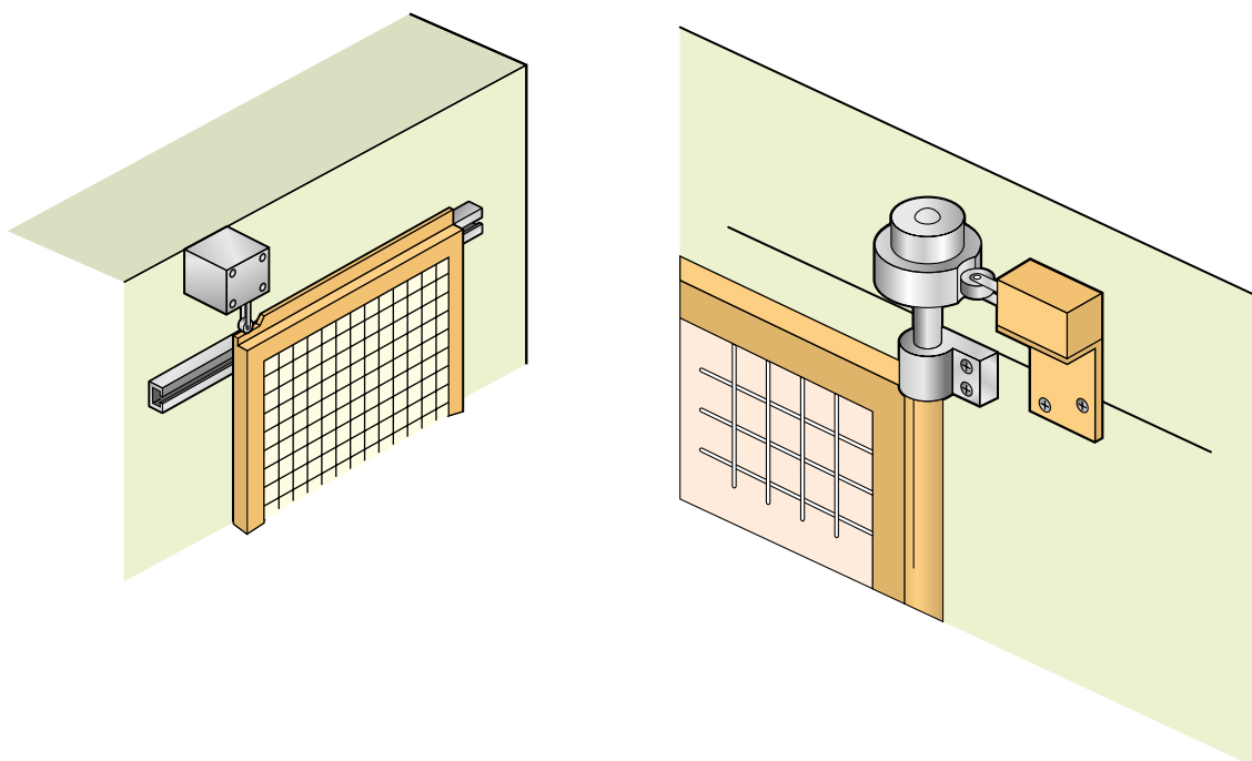
Figure 9.16 Typical sliding and hinged interlocking guards
