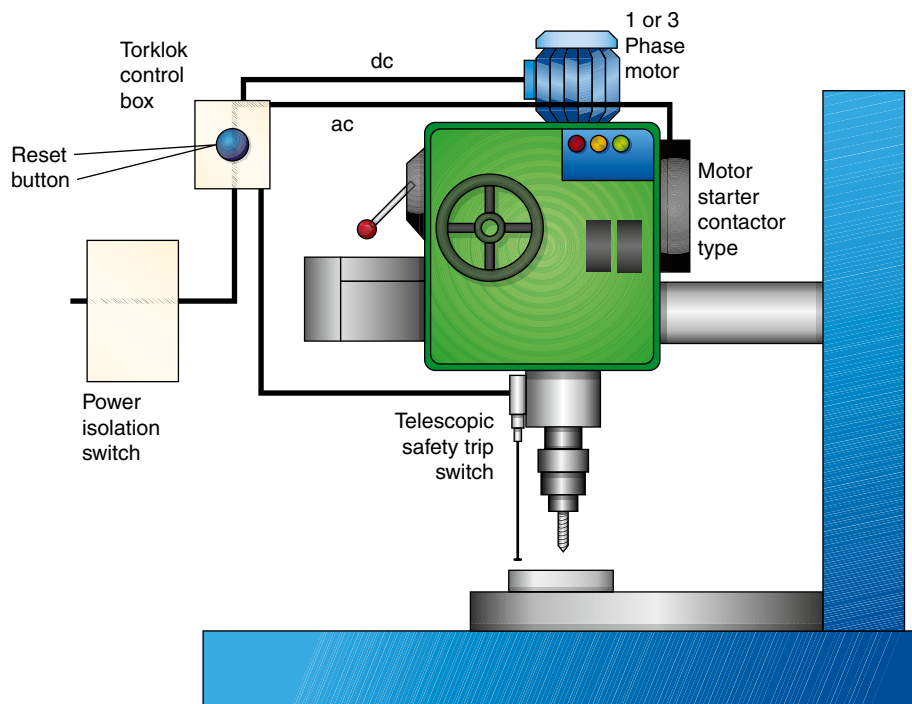
Figure 9.17 Schematic diagram of a telescopic trip device fitted to a radial drill
