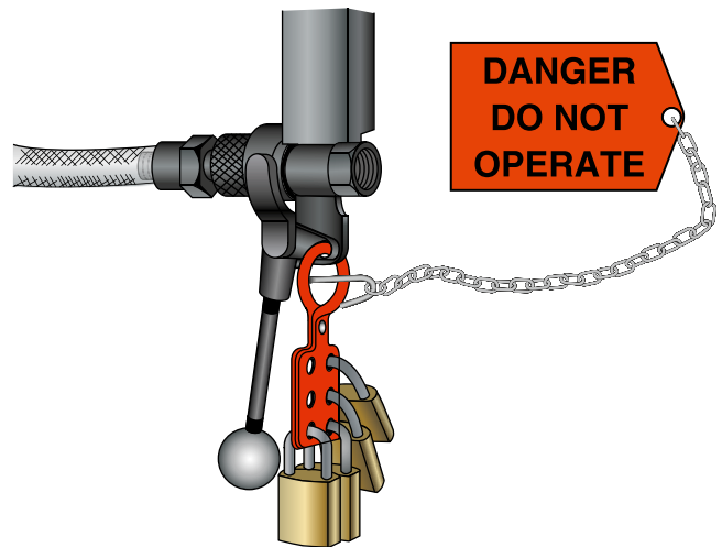
Figure 4.26 Multipadlocked hasp for locking off an isolation valve – Each worker puts on their own padlock
