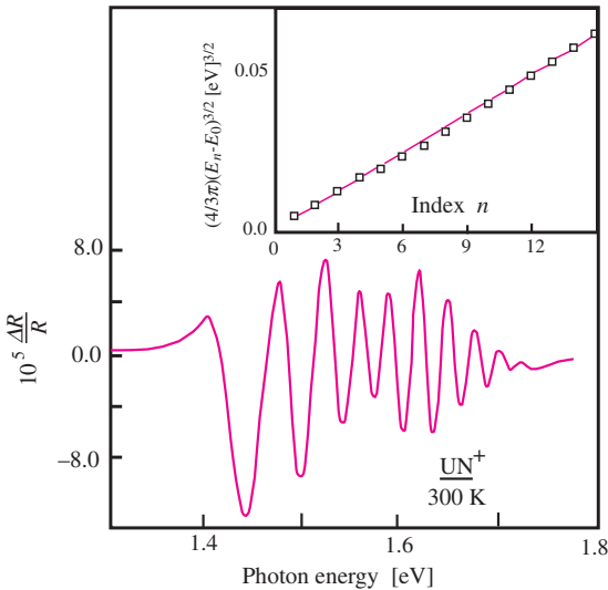
Fig. 6.53. Photoreflectance spectrum of a GaAs sample at room temperature obtained with a 633 nm laser for a modulating power between 3\text{ }\mu\text{W cm}^{-2} and 2\text{ }\mu\text{W cm}^{-2} . The inset shows a plot of (4/3\pi)(E_n - E_0)^{3/2} as a function of the index n which labels the extrema [6.130]
