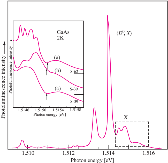
Fig. 7.10. Photoluminescence of GaAs at 2 K measured by Sell et al. [7.25]. The inset is an enlargement of the spectra within the rectangle labeled X. It contains the part of the emission spectrum associated with free excitons. The spectrum in the inset labeled (a) and those labeled (b) and (c) correspond to two different samples. The spectrum (c) was excited by light intensity ten times higher than that used for spectrum (b). The peak labeled ( D^0, X ) is attributed to recombination of excitons bound to neutral donors
