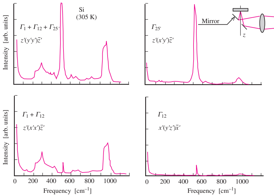
Fig. 7.22. First (peak at 520 \text{ cm}^{-1} ) and second order Raman spectra of Si obtained in the scattering geometry shown in the inset . The notations for the scattering configuration in each spectrum are defined in Sect. 7.2.2. (From [7.68])
