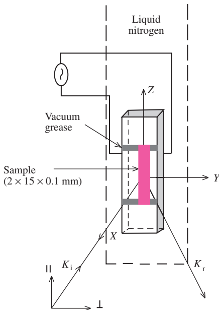
Fig. 6.46. Details of the piezoelectric transducer modulator arrangement used by Gavini and Cardona [6.113] for piezorefectance measurements. The black-shaded parallelepiped represents a lead zirconate-titanate (PZT) transducer. The ends of a thin (100 \mu\text{m} ) sample (shaded red) are glued to the transducer with vacuum grease (shaded black) which freezes at low temperatures, thus giving a strong bond to the transducer
