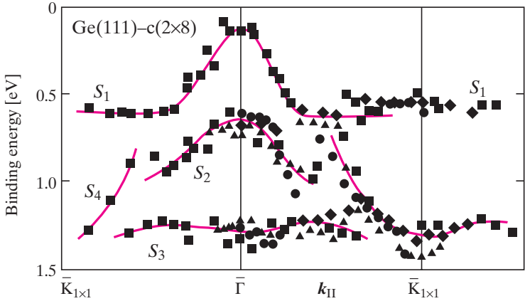
Fig. 8.25. Dispersion of the Ge(111)-c(2 × 8) surface bands measured by angle-resolved UPS. Note that the results are plotted in the BZ of the unreconstructed (1 × 1) unit cell, which is an extended zone of the reconstructed structure. (The different symbols represent results from different groups) [Ref. 8.11, p. 186]. The red lines are drawn through the measured points as a guide to the eye
